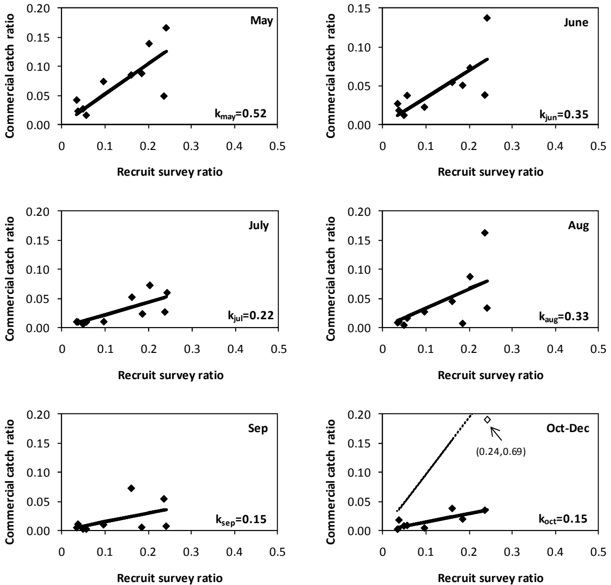
Figure A2. The regressions of the ratio of small sardine bycatch : anchovy 16 in the monthly commercial catch against that observed in the recruit survey, i.e. minimising \sum_{y=2002}^{2011} \left[ \left( C_{y,m}^{S,byc} / C_{y,m}^A \right) - k_m \left( N_{1,y,r}^{S,obs} / N_{1,y,r}^{A,obs} \right) \right]^2 w.r.t. k_m . The outliers of commercial ratio of 0.69 in October to December 2010 (shown as an open diamond) is removed, as this could have been biased by the mid-water trawl experiments which occurred during this time. The regression including this outlier is given by the dotted line.
