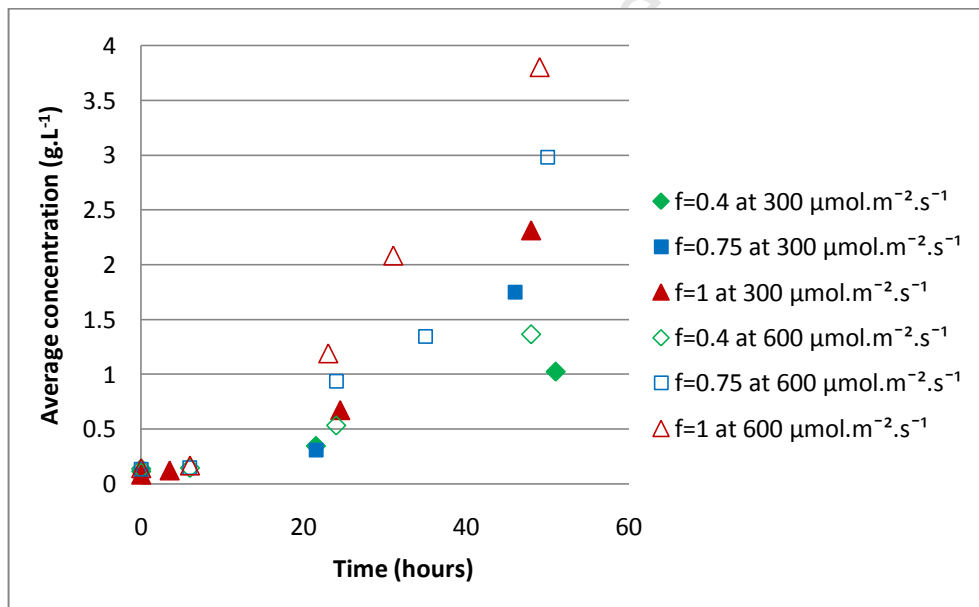
Figure 6. 3: The effect of light intensity and light fraction ( f = t_l/t_c ) on the biomass concentration of Scenedesmus sp. in the tubular photobioreactors at 25 \pm 1^\circ\text{C} at (a) a cycle time of 33 s and (b) a cycle time of 21 s (diamond, square and triangle symbols represent light fractions of 0.4, 0.75 and 1 respectively)
