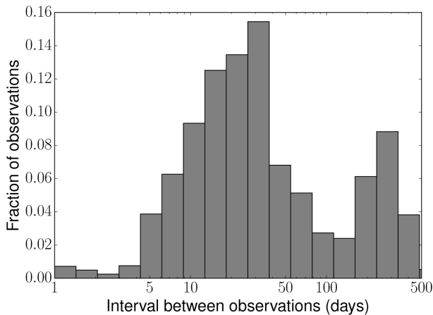
Figure 3. Distribution showing the interval, in days, between CRTS observations. The median interval was 28 d, 16 per cent of the intervals were less than 10 d, and 61 per cent were between 10 and 100 d.
