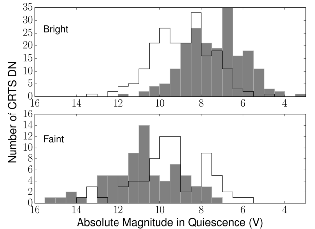
Figure 13. Distribution of the quiescent absolute magnitudes for the DN with distance limits. Top panel: bright limit for the quiescent absolute magnitude ( V_Q^{\text{lim},b} ). The solid line gives the equivalent estimate ( V_Q^b ). Bottom panel: faint limit for the quiescent absolute magnitude ( V_Q^{\text{lim},f} ). The solid line gives the equivalent estimate ( V_Q^f ).
