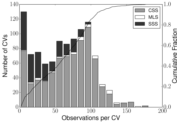
Figure 5. Distribution showing the number of CRTS observations per CV over the time range used to make this catalogue, as well as the normalized cumulative distribution. The sampling cadence is uneven, and varies as a function of time and position on-sky. The variation between the subsurveys is as a result of the different survey lengths and observing strategies (see Drake et al. 2014). Note that CVs with non-unique CRTS identifiers are only plotted once – if a CV is detected in more than one subsurvey it will be plotted under its CSS identifier.
