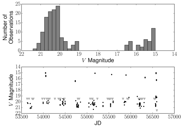
Figure 2. Illustration of the initial classification step (see Fig. 1), where the light curve (bottom panel) is histogrammed by magnitude (top panel) in order to determine whether it shows standard DN-type behaviour. In this example, the CV was given the initial classification of ‘DN’, because the higher histogram peak is in the fainter half of the magnitude range – as one would expect from a DN that spends the majority of its time in quiescence. Subsequent tests in the script confirmed the ‘DN’ classification, counted seven outbursts, and estimated v_Q = 20.1 mag and v_O < 15.5 mag. Note that the non-detections in the light curves are shown at the typical detection limit of the survey (currently the CRTS data release does not provide upper limits).
