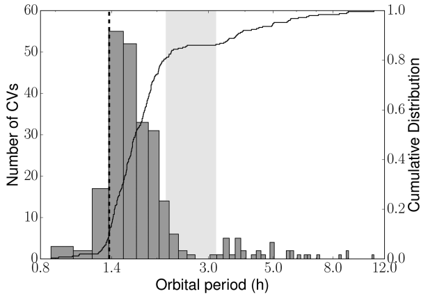
Figure 6. Orbital period distribution of the CRTS CVs with known P_{\text{orb}} in RKCcat (Ritter & Kolb 2003). The cumulative distribution is indicated by the solid line, the shaded region indicates the period gap (with boundaries at 2.15 and 3.18 h; Knigge 2006) and the dotted line indicates the period minimum determined from the SDSS CVs ( \approx 82 min; Gänsicke et al. 2009). The nova X Serpentis ( P_{\text{orb}} = 35.52 d; see Thorstensen & Taylor 2000) has been omitted for clarity.
