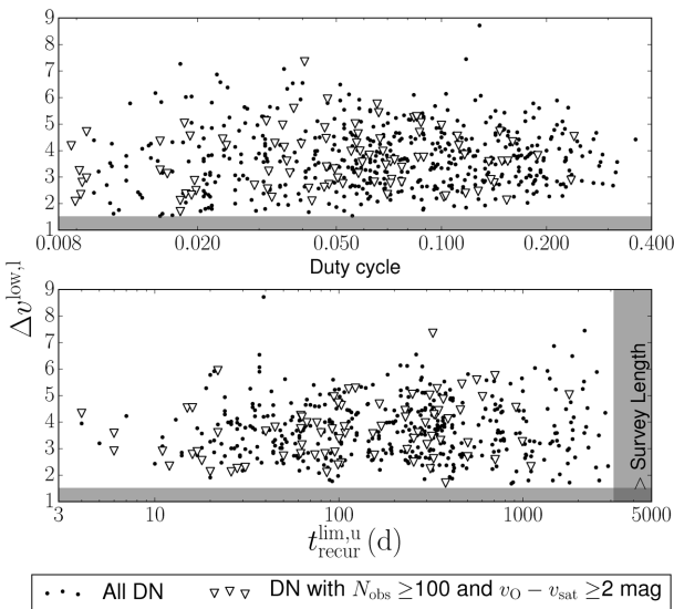
Figure 9. Distribution of the outburst amplitude lower limit with duty cycle (top panel), and the upper limit on the recurrence time (lower panel). The shaded regions indicate where the range exceeds the survey length, and where the outburst amplitude is smaller than 1.5 mag. The well-sampled DN (those with more than 100 CRTS observations that did not have v_{\text{O}}^{\text{lim,f}} within 2 mag of the saturation limit) are indicated to show that the observational effects are not masking correlations between the properties. The density fluctuations in the recurrence time limit are as a result of CRTS observing cycles due to seasonal variations.
