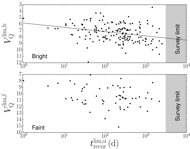
Figure 15. Distribution of the bright- and faint limit of the absolute magnitude in quiescence with respect to the upper limit on the outburst recurrence time. The solid line indicates the linear least-squares fit.
