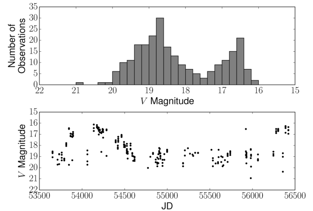
Figure 4. Example of a light curve that was designated as ‘non-DN’ by the classification script because it shows high states and low states in the light curve (see Fig. 1). Magnetic CVs typically show high states in their optical light curves.
