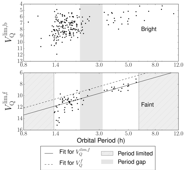
Figure 14. Variation of the quiescent absolute magnitudes with P_{\text{orb}} . See the text for a description of the symbols. The period gap is indicated by the grey region in both panels. Top panel: V_Q^{\text{lim},b} is directly derived from P_{\text{orb}} , so this is plotted purely for comparison purposes. Bottom panel: the solid and dashed lines indicate the linear least-squares fit to V_Q^{\text{lim},f} , and V_Q^f , respectively. The range of orbital periods for which this distance determination method is not appropriate is indicated by the hatched region.
