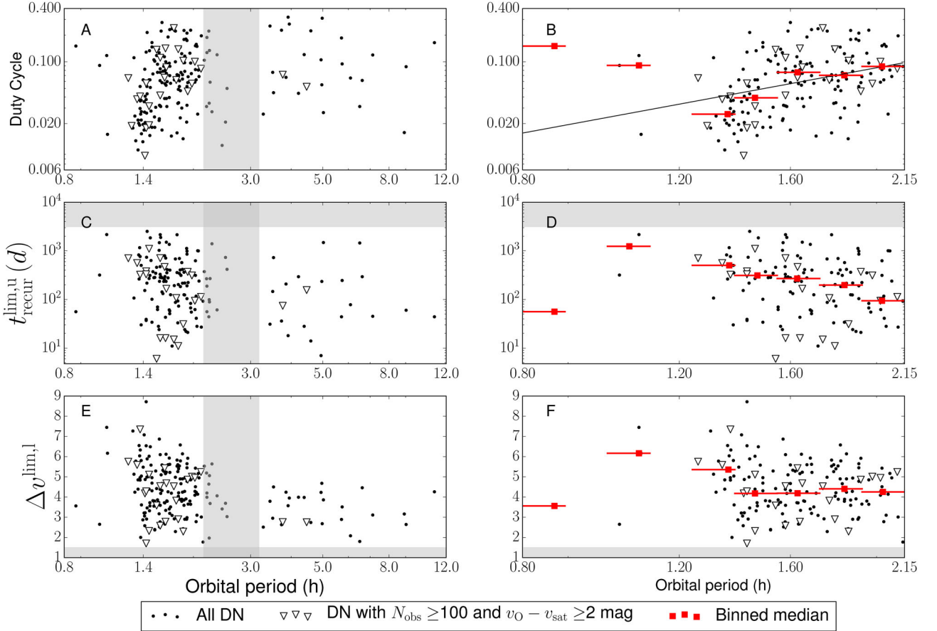
Figure 11. The dependence of the outburst properties (duty cycle, upper limit on the recurrence time and lower limit on the outburst amplitude) on the orbital period. The panels on the left show the full P_{\text{orb}} range, while the panels on the right show the range P_{\text{orb}} < 2.15 h. Red squares indicate the median value within a given logarithmic period bin (the size of which is indicated by the error bars), to show the trend. The shaded regions indicate the period gap and survey limits. The nova X Serpentis ( P_{\text{orb}} = 35.5 d, see Thorstensen & Taylor 2000) has been omitted for clarity.
