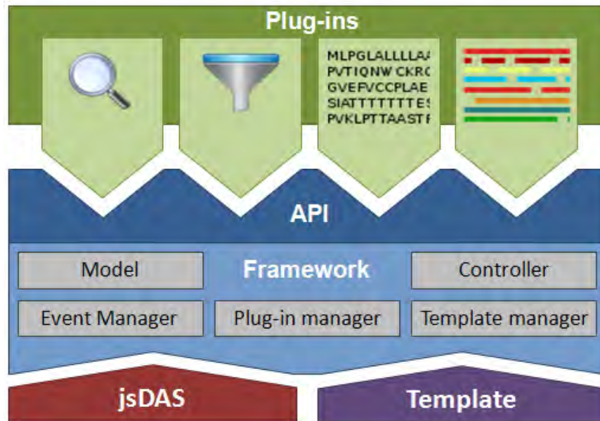
Figure 2.3.1: DASTy3 Architecture
