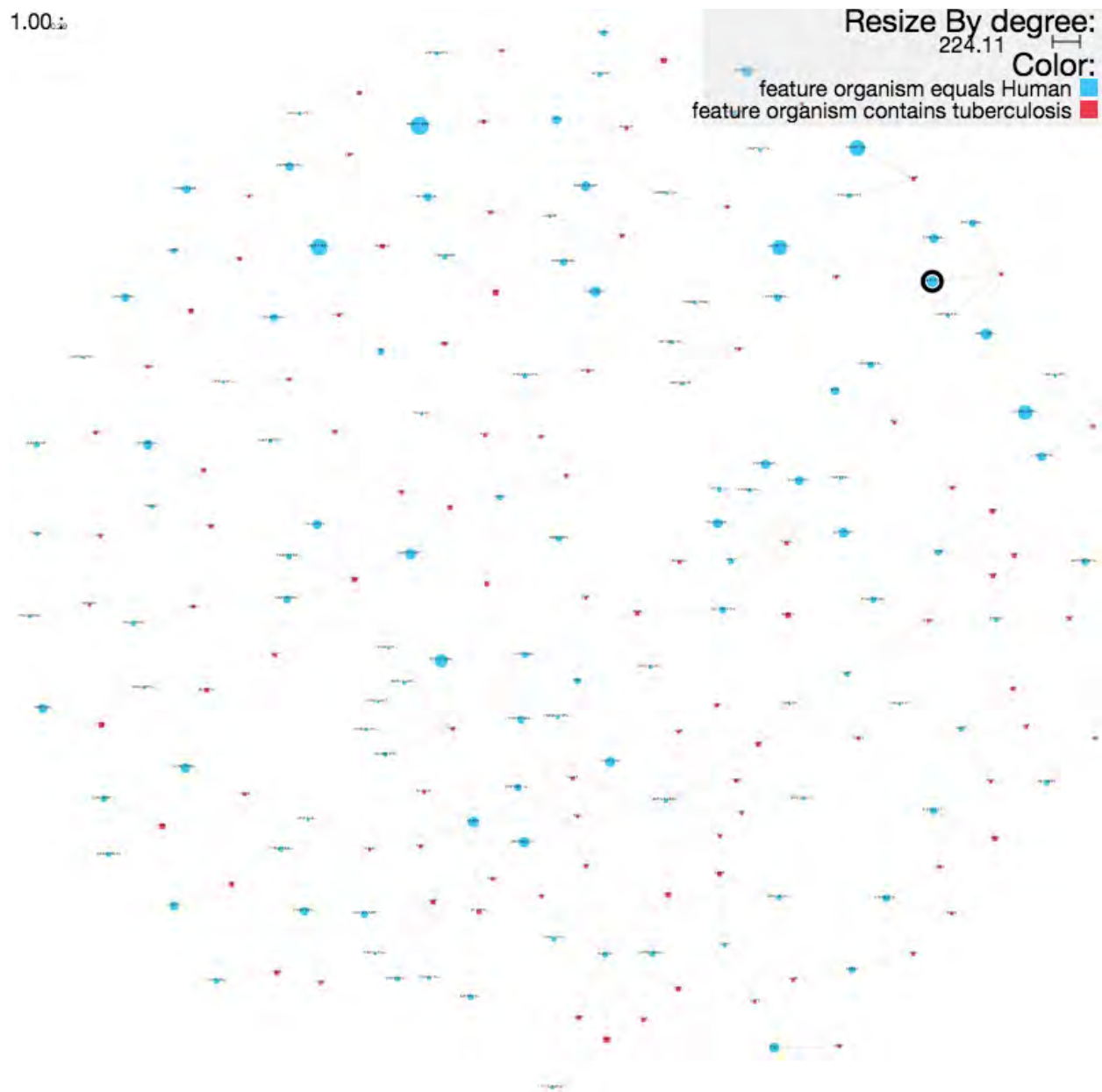
Figure 4.1.1: Predicted functional interactions between MTB and Human. Blue circles are human proteins while red squares are from the MTB microorganism.
