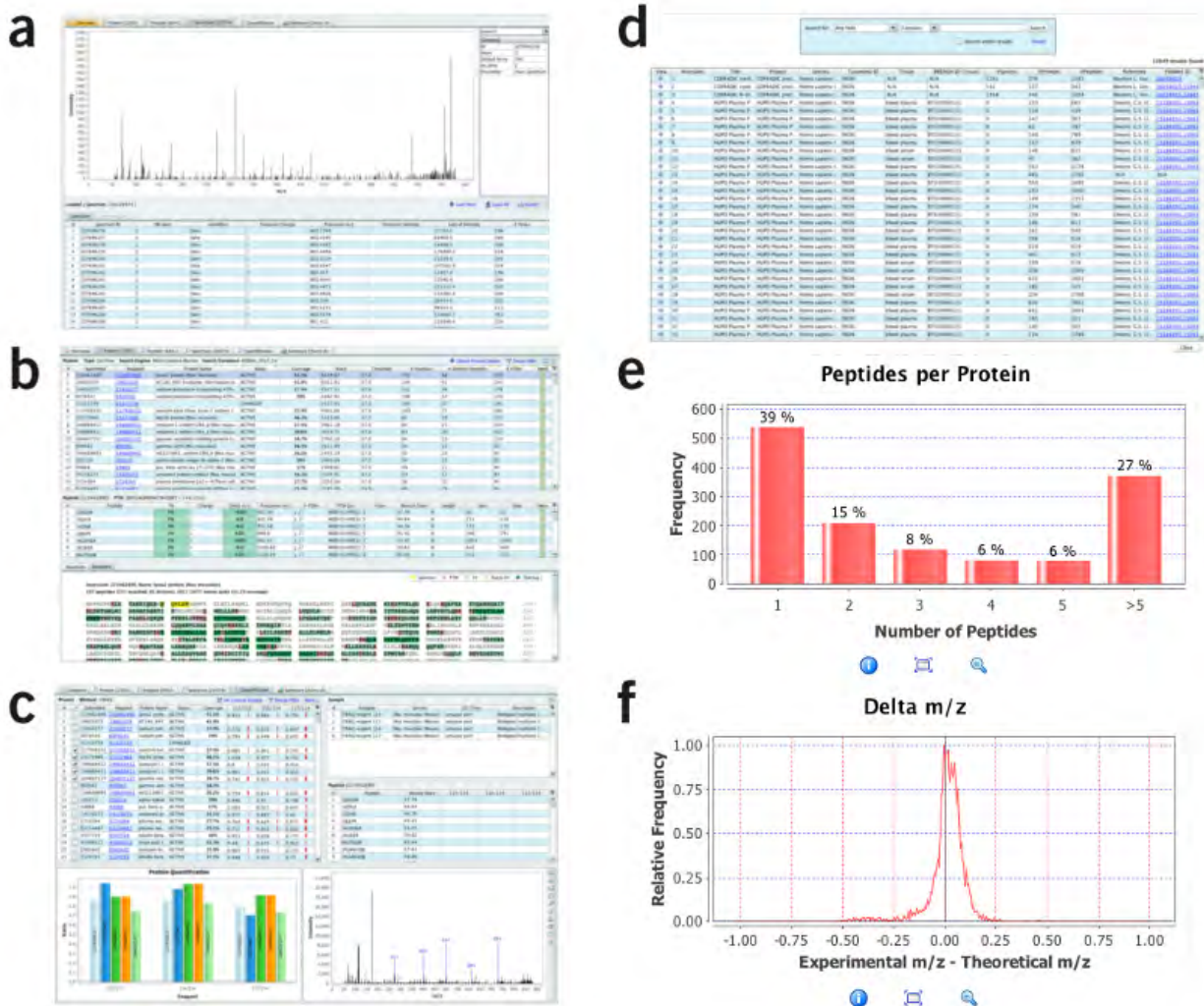
Figure 1.2.9: Snapshots of the PRIDE inspector toolset: (a) Section of the spectrum view tab. (b) Protein view tab, including the spectrum viewer showing MS/MS fragment ion annotations (only b ion annotations are shown). (c) Quantification view. (d) 'Search PRIDE' panel. (e) Number of peptides identified per protein chart. (f) 'Delta m/z' chart.
