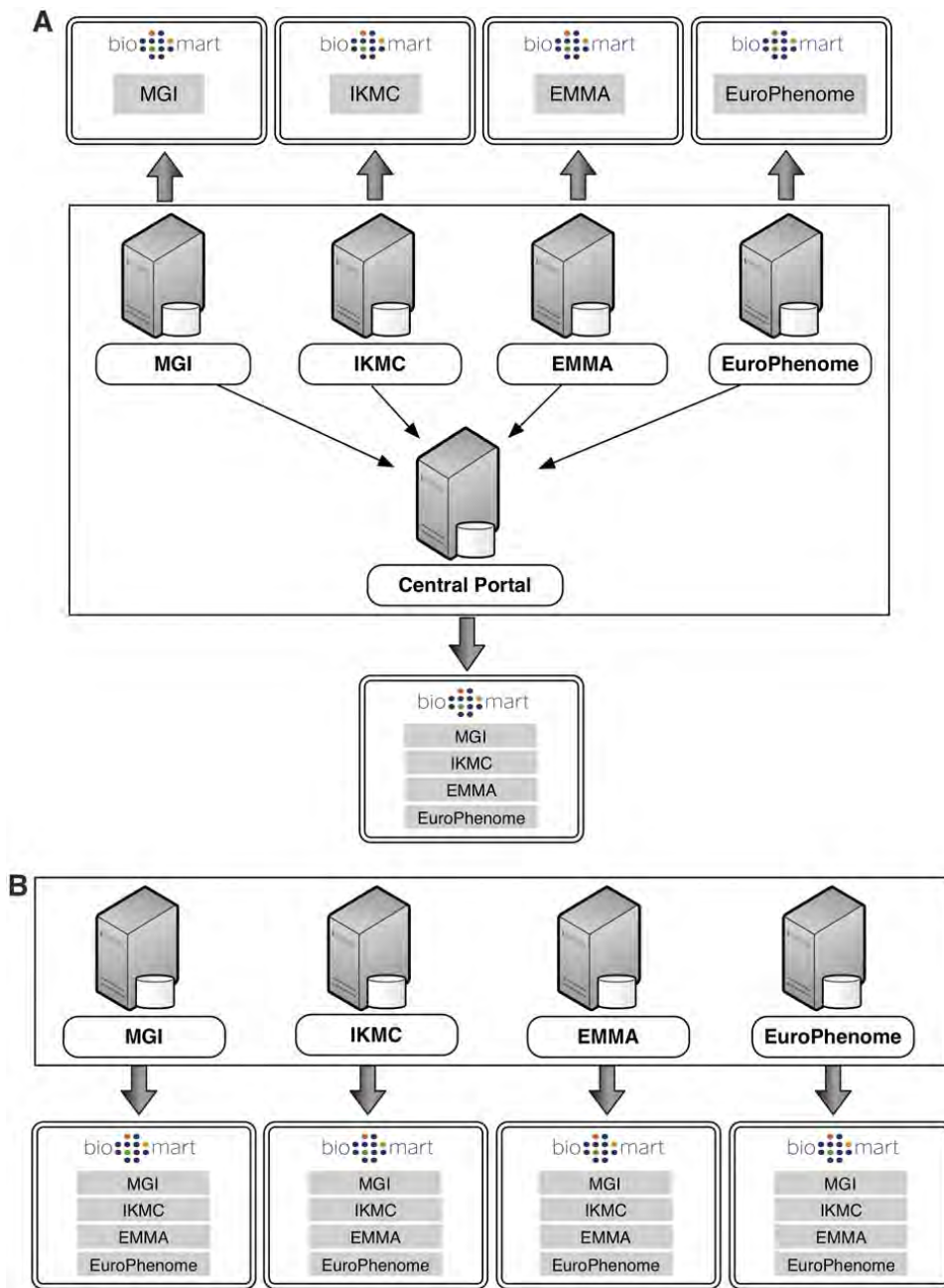
Figure 1.1.3: Biomart Portal Architecture. The portal can be set either with a master/slave or with a peer-to-peer configuration.
