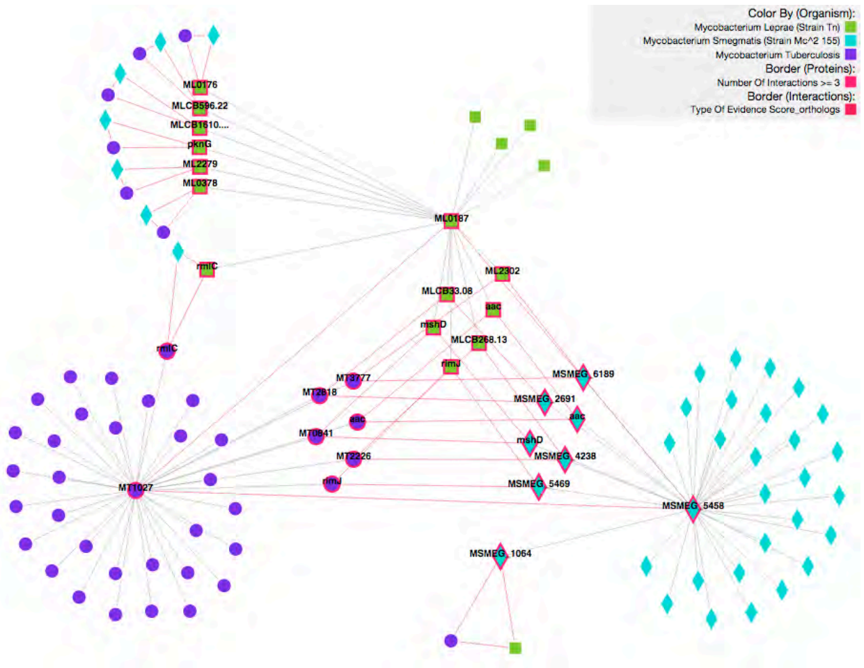
Figure 4.2.1: Three orthologs proteins in MTB, MLP and MSM: Q7D903, Q9CD64, A0R3F9 and their neighbours.
