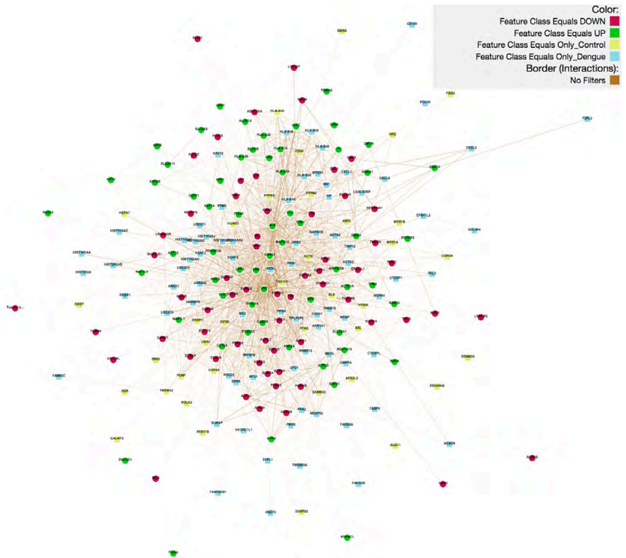
Figure 4.3.1: PPI network of differentially expressed platelets proteins in a dengue study.
