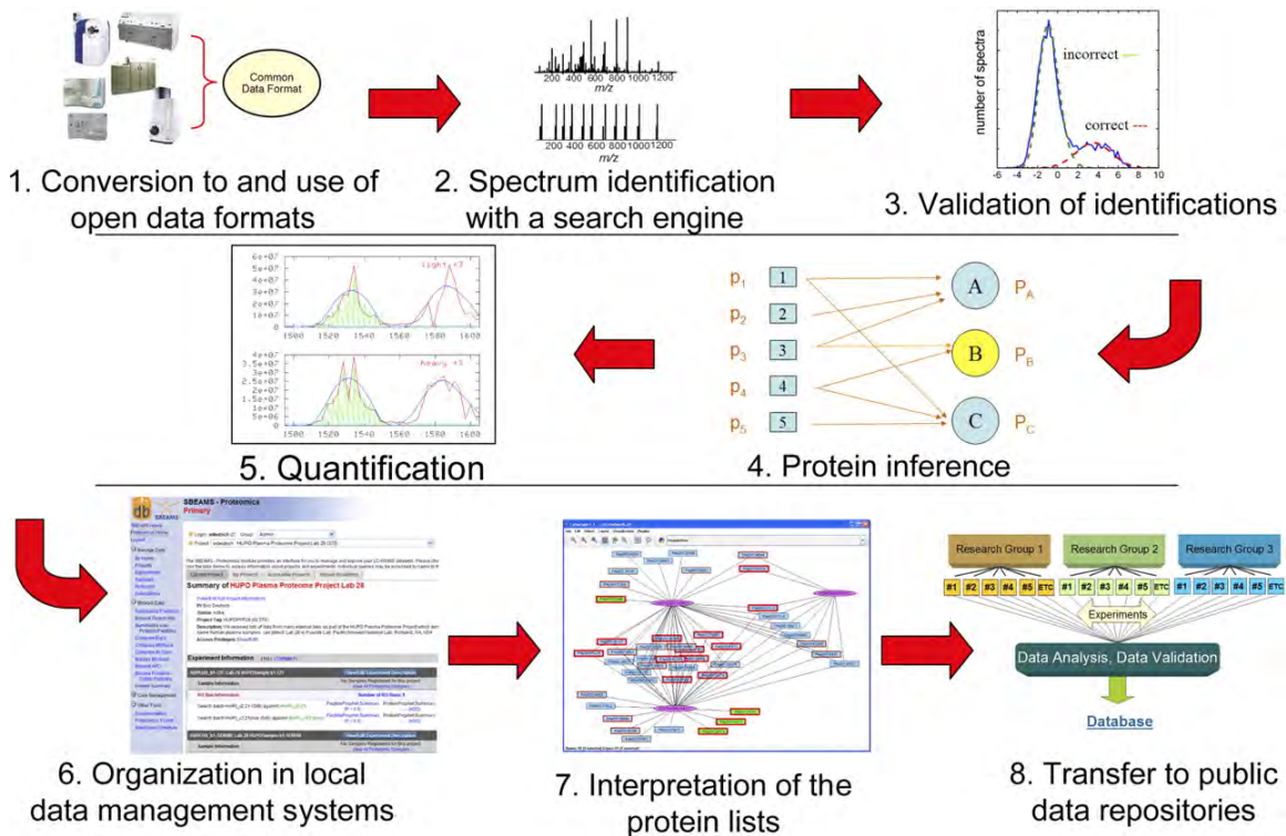
Figure 1.2.8: Tandem mass spectrometry workflow [22].
