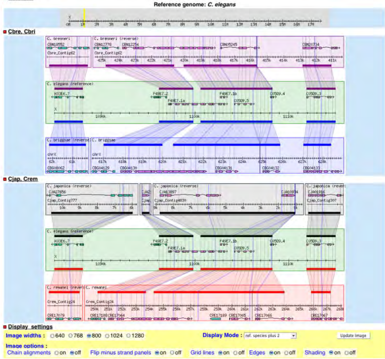
Figure 1.2.5: A five species whole genome DNA sequence alignment comparison from WormBase using GBrowse_syn.
