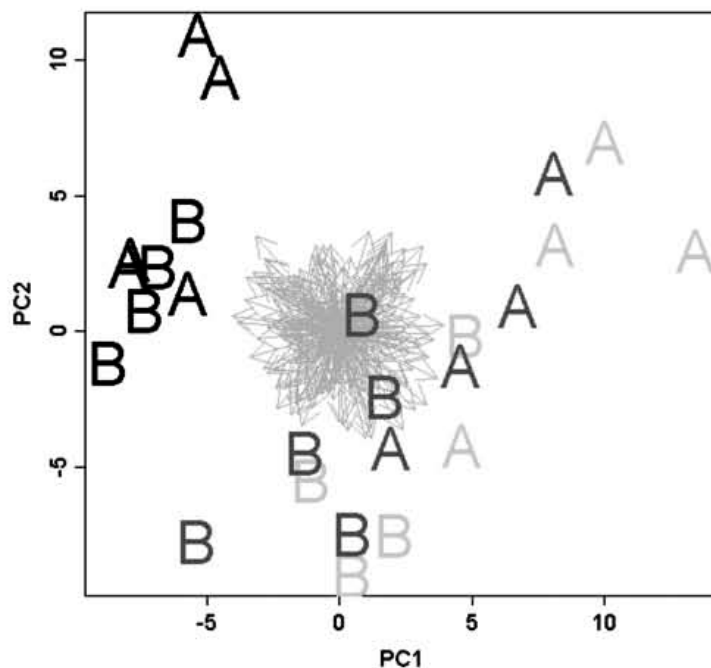
Figure 1.2.7: A biplot displaying PCA results. Figure taken from [98].
