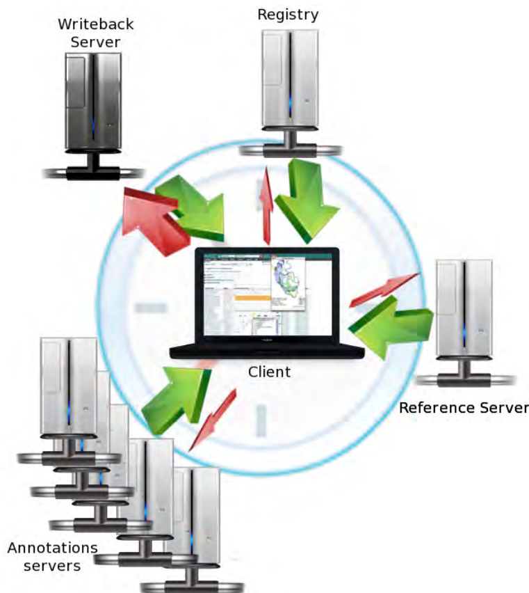
Figure 2.2.1: Writeback in the DAS Architecture: Extension of the DAS architecture for the writeback. A third party writeback server is the last to be queried by the client, and its response is used to update the information provided by the annotation servers. Communication with the writeback server has the peculiarity that the amount of information sent by the client is considerably larger than for any other server. The clock in the background represents the chronological order of the actions in a DAS transaction.
