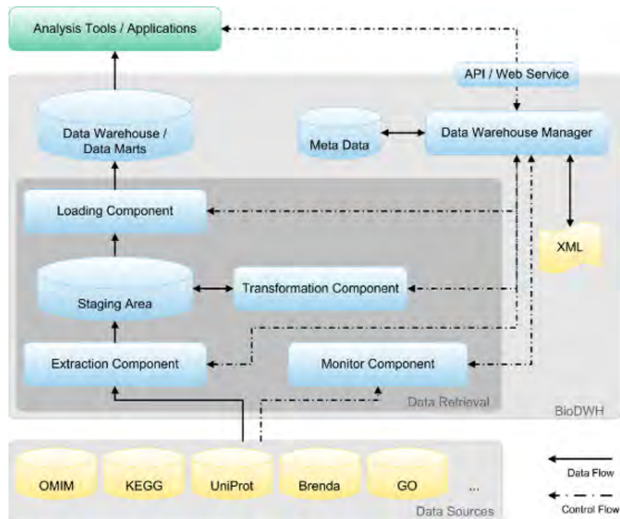
Figure 1.1.2: BioDWH System Architecture.
