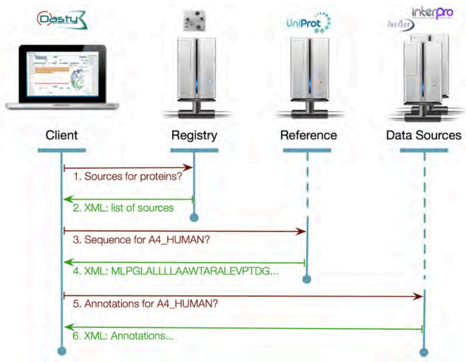
Figure 1.1.6: Flow of information in a standard query in the Distributed Annotating System.
