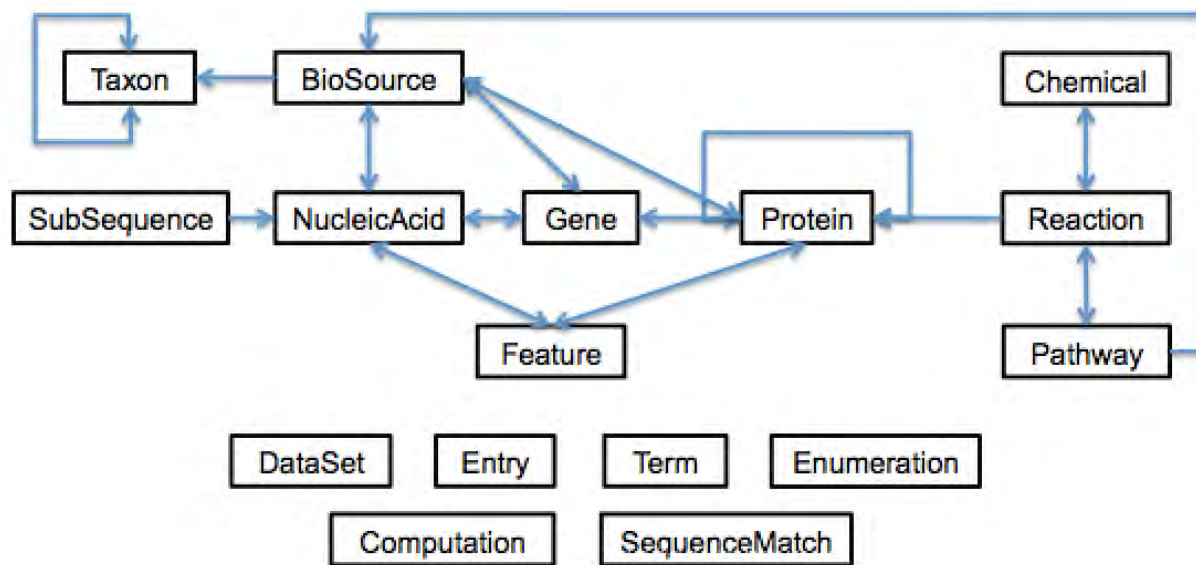
Figure 1.1.1: The main datatypes in the BioWarehouse schema, and the relationships between them.
