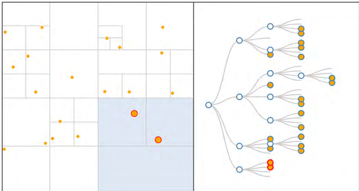
Figure 3.2.7: Quadtree representation of nodes in graphic.
