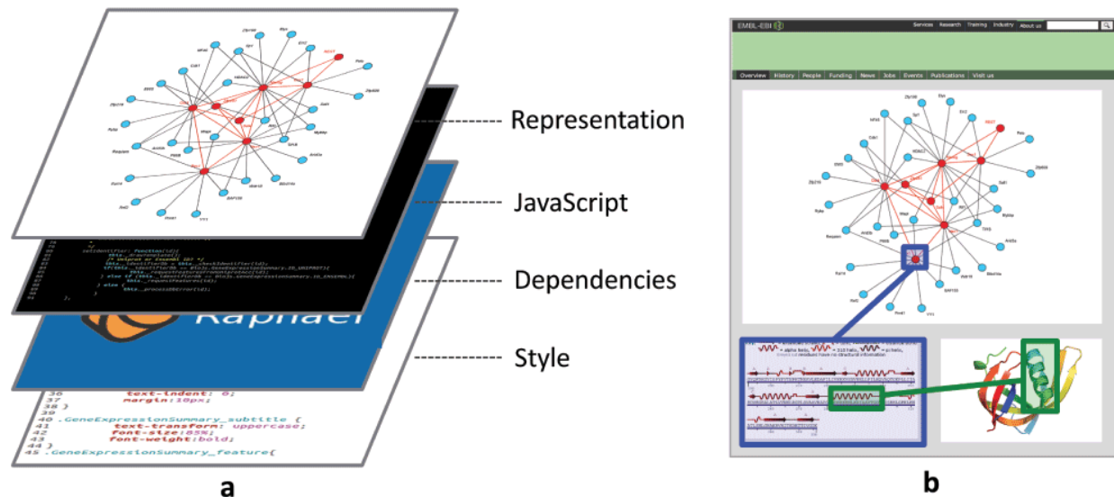
Figure 3.1.1: a. shows the different layers that a BioJS component is divided into. The representation layer sits on top of the JavaScript layer, which similarly possesses a layer of dependencies and a style. b. presents an example of interactivity between three components, a protein-protein interaction network viewer, a secondary structure viewer and a tertiary structure viewer.
