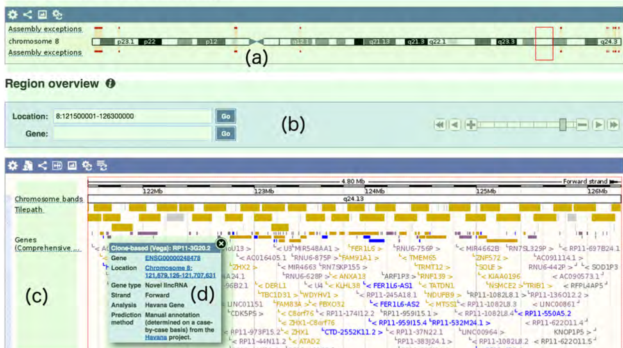
Figure 1.2.3: Snapshot of the Ensembl genome browser highlighting the components that support the implementation of Shneiderman mantra: overview(a), zoom(b), filter(c), details-on-demand(d).
