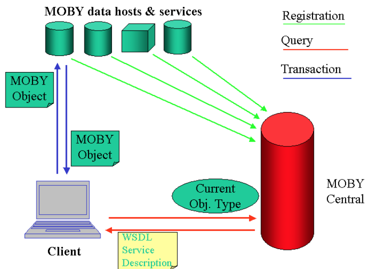
Figure 1.1.5: BioMoby Overview.
