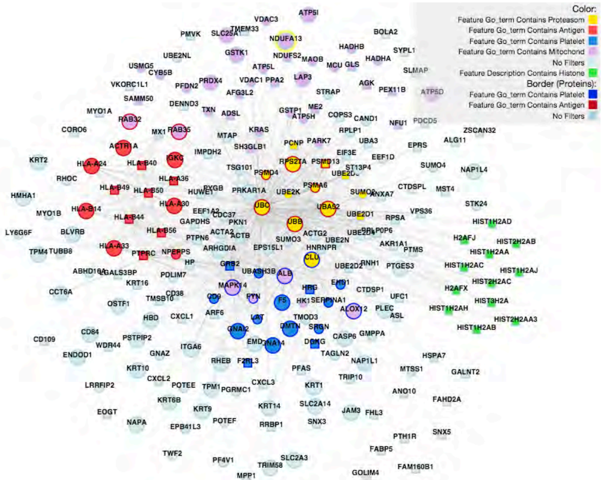
Figure 4.3.2: Subnetwork of the differentially expressed proteins in the Dengue platelets dataset, identifying the most predominant GO terms by colour.
