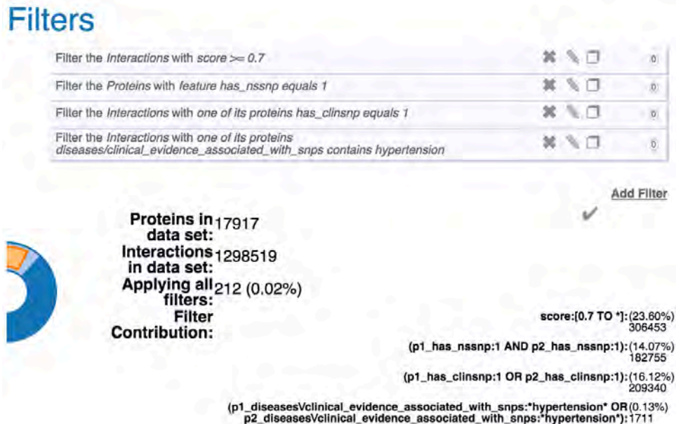
Figure 4.4.2: Selection of filters for image 4.4.1
