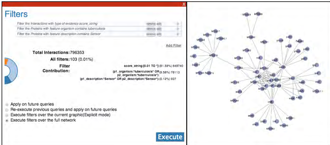
Figure 3.2.2: PINV Filters Dialog. Snapshot of the dialog where the user can explore a dataset by defining filters.
