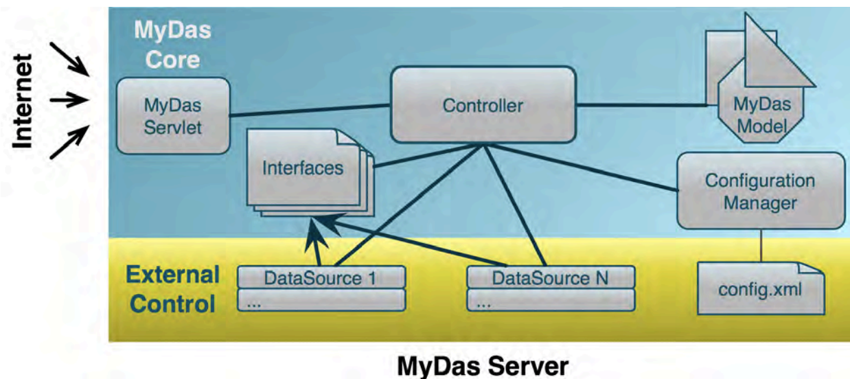
Figure 2.1.1: MyDas Architecture. The requesters can interact with MyDas through the servlet, which communicates the commands to the Controller. The Controller knows which Data Sources have been implemented by querying the Configuration Manager. Data Sources should implement at least one of the provided Interfaces. MyDas internally implements the DAS model.
