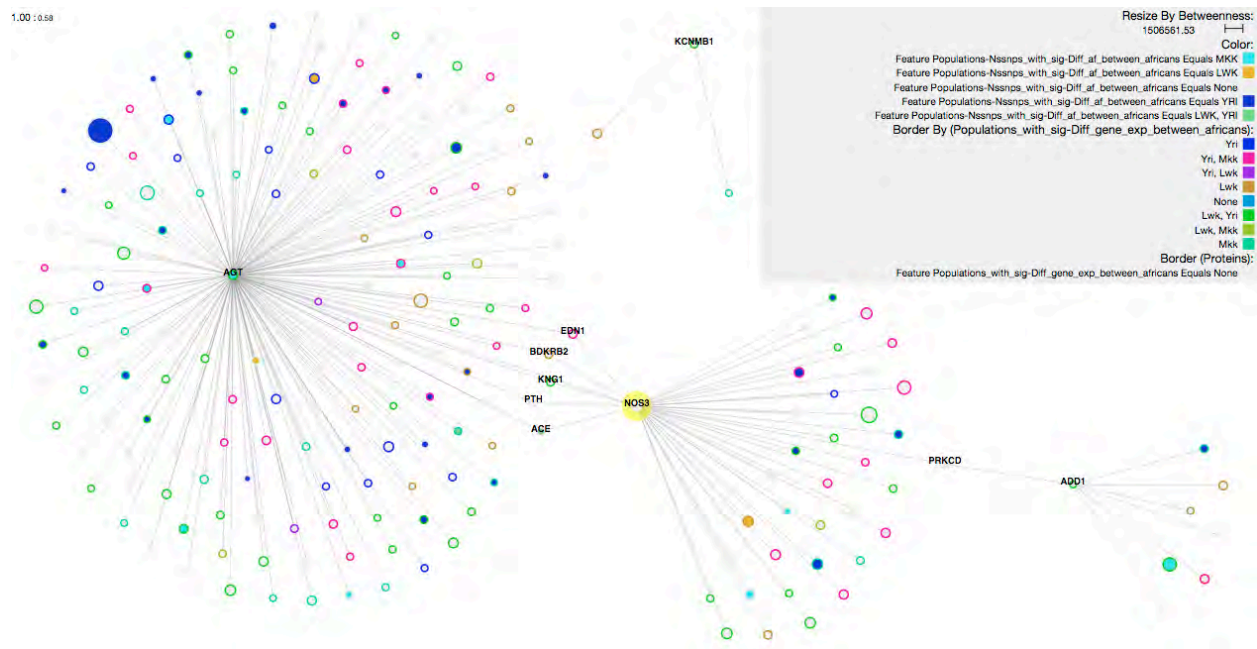
Figure 4.4.1: Interactions between proteins with a hypertension clinSNP and proteins with nsSNPs in the context of AF and gene expression differences between African populations.
