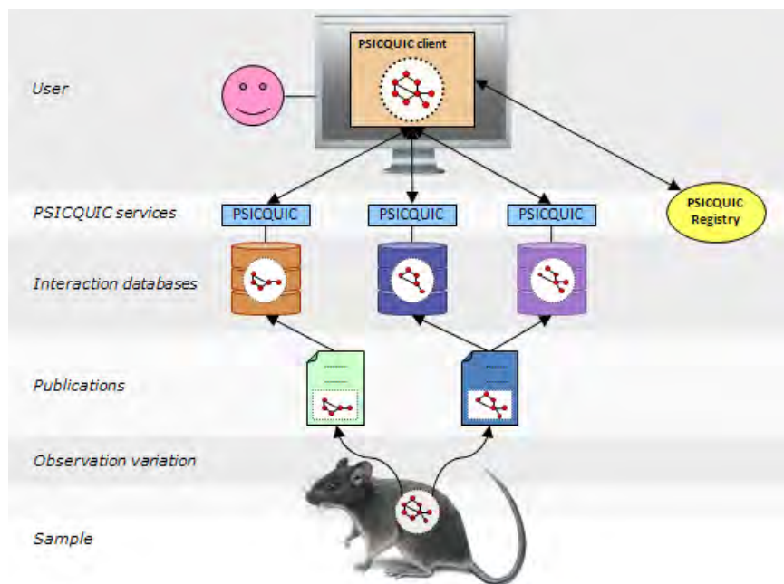
Figure 1.1.4: PSICQUIC Architecture.
