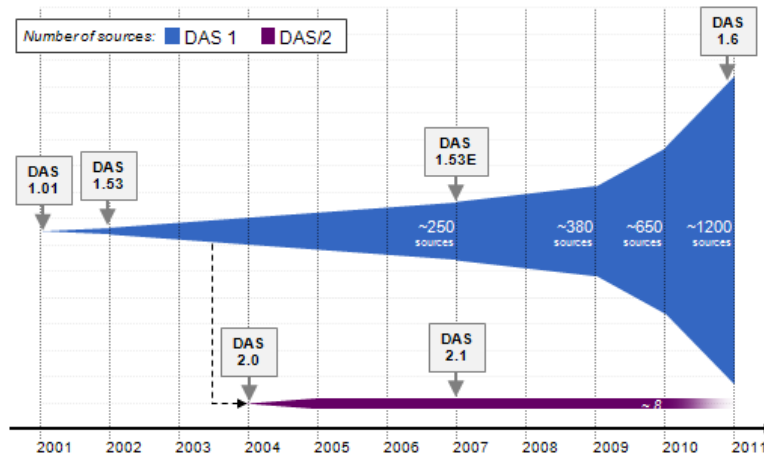
Figure 1.1.7: DAS Evolution.
