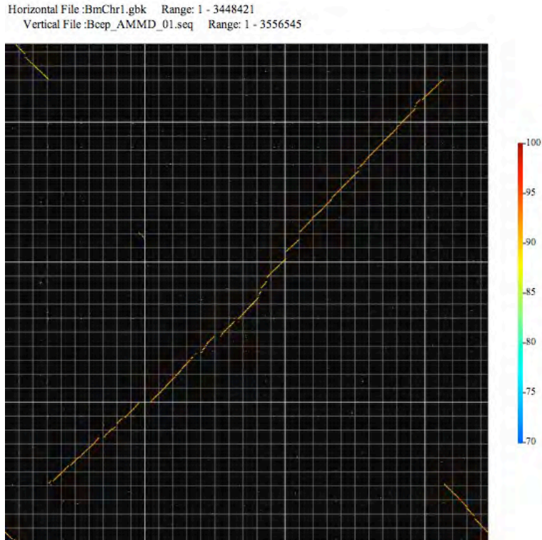
Figure 1.2.4: Dot plot comparison created with GenomeMatcher
