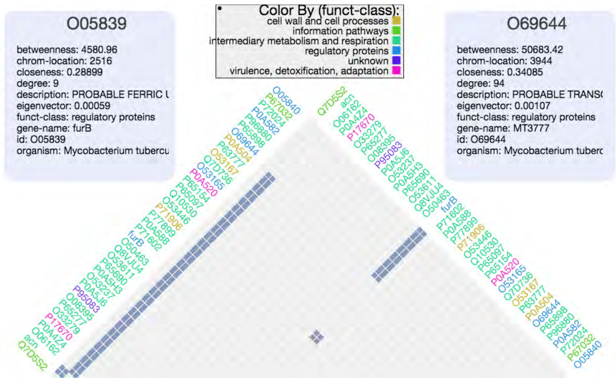
Figure 3.2.4: PINV Heatmap Visualization of the proteins O53166 and O05839 from the MTB dataset.
