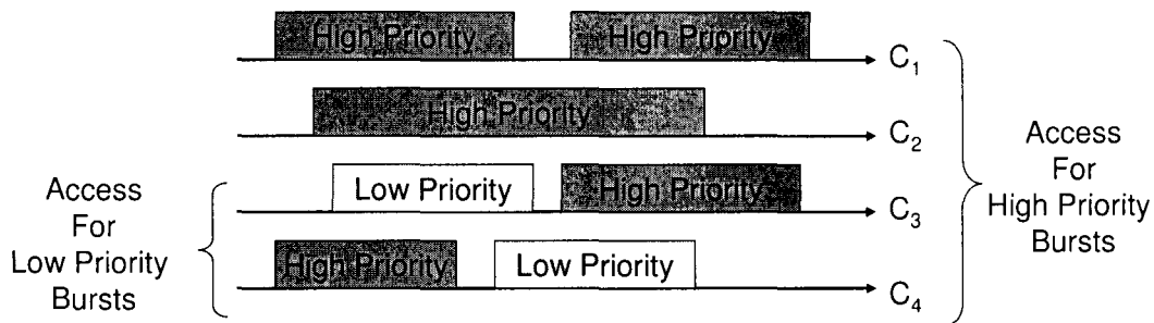
Figure 2.20 Threshold-based Dropping.
