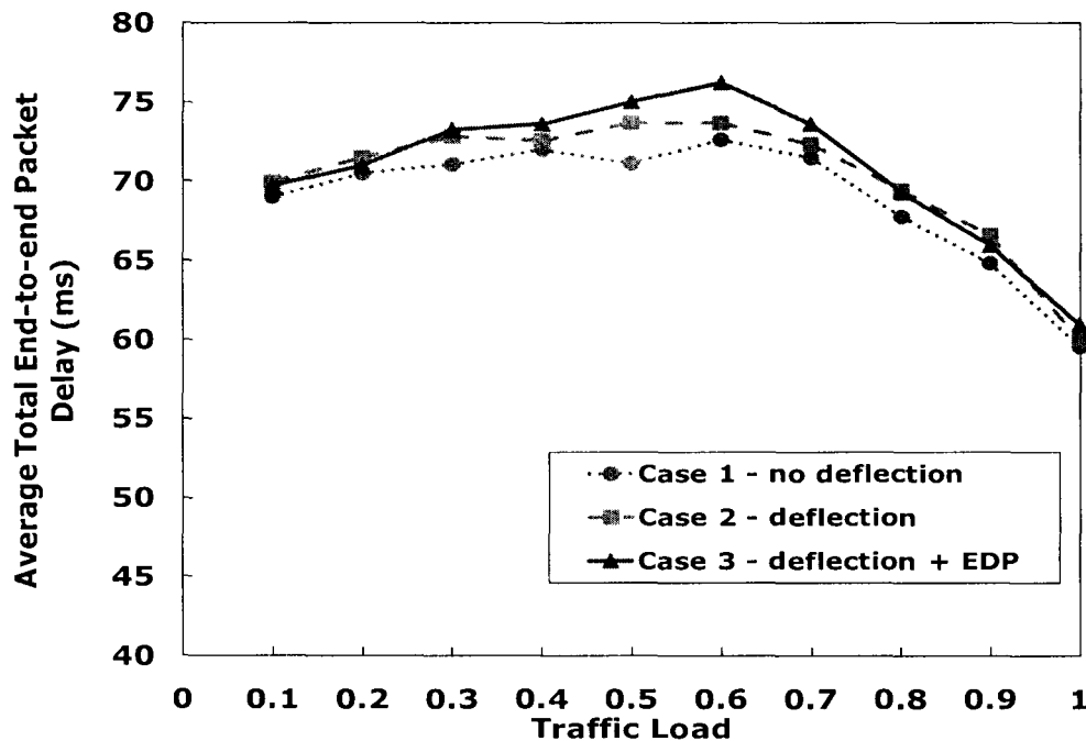
Figure 5.11 Average Total End-to-end Delay versus Traffic Load.
