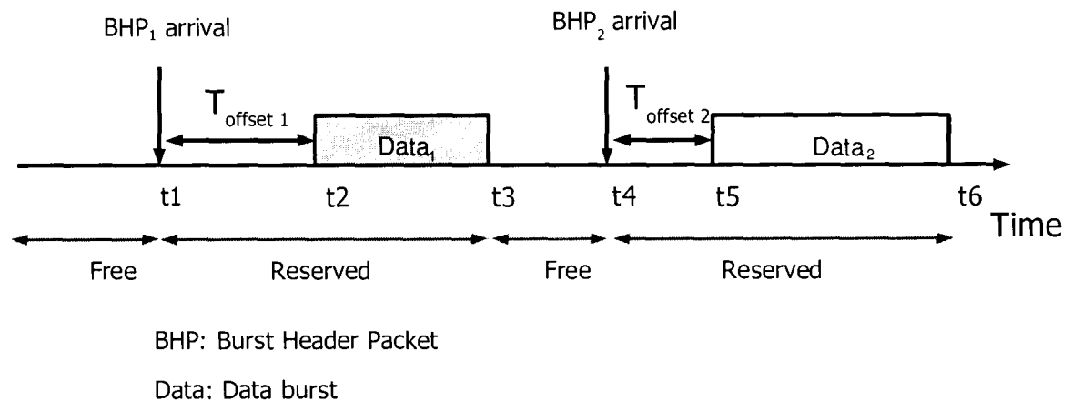
Figure 2.10 An Immediate Reservation Mechanism (JIT).
