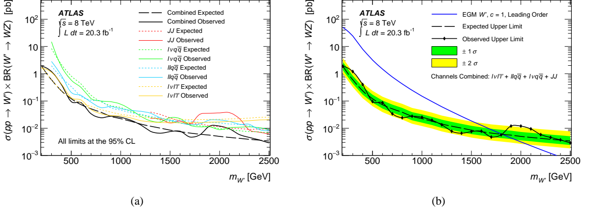
Figure 3: The 95% CL limits on (a) the EGM W' using the \ell\nu\ell'\ell' , \ell\ell q\bar{q} , \ell\nu q\bar{q} , and JJ channels and their combination, and (b) the combined 95% CL limit with the green (yellow) bands representing the 1\sigma ( 2\sigma ) intervals of the expected limit including statistical and systematic uncertainties.
