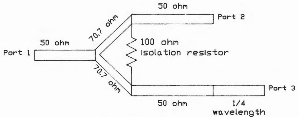
Figure 8.7. Wilkinson coupler with 90^\circ phase lag.
