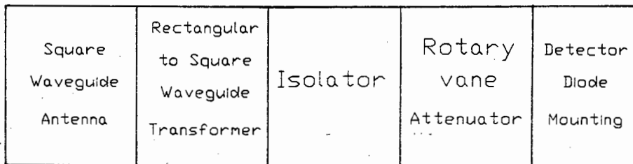
Figure 6.1. Use of Rotary Vane Attenuator
