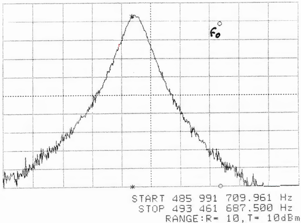
Figure 7.25. Cavity Response for Second Horizontal Orientation.
