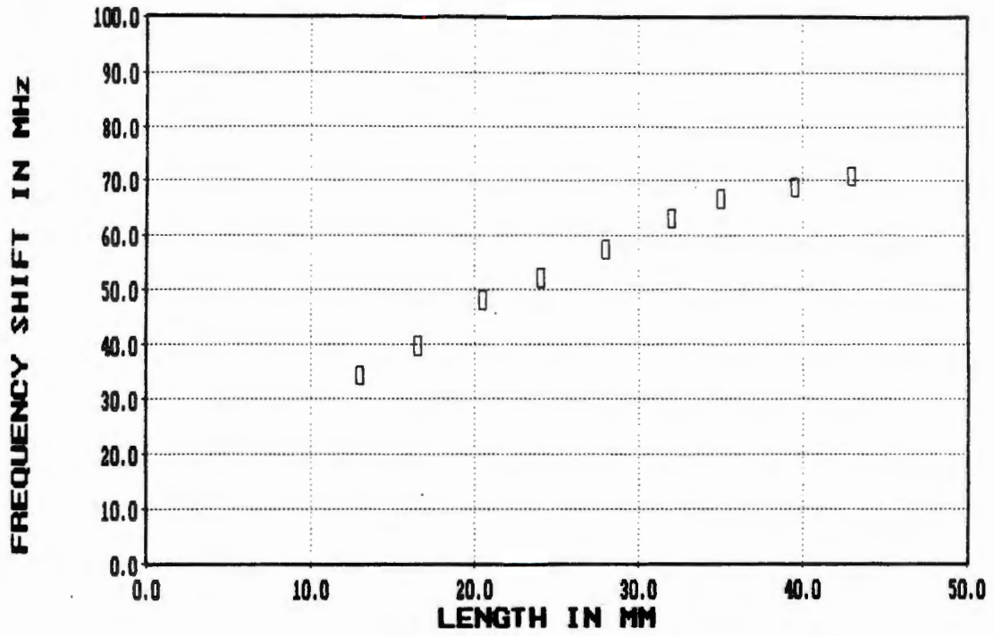
Figure 8.26. Sample length versus frequency shift
