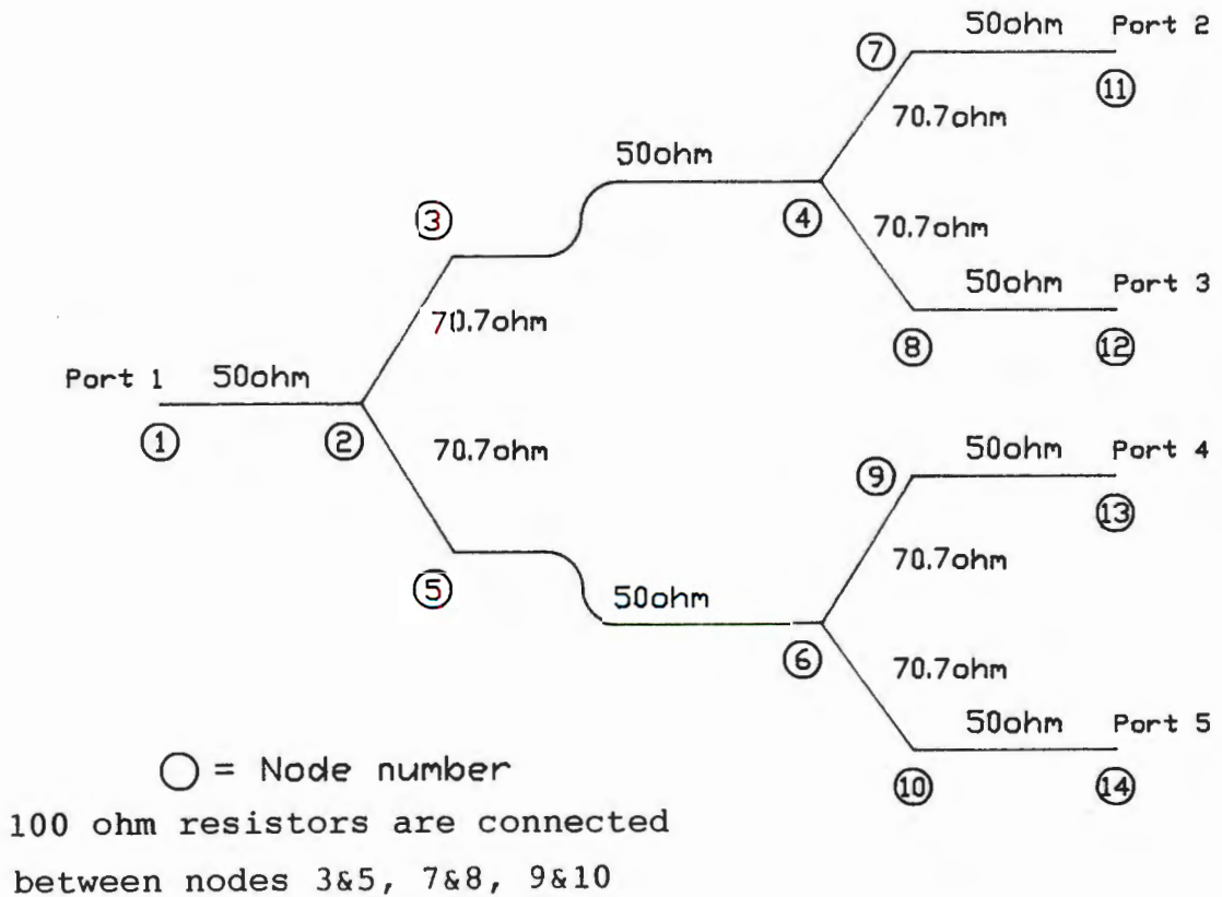
Figure 8.19. Nodal model of four way power splitter
