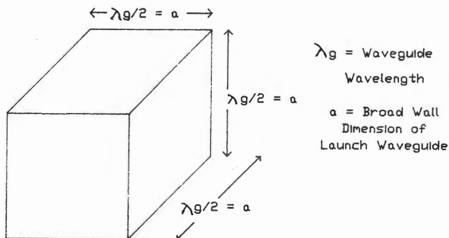
Figure 8.18. Cube dimension
