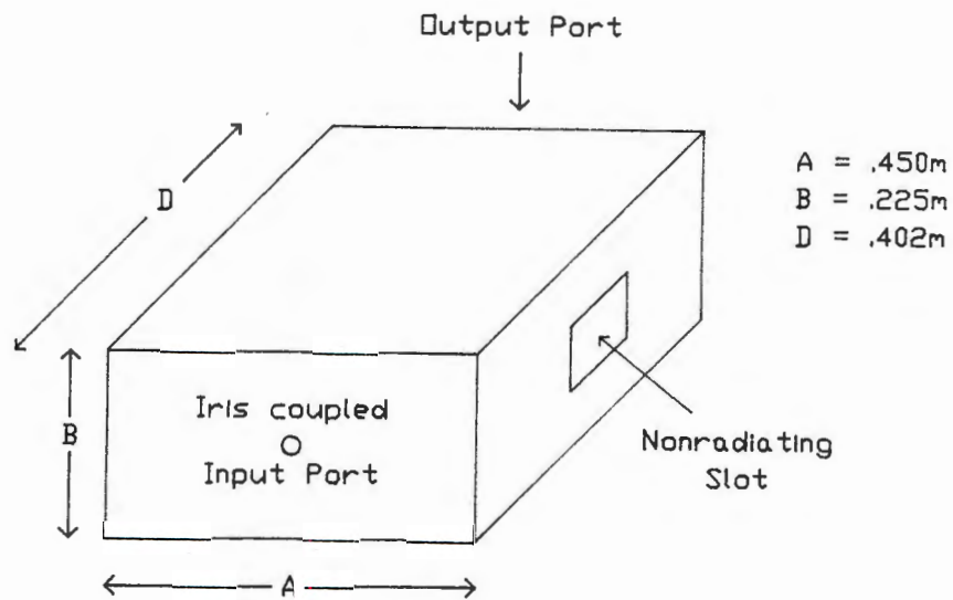
Figure 7.14. Rectangular Resonant Cavity
