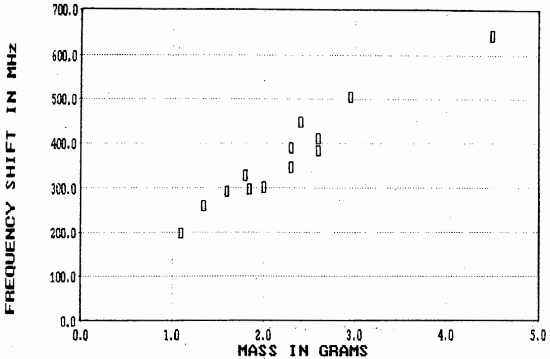
Figure 8.31. Sample mass versus the square root of the sum of the squares of the cavity outputs
