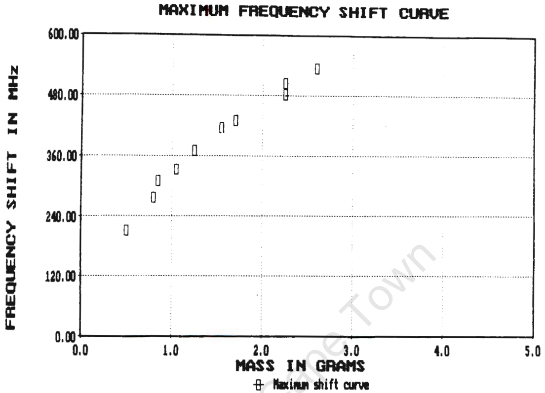
Figure 8.25. Plot of sample mass versus maximum frequency shift
