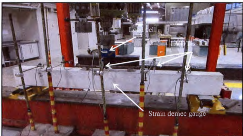
Figure 3.19: Experimental setup for the deflection and load results
