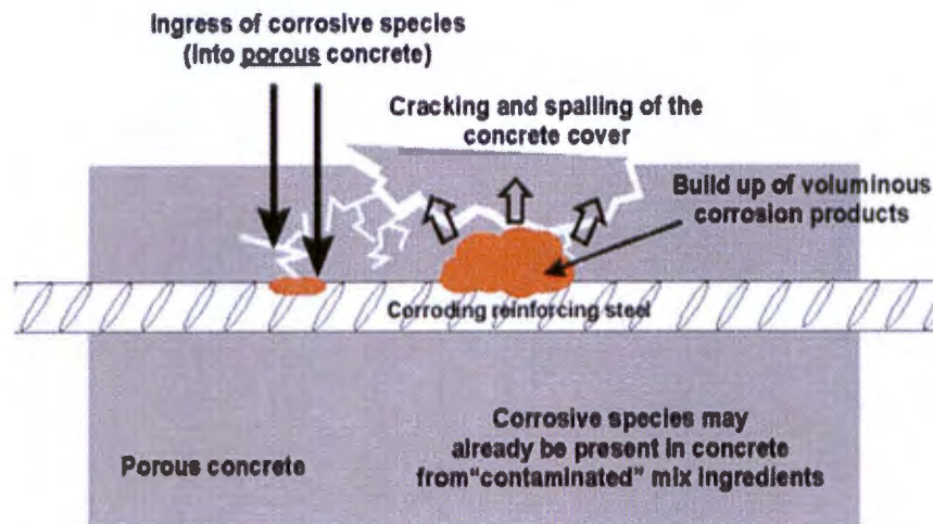
Figure 2.2: Spalling of reinforced concrete
