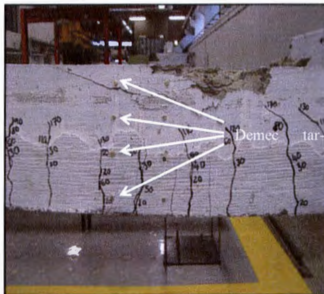
Figure 3.20: Configuration I of the demec strain targets
