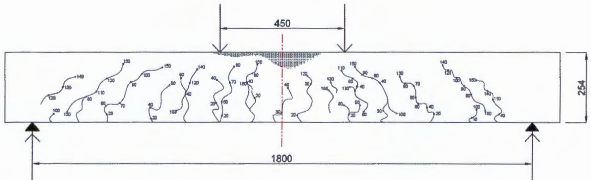
Figure 4.5: Progression of damage observed for beam C3
