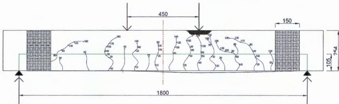
Figure 4.10: Progression of damage observed for beam S2.3
