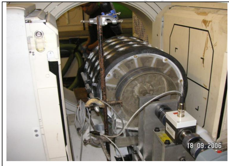
Fig 14: Torque sensor on shaft connecting mill and motor at the UB.
