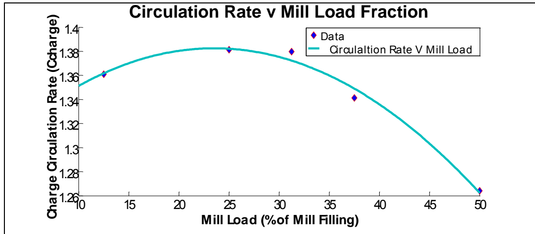
Fig 27: Variation of circulation rate with mill load fraction (volumetric filling).
