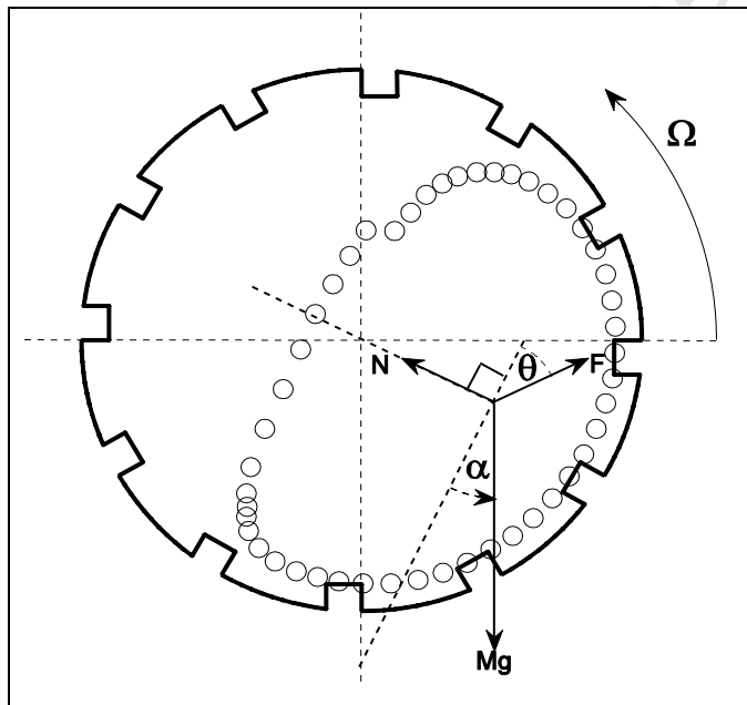
Fig 52: The torque-arm approach [23].
