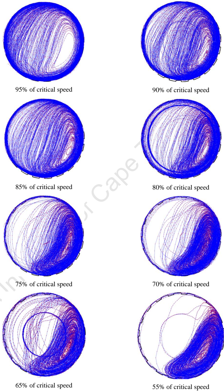
Fig 21: Front view trajectory field of a 1mm particle in a mill charged with a 40% loading and 30% solids. Lifter bars are 5mm high, 20mm wide with a 90° face angle.
