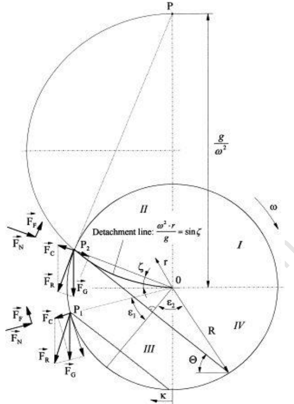
Fig 43: Illustration of the mill geometry at high speeds showing the Davis circle - Mellmann [15].
