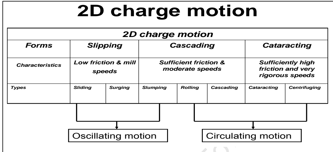
Fig 40: Delineating tumbling charge motion
