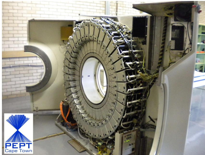
Fig 12: The ECAT ‘EXACT3D’ PET camera at PEPT Cape Town consisting of 48 rings of 576 BGO detector elements.
