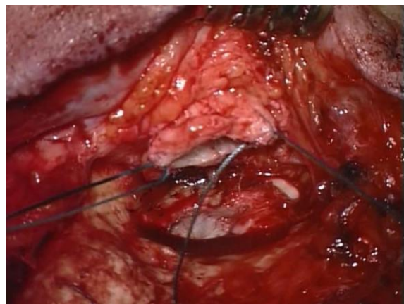
Figure 13: Stay sutures
