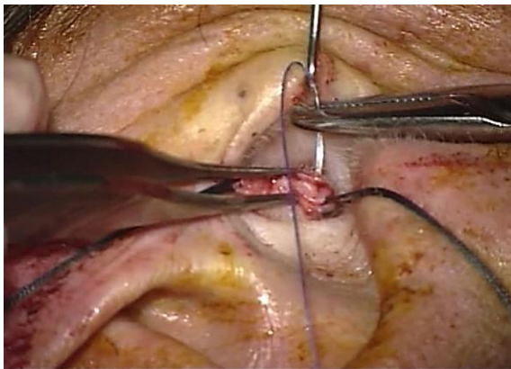
Figure 15: Oversewing canal
