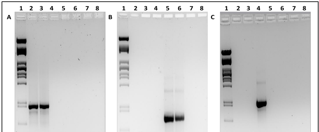
Figure 2.4: Species-specific colony PCR test for A: C. saccharobutylicum , B: C. beijerinckii and C: C. acetobutylicum strains. Lane 1, \lambda -PstI DNA marker; 2, NCP262 T ; 3, NCP108; 4, ATCC 824 T ; 5, NCIMB 8052 T ; 6, NCP260; 7, E. coli JM109 and 8, no template control.
