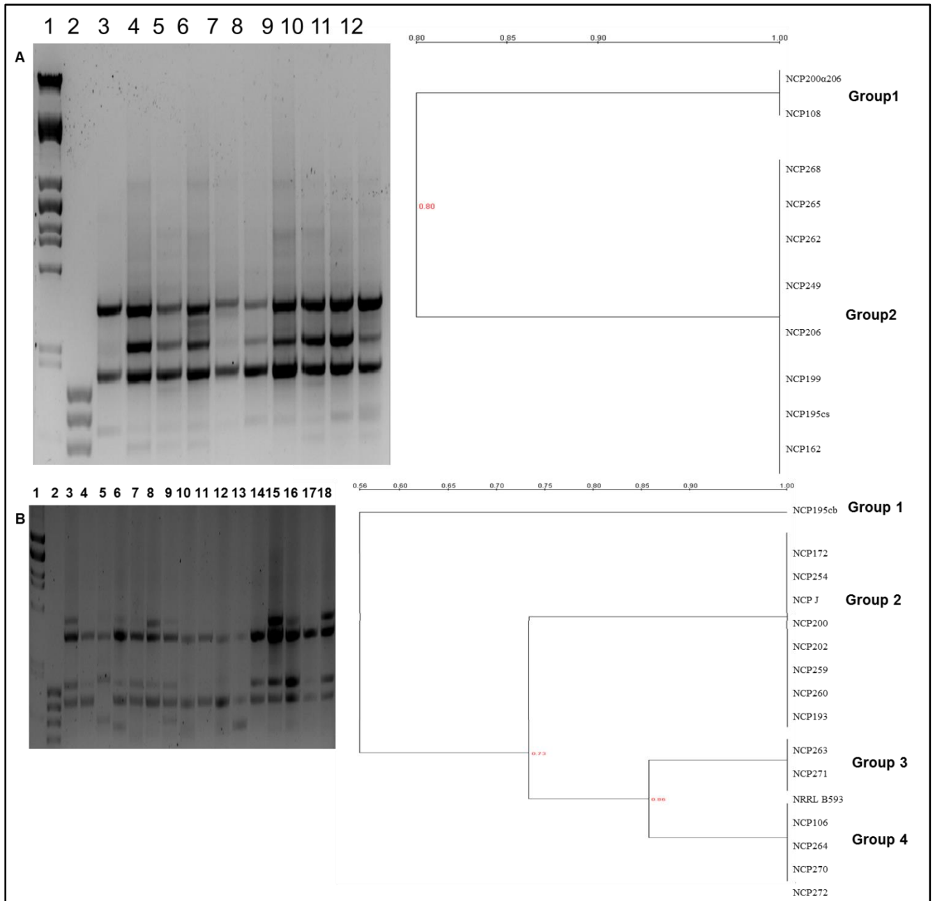
Figure 2.6: RAPD Analysis and clustering of NCP species using UPGMA analysis for A: C. saccharobutylicum : lane 1, \lambda - Pst I marker; 2, 100 bp marker; 3, NCP108; 4, NCP162; 5, NCP195cs; 6, NCP199; 7, NCP200 \alpha 206; 8, NCP206; 9, NCP249; 10, NCP262; 11, NCP265 and 12, NCP268. B: C. beijerinckii strains: lane 1, \lambda - Pst I marker; 2, 100 bp marker; 3, NCP106; 4, NCP172; 5, NCP195cb; 6, NCP254; 7, NCP J; 8, NRRL B593; 9, NCP193; 10, NCP200; 11, NCP202; 12, NCP259; 13, NCP260; 14, NCP263; 15, NCP264; 16, NCP270; 17, NCP271 and 18, NCP272.
