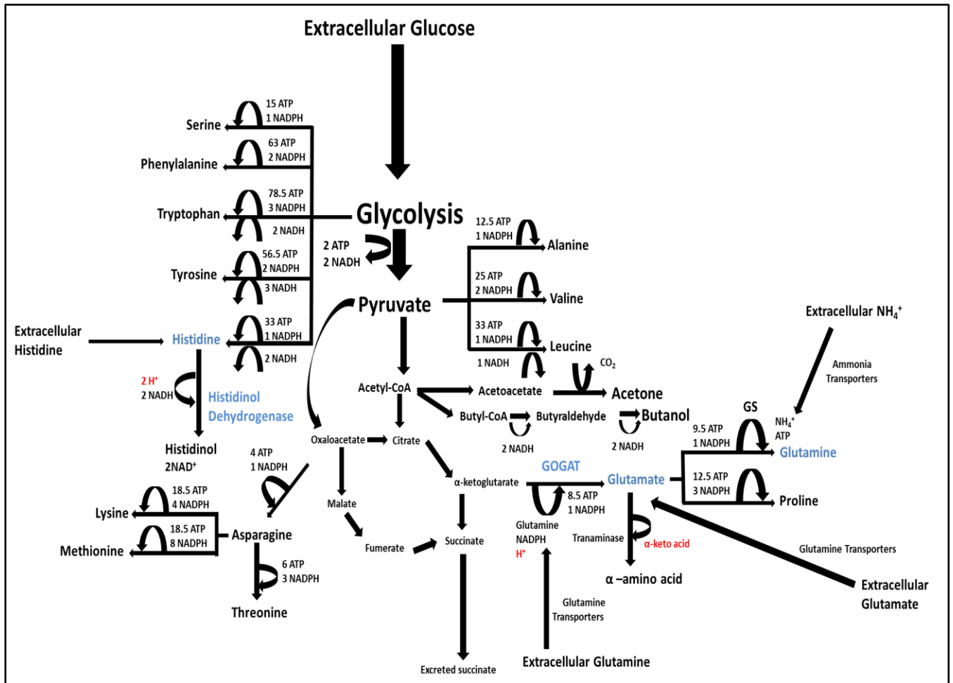
Figure 5.1: A hypothetical model of the amino acid biosynthesis, ATR and solvent production in C. beijerinckii and C. saccharobutylicum . ATP and NADH/NADPH amino acid biosynthesis costs are indicated. Amino acids and enzymes involved in the ATR are indicated in blue and sources of intracellular protons are indicated in red. The amino acid biosynthesis pathways are from Amador-Noguez et al. (2011) and bioenergetics costs of amino acids from Craig and Weber (1998).
