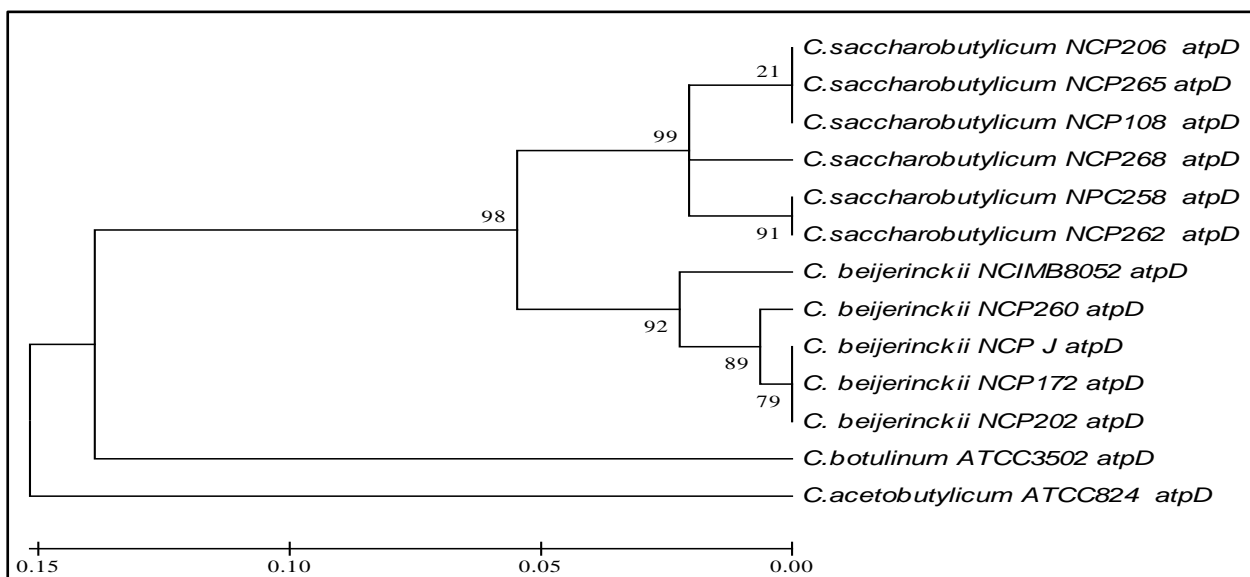
Figure A1: atpD gene phylogenetic tree based on 179 bp of amplified sequence for NCP strains, compared to other members of the genus Clostridium using the Maximum Likelihood method. Bootstrap values calculated from 1000 resampled datasets. One scale bar =0.05 nucleotide substitutions per nucleotide position.
