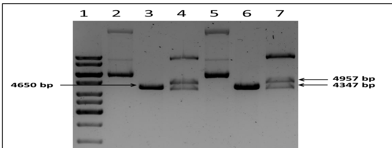
Figure 4.8: Restriction enzyme digests of spectinomycin resistant E. coli pMTL007S-E2_5033PII and pMTL007S-E2_5034Amt plasmids. Lane 1, molecular marker; lane 2, undigested pMTL007S-E2_5033PII; lane 3, pMTL007S-E2_5033PII digested with KpnI ; lane 4, pMTL007S-E2_5033PII digested with SdaI – AscI ; lane 5, undigested pMTL007S-E2_5034Amt; lane 6, pMTL007S-E2_5034Amt digested with KpnI and lane 7, pMTL007S-E2_5034Amt digested with SdaI – AscI .
