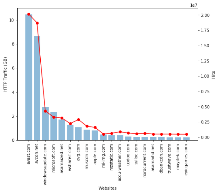
Figure 4.14: School traffic
