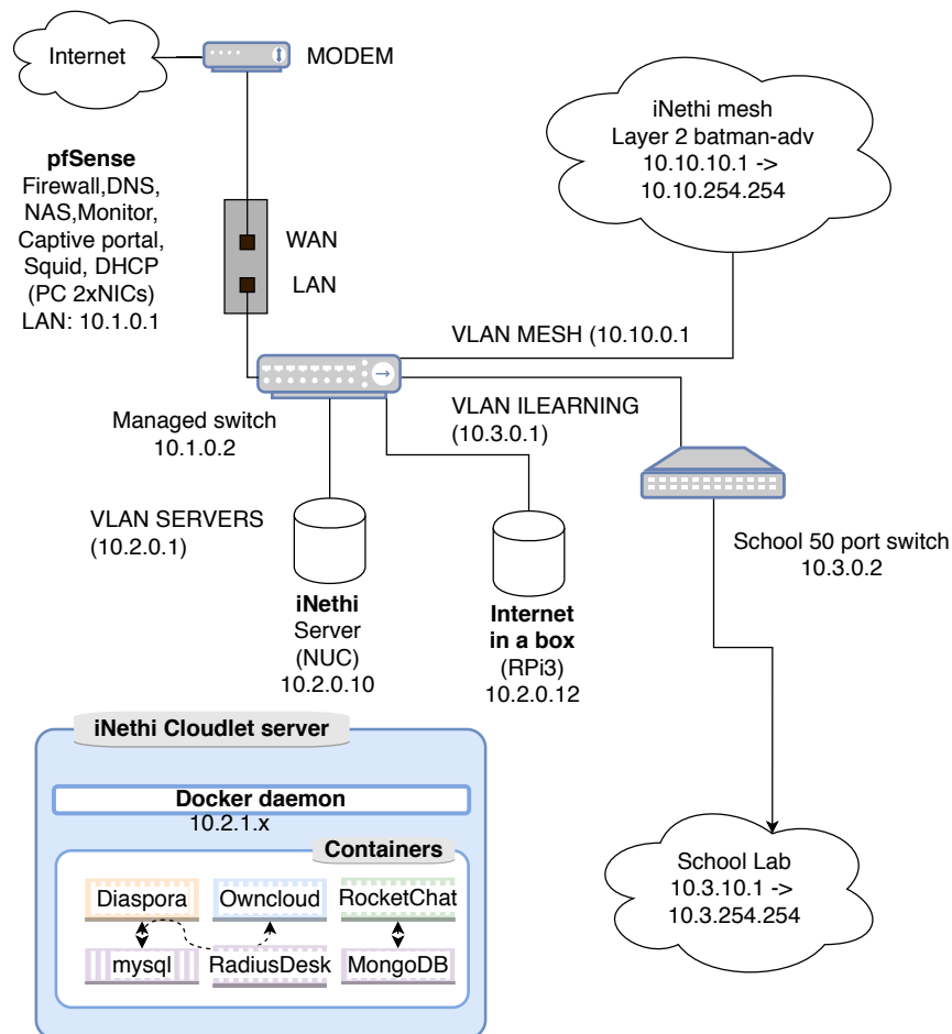
Figure 4.6: iNethi system architecture
