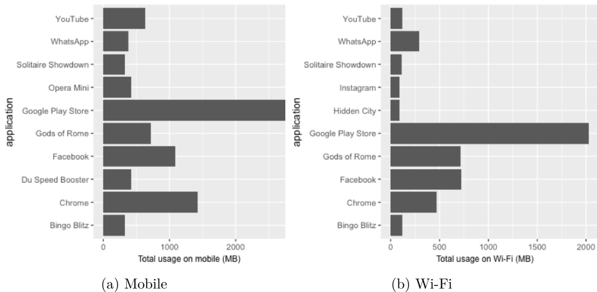
Figure 4.4: Top 10 applications
