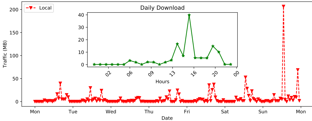
Figure 4.11: Local Services
