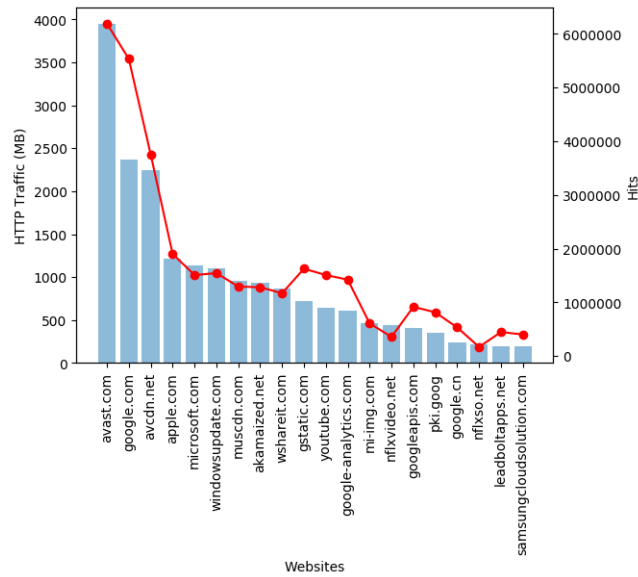
Figure 4.15: Mesh traffic
