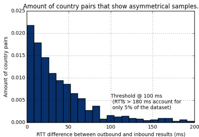
Figure 7.5: Distribution of countries pairs that show asymmetrical samples. The data suggested a threshold at 100 ms, where the symmetrical tendency was broken and marked the beginning of a long random tail
