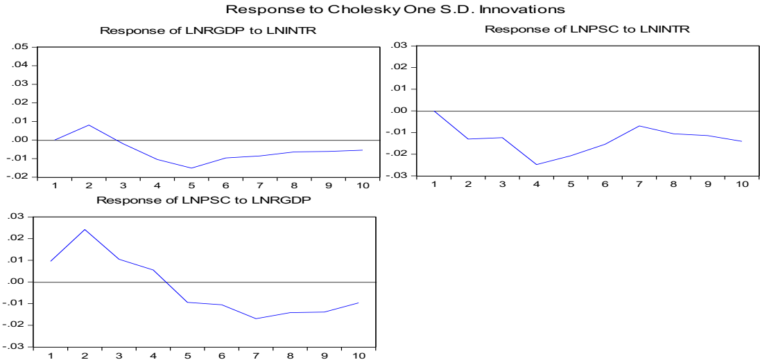
Figure 4.1 Impulse Response Function
