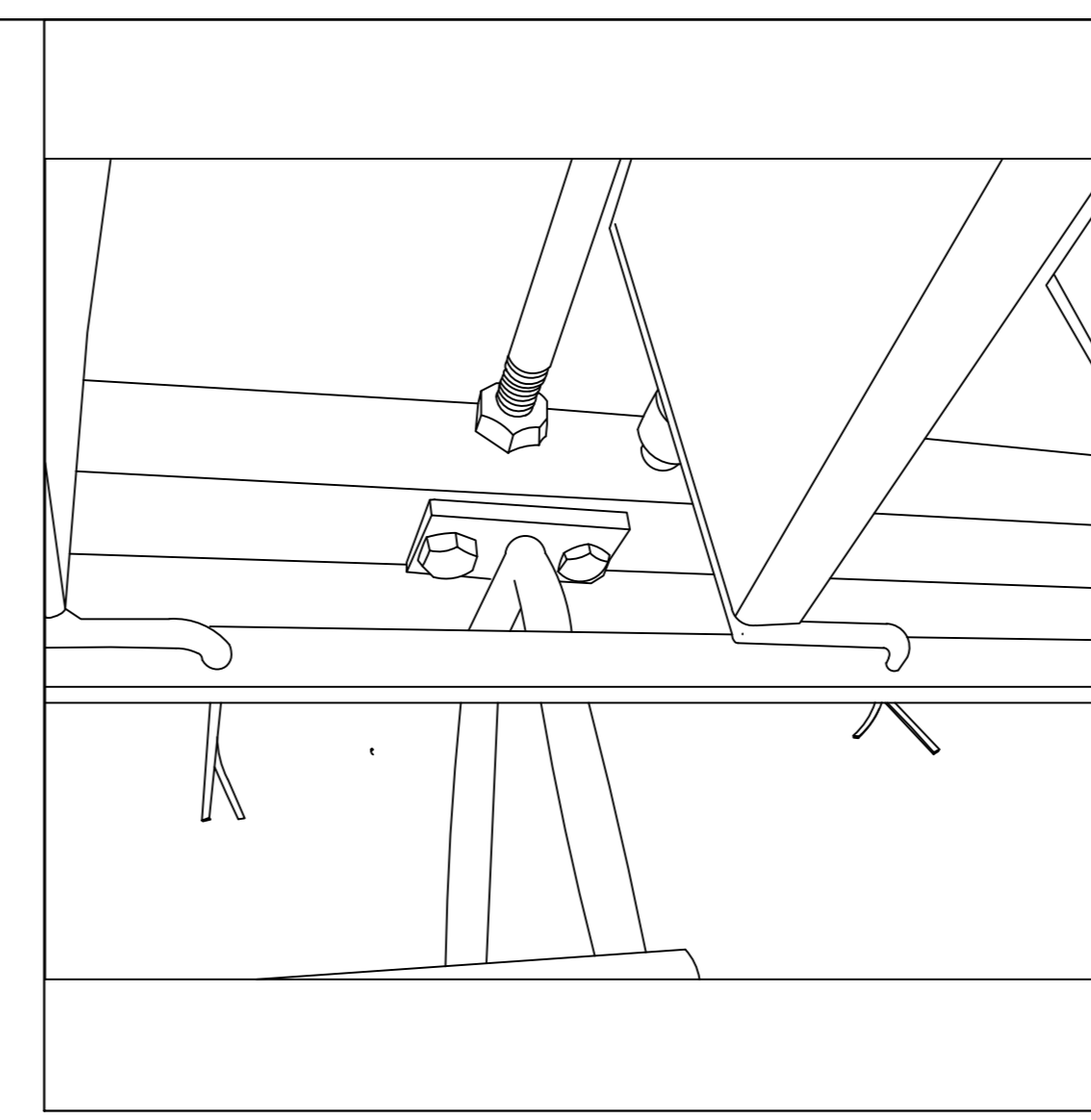
LOUVER DETAIL
