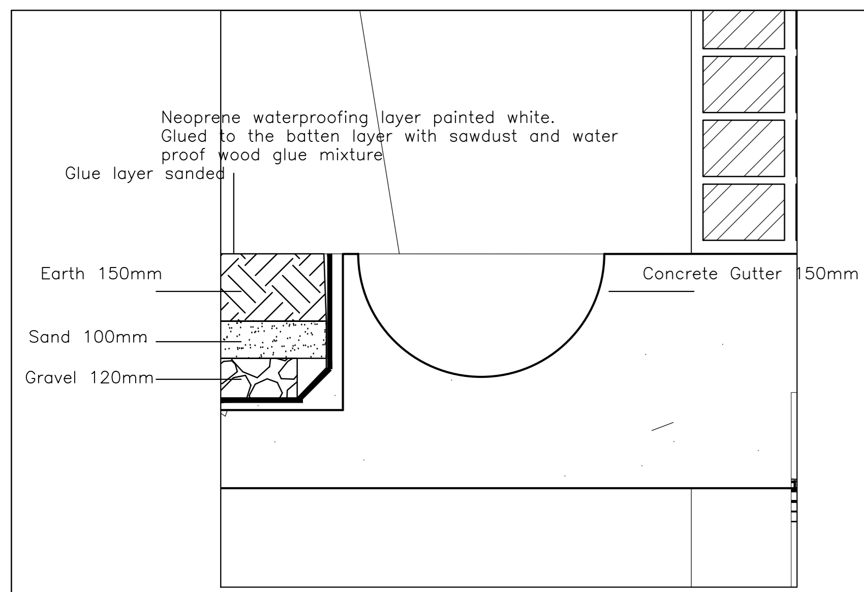
DETAIL A 1:5
