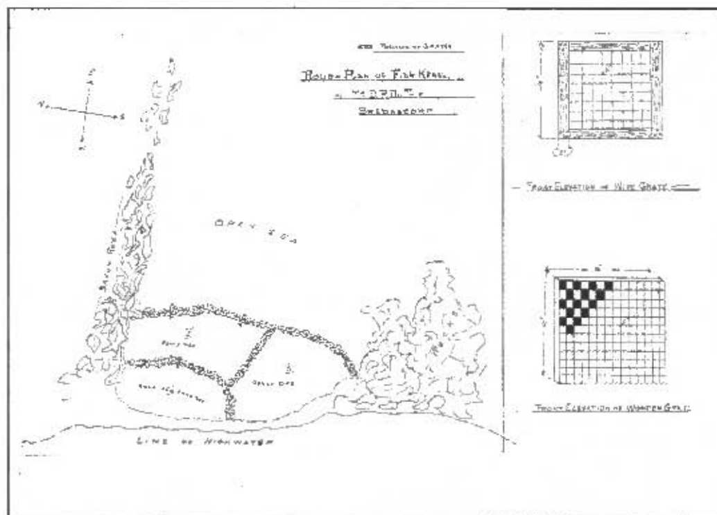
Figure 5.3. Rough plan of fish kraal of Mr. D. P. du Toit at Saxon or Bull Dog Reef. Plan done in May 1913. PAN 55 K23.
