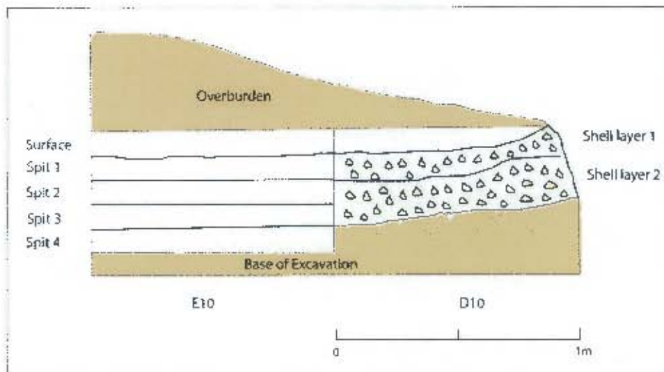
Figure 3.7. Section drawing along 10/9 line.
