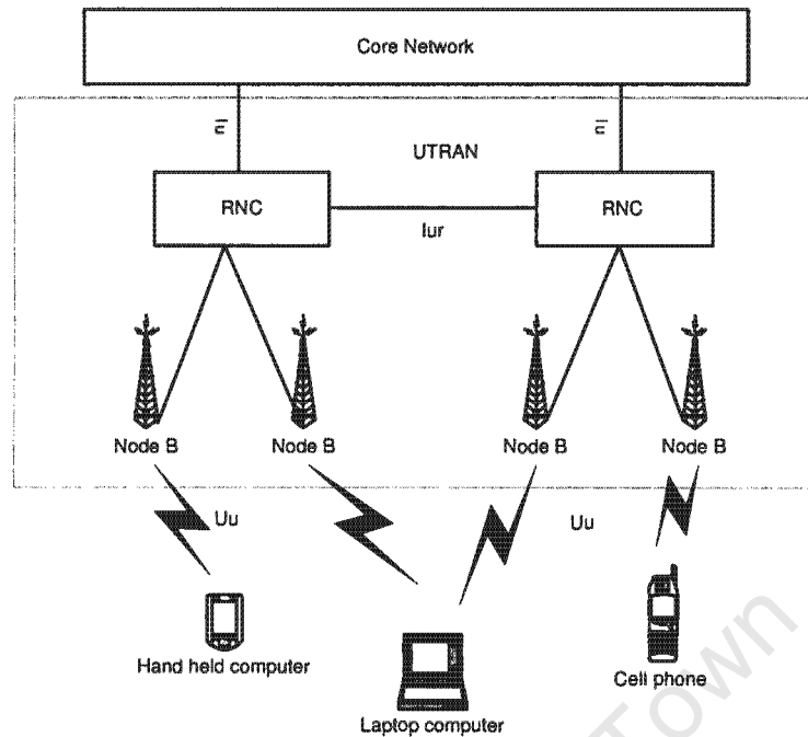
Figure 6: UTRAN Architecture
