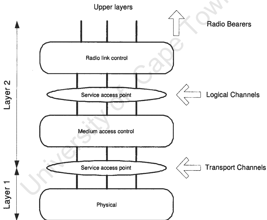
Figure 16: User Equipment User-Plane Protocol Architecture
