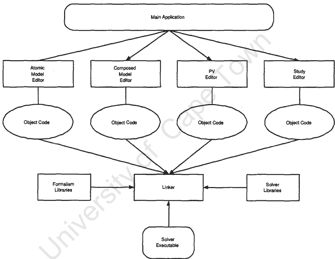
Figure 2: Möbius Tool Architecture
