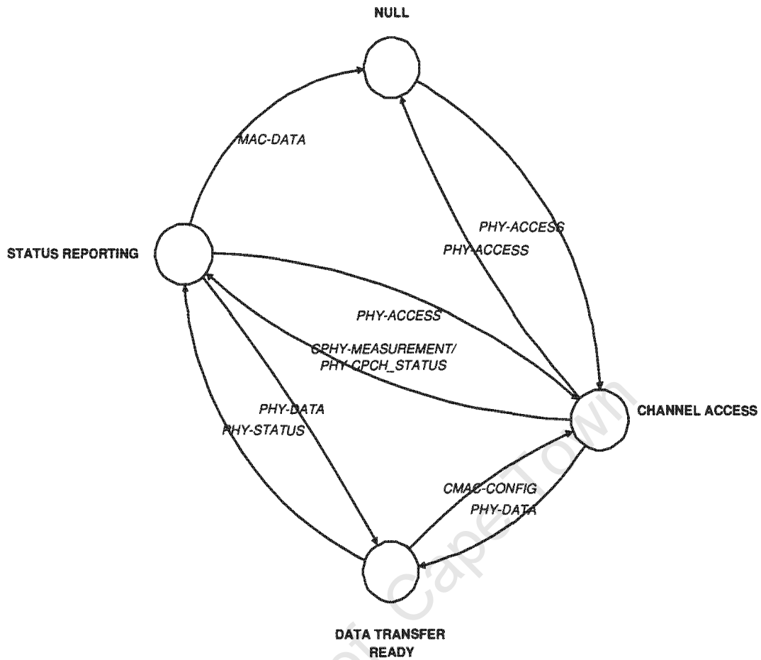
Figure 17: The State Model for the Physical Layer
