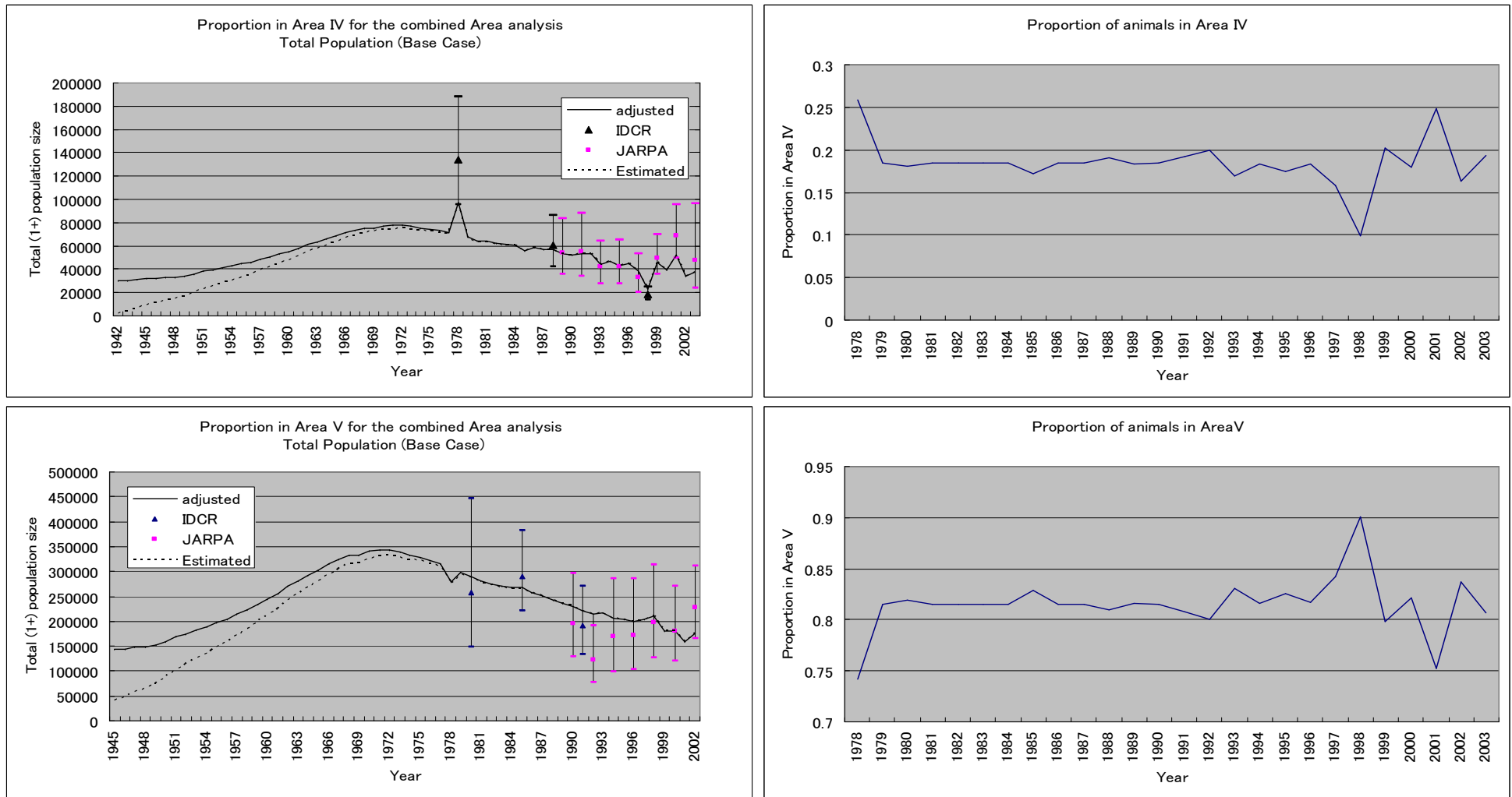
Figure 3a. Fits of the ADAPT-VPA model to the total (1+) abundance estimates for Areas IV and V separately for each Area, together with the estimates for the proportions ( p_y and 1-p_y ) of the total population in each Area each year for the Area IV+V combined Base Case. The abundance plots include the survey estimates of abundance together with their survey sampling estimated 95% confidence intervals. The difference between the “estimated” and “adjusted” total population sizes is explained in the text.
