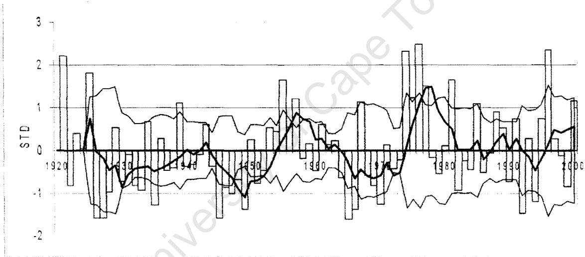
Figure 4 Total annual (January – December) rainfall from 1921 - 2000. Bars: Jan – Dec standardised rainfall. Central curve: 5 – year running mean rainfall. Shading: 5 – year running standard deviation.
