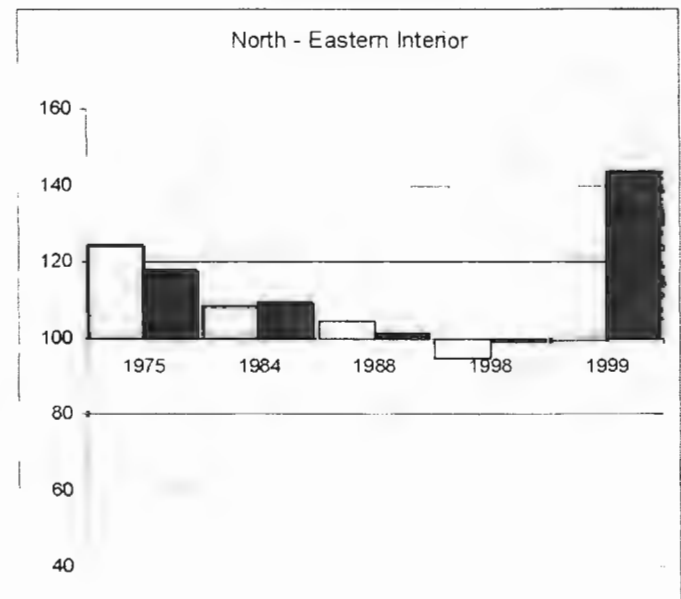
Figure 8 Total annual rainfall in each rainfall area for each La Niña episode expressed as a percentage of the 1921 – 2000 annual average (i.e. 100 corresponds to the average rainfall). Light (dark) shading is for the year of the La Niña (following La Niña).
