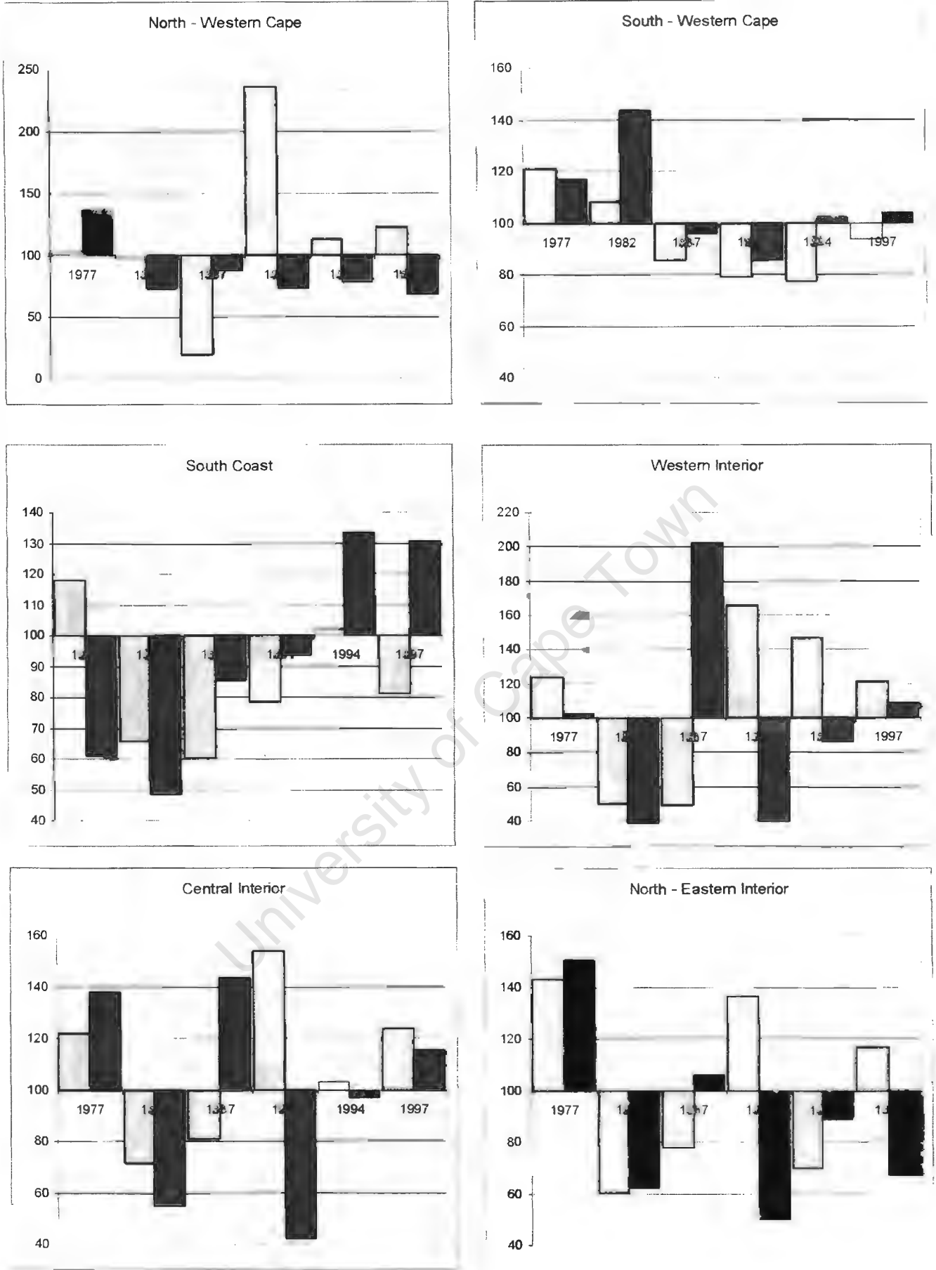
Figure 7 Total late summer (Jan – Mar) rainfall in each rainfall area for each El Niño episode expressed as a percentage of the 1921 – 2000 late summer average (i.e. 100 corresponds to the average rainfall). Light (dark) shading is for the year of the El Niño (following El Niño).
