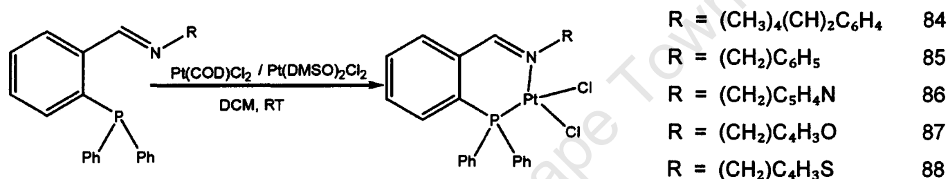
Figure 2.2: The synthesis of novel platinum dichloride complexes 118
