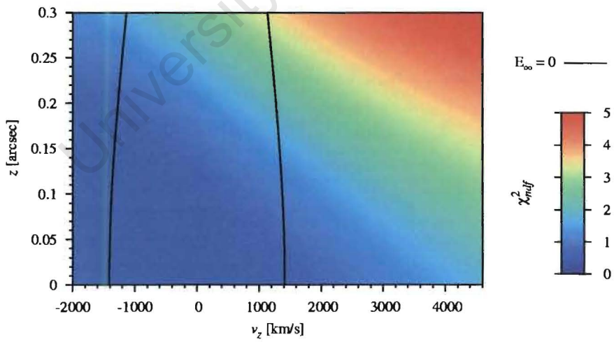
Figure 17: \chi^2_{ndf} phase space plot for S0-2 with fermion ball. Epoch 1992.7.
