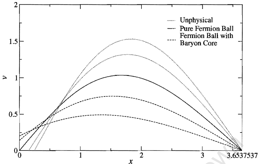
Figure 6: Solutions of the Lane-Emden equation
