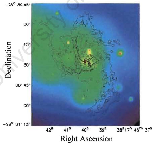
Figure 4: 0.5→7keV image of the central region of the Milky Way. The image has been adaptively smoothed and flat-fielded. Overlaid on the image are \lambda=6\text{cm} contours from Figure 2. X-ray emission from the vicinity of Sgr A* appears as a red dot at 17^{\text{h}}45^{\text{m}}40.0^{\text{s}} , -29^{\circ}00'28'' (J2000.0) [8].
