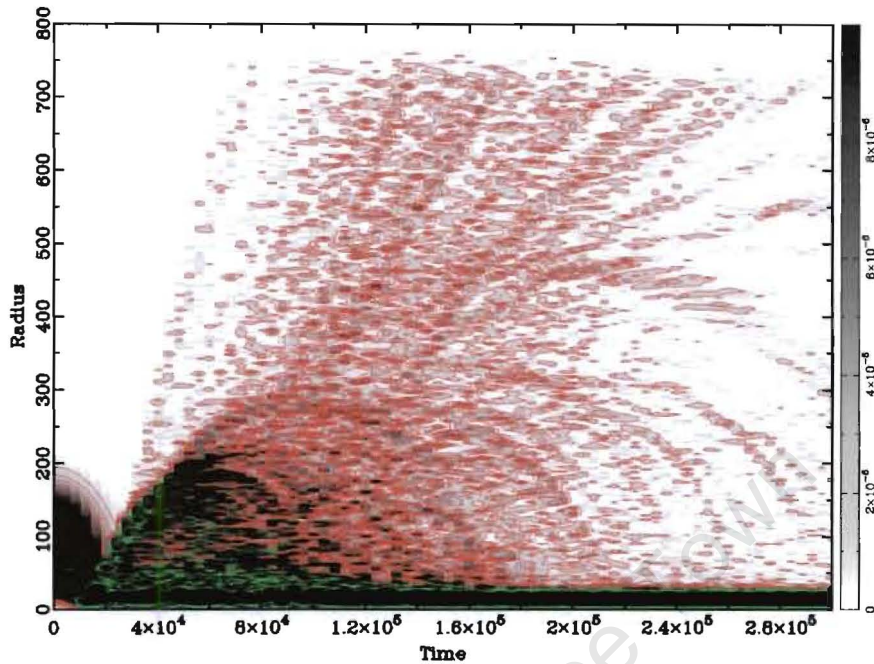
Figure 12: Combined contour-density plot for the evolution of |r\Psi|^2 . Green contour lines denote levels from 10^{-5} to 10^{-4} while red lines denote levels below 10^{-5} . Gravitational collapse is followed by an ejection of excess matter leaving a fermion ball at the centre [35].
