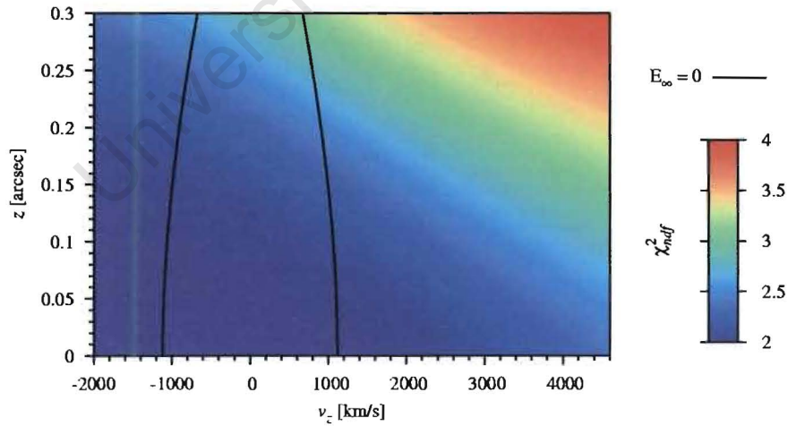
Figure 15: \chi_{ndf}^2 phase space plot for S0-1 with fermion ball. Epoch 1992.7.
