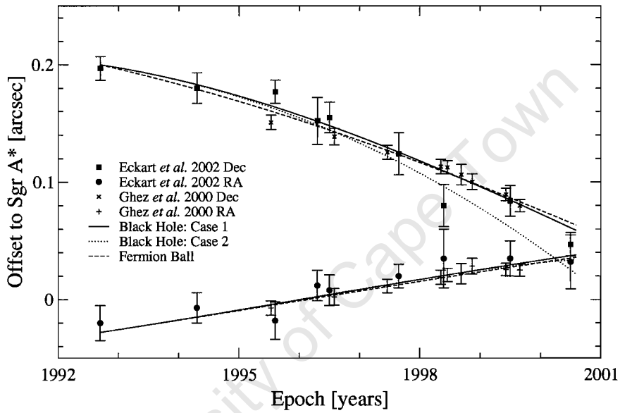
Figure 22: Best fits for S0-2. “Black Hole: Case 1” has z=0.099 arcsec, v_z=1090 km/s with a bound orbit and \chi_{ndf}^2 = 0.68 . “Black Hole: Case 2” has z=0.099 arcsec, v_z=500 km/s with a bound orbit and \chi_{ndf}^2 = 3.27 . “Fermion Ball” has z=0 arcsec, v_z=40 km/s with a bound orbit and \chi_{ndf}^2 = 0.65 . “Black Hole: Case 2” has been chosen in order to describe a very tight orbit around Sgr A*.
