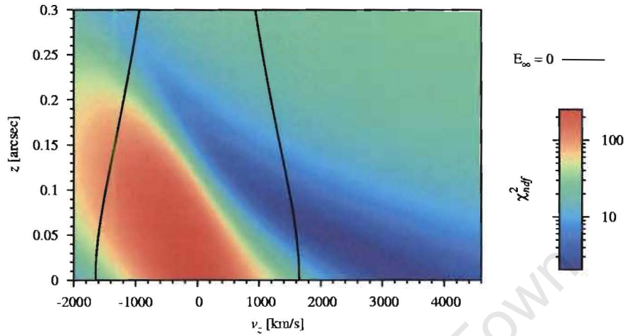
Figure 14: \chi_{ndf}^2 phase space plot for S0-1 with black hole. The lines represent the escape velocity required of the v_z component only, bound orbits being within the lines and unbound orbits outside. Epoch 1992.7.
