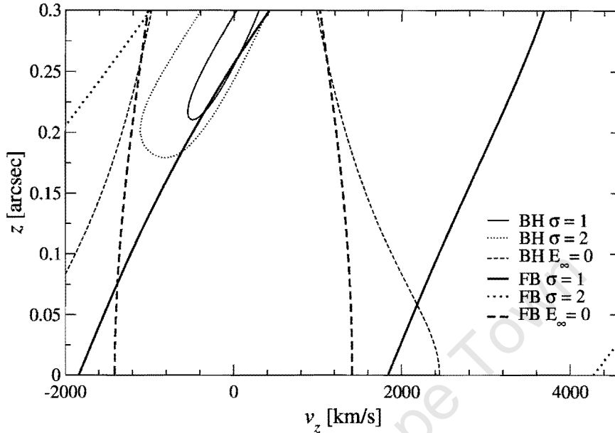
Figure 27: \chi_{ndf}^2 phase space plot for S0-2 at epoch 2005. The minimal \chi^2 paths in Figure 22 have been used to give the ‘initial’ position and velocity parameters for this plot, values are in Table 5. Contour lines for \chi_{ndf}^2=1 and 2 are shown for both black hole and fermion ball scenarios, alongside the corresponding escape velocities. In this case, an accurate measurement of z or v_z may only allow for elimination of the black hole scenario, as the fermion ball minimal \chi_{ndf}^2 region is quite large.
