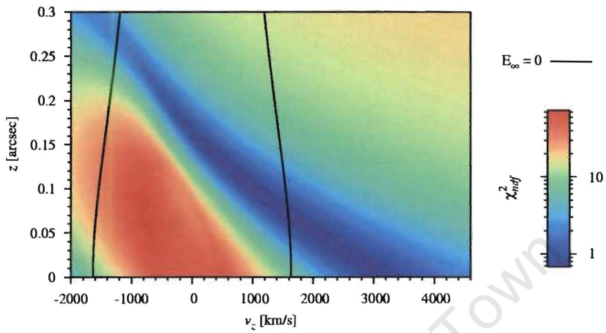
Figure 16: \chi^2_{ndf} phase space plot for S0-2 with black hole. Epoch 1992.7.
