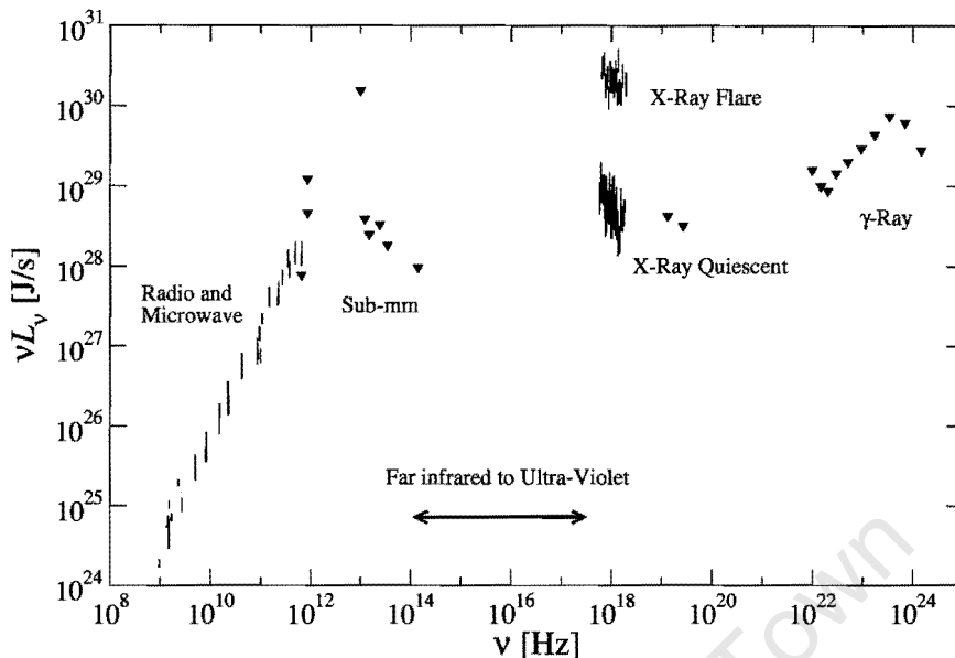
Figure 5: Compilation of spectral data in the direction of Sgr A. Triangular data points are upper limits [52].
