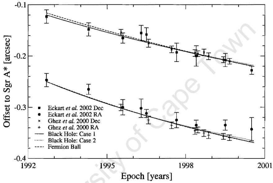
Figure 24: Best fits for S0-4. “Black Hole: Case 1” has z=0 arcsec, v_z=-1190 km/s with an unbound orbit and \chi_{ndf}^2 = 0.68 . “Black Hole: Case 2” has z=0 arcsec, v_z=0 km/s with a bound orbit of \chi_{ndf}^2 = 0.72 . The “Fermion Ball” case has z=0.072 arcsec, v_z=-410 km/s with a bound orbit and \chi_{ndf}^2 = 0.65 .
