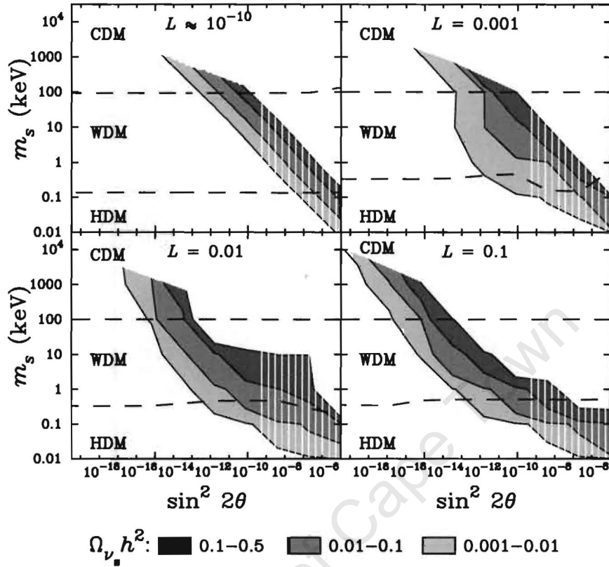
Figure 32: Regions of \Omega_{\nu_s} produced by resonant and non-resonant electron neutrino mixing with a sterile neutrino. L denotes lepton asymmetry. Regions of parameter space disfavoured by supernova core collapse considerations are shown with vertical stripes. From [25].
