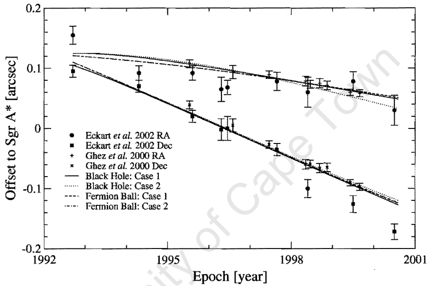
Figure 20: Best fits for S0-1. “Black Hole: Case 1” has z=0.012 arcsec, v_z=3190 km/s with an unbound orbit and \chi_{ndf}^2 = 2.06 . “Black Hole: Case 2” has z=0.075 arcsec, v_z=1360 km/s with a bound orbit and \chi_{ndf}^2 = 2.54 . “Fermion Ball: Case 1” has z=0.072 arcsec, v_z=-1940 km/s with an unbound orbit and \chi_{ndf}^2 = 2.02 . “Fermion Ball: Case 2” has z=0 arcsec, v_z=0 km/s with a bound orbit and \chi_{ndf}^2 = 2.03 .
