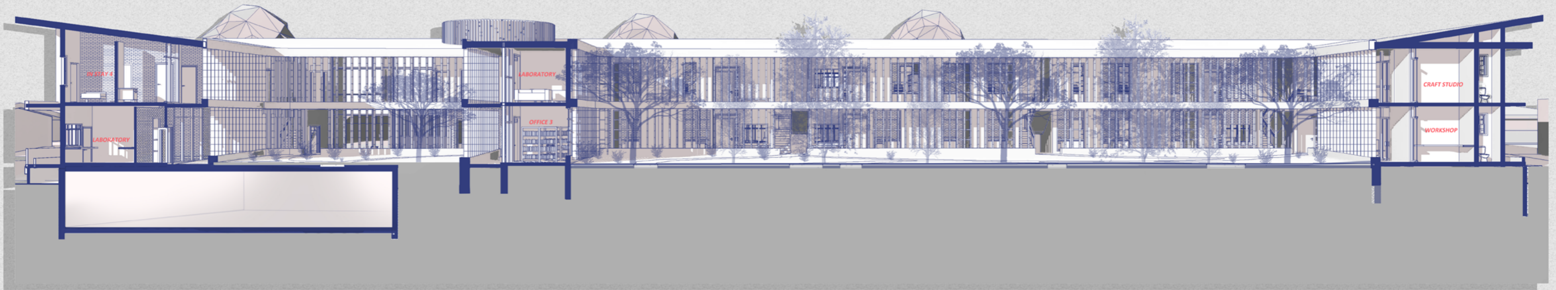
SOUTH WEST SECTIONAL PERSPECTIVE SCALE 1:100 1 - 100
