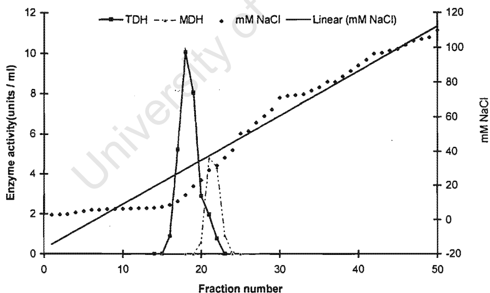
Fig. 7. Elution pattern of tauropine dehydrogenase from extract of Haliotis midae adductor muscles on DEAE-Sephacel. The gradient profile ( — ) is expressed as concentration of sodium chloride added to the equilibrium buffer ( 50 mM imidazole buffer, pH 7.2). Assay condition for tauropine dehydrogenase activity: 50 mM imidazole / HCl, pH 7.0, 0.15 mM NADH, 2.5mM pyruvate, 80 mM taurine.
