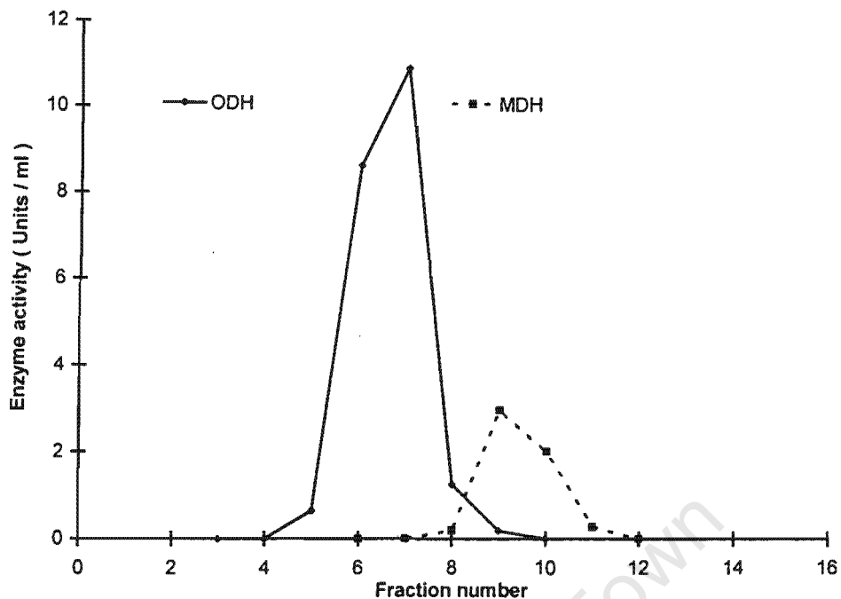
Fig 8. Elution pattern of octopine dehydrogenase from mantle muscle of Loligo vulgaris on DEAE-Sephacel, 10 mM Tris / HCl buffer pH 5.0. Assay conditions for octopine dehydrogenase activities : 10 mM Tris / HCl buffer, pH 5.0, 0.15 mM NADH, 2.5 mM pyruvate, 5 mM arginine.
