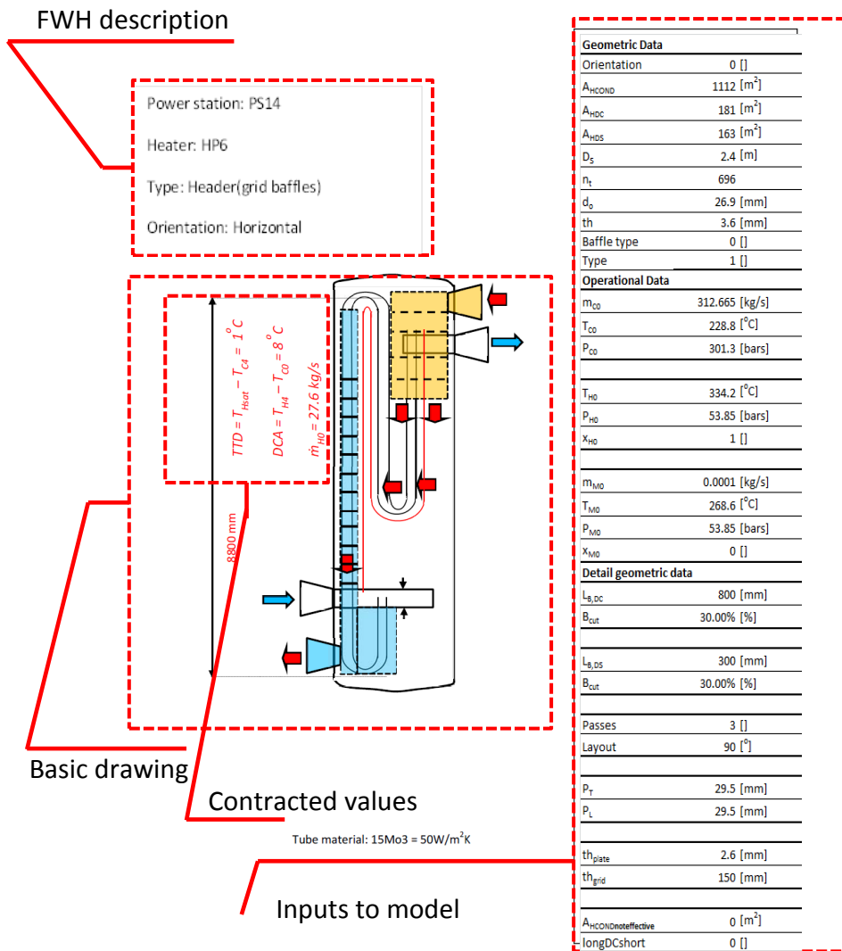
Figure 5-8. Extract from Appendix C illustrating input sheet for the HP6 FWH from station PS14
