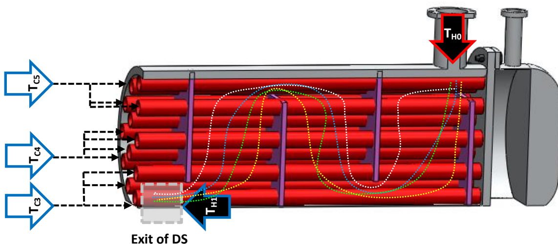
Figure 3-14. Cross section view through DS with the possibility of three different inlet tube temperatures applicable for a three zone heater [27]
