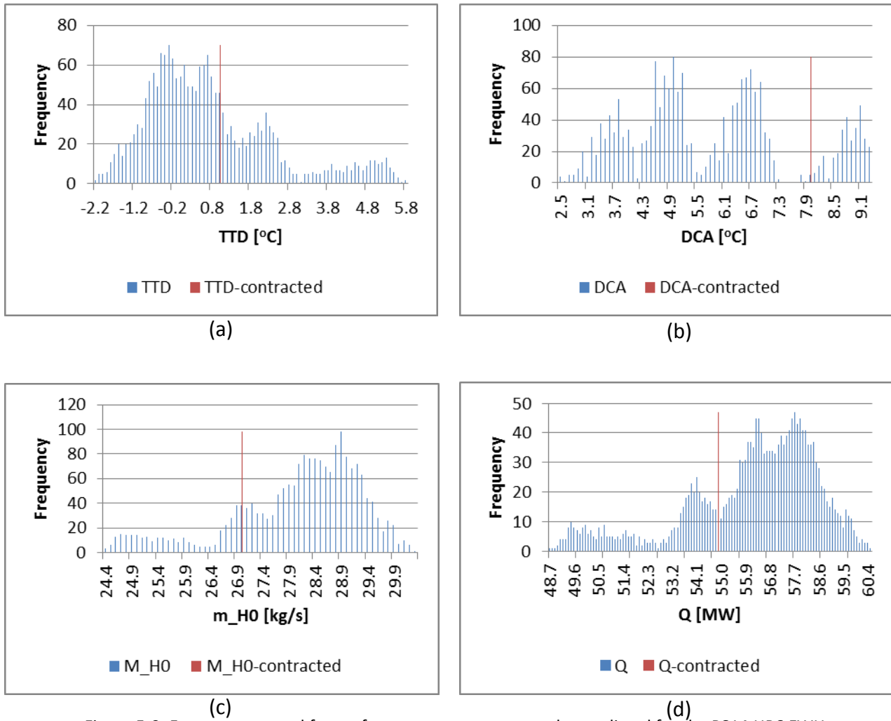
Figure 5-9. Frequency spread for performance parameter results predicted for the PS14 HP6 FWH
