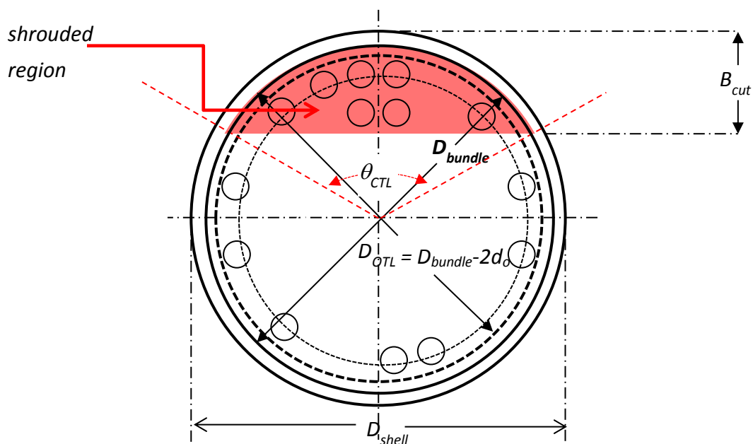
Figure 2-25. Baffle and tube bundle geometry for shrouded region within a STHE applying the Bell-Delaware model
