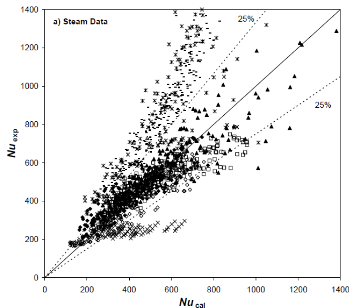
Figure 2-37. Comparison of the McNaught correlation to experimental data [42]
