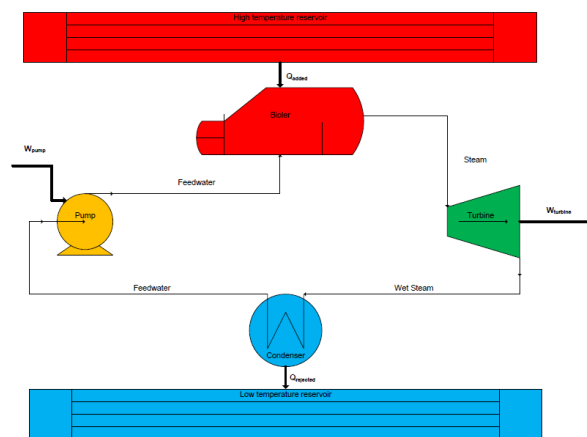
Figure 2-1. Illustration of a basic power generation cycle
