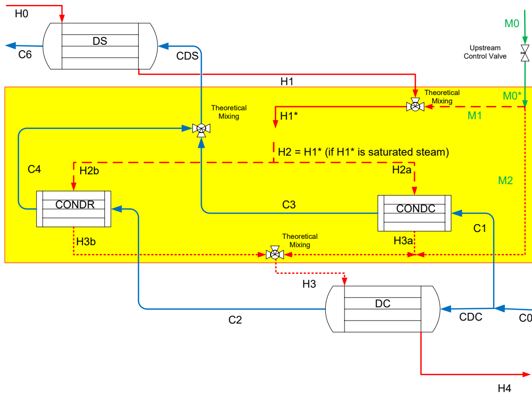
Figure 3-12. General process flow diagram for a 3 zone FWH
