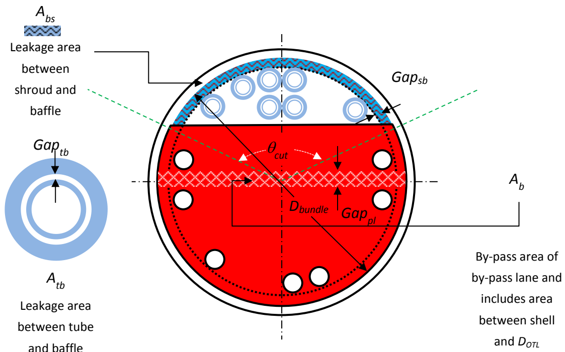
Figure 2-26. Leakage and by-pass areas of a tube bundle
