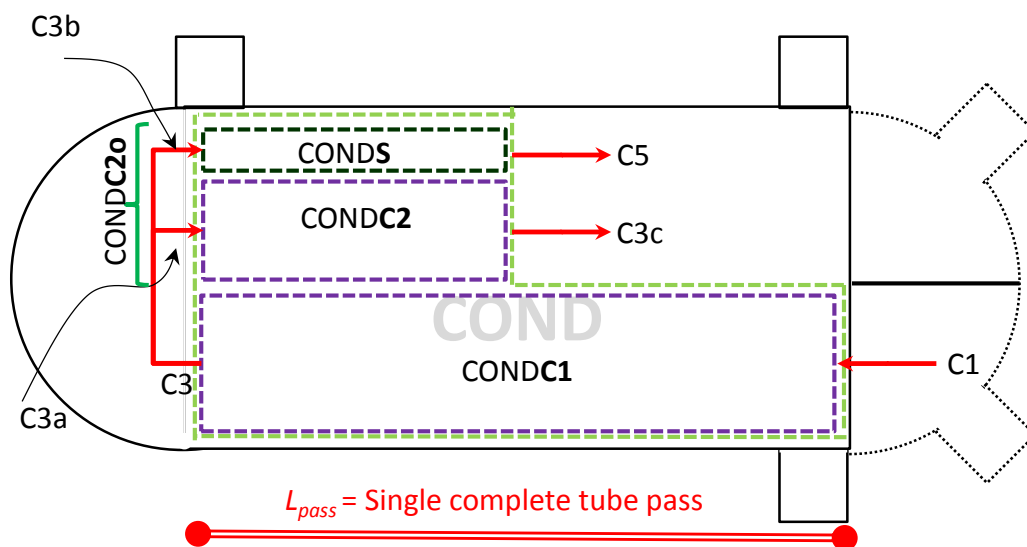
Figure 4-6. Designation and the location of COND S sub-zone and associated feedwater streams for a FWH with no DC
