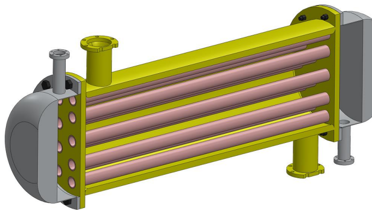
Figure 2-17. Illustration of an un baffled shell where tubes are only supported at their ends by the tube plates [27]
