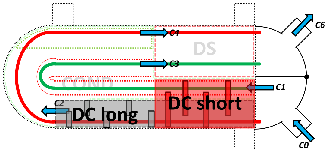
Figure 3-15. FWH fitted with either a long or short DC
