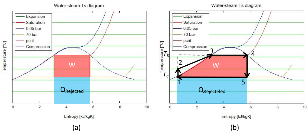
Figure 2-2. T-S diagram of a Carnot (a) and Rankine cycle (b) for a hypothetical power station
