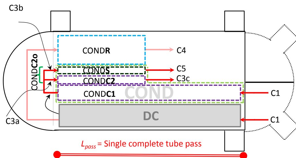
Figure 4-7. Designation and the location of COND S sub-zone and associated feedwater streams for a FWH with a DC
