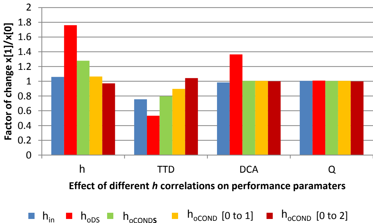
Figure 5-1. Effect of the option 1 or option 2 correlation on the performance parameters relative to the results from the option 0 correlation (PS14 HP6 case study)
