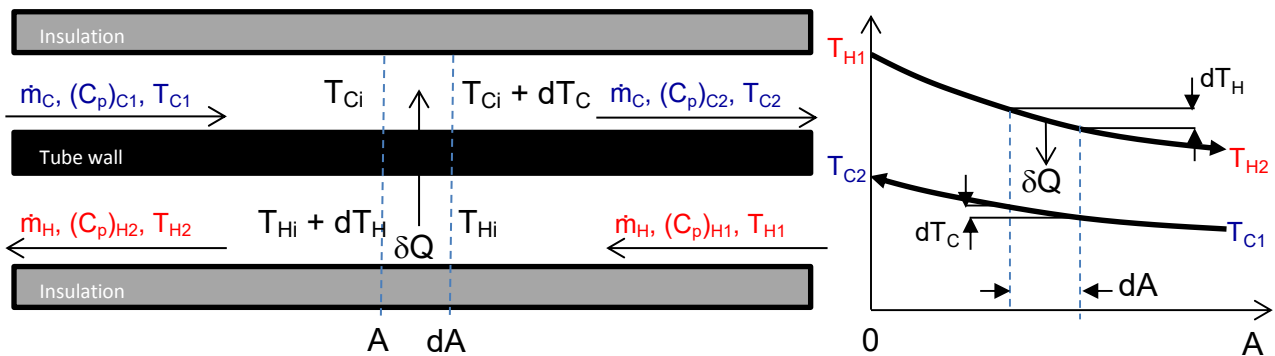
Figure 2-6. Assignment of thermal parameters and the associated temperature profiles for hot and cold streams for a two-fluid heat exchanger
