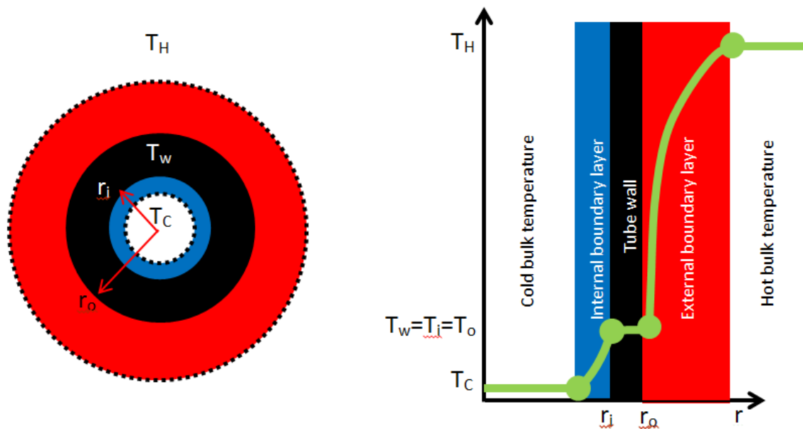
Figure 2-7. Radial temperature profile across a single tube of a heat exchanger
