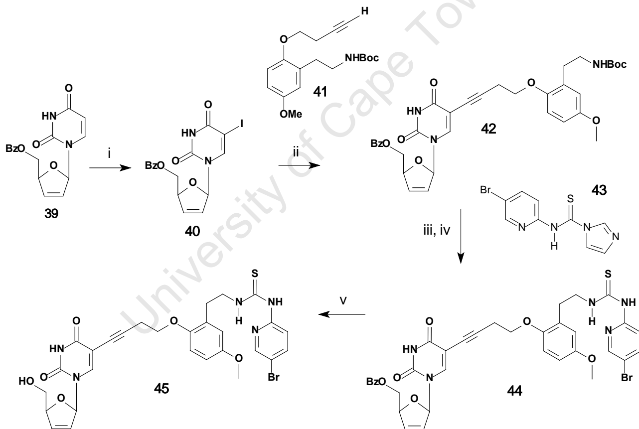
Scheme 1.10 Reagents and Conditions: (i) I 2 , CAN, CH 3 CN, 60 °C, 1 h (80%); (ii) alkyne 38 , (PPh 3 ) 4 Pd (10%), CuI (50%), Et 3 N (2 eq.), DMF:THF (1:2), rt, 4 h (69%); (iii) CF 3 COOH, CH 2 Cl 2 , 0 °C; (iv) EtN(i-Pr) 2 followed by 40 , THF, rt / overnight (60% for 2 steps); (v) NaOMe (cat), MeOH, 0 °C, 20 min (51%).
