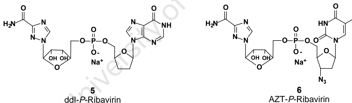
Figure 1.41 Structures of AZT, ddl, Ribavirin and HEPU heterodimers.
