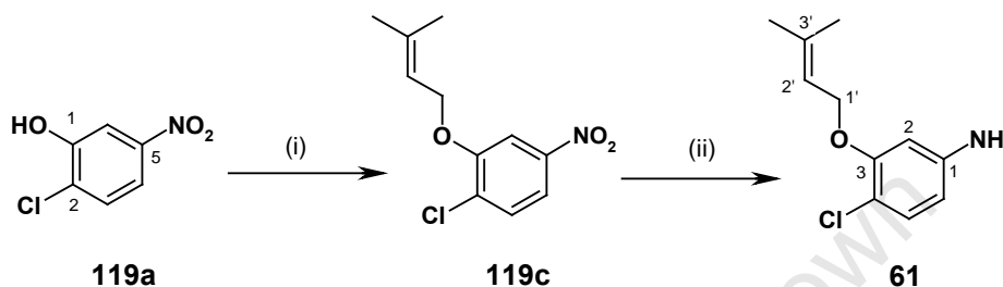
Scheme 3.2 Reagents and conditions: (i) 4-bromo-2-methyl-2-butene, \text{K}_2\text{CO}_3 , n\text{-Bu}_4\text{NI} , MEK, r.t (94%); (ii) Fe mesh, HCl, \Delta (88%).
