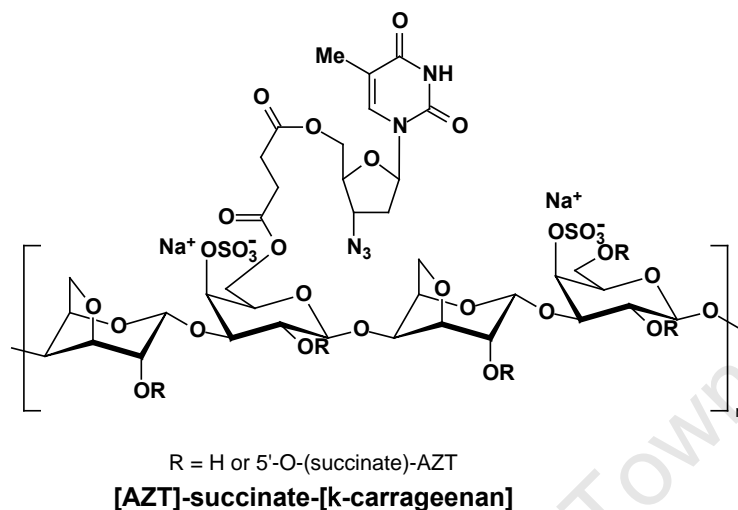
Figure 1.40 Structure of [AZT]-succinate-[k-Carrageenan Conjugates].
