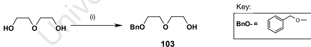
Scheme 2.11 Reagents and conditions: (i) BnBr, NaH, THF, rt (70%).
