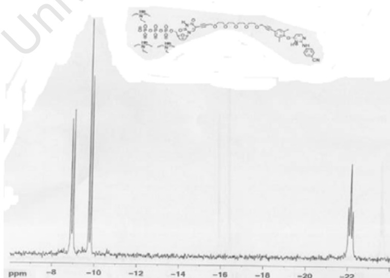
Figure 4.9 ^{31}\text{P} NMR of [d4U-TP]-propyne-4-PEG-propyne-[TMC120] 148 .
