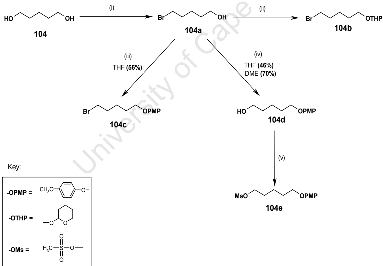
Scheme 2.12 Reagents and conditions: (i) HBr, H 2 O, toluene, \Delta (55%); (ii) DHP, Amberlite®, CH 2 Cl 2 (82%); (iii) p -methoxyphenol, PPh 3 , DIAD, THF (56%); (iv) p -methoxyphenol, NaH, solvent, \Delta (THF-46%, DME-70%); (v) MsCl, pyr, CH 2 Cl 2 , DMAP, rt (93%).
