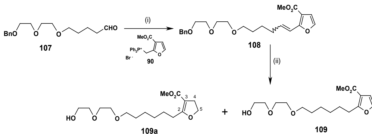
Scheme 2.15 Reagents and conditions: (i) phosphonium salt 90 , NaOMe, MeOH, rt (81%); (ii) H 2 , Pd/C, EtOH, rt.
