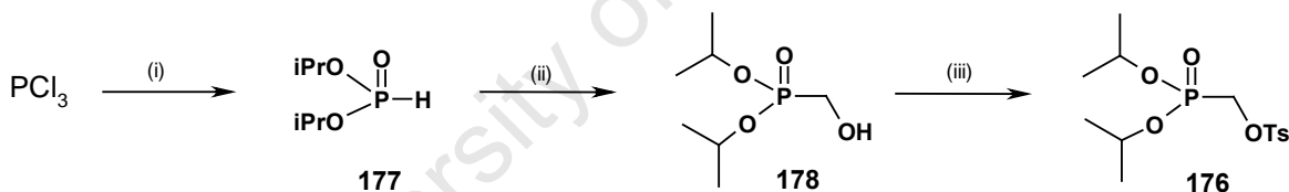
Scheme 4.10 Reagents and conditions: (i) IPA (3eq), NaH (2eq), THF, r.t (98%); (ii) (\text{H}_2\text{CO})_n , \text{K}_2\text{CO}_3 , IPA, 60 °C (98%); (iii) p -TsCl, \text{NEt}_3 , \text{CH}_2\text{Cl}_2 , DMAP (cat), r.t (92%).
