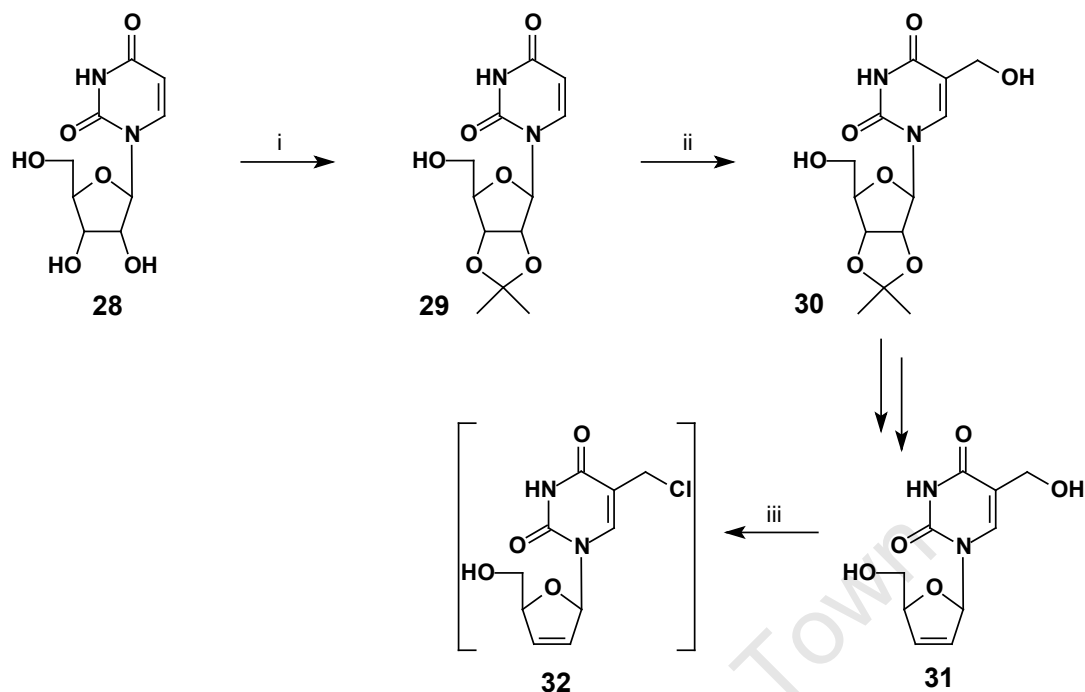
Scheme 1.7 Reagents and Conditions: (i) 2,2-DMP, APTS, MeCOMe. (ii) \text{CH}_2\text{O} , \text{Et}_3\text{N} , 60\text{ }^\circ\text{C} ; 93%. (iii) \text{TMSCl} , 1,4-dioxane, 60\text{ }^\circ\text{C} .
