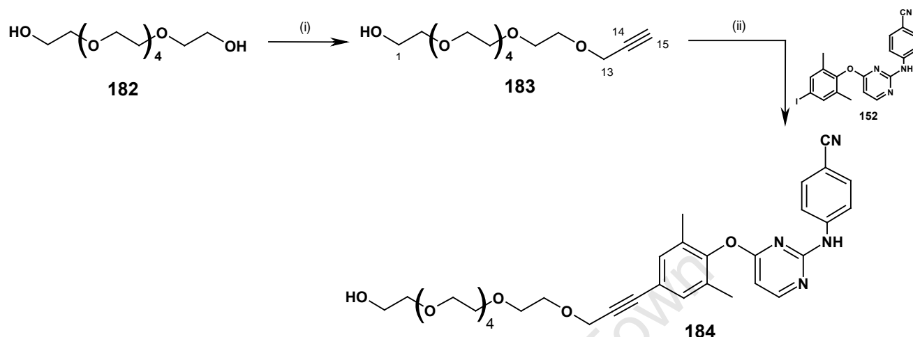
Scheme 4.14 Reagents and conditions: (i) propargyl bromide, NaH, THF, r.t (53%); (ii) 152 , Pd(PPh 3 ) 4 (10%), CuI (50%), NEt 3 (2 eq), DMF/THF (1:2), r.t (46%).
