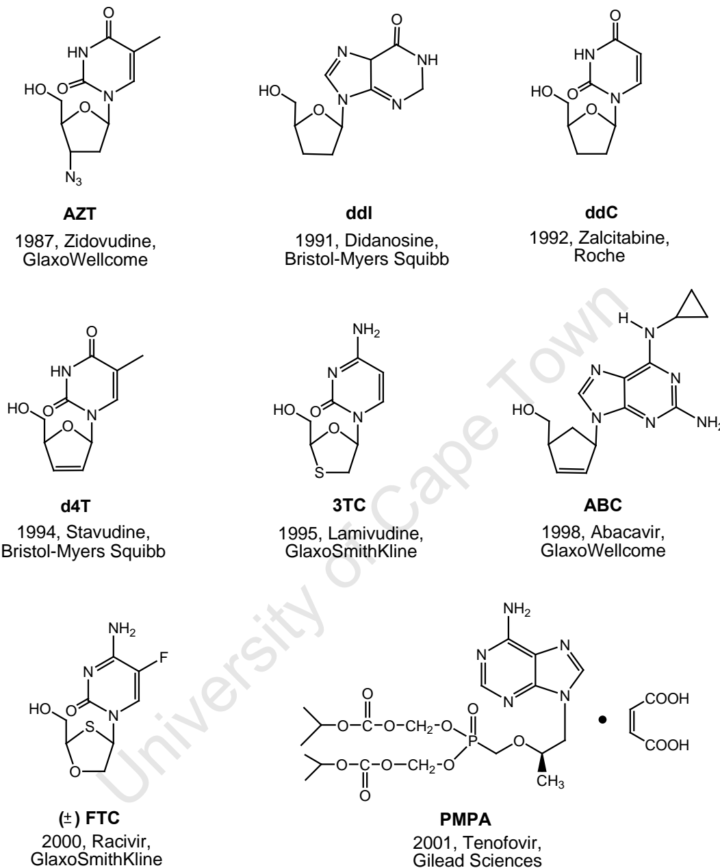
Figure 1.8 Nucleoside reverse transcriptase inhibitors and Tenofovir (PMPA).
