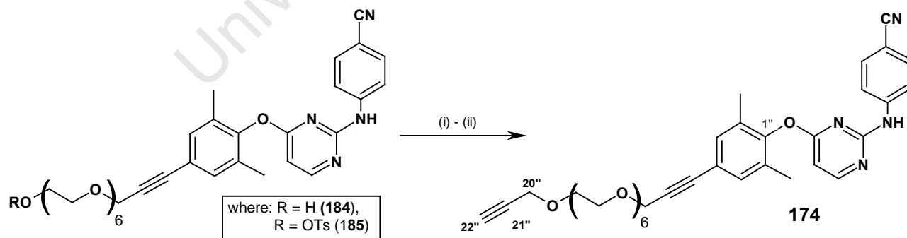
Scheme 4.15 Reagents and conditions: (i) p -TsCl, NEt 3 , CH 2 Cl 2 , DMAP (cat) (57%); (ii) propargyl alcohol, NaH, THF, \Delta (89%).
