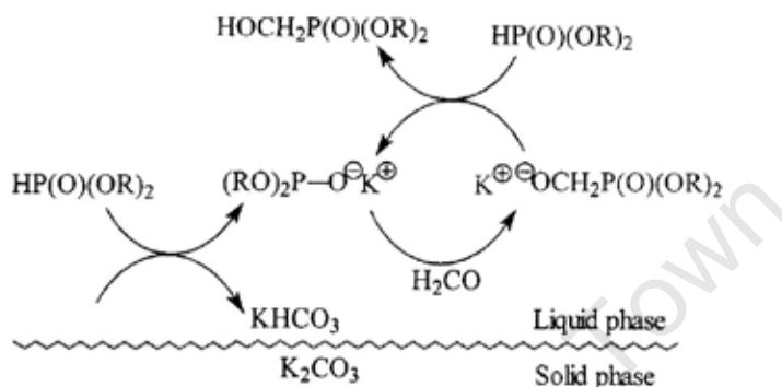
Figure 4.15 Proposed mechanism of the Pudovik reaction in heterogeneous conditions. 202
