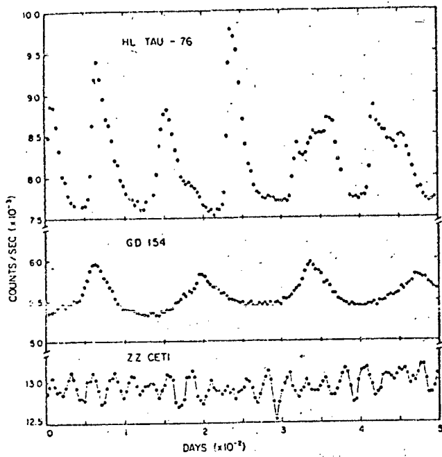
Figure 11. Typical light curves for 3 of the ZZ Ceti stars.
