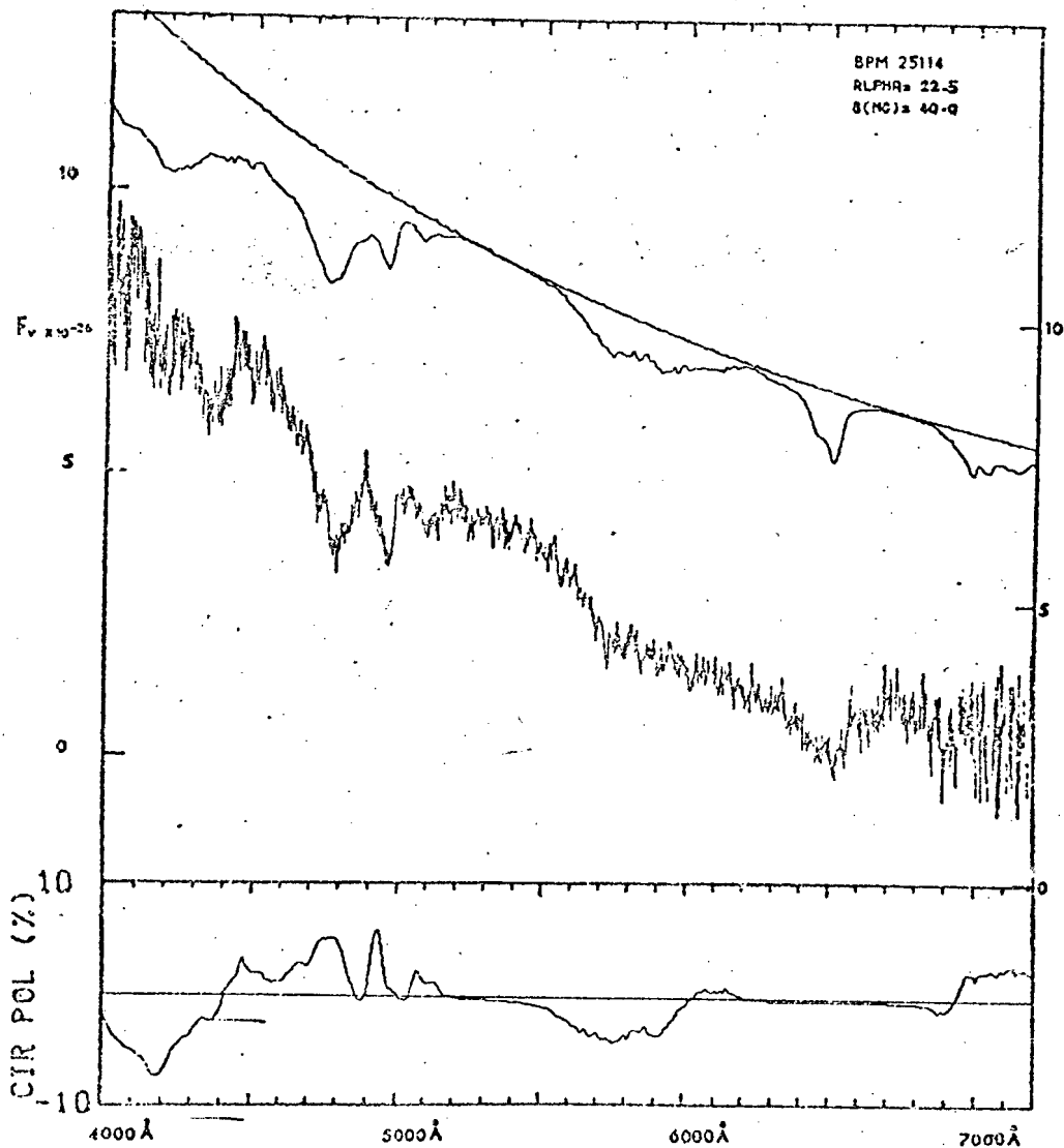
Figure 5. Observed and theoretical fluxes and theoretical circular polarization for BPM 25114. The zero of the theoretical curve, a model 20 000 K magnetic white dwarf with dipole strength 40 MG and viewing angle 22.5^\circ , is marked as such. The zero of the observations is the upper annotated axis corresponding to +10% circular polarization. The observed and theoretical curves are normalized at 4000 Å. The smooth theoretical curve is the predicted continuum.
