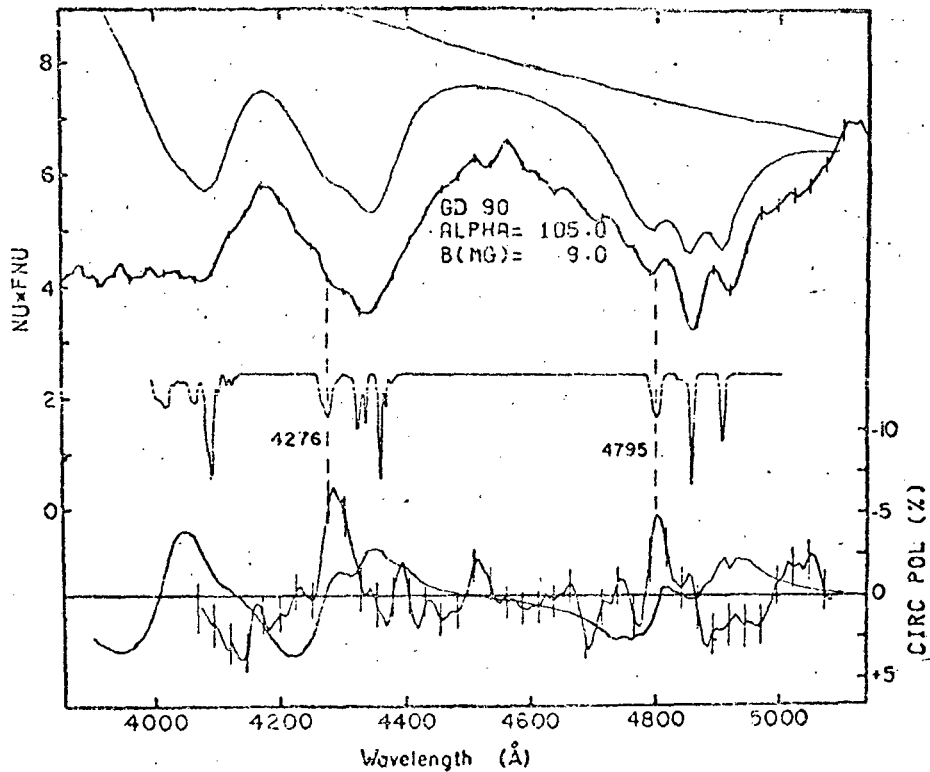
Figure 7. Observations of line and polarization profiles for GD 90 taken from Angel et al. (1974a), together with theoretical model curves. The top two represent continuum and line profiles for a 12000 K magnetic white dwarf, centred dipole of strength 9 MG and viewing angle 105^\circ . The theoretical and observed profiles are normalized at 4600 Å and the vertical axis \nu f_\nu has an arbitrary scale. The theoretical polarization curve (no error bars) is plotted on the same axis as the observed curve.
