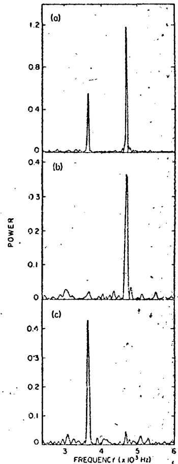
Figure 12. Power spectra of the light curve of ZZ Ceti on U.T. dates (a) 6 October, 1975 ; (b) 7 October, 1975 ; (c) 8 October, 1975.
