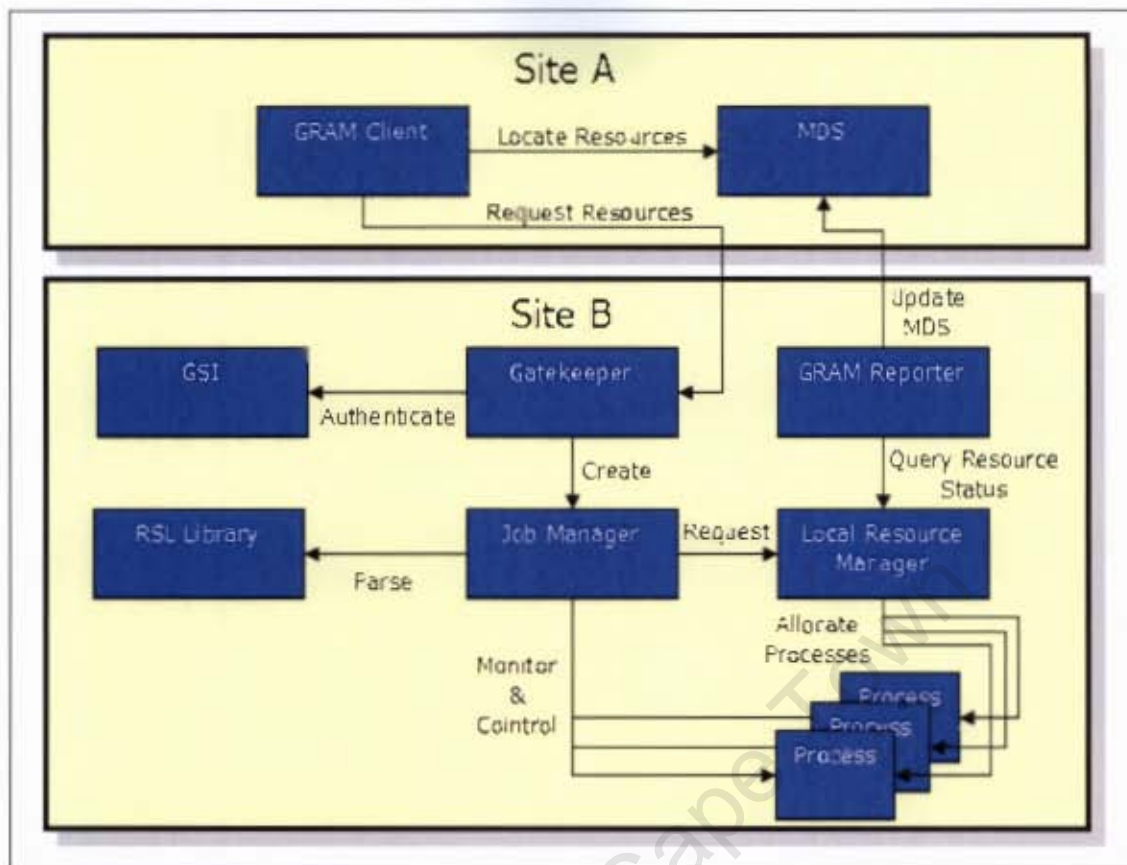
Figure 2.2: Globus GRAM workflow
