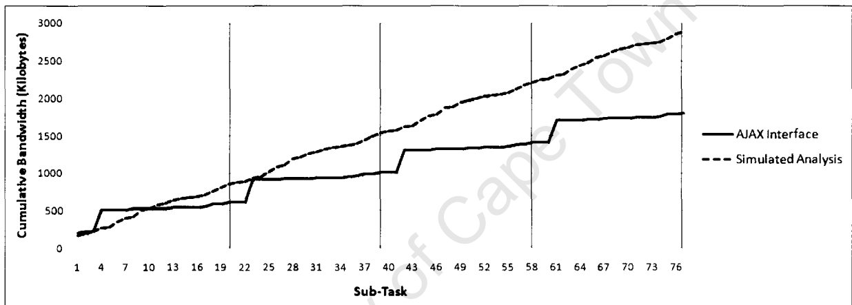
Figure 7.5: Cumulative bandwidth usage of the AJAX interface vs. an identical hypothetical non-dynamic HTML-only interface for four consecutive repetitions of the interface usage scenario
