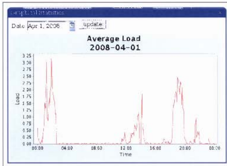
Figure 5.16: Statistics Component
