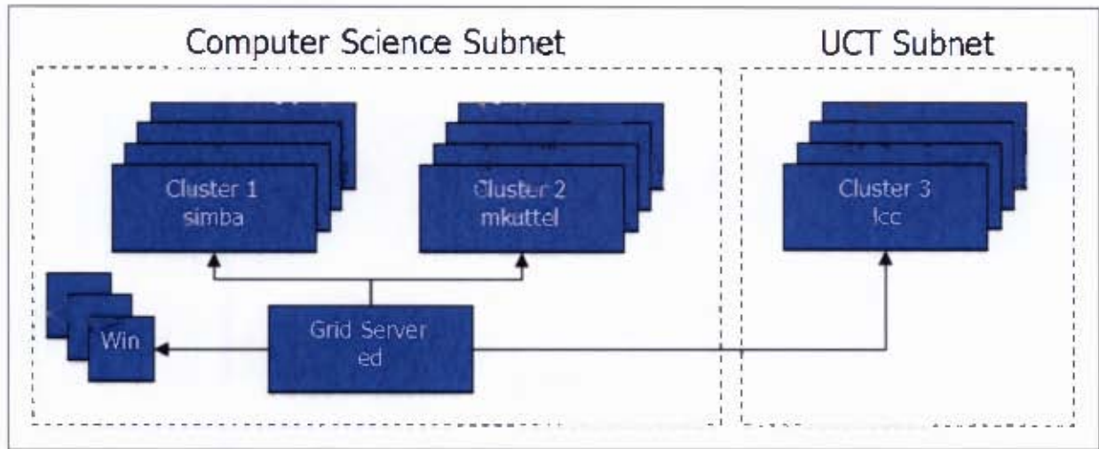
Figure 5.1: High-level Grid architecture with the Condor flocking system
