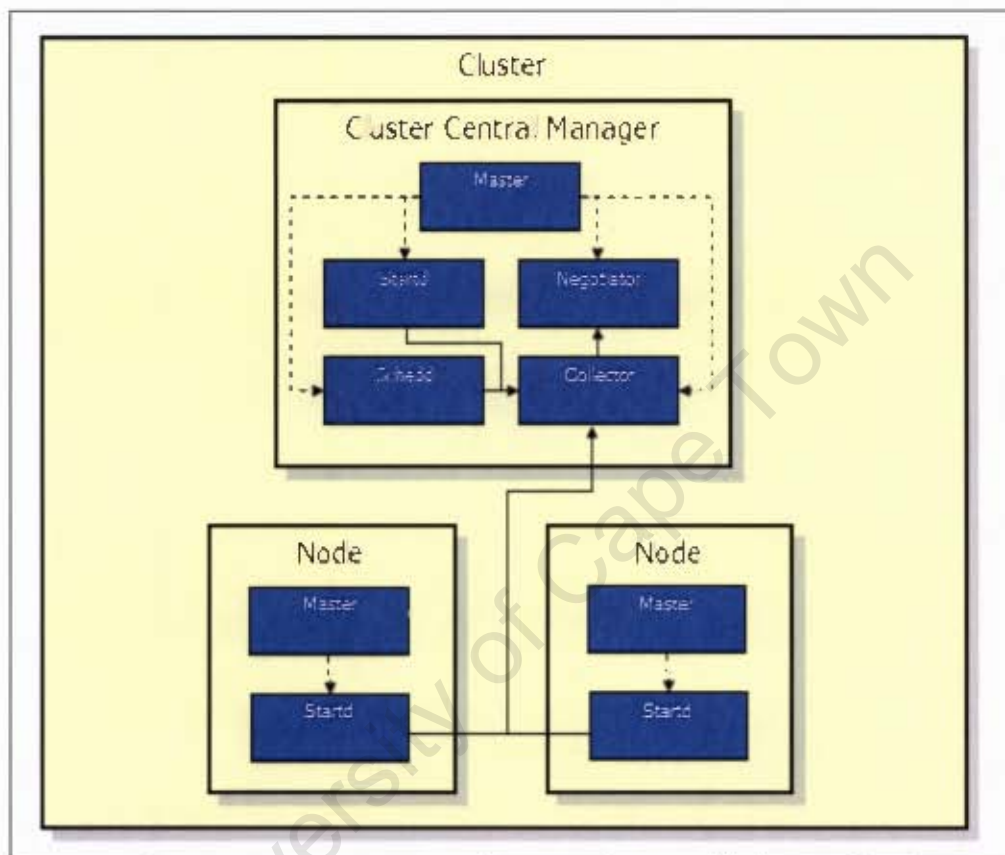
Figure 3.1: Condor Communication Layer
