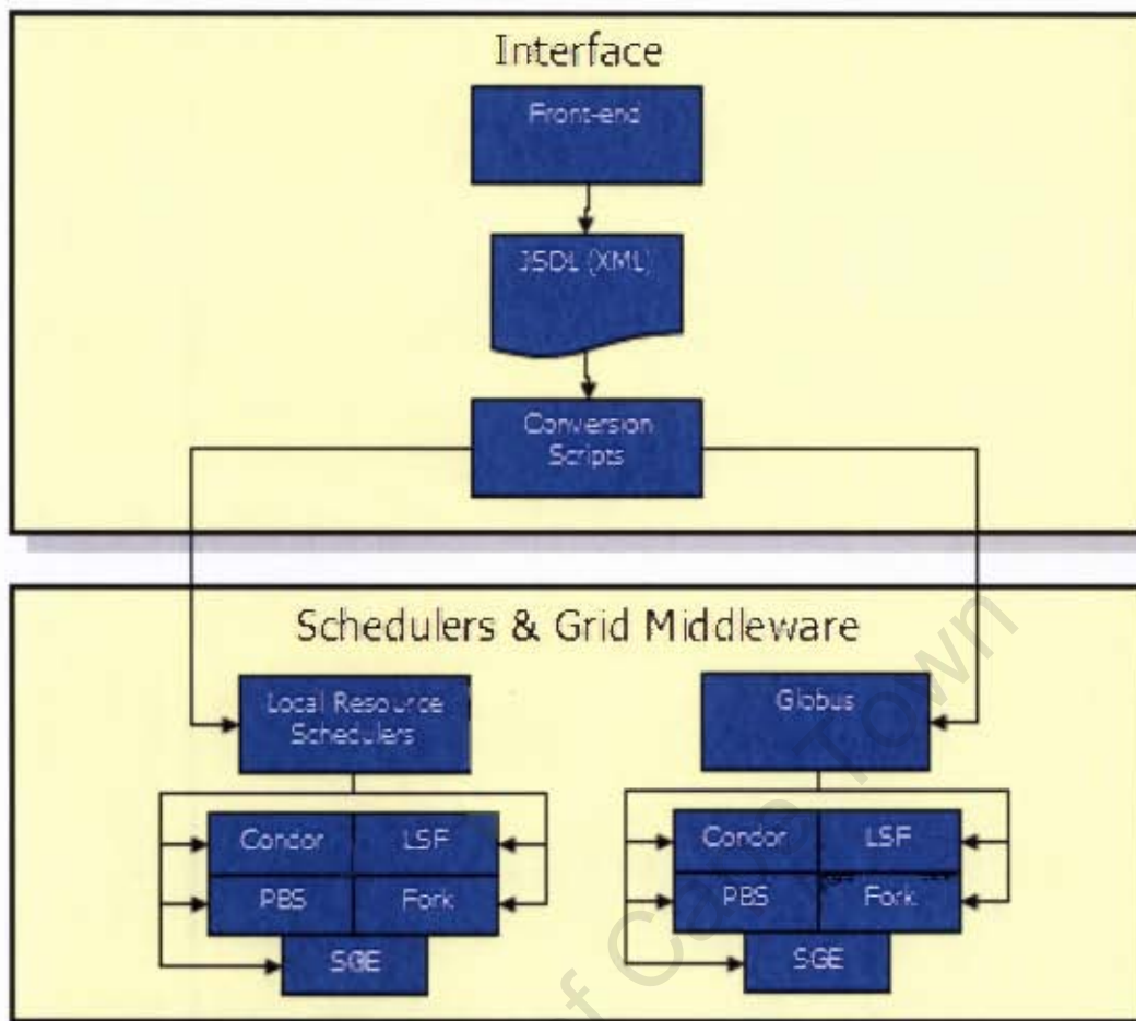
Figure 2.4: Conversion of custom front-end data into system neutral JSDL
