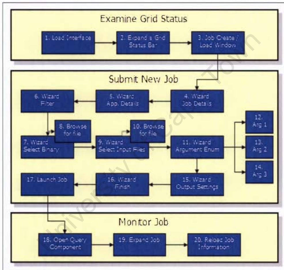
Figure 7.1: User evaluation tasks represented as a flowchart of sub-tasks
