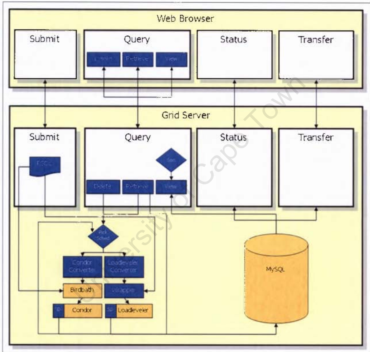
Figure 5.4: High-level system architecture. Components coloured in yellow represent existing systems, those coloured in purple represent custom-built components.
