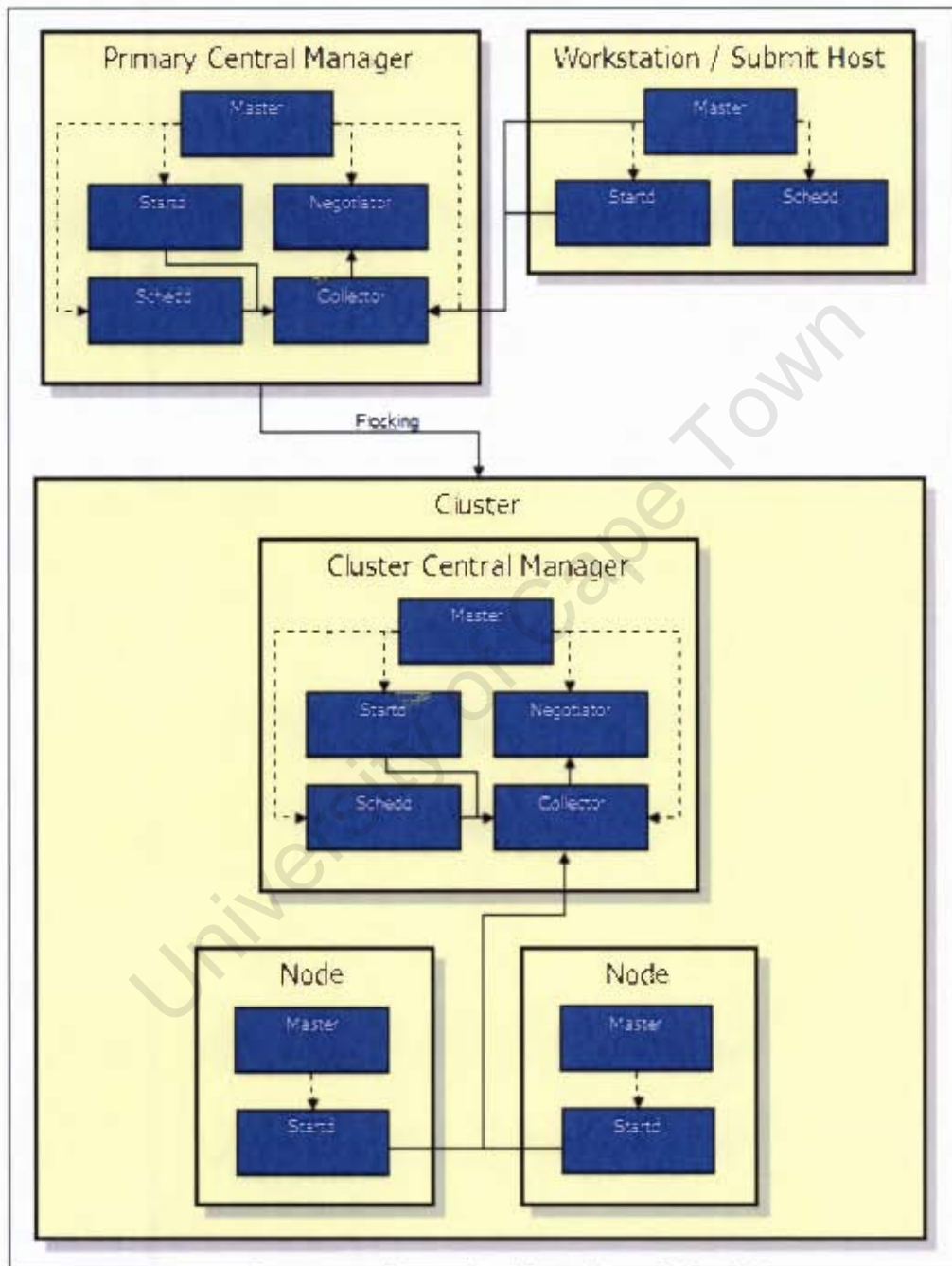
Figure 3.4: Condor Flocking Architecture
