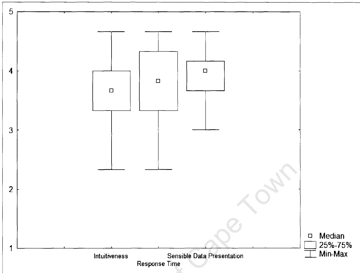
Figure 7.2: Box and Whisker plots of intuitiveness, response time and data presentation for the entire Grid interface
