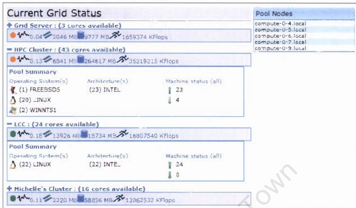
Figure 5.5: Grid status component
