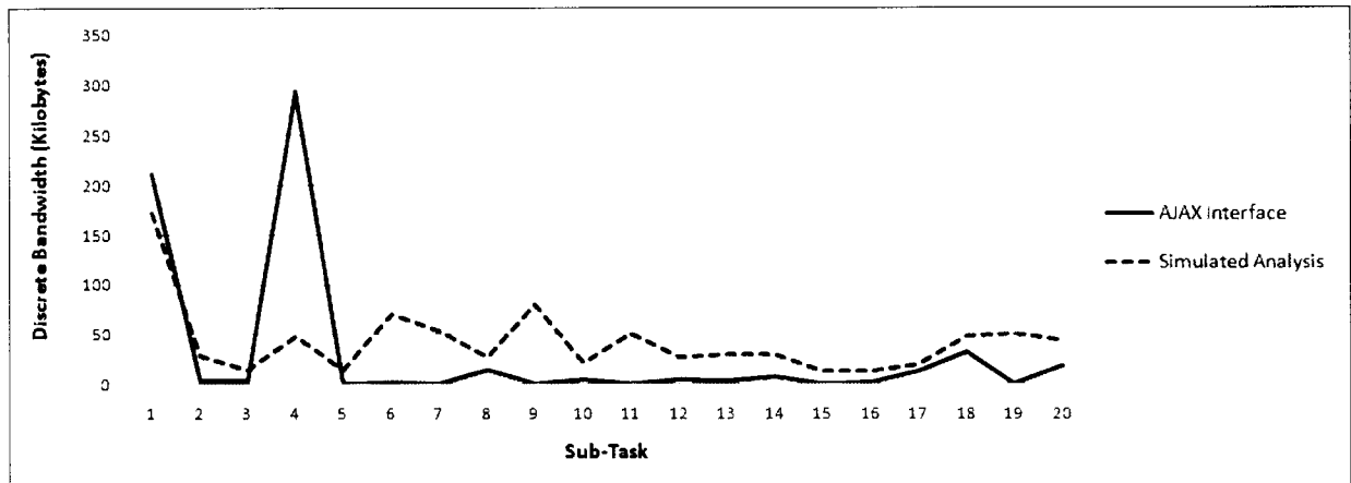
Figure 7.6: Discrete bandwidth consumption of the AJAX interface vs. an identical hypothetical non-dynamic interface for the interface usage scenario
