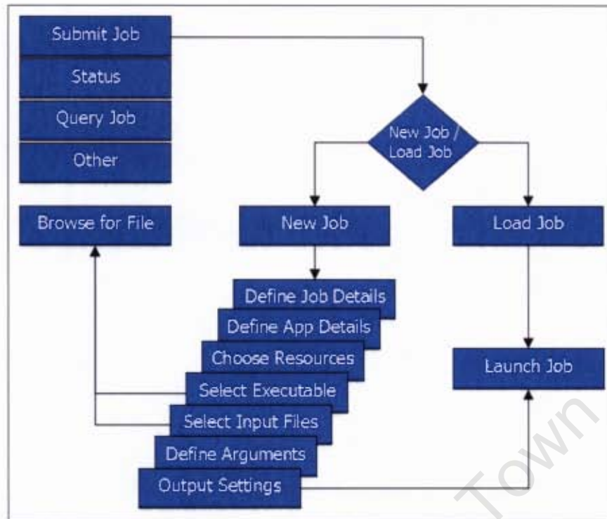
Figure 5.3: Interface component flowchart
