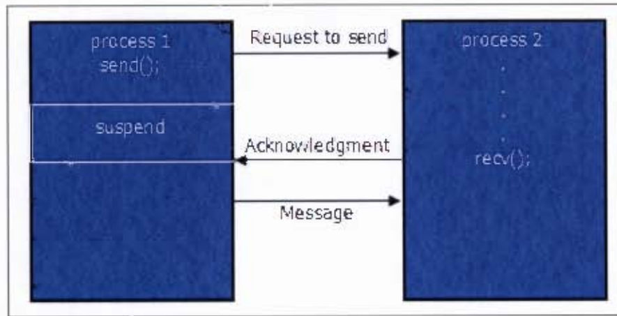
Figure 2.1: Message Passing Example
