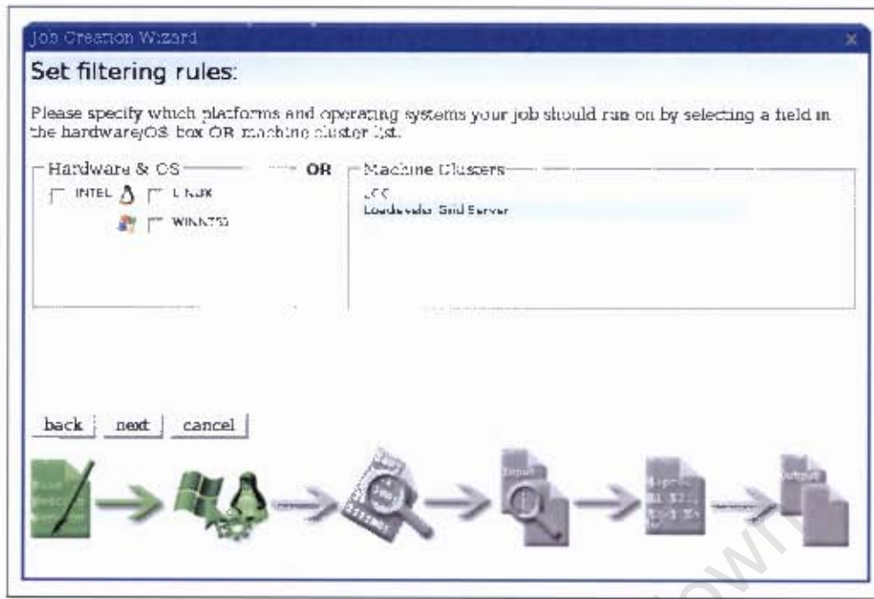
Figure 5.7: Resource Filtering Wizard
