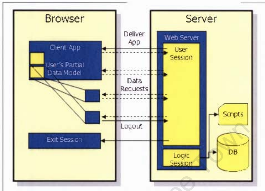
Figure 2.6: AJAX Web Application
