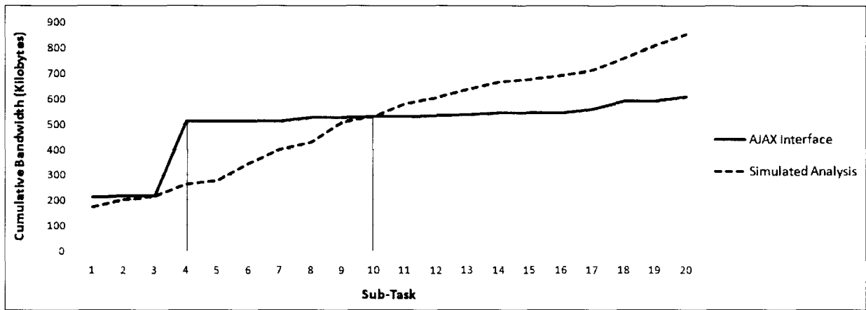
Figure 7.4: Cumulative bandwidth usage of the AJAX interface vs. an identical hypothetical non-dynamic HTML-only interface for the interface usage scenario
