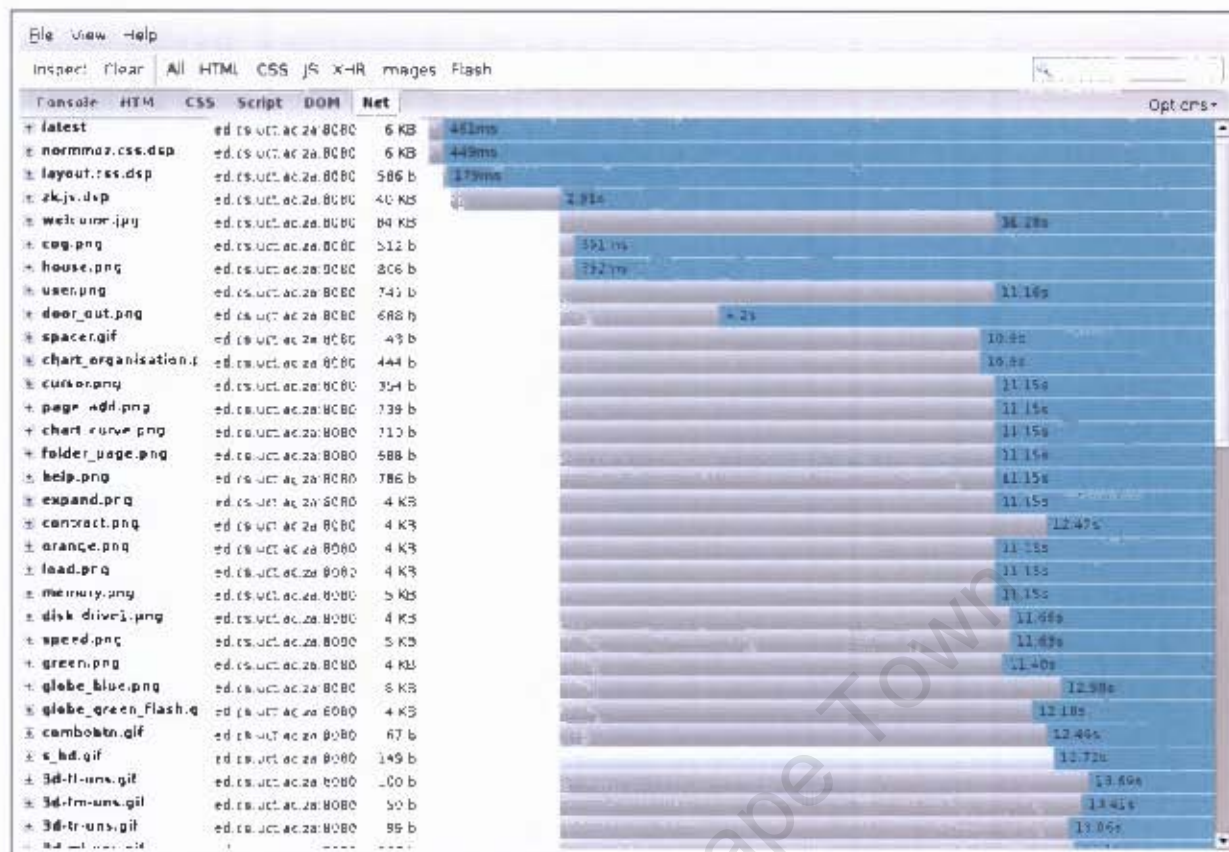
Figure 7.3: Firebug in action during interface loading
