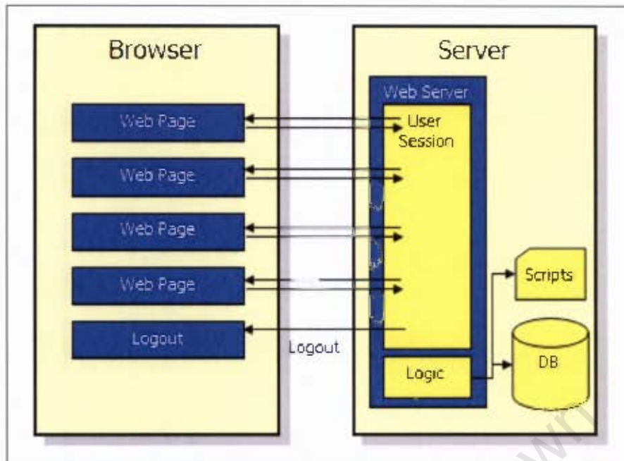
Figure 2.5: Traditional Web Application
