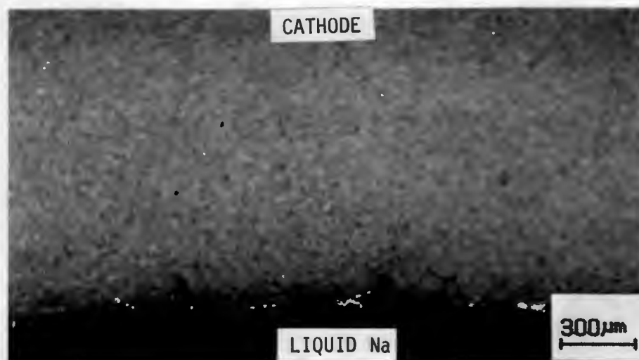
FIGURE 7.11. AN OPTICAL MICROGRAPH OF AN Ag DECORATED POLISHED CROSS-SECTION OF THE ELECTROLYTE WALL FROM AN OVERDISCHARGED CELL.
