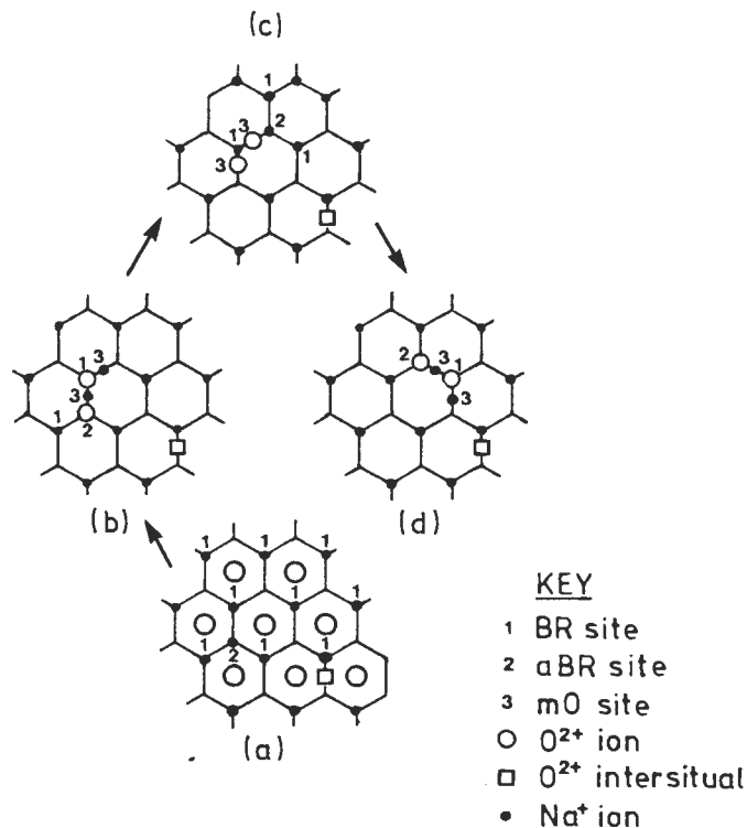
FIGURE 3.5. THE CONDUCTION MECHANISM IN \beta -ALUMINA.
