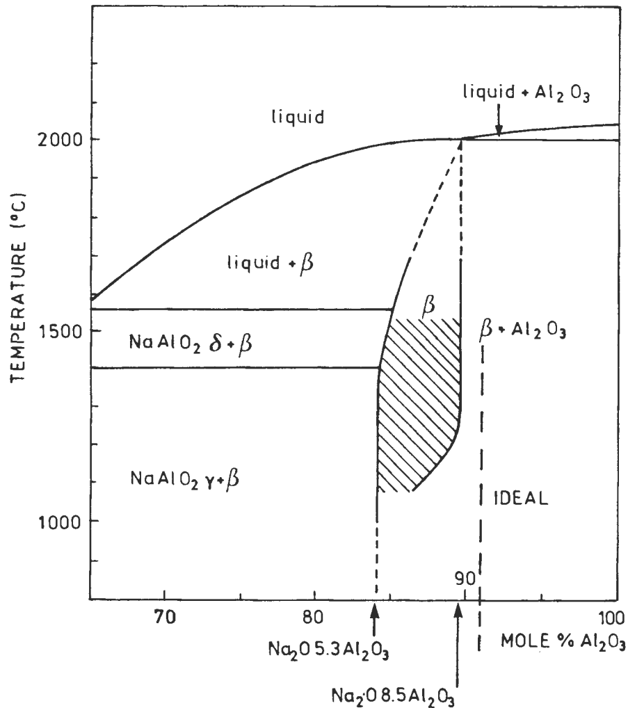
FIGURE 3.3. THE Na 2 O/Al 2 O 3 PHASE DIAGRAM.
