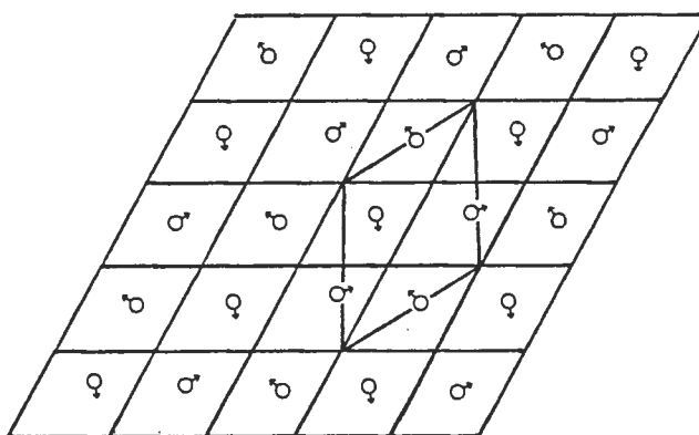
FIGURE 3.4. THE SUPERSTRUCTURE FORMED BY THE \text{Na}^+ IONS IN THE CONDUCTION PLANE OF \beta -ALUMINA.
