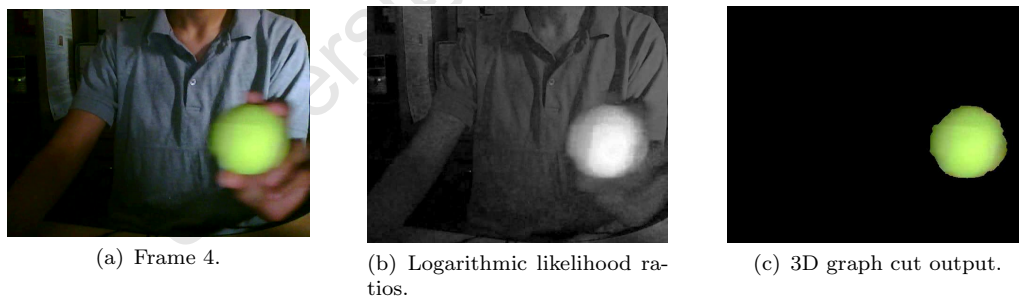
FIGURE 5.7: Region properties using GMMs in 3D graph cuts. The (a) original frame 4 is segmented using graph cuts in (c) based on probability maps in (b).
