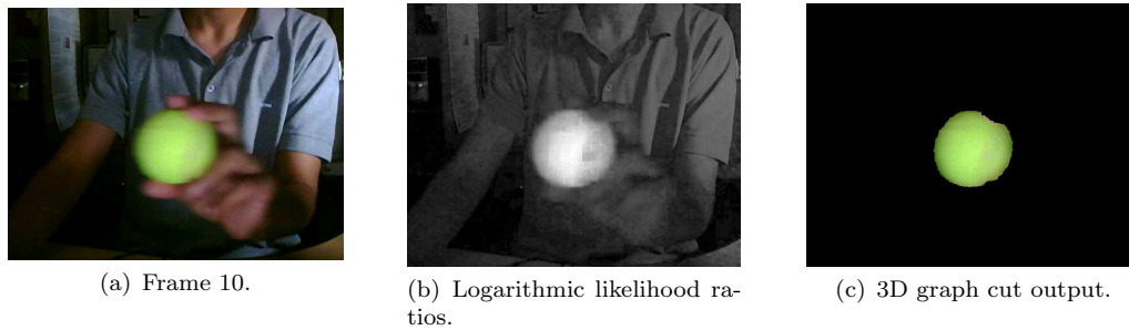
FIGURE 5.8: Region properties using GMMs in 3D graph cuts. The (a) original frame 10 is segmented using graph cuts in (c) based on probability maps in (b).
