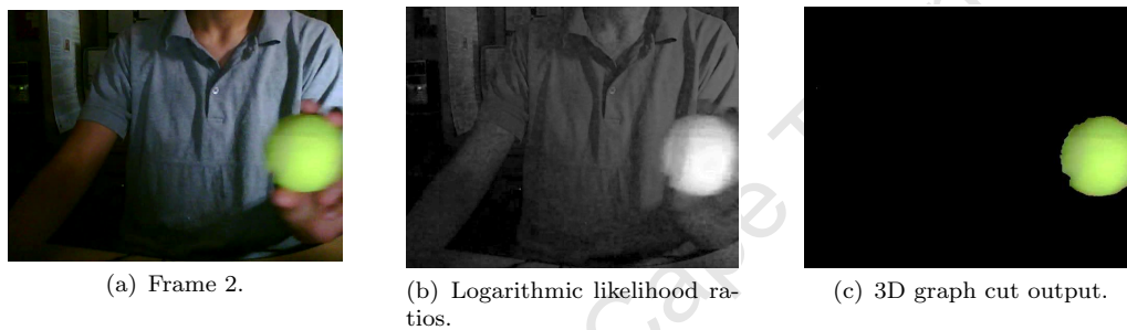
FIGURE 5.6: Region properties using GMMs in 3D graph cuts. The (a) original frame 2 is segmented using graph cuts in (c) based on probability maps in (b).
