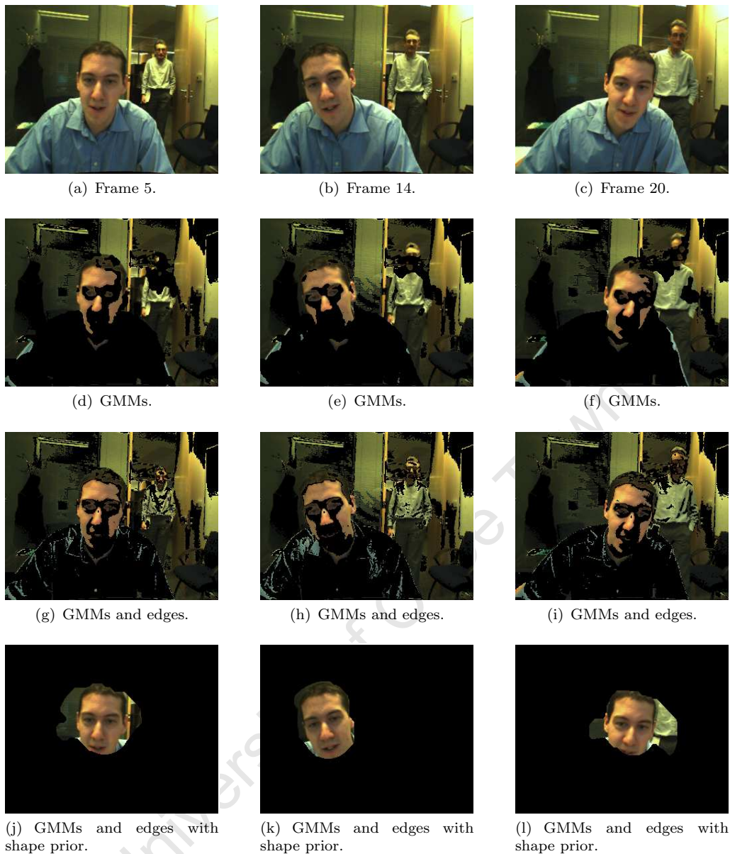
FIGURE 5.15: Comparison of segmentation methods on the ‘Geoff’ video sequence. Some frames (a-c) from the original sequence are shown in the first row. Segmentations using graph cuts and colour GMMs (d-f), GMMs with edge detection methods (g-i) and GMMs with shape priors (j-l) are shown.
