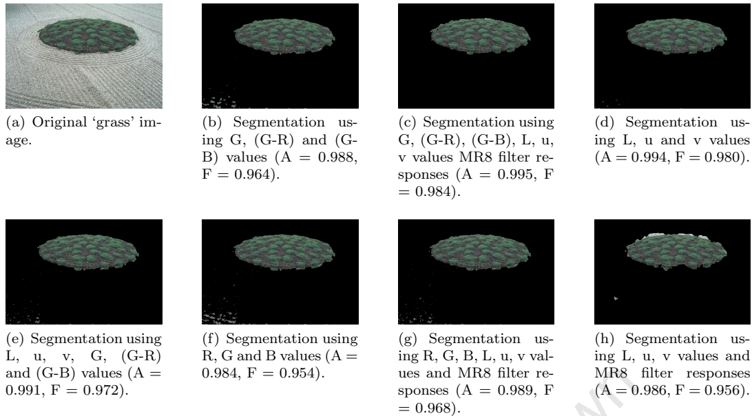
FIGURE 4.17: Segmentation of the 'grass' image using different region costs. Original image is shown in (a). Segmentations are shown for (b) G, (G-R) and (G-B) values, (c) G, (G-R), (G-B), L, u, v values and MR8 filter responses, (d) L, u and v values, (e) G, (G-R), (G-B), L, u and v values, (f) R, G and B values, (g) R, G, B, L, u, v values and MR8 filter responses and (h) L, u, v values and MR8 filter responses.
