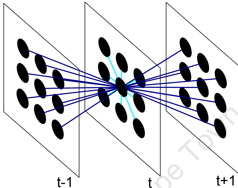
FIGURE 5.5: The 26-pixel neighbourhood connectivity of pixels in a video. The figure shows a connectivity of the center pixel in the frame at time t . Intra-frame connections are cyan and inter-frame connections are blue. Other pixels are connected in an analogous way.
