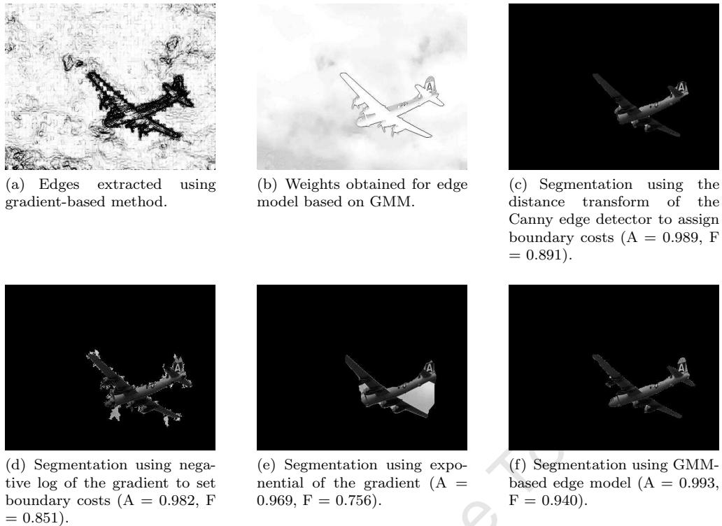
FIGURE 4.14: Different methods to set the boundary costs are evaluated. Gradient-based methods are used in (a) and a GMM-based edge model is used in (b). Segmentations achieved using boundary properties based on (c) the Canny edge detector with distance transform, (d) negative log of gradient, (e) gradient-based methods and (f) GMM-based edge model are shown. From (b) and (f) it can be clearly seen that the proposed edge model works better than other methods.
