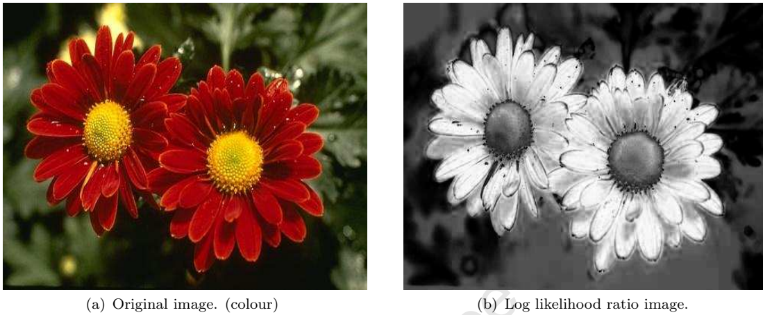
FIGURE 4.2: Original image and the logarithmic likelihood ratio of each pixel in the image based on GMMs of colour using RGB and Luv colour spaces.
