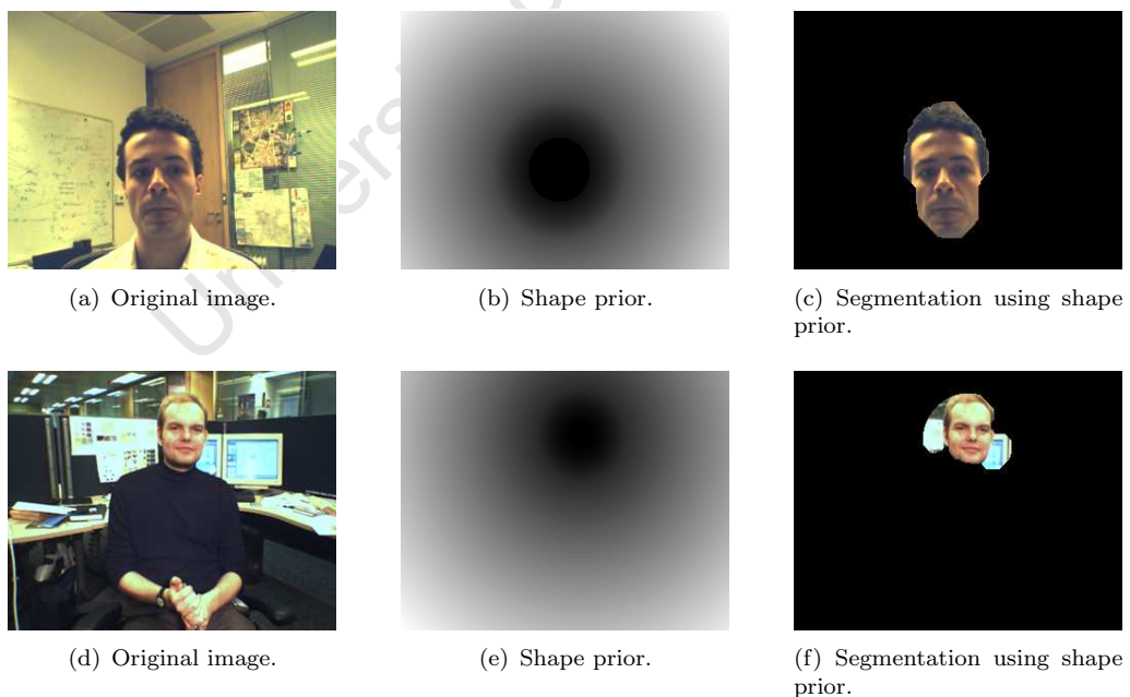
FIGURE 4.21: Image segmentation using shape priors and graph cuts. The figure shows (a) and (d) the original images, (b) and (e) the distance transform from the shape prior aligned using Powell's method, and (c) and (f) the output of the graph cut.
