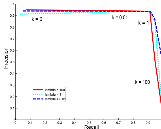
FIGURE 4.10: A family of precision-recall curves as \mathcal{K} and \lambda vary.
