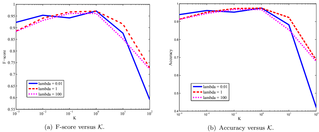
FIGURE 4.9: The effect of changes in \mathcal{K} on F-score and accuracy of the segmentation.
