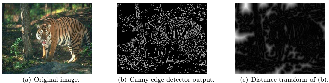
FIGURE 4.4: Assignment of boundary costs for (a) the original image. The edges detected by the Canny detector are shown in (b). The distance transform of (b) is shown in (c). A high value in (c) indicates that a large cost should be assigned to the boundary elements at the corresponding location.
