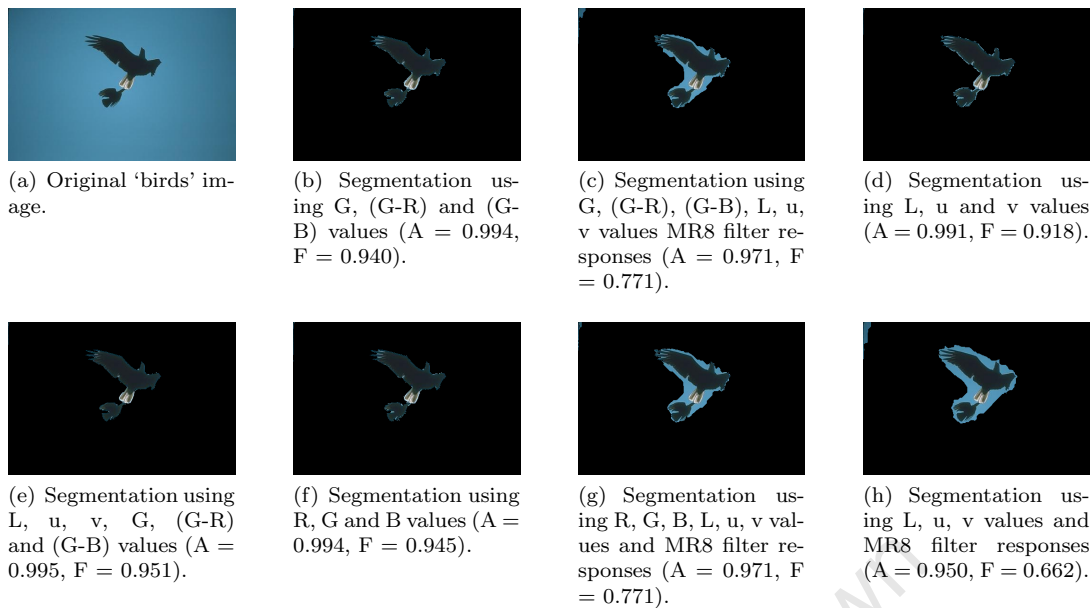
FIGURE 4.15: Segmentation of the 'birds' image using different region costs. Original image is shown in (a). Segmentations are shown for (b) G, (G-R) and (G-B) values, (c) G, (G-R), (G-B), L, u, v values and MR8 filter responses, (d) L, u and v values, (e) G, (G-R), (G-B), L, u and v values, (f) R, G and B values, (g) R, G, B, L, u, v values and MR8 filter responses and (h) L, u, v values and MR8 filter responses.
