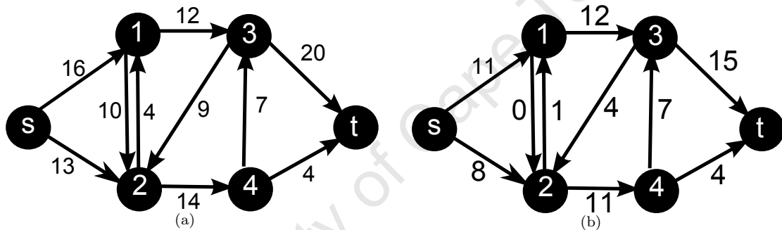
FIGURE 2.4: A flow network \mathcal{G} = (\mathcal{V}, \mathcal{E}) is shown in (a). Each edge in (a) is labeled with its capacity. A flow f with value |f| = 19 is shown in (b). Each edge in (b) is labeled with its positive flow.
