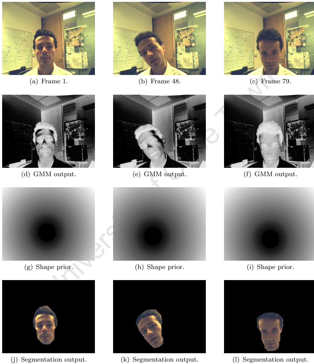
FIGURE 5.13: Video segmentation of ‘Antonio’ video sequence using shape priors. The first row contains the original frames (a-c). The output of the GMMs (d-f) are shown in the second row. The distance transform from the aligned shape priors (g-i) is shown in the third row. The segmentations using shape priors (j-l) are shown in the final row.
