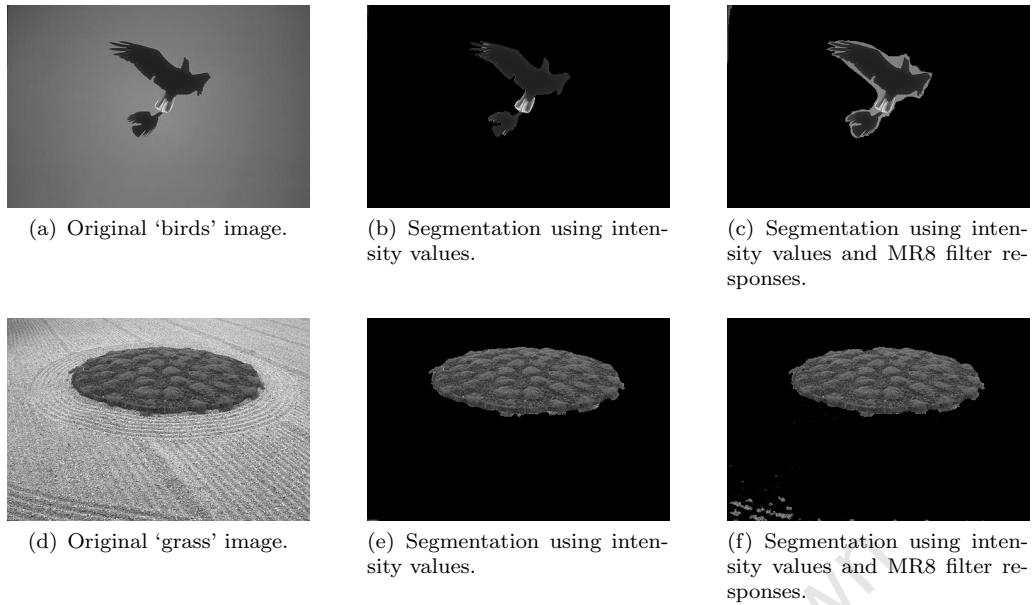
FIGURE 4.12: Segmentations based on different region costs. Boundary costs are kept constant and are calculated using gradient-based methods. (a) Original 'birds' image is segmented using (b) intensity values only and (c) intensity values and MR8 filter responses. (d) Original 'grass' image is segmented using (e) intensity values only and (f) intensity values and MR8 filter responses.
