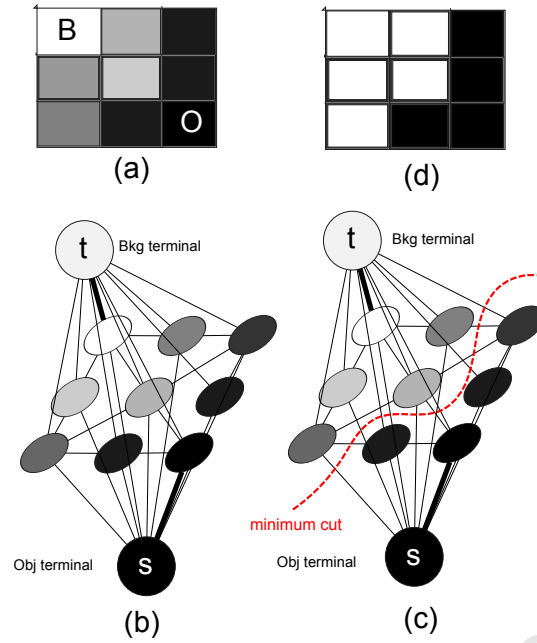
FIGURE 2.6: A simple 2D segmentation of 3 \times 3 image. In (a) the top left pixel and bottom right pixel are seeds for background and object respectively. The cost is reflected by the edge thickness. The region cost and hard constraints define t-weights. The boundary cost defines n-weights [2]. The dotted red line in (c) represents the minimum cut and the resulting segmentation is shown in (d).
