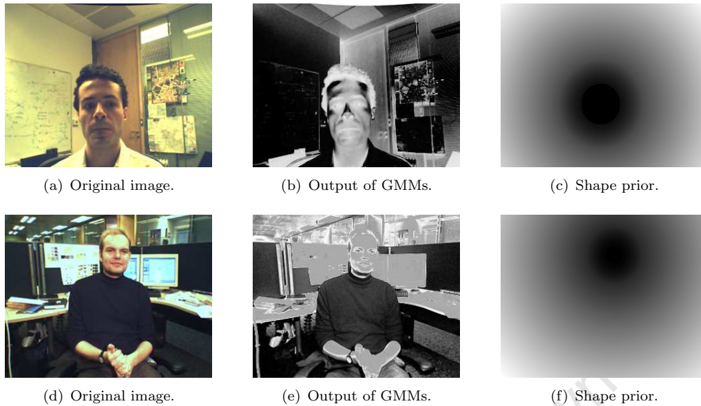
FIGURE 4.20: Image segmentation using shape priors and graph cuts. The figure shows (a) and (d) the original images, (b) and (e) probability estimation using GMMs, (c) and (f) distance transform from the shape prior aligned using Powell's method.
