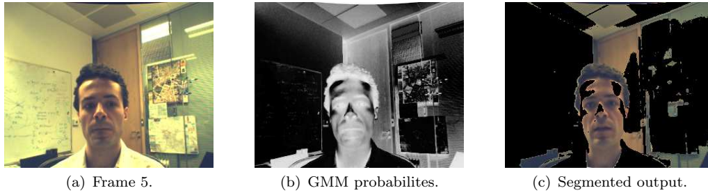
FIGURE 5.12: Segmentation without shape priors of the ‘Antonio’ video sequence. The original frame (a) is segmented using the logarithmic likelihood ratio derived from the GMM probabilities in (b) and motion information shown in Figure 5.11. The output of the 3D graph cut is shown in (c).
