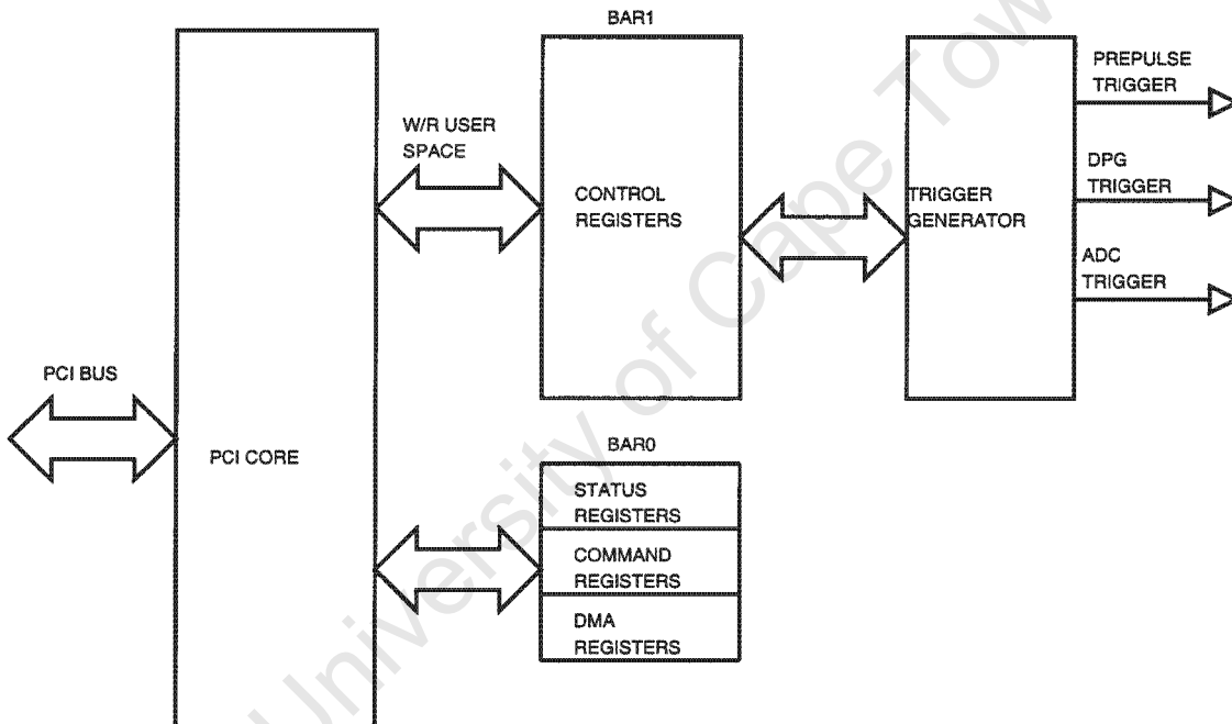
Figure 6.5: PM440 Firmware
