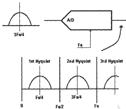
Figure 2.5: Direct IF Sampling
