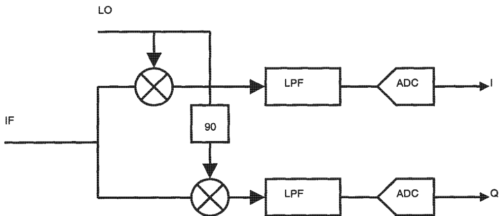
Figure 2.4: Direct Conversion
