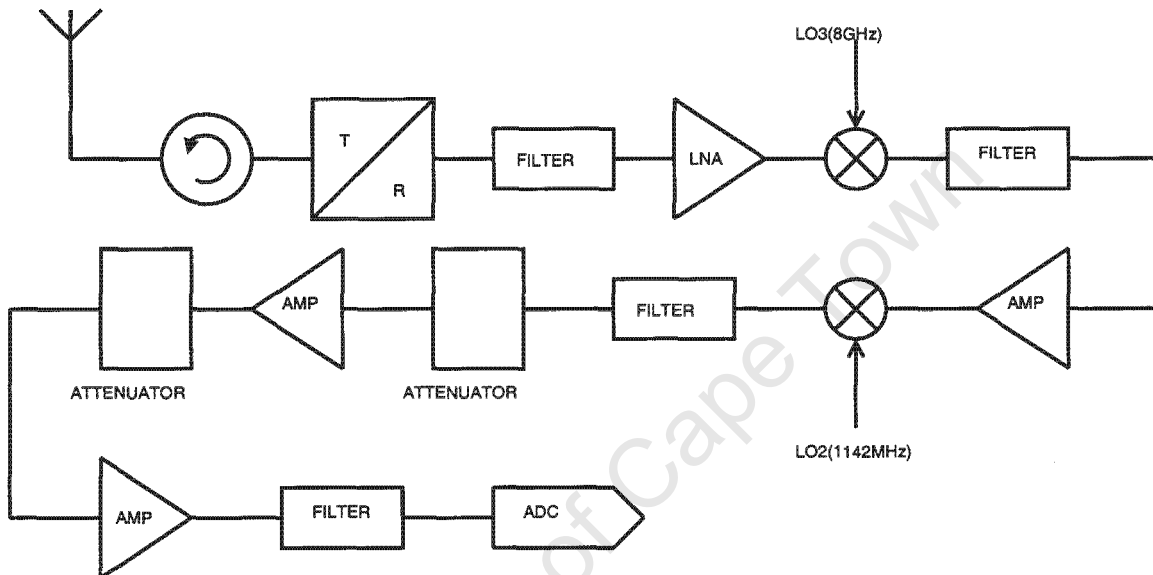
Figure 3.3: Receiver Architecture [8]
