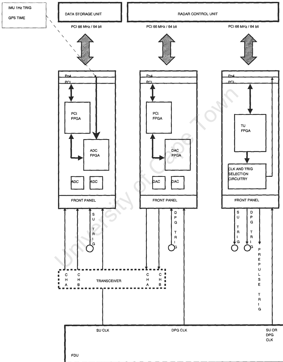
Figure 5.4: RDU System
