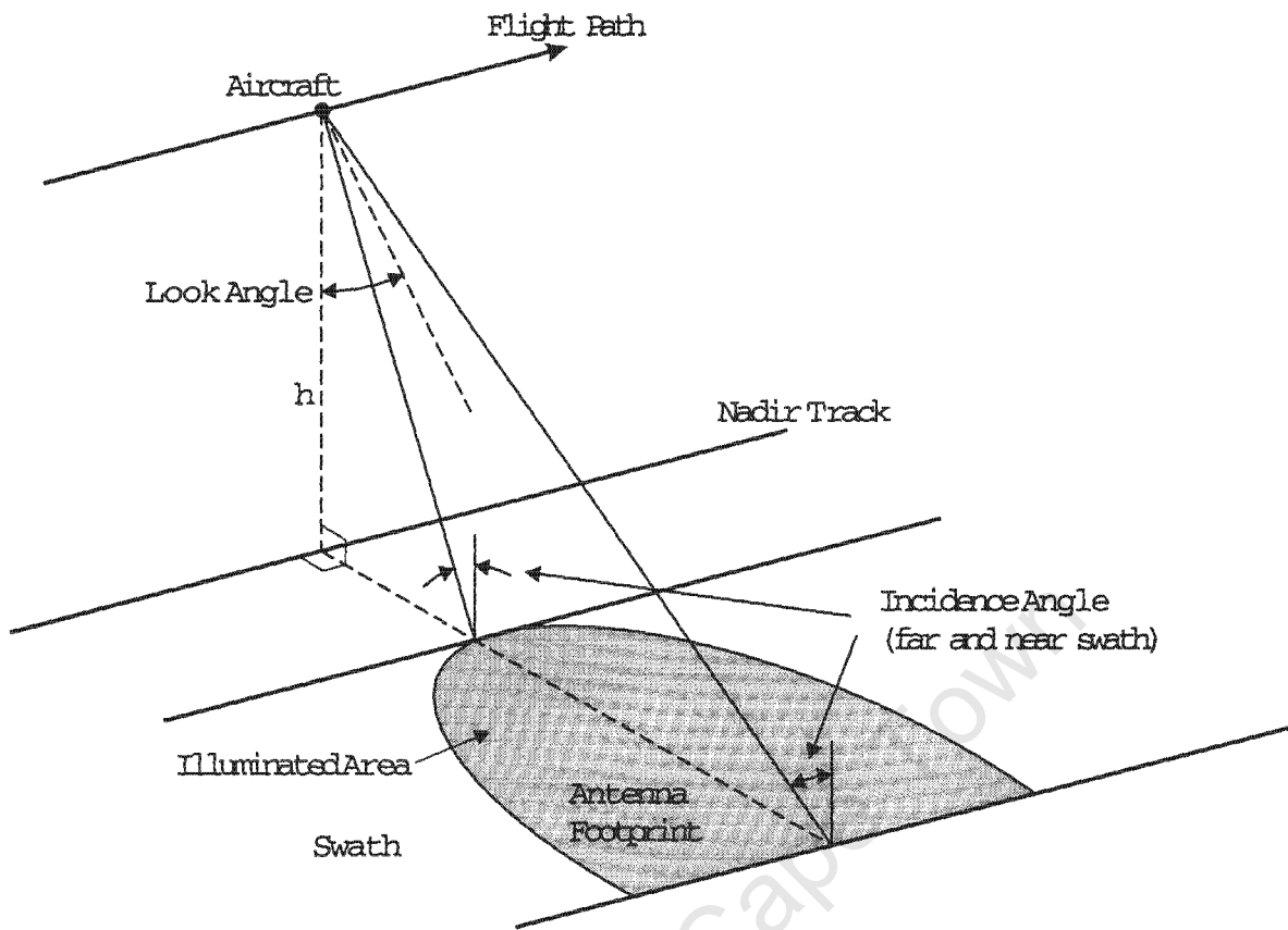
Figure 2.1: Synthetic Aperture Radar Geometry
