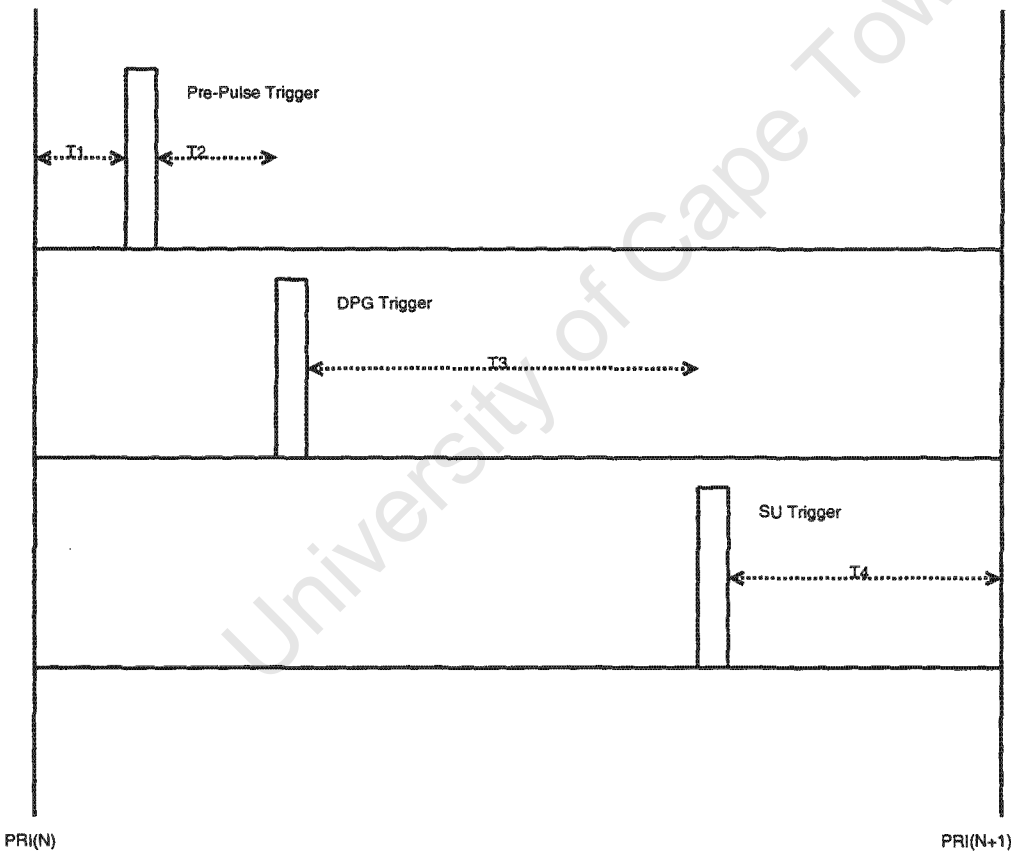
Figure 4.3: Trigger Timing
