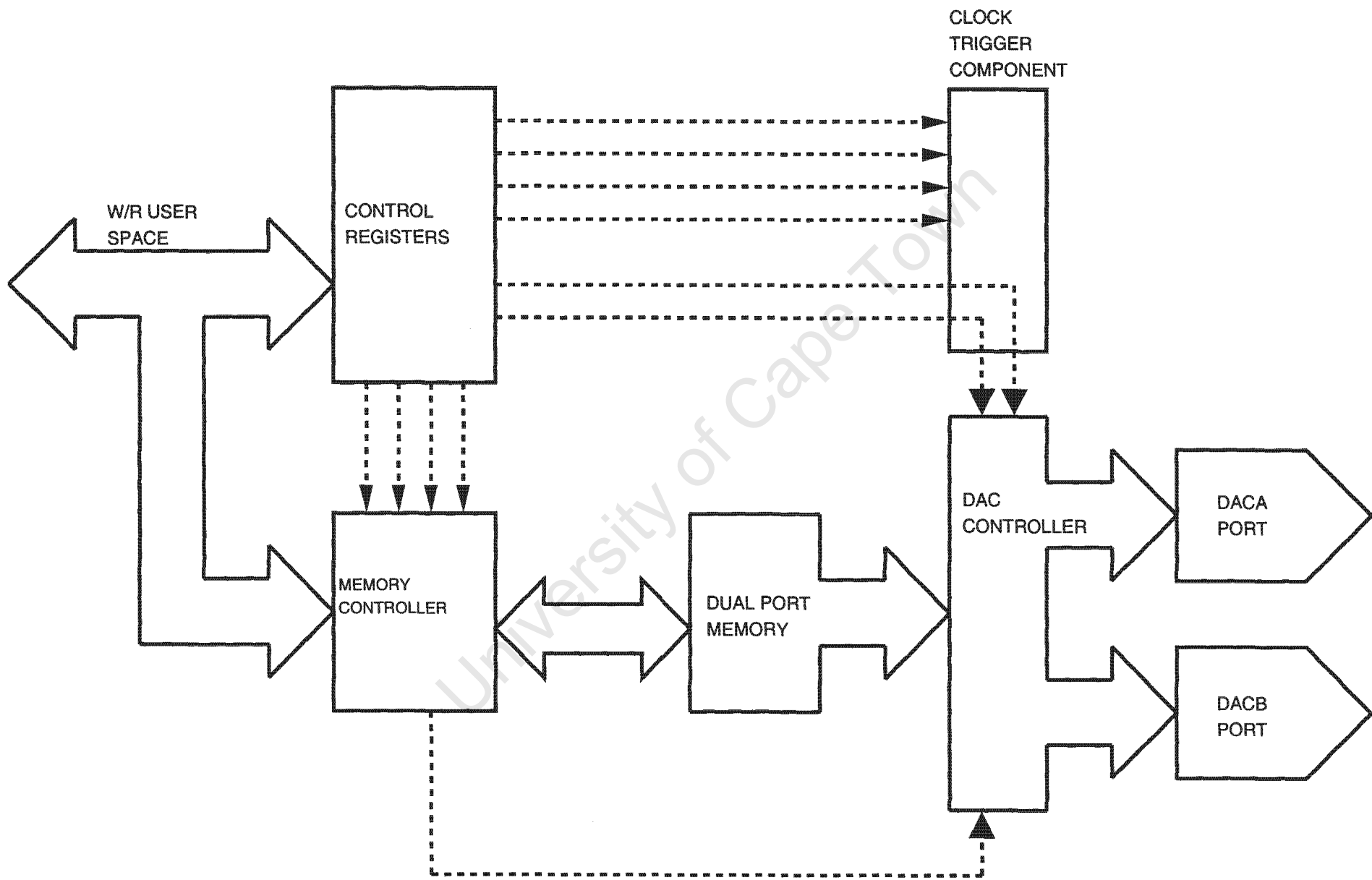
Figure 6.2: PM488 DAC FPGA Firmware
