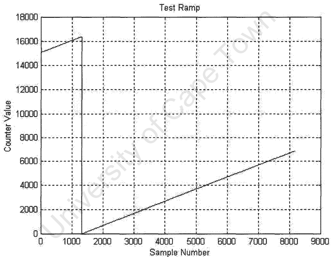
Figure 7.1: Test Ramp
