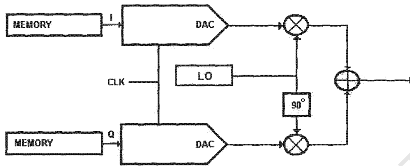
Figure 5.1: Digital Pulse Generator and IQ Modulation
