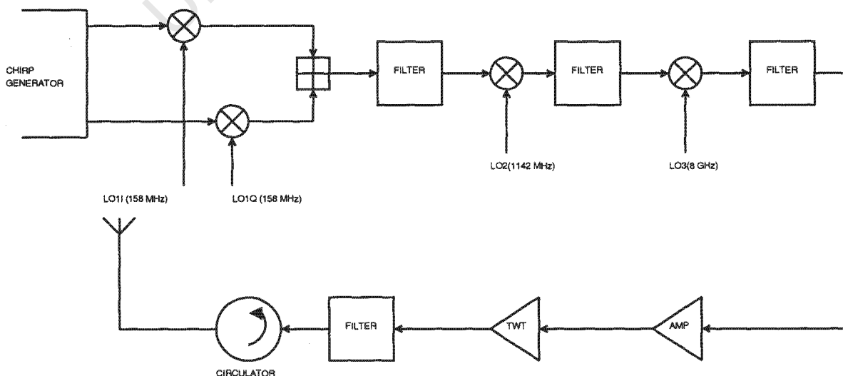
Figure 3.2: Transmitter Architecture [7]
