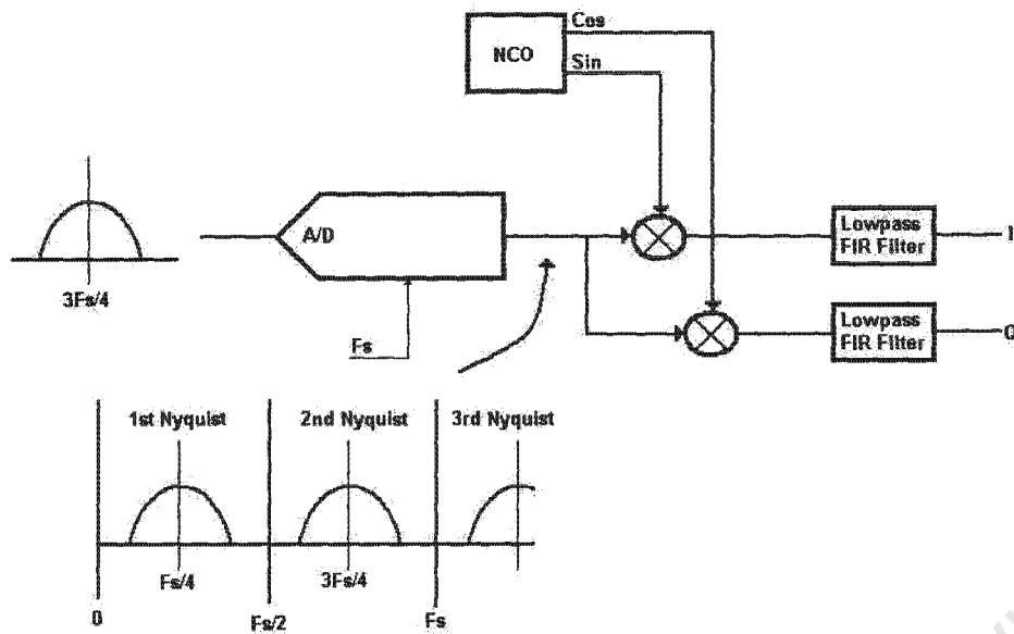
Figure 4.4: Digital Downconversion
