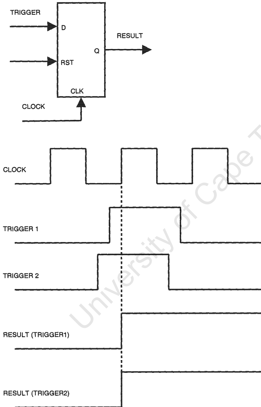
Figure 4.1: Trigger Detection
