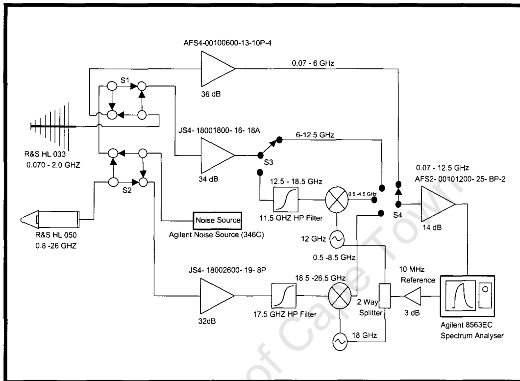
Figure 4.3: Block Diagram of RFI System 2 (from[17])
