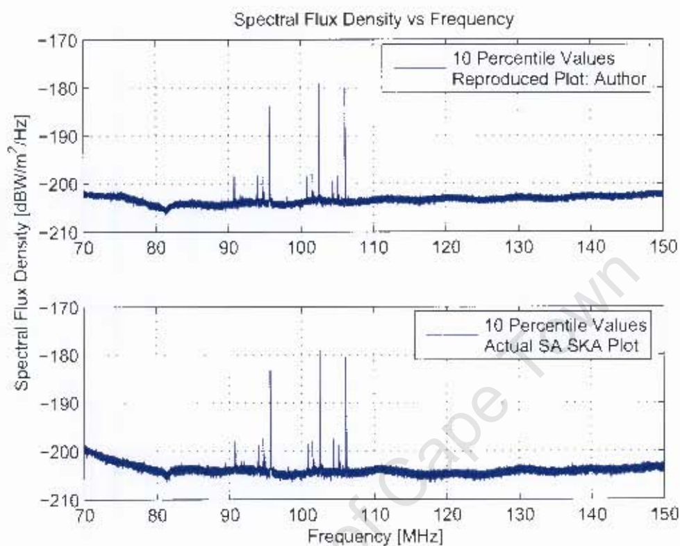
Figure 5.5: Plot of Frequency versus Spectral Flux Density. Top graph shows the re-processed plot as performed by the author whilst the bottom shows a plot derived by the SA SKA team. The plots were constructed using the ten percentile spectral flux density values .
