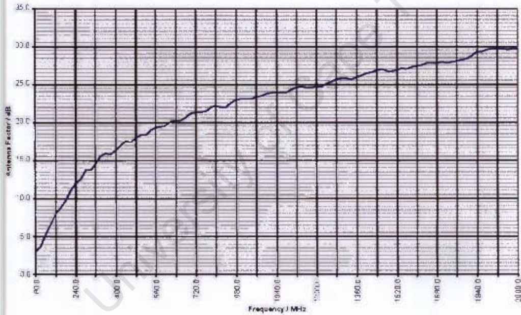
Figure D.1: Antenna Factor values of the R&S HL033 Log. Periodic Broadband
