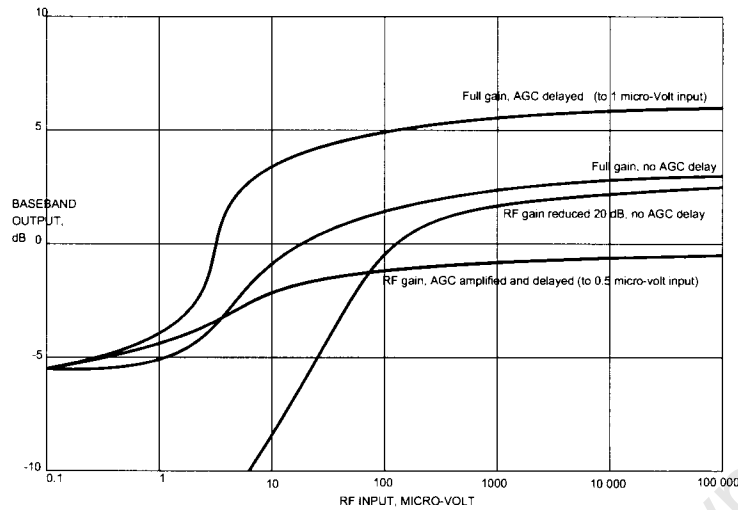
Figure 3.4: Representative input-output AGC curves (from [30])
