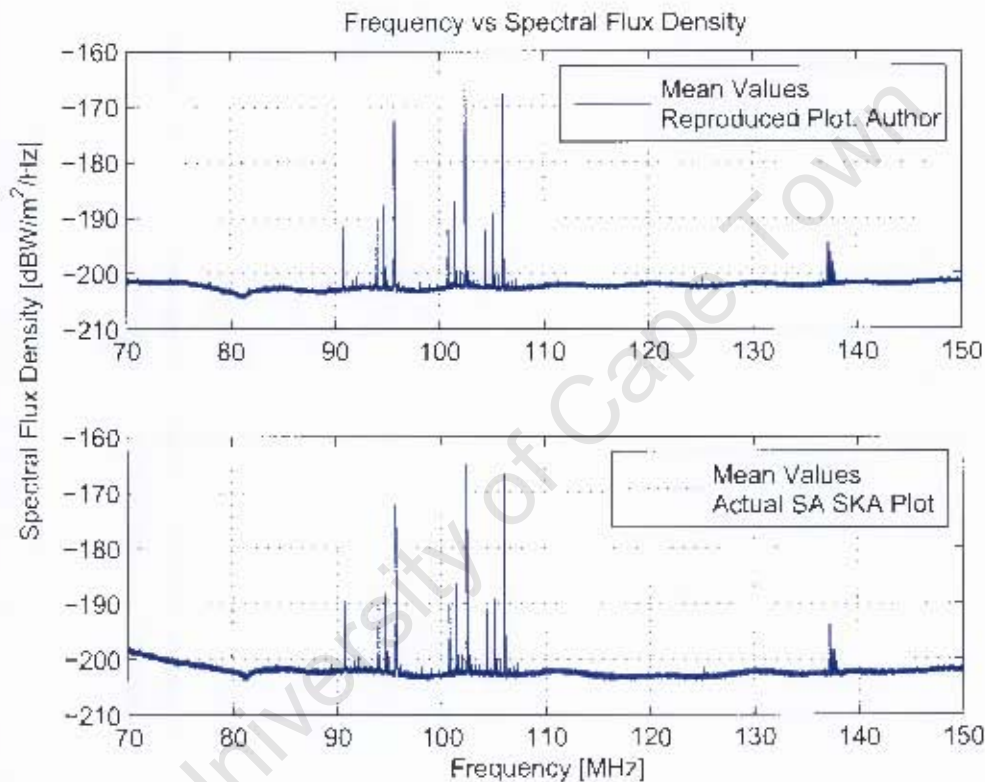
Figure 5.6: Plot of Frequency versus Spectral Flux Density. Top graph shows the reprocessed plot as performed by the author whilst the bottom shows a plot derived by the SA SKA team. The plots were constructed using the mean spectral flux density values . The two plots show maximum values of -166.4 \text{ dBW/m}^2/\text{Hz} at a frequency of 102.5 MHz and -164.8 \text{ dBW/m}^2/\text{Hz} .
