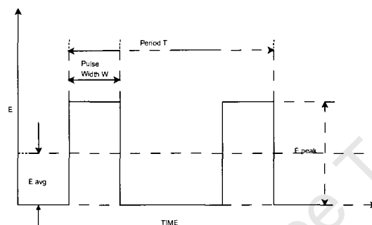
Figure 2.1: Basic Characteristics of a pulsed waveform showing the Marks and Spaces. The space gives the receiver a false sense of pulse inactivity which is not necessary the case.
