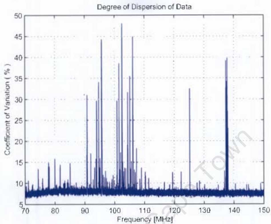
Figure 5.2: Plot of Coefficient of Variation (%) versus Frequency (MHz)
