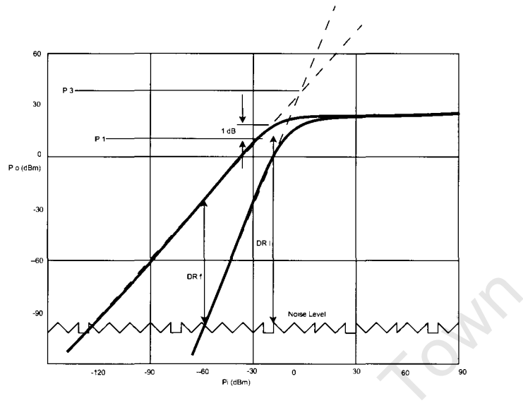
Figure 3.2: Illustration of linear dynamic and spurious free dynamic range (from[18])
