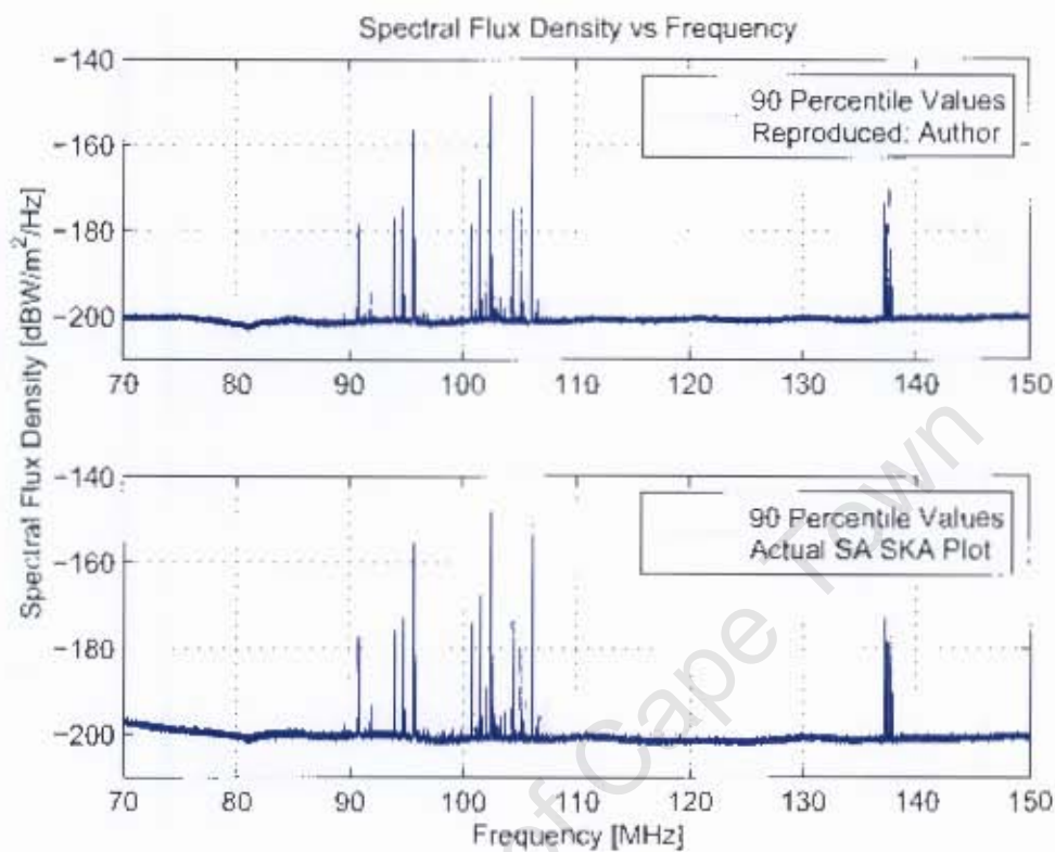
Figure 5.8: Plots of Frequency versus Spectral Flux Density. Top graph shows the reprocessed plot as performed by the author whilst the bottom shows a plot derived by the SA SKA team. The plots were constructed using the 90 Percentile spectral flux density values.
