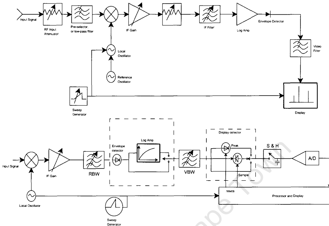
Figure 3.5: Block diagrams of a classic superheterodyne spectrum analyzer (from[22, 40])
