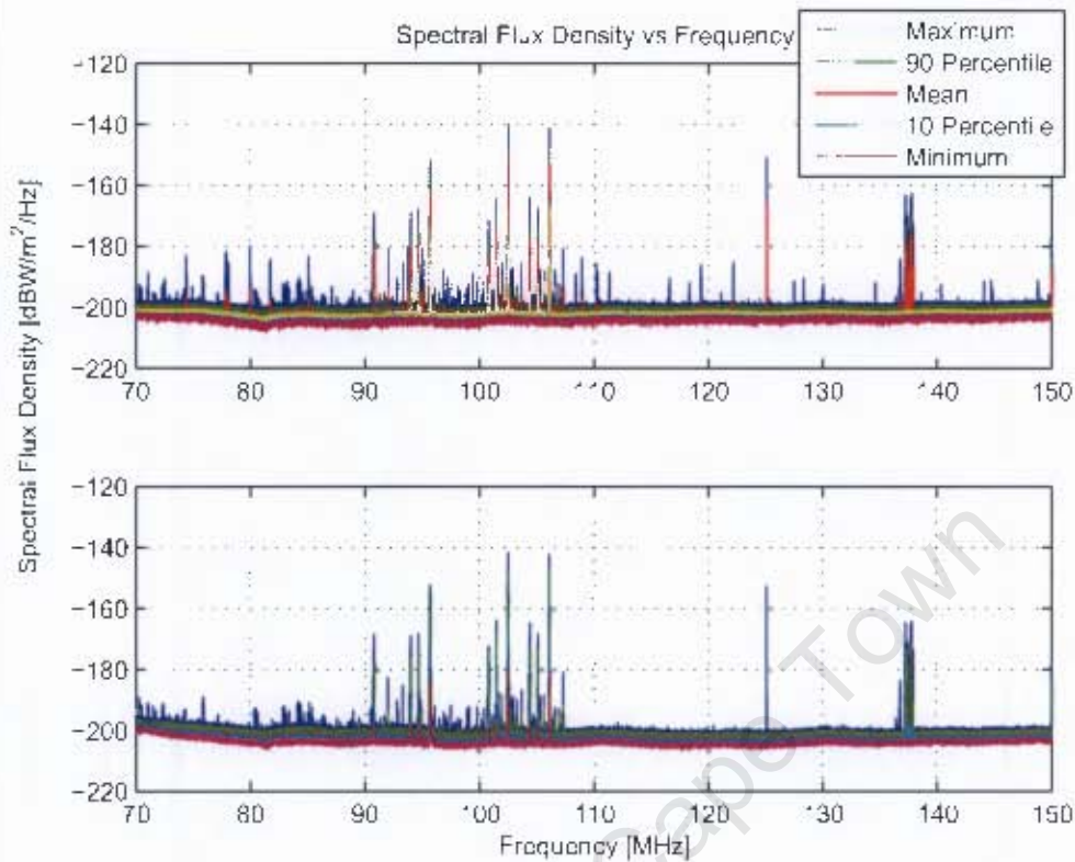
Figure 1.3: Radio Frequency Interference plot for the 70 - 150 MHz band: OPTION 3-(Top) Simulation (Bottom) SA SKA Measurement
