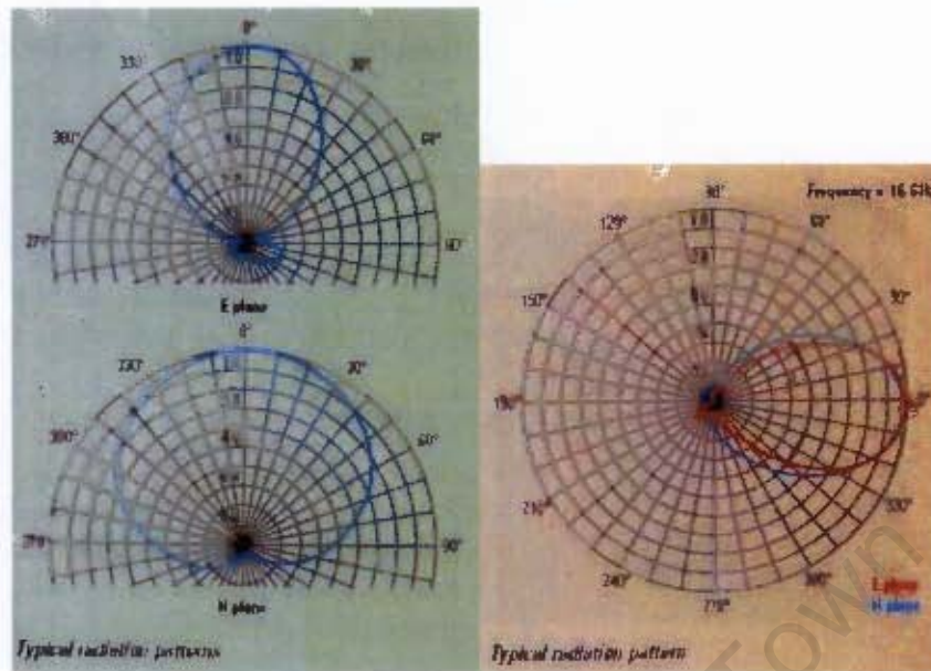
Figure 4.2: Radiation beam patterns of R&S HL 033 (left)[53] and R&S HL 050 (right) [54] antennas
