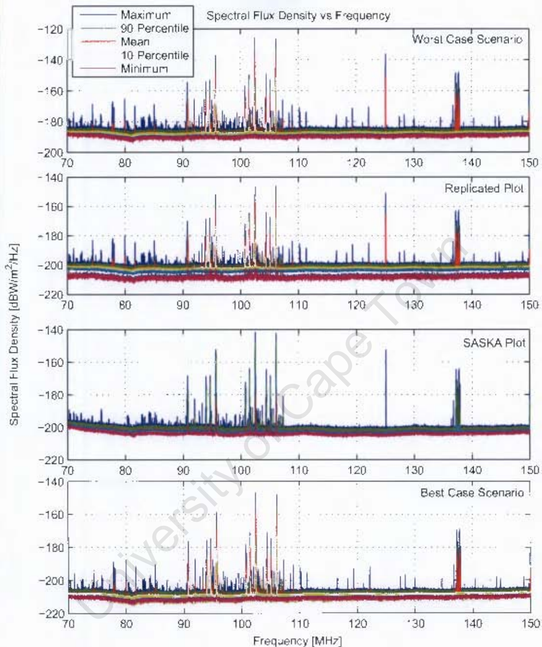
Figure 5.10: The above plots shows the spectral flux density as a function of RBW frequency. The top most plot shows the spectral flux density as function of frequency for a worst case scenario . This is when the positive tolerances of the components are taken into account and this reduces the theoretical system gain. The best case scenario is when the system gain is increased by subtracting the tolerances. The second to last plot depicts the plot as generated by SA SKA whereas the second plot from the top is an attempt to replicate the SA SKA plot.
