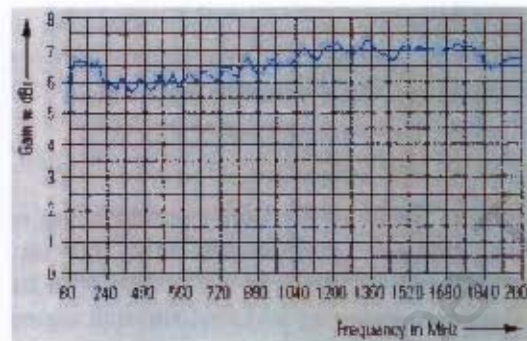
Figure 5.1: Gain vs Frequency (from[53])
