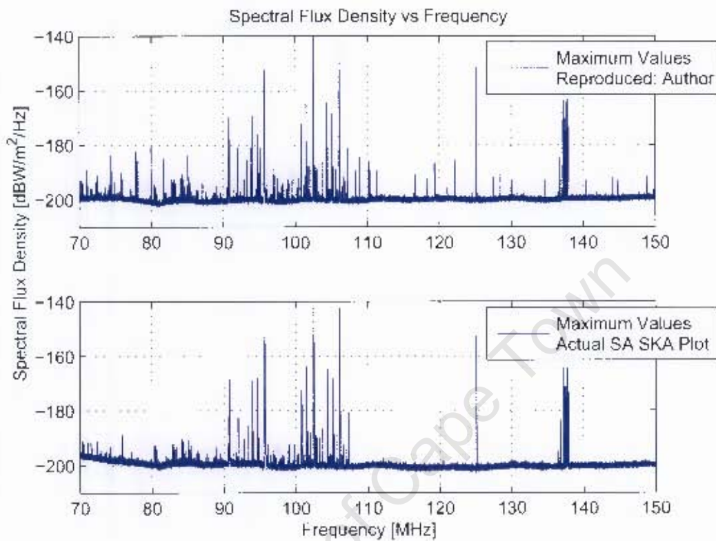
Figure 5.9: Plot of Frequency versus Spectral Flux Density. Top graph shows the reprocessed plot as performed by the author whilst the bottom shows a plot derived by the SA SKA team. The plots were derived using the maximum spectral flux density values .
