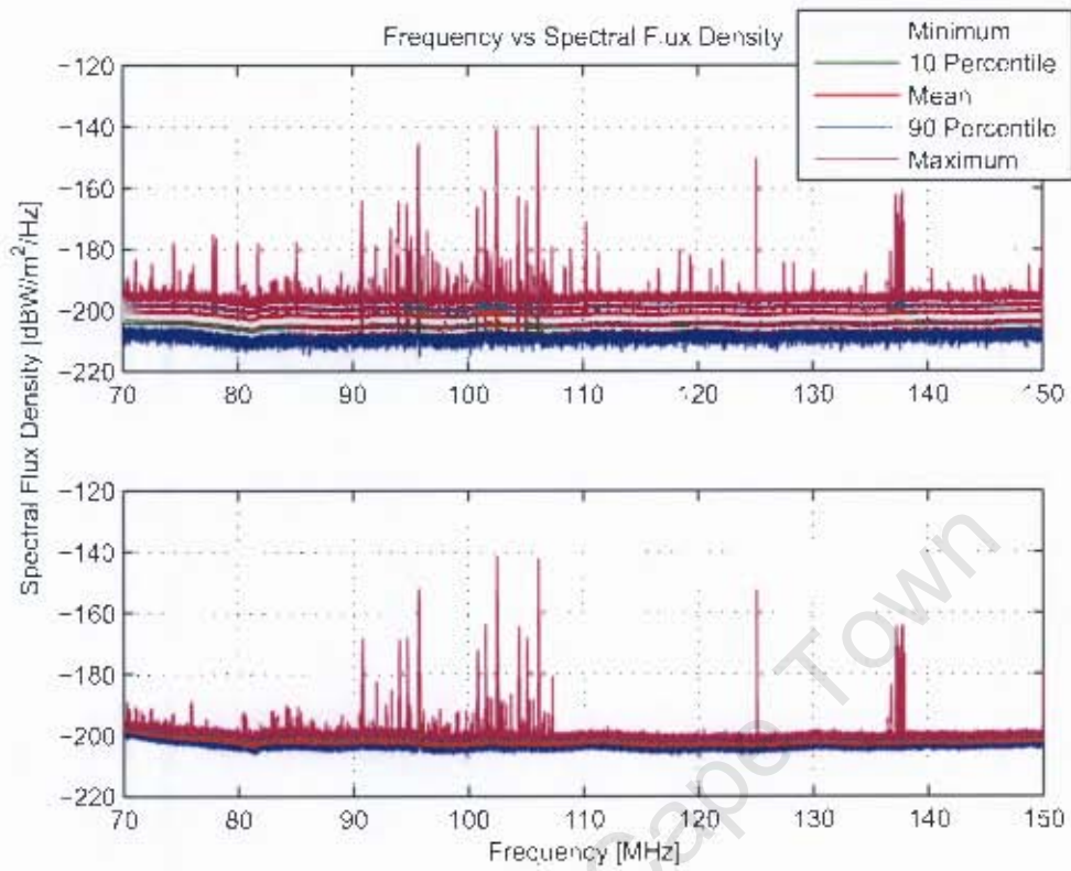
Figure 1.2: Radio Frequency Interference plot for the 70 - 150 MHz band: OPTION 2-(Top) Reprocessed (Bottom) SA SKA Measurement
