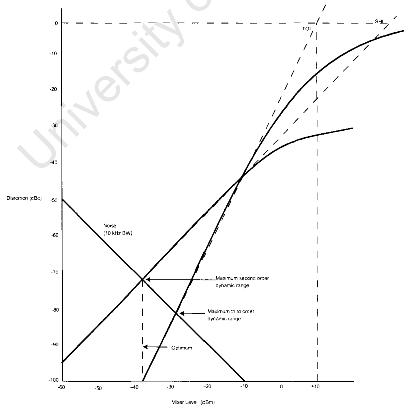
Figure 3.3: Dynamic range versus distortion and noise (from[22])
