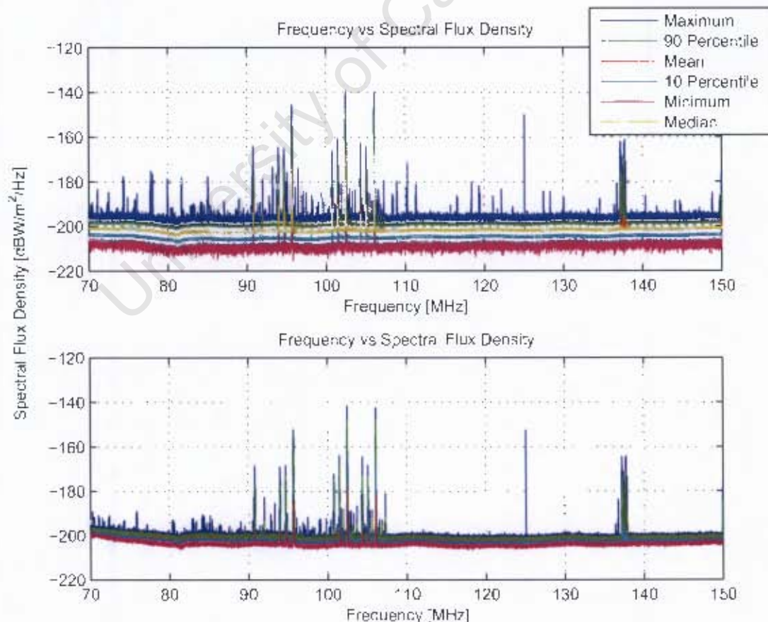
Figure 1.1: Radio Frequency Interference plot for the 70 - 150 MHz band: OPTION 1- (Top) Reprocessed (Bottom) SA SKA Measurement. It can be seen (through direct observation) that the (Top) plot has more spectral activity than the (Bottom) Plot.
