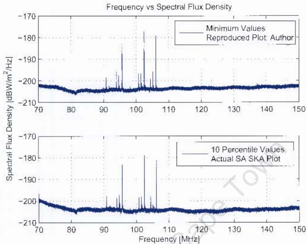
Figure 5.4: Plot of Frequency versus Spectral Flux Density. The plots were derived using the minimum spectral flux density values and 10 percentile SFD values . Top graph shows the reprocessed plot as performed by the author whilst the bottom shows a plot derived by the SA SKA team . The correlation between the two curves is 0.3218.
