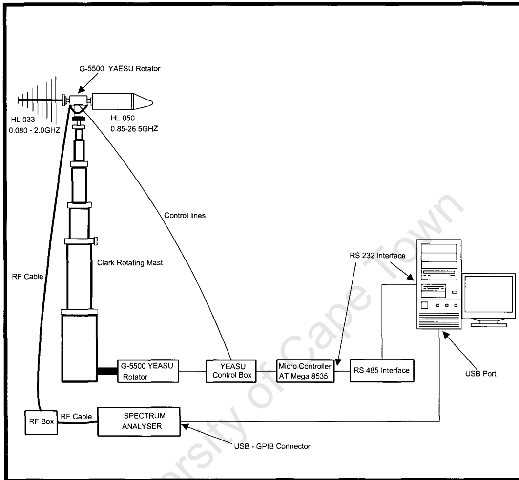
Figure 4.1: Block diagram showing the complete RFI Measurement System 2
