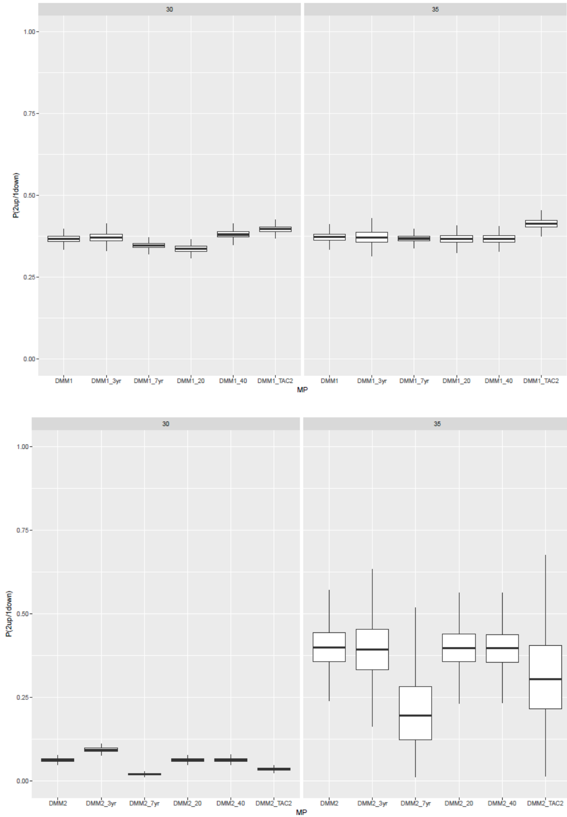
Figure 7. Probability ( TAC_{r+3} < TAC_{r+2n} ) if TAC_{r+2} > TAC_{r+1} and TAC_{r+1} > TAC_r , for the r^{\text{th}} TAC decision (default is currently r=1 ) for DMM1 and DMM2 and their sensitivity scenarios, tuned to 30% SSB_0 and 35% SSB_0 in the year 2035. Details of the sensitivity scenarios are the same as described in Table 1.
