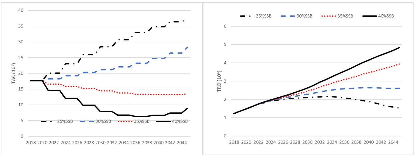
Figure 2. Median of TAC and TRO for DMM2 for the projection years when tuned to 25%, 30%, 35% and 40% SSB 0 in the year 2035.
