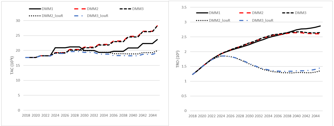
Figure 16. Plots of the medians for TAC and TRO for DMM1, DMM2, DMM3, DMM2_lowR and DMM3_lowR for the projection years when tuned to 30% SSB 0 in the year 2035.
