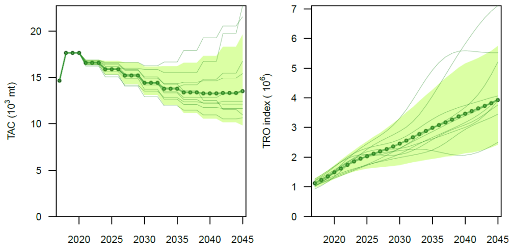
Figure 15. Worm plots for TAC and TRO for DMM1 and DMM2 for the projection years when tuned to 35% SSB 0 in the year 2035.
