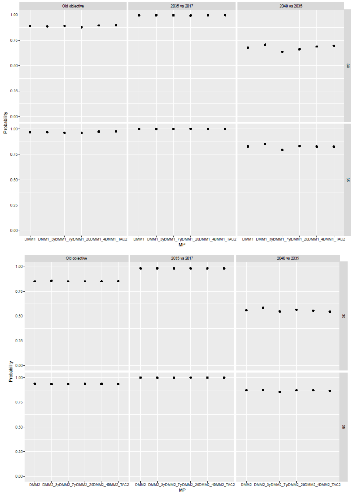
Figure 3. Plots showing the TRO statistics for DMM1 and DMM2 and their sensitivity scenarios, tuned to 30% SSB 0 and 35% SSB 0 in year 2035. Details of the sensitivity scenarios are the same as described in Table 1. The leftmost panel plots Probability ( TRO_{2035} > 0.2 TRO_0 ): the previous MP tuning objective; the middle panel plots Probability ( TRO_{2035} > TRO_{2017} ): the probability that the TRO in the tuning year is greater than the current level; and the rightmost panel plots Probability ( TRO_{2040} > TRO_{2035} ): the probability that the TRO five years after the tuning year is above that in the tuning year, to identify MPs which increase the TAC too high/fast when attaining the tuning objective and cause a future “undershoot”.
