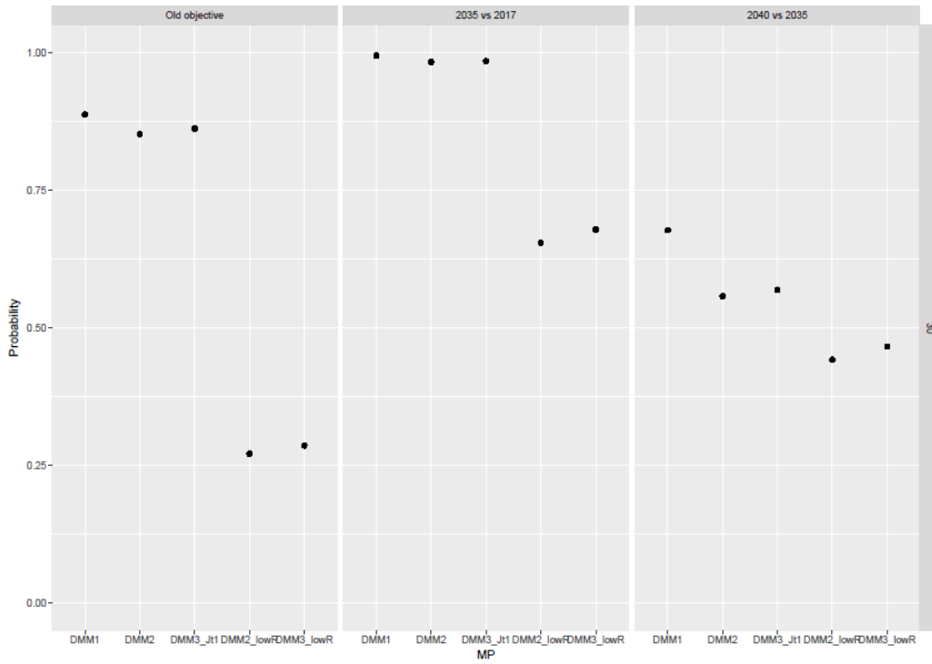
Figure 8. Plots showing the TRO statistics for DMM1, DMM2, DMM3, DMM2_lowR and DMM3_lowR tuned to 30% SSB_0 in year 2035. The leftmost panel plots Probability ( TRO_{2035} > 0.2 TRO_0 ): the previous MP tuning objective; the middle panel plots Probability ( TRO_{2035} > TRO_{2017} ): the probability that the TRO in the tuning year is greater than the current level; and the rightmost panel plots Probability ( TRO_{2040} > TRO_{2035} ): the probability that the TRO five years after the tuning year is above that in the tuning year, to identify MPs which increase the TAC too high/fast when attaining the tuning objective and cause a future “undershoot”.
