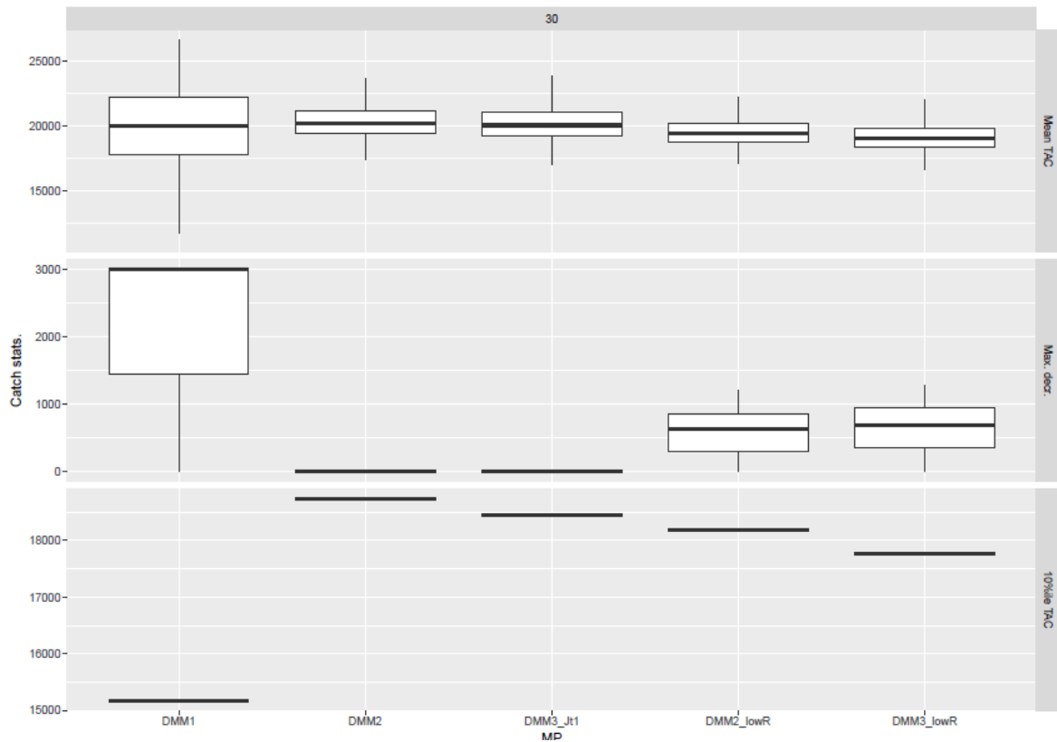
Figure 10. Plots of the summary statistics for TACs for DMM1, DMM2, DMM3, DMM2_lowR and DMM3_lowR tuned to 30% SSB 0 . “Mean TAC “ is calculated for the years from 2021 to 2035. “Max. decr.” is the maximum TAC decrease from 2021 to 2035. “10%ile TAC” is mean (averaged over years and from 2021 to 2035) of the lower 10%ile in the TAC.
