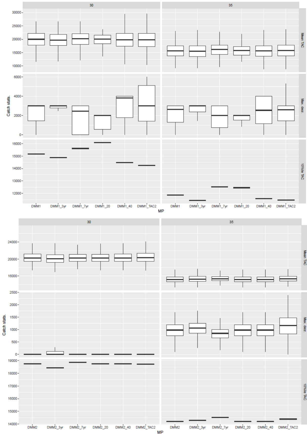
Figure 5. Plots of the summary statistics for TACs for DMM1 and DMM2 and their sensitivity scenarios, tuned to 30% SSB_0 and 35% SSB_0 in the 2035. Details of the sensitivity scenarios are the same as described in Table 1. “Mean TAC “ is calculated for the years from 2021 to 2035. “Max. decr.” is the maximum TAC decrease from 2021 to 2035. “10%ile TAC” is mean (averaged over years and from 2021 to 2035) of the lower 10%ile in the TAC.
