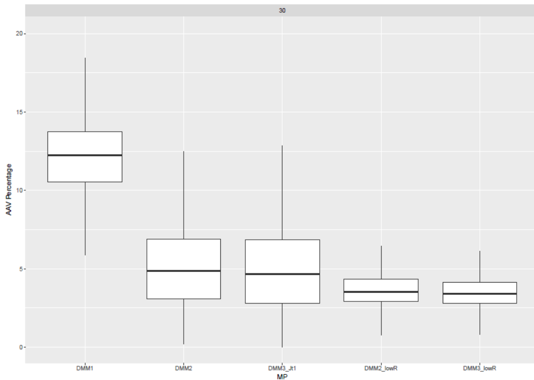
Figure 11. Plots of AAV (%) from 2021 to 2035 for DMM1, DMM2, DMM3, DMM2_lowR and DMM3_lowR tuned to 30% SSB 0 .
