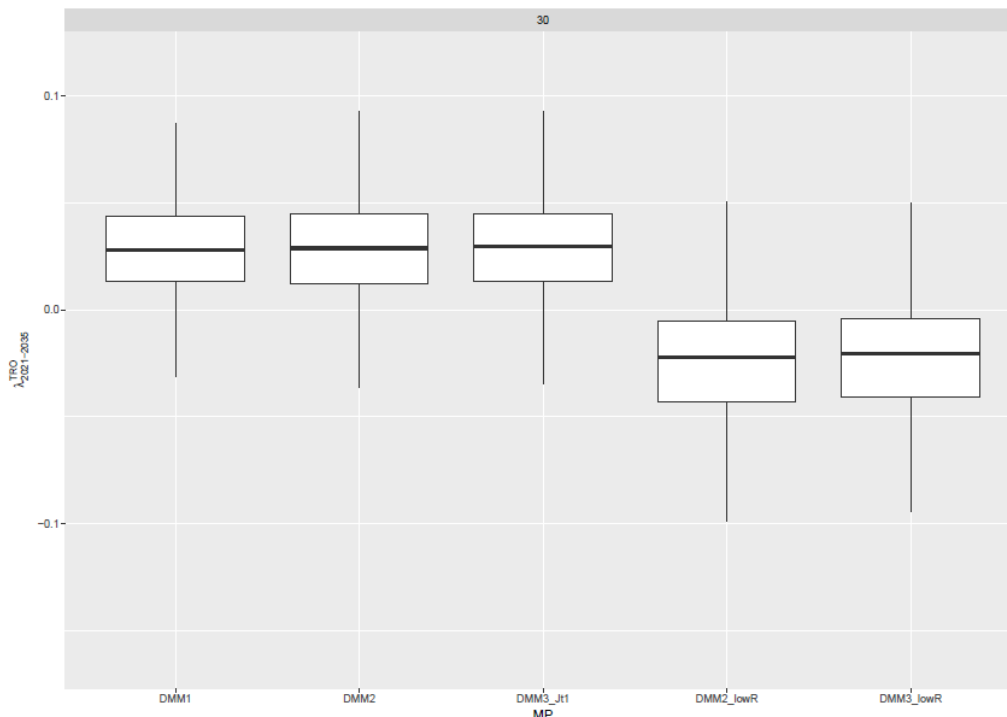
Figure 9. Log-linear trends in TRO from 2021 to 2035 for DMM1, DMM2, DMM3, DMM2_lowR and DMM3_lowR tuned to 30% SSB_0 .
