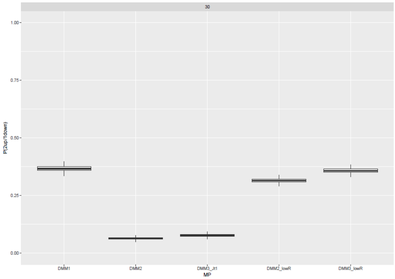
Figure 12. Probability ( TAC_{r+3} < TAC_{r+2n} ) if TAC_{r+2} > TAC_{r+1} and TAC_{r+1} > TAC_r , for the r^{\text{th}} TAC decision (default is currently r=1 ) for DMM1, DMM2, DMM3, DMM2_lowR and DMM3_lowR tuned to 30% SSB_0 in the year 2035.
