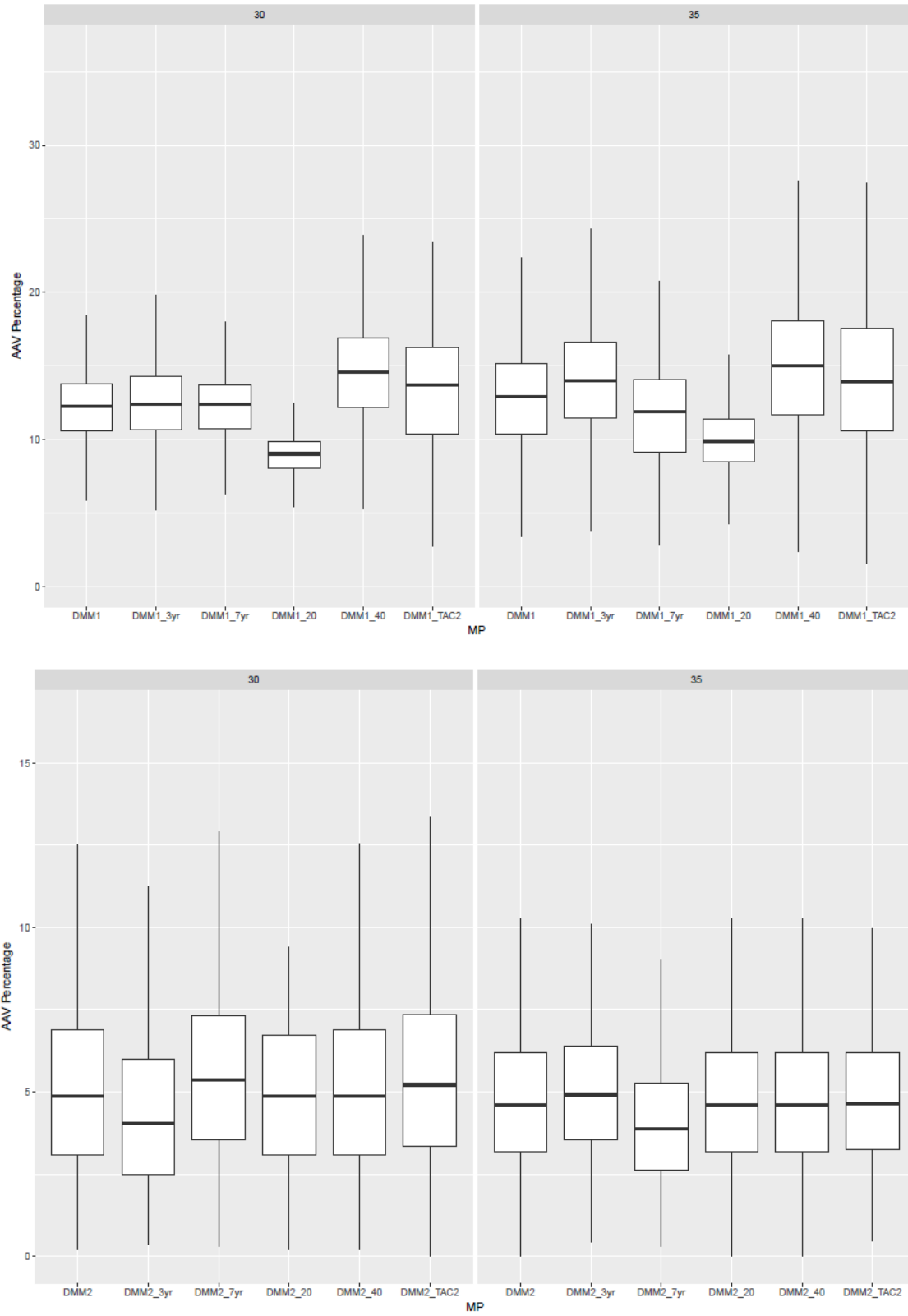
Figure 6. Plots of AAV (%) from 2021 to 2035 for DMM1 and DMM2 and their sensitivity scenarios, tuned to 30% SSB 0 and 35% SSB 0 in year 2035. Details of the sensitivity scenarios are the same as described in Table 1.
