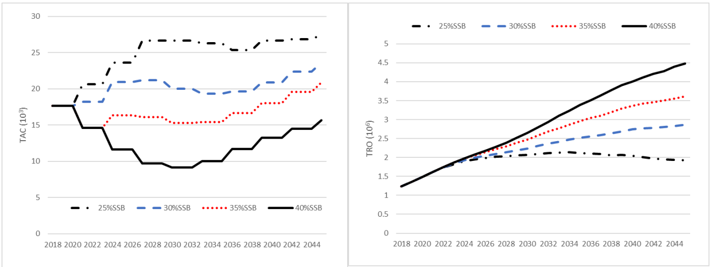
Figure 1. Median of TAC and TRO for DMM1 for the projection years when tuned to 25%, 30%, 35% and 40% SSB 0 in the year 2035.
