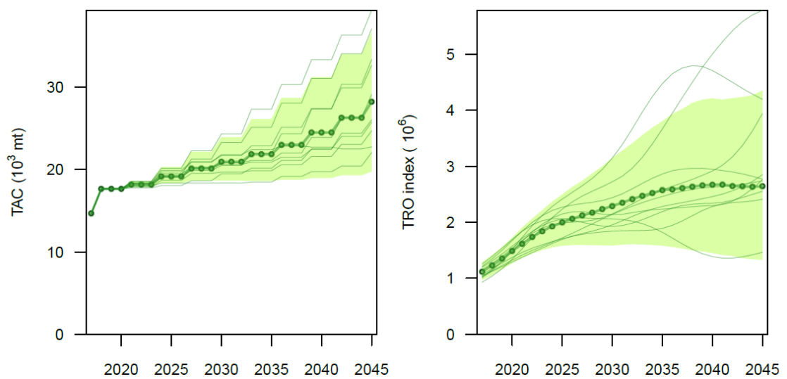
Figure 13. Worm plots for TAC and TRO for DMM1, DMM2 and DMM3 for the projection years when tuned to 30% SSB_0 in the year 2035.
