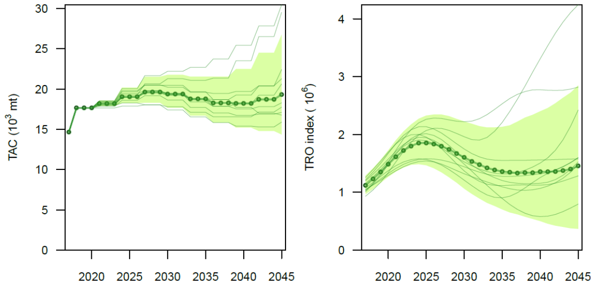
Figure 14. Worm plots for TAC and TRO for DMM3 (30% SSB 0 ) when applied for lowR ( n=10 ) case.
