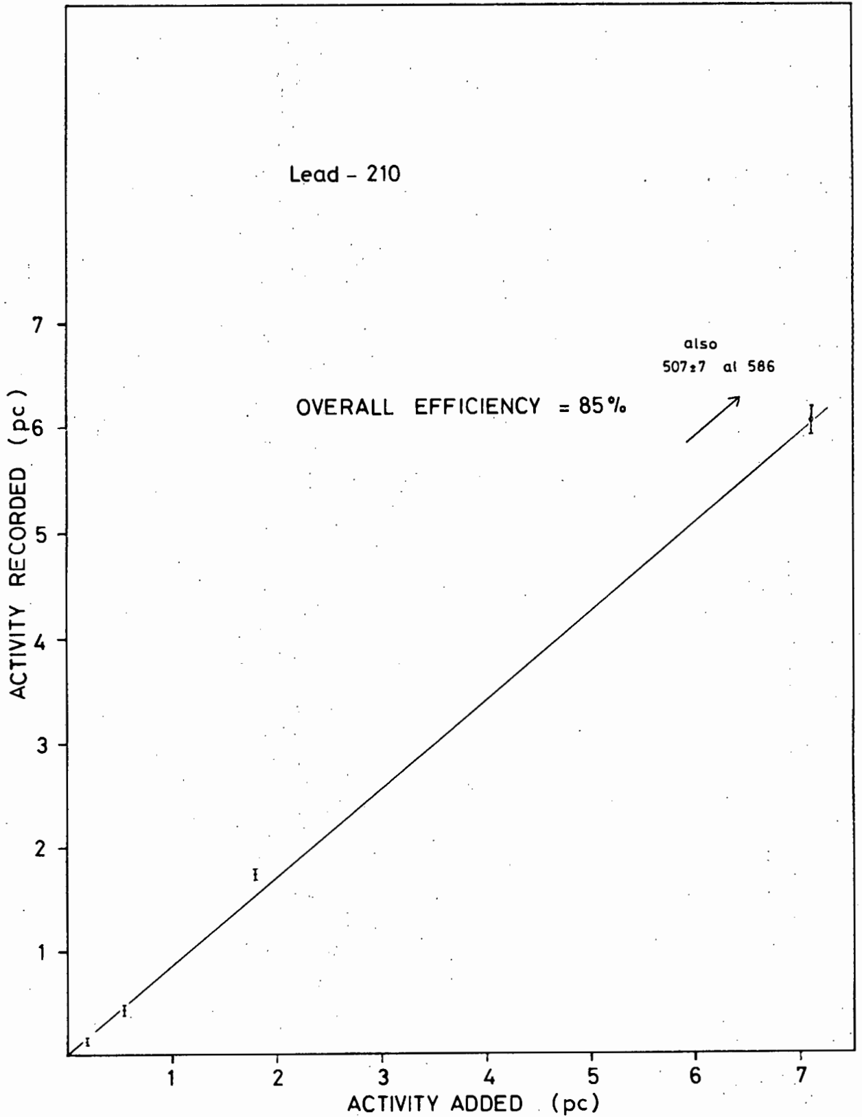
FIG.15 CALIBRATION CURVE — LEAD - 210
