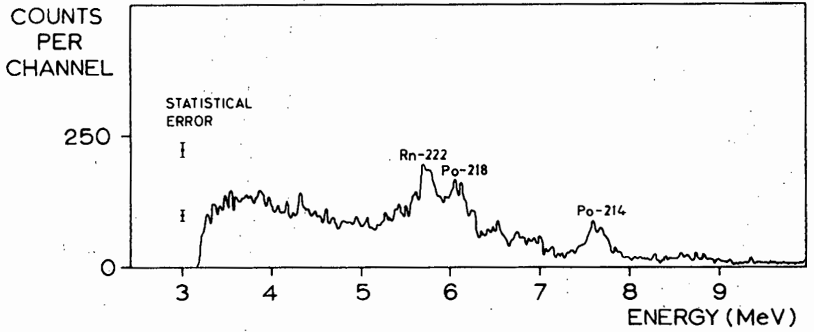
FIG. 5 ION CHAMBER - BACKGROUND BLANK RUN - 50 HRS.
