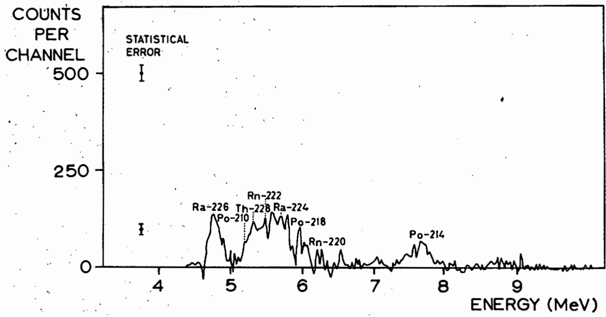
FIG. 12 ION CHAMBER ALPHA-SPECTRUM SAMPLE 212 -50 HRS.
