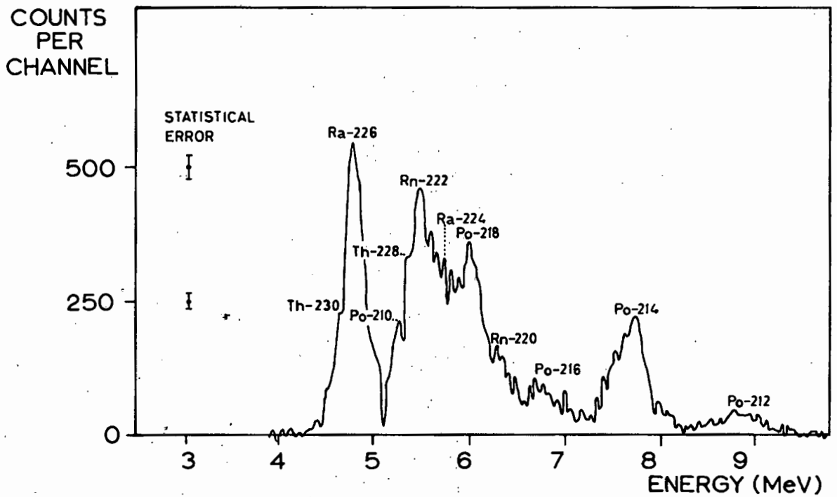
FIG. 9 ION CHAMBER ALPHA-SPECTRUM SAMPLE 214 -50 HRS.
