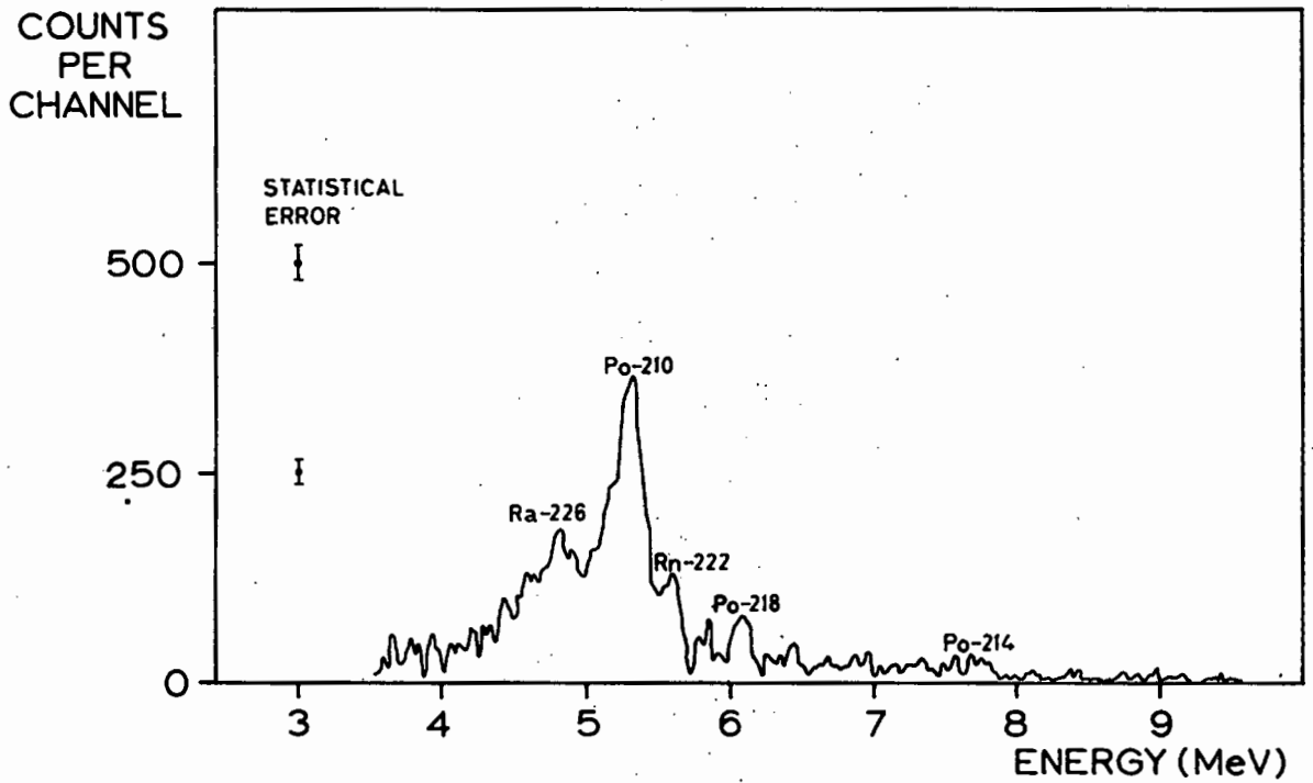
FIG. 8 ION CHAMBER ALPHA-SPECTRUM SAMPLE 16 -50 HRS.
