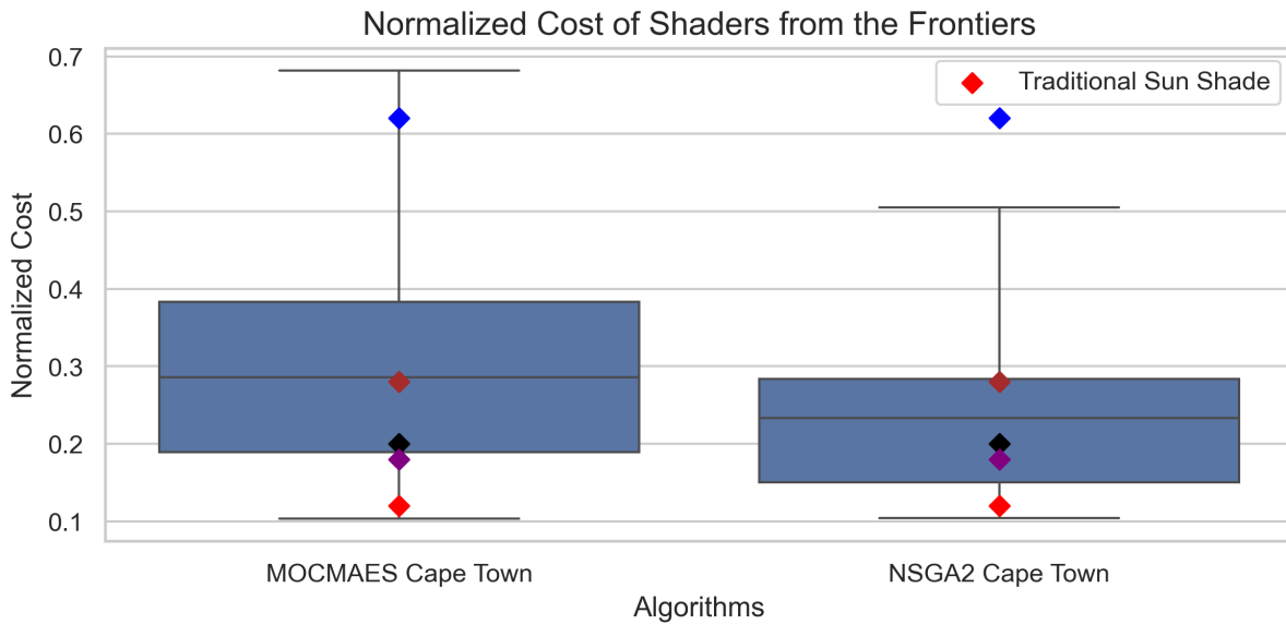
Figure 5.4: Box plots of the normalized cost frontier for Cape Town. Diamond shapes portray the performance of traditional sunshades (A, B, C, D, and E represent red, black, blue, purple, and brown, respectively 4.1). The left and right distributions correspond to MO-CMA-ES and NSGA-II results, respectively. Lower values indicate improved performance.
