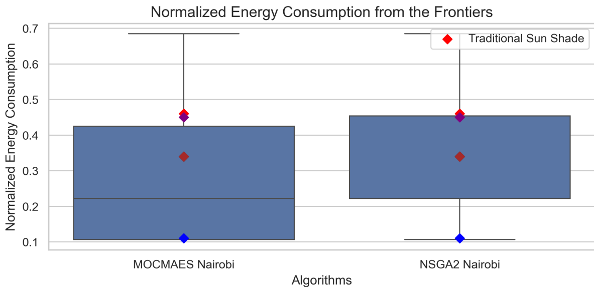
Figure 5.8: Box plots of the normalized energy consumption frontier for Nairobi. Diamond shapes portray the performance of traditional sunshades (A, B, C, D, and E represent red, black, blue, purple, and brown, respectively 4.1). The left and right distributions correspond to MO-CMA-ES and NSGA-II results, respectively. Lower values indicate improved performance.
