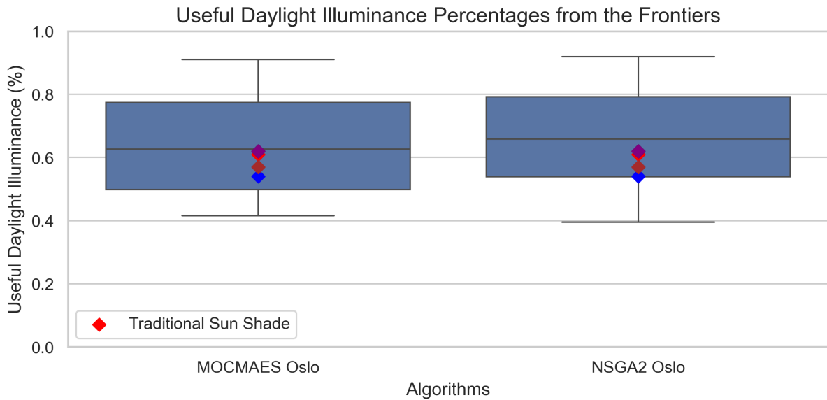
Figure 5.21: Box plots of the normalized UDI percentage frontier for Oslo. Diamond shapes portray the performance of traditional sunshades (A, B, C, D, and E represent red, black, blue, purple, and brown, respectively 4.1). The left and right distributions correspond to MO-CMA-ES and NSGA-II results, respectively. Higher values indicate improved performance.
