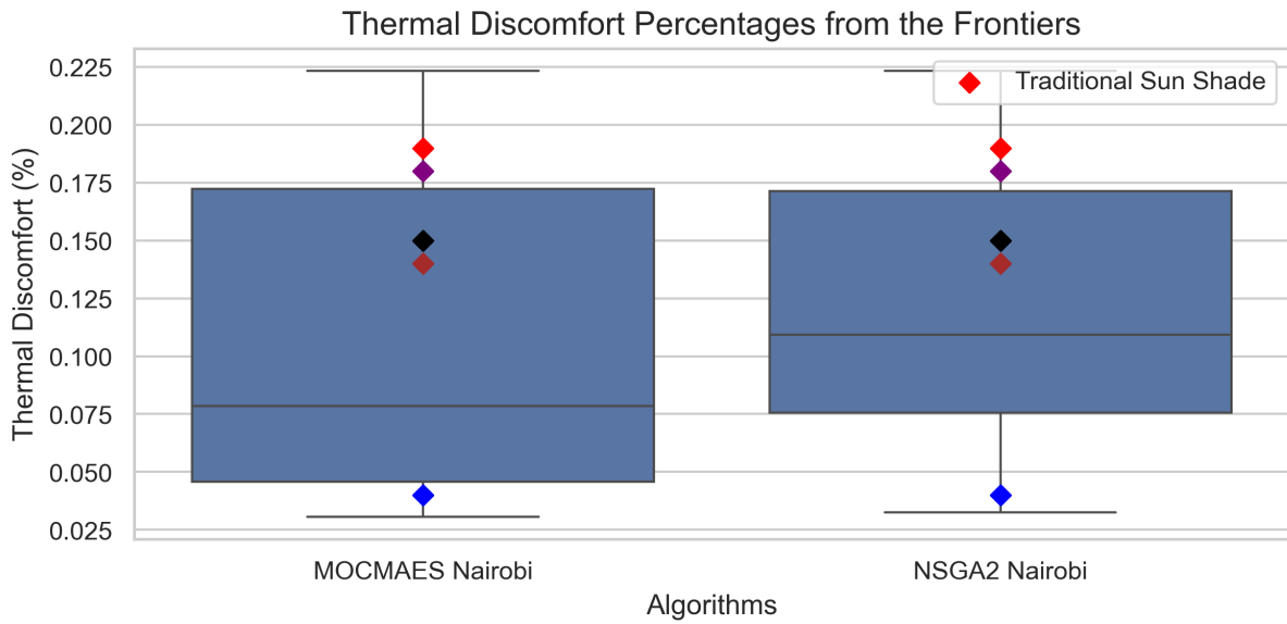
Figure 5.7: Box plots of the normalized thermal discomfort percentage frontier for Nairobi. Diamond shapes portray the performance of traditional sunshades (A, B, C, D, and E represent red, black, blue, purple, and brown, respectively 4.1). The left and right distributions correspond to MO-CMA-ES and NSGA-II results, respectively. Lower values indicate improved performance.
