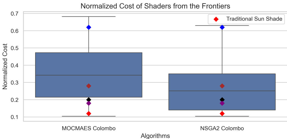
Figure 5.16: Box plots of the normalized cost frontier for Colombo. Diamond shapes portray the performance of traditional sunshades (A, B, C, D, and E represent red, black, blue, purple, and brown, respectively 4.1). The left and right distributions correspond to MO-CMA-ES and NSGA-II results, respectively. Lower values indicate improved performance.
