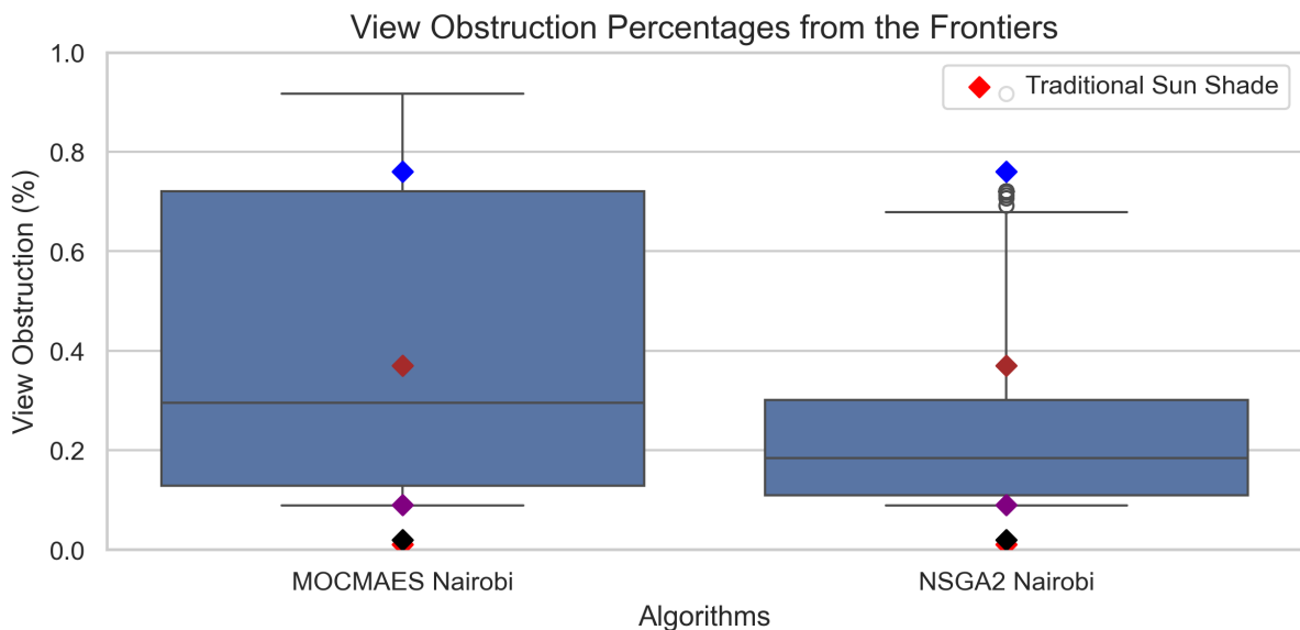
Figure 5.11: Box plots of the normalized window obstruction percentage frontier for Nairobi. Diamond shapes portray the performance of traditional sunshades (A, B, C, D, and E represent red, black, blue, purple, and brown, respectively 4.1). The left and right distributions correspond to MO-CMA-ES and NSGA-II results, respectively. Lower values indicate improved performance.
