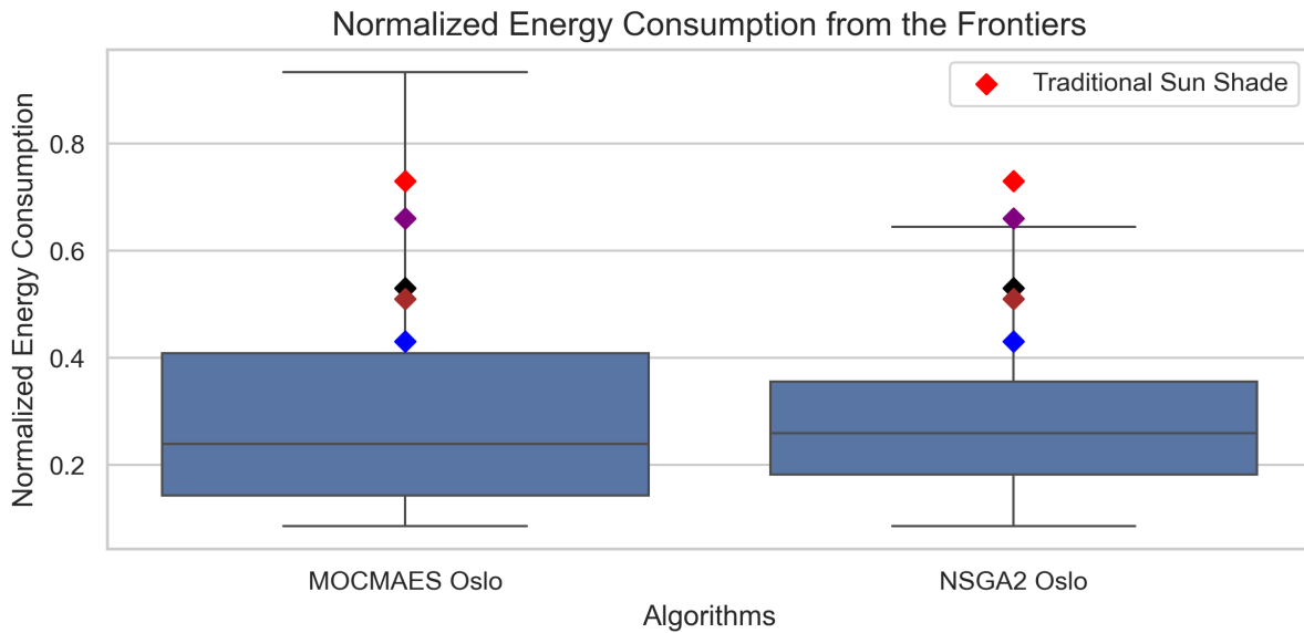
Figure 5.20: Box plots of the normalized energy consumption frontier for Oslo. Diamond shapes portray the performance of traditional sunshades (4.1). The left and right distributions correspond to MO-CMA-ES and NSGA-II results, respectively. Lower values indicate improved performance.
