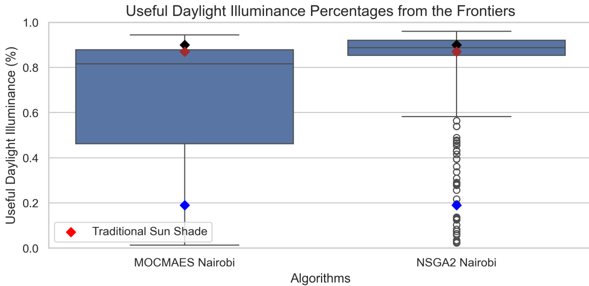
Figure 5.9: Box plots of the normalized UDI percentage frontier for Nairobi. Diamond shapes portray the performance of traditional sunshades (A, B, C, D, and E represent red, black, blue, purple, and brown, respectively 4.1). Some overlap made all five points not fully visible. The left and right distributions correspond to MO-CMA-ES and NSGA-II results, respectively. Higher values indicate improved performance.
