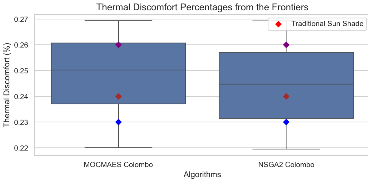
Figure 5.13: Box plots of the normalized thermal discomfort percentage frontier for Colombo. Diamond shapes portray the performance of traditional sunshades (A, B, C, D, and E represent red, black, blue, purple, and brown, respectively 4.1). Some overlap made all five points not fully visible. The left and right distributions correspond to MO-CMA-ES and NSGA-II results, respectively. Lower values indicate improved performance.
