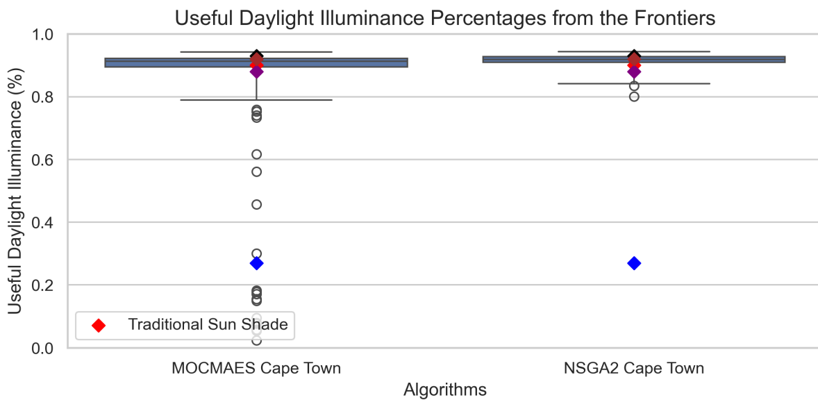
Figure 5.3: Box plots of the normalized UDI percentage frontier for Cape Town. Diamond shapes portray the performance of traditional sunshades (A, B, C, D, and E represent red, black, blue, purple, and brown, respectively 4.1). The left and right distributions correspond to MO-CMA-ES and NSGA-II results, respectively. Higher values indicate improved performance.
