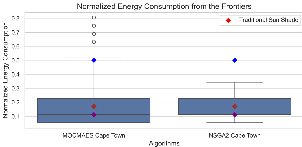
Figure 5.2: Box plots of the normalized energy consumption frontier for Cape Town. Diamond shapes portray the performance of traditional sunshades (A, B, C, D, and E represent red, black, blue, purple, and brown, respectively 4.1). Some overlap made all five points not fully visible. The left and right distributions correspond to MO-CMA-ES and NSGA-II results, respectively. Lower values indicate improved performance.
