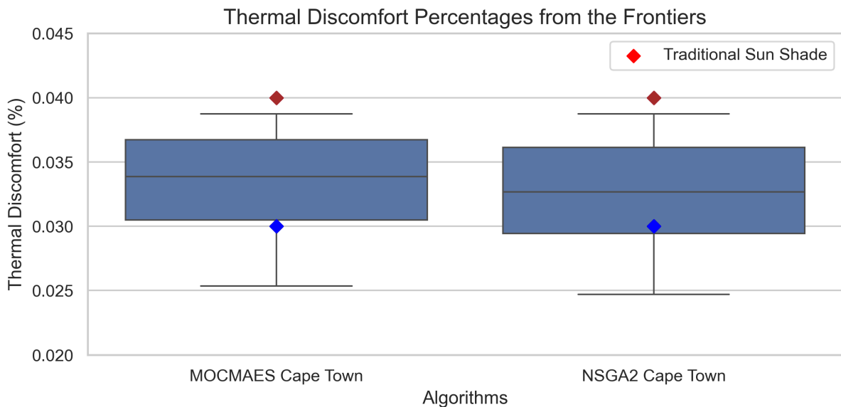
Figure 5.1: Box plots of the normalized thermal discomfort percentage frontier for Cape Town. Diamond shapes portray the performance of traditional sunshades (A, B, C, D, and E represent red, black, blue, purple, and brown, respectively 4.1 ). Some overlaps made all five points not fully visible. The left and right distributions correspond to MO-CMA-ES and NSGA-II results, respectively. Lower values indicate improved performance.
