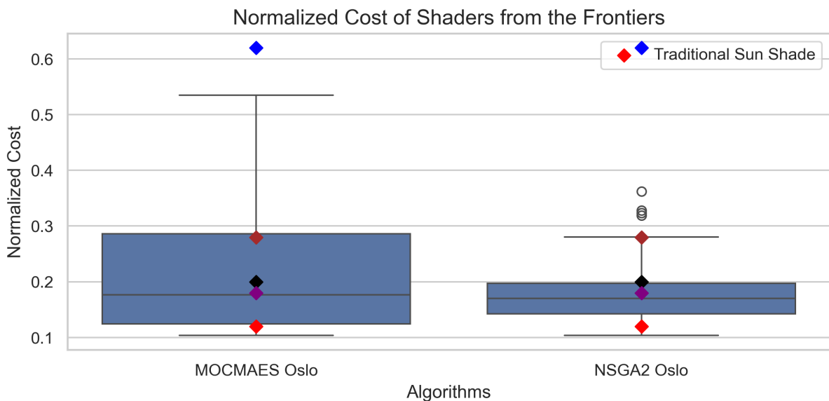
Figure 5.22: Box plots of the normalized cost frontier for Oslo. Diamond shapes portray the performance of traditional sunshades (A, B, C, D, and E represent red, black, blue, purple, and brown, respectively 4.1). The left and right distributions correspond to MO-CMA-ES and NSGA-II results, respectively. Lower values indicate improved performance.
