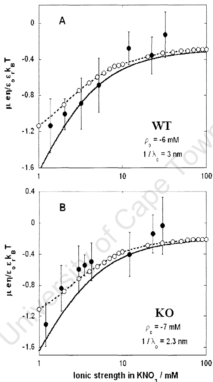
Figure 3.4.4. Electrophoretic mobilities as a function of ionic strength (KNO 3 , pH 6.5) for the two types of S. cerevisiae strains. Experimental data (filled circles) were fitted by using the rigorous numerical evaluations (plain lines) with free parameters, 1/\lambda_0 characterising the typical flow penetration length within the soft polymeric layer and \rho_0 the volumic charge density of that layer. The thickness of the permeable polyelectrolyte layer ( \delta ) has been considered to be 100 nm with a core radius close to 1.5 \mu\text{m} .
