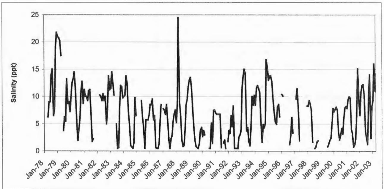
Figure 2: Salinity trend for Sandvlei for the period from April 1978 to March 2003 using the monthly averages of sites 3, 5, 7 and 9 (see Figure 1 for the location of the sampling sites in the estuary).
