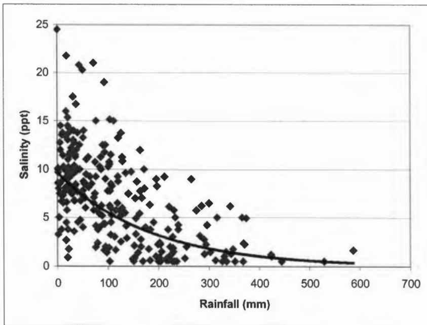
Figure 5 : Regression using monthly rainfall (mm) from Kirstenbosch weather station as the independent variable and the average salinity of the first reading of the following month for sites 3, 5, 7 and 9 as the dependent variable ( n = 269 , R^2 = 0.3911 , p < 0.001 ).
