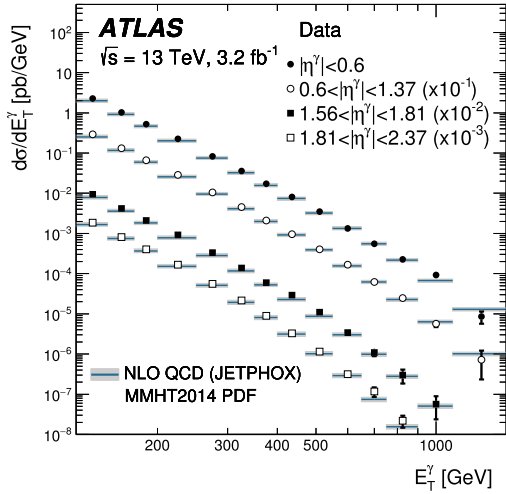
Fig. 2. Measured cross sections for isolated-photon production as functions of E_T^\gamma in |\eta^\gamma| < 0.6 (black dots), 0.6 < |\eta^\gamma| < 1.37 (open circles), 1.56 < |\eta^\gamma| < 1.81 (black squares) and 1.81 < |\eta^\gamma| < 2.37 (open squares). The NLO pQCD predictions from JETPHOX based on the MMHT2014 PDFs (solid lines) are also shown. The measurements and the predictions are normalised by the factors shown in parentheses to aid visibility. The error bars represent the statistical and systematic uncertainties added in quadrature. The shaded bands display the theoretical uncertainty.
