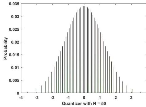
Fig. 3.1: Vector quantization of the Standard Normal distribution
