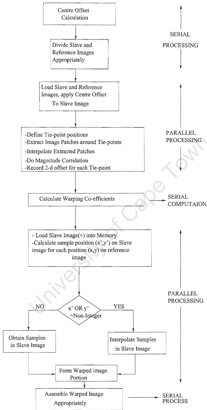
Figure 3.7: Algorithm Flow Diagram
