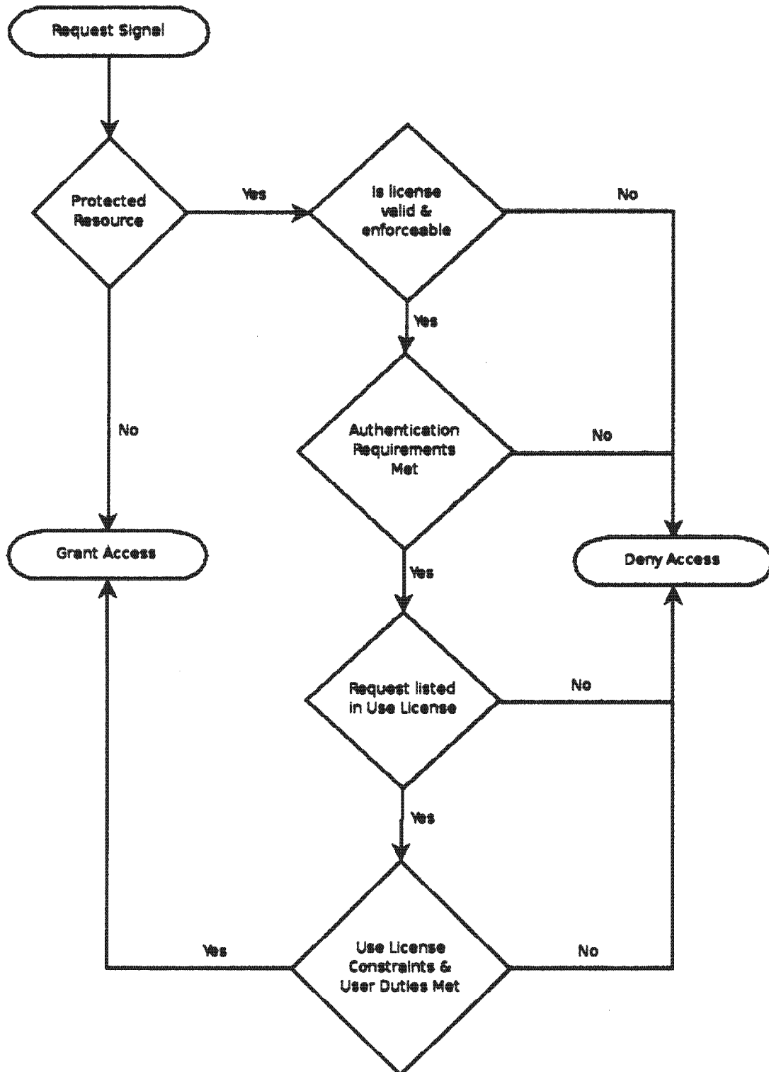
Figure 9.1: DRM Controller Decision Flowchart
