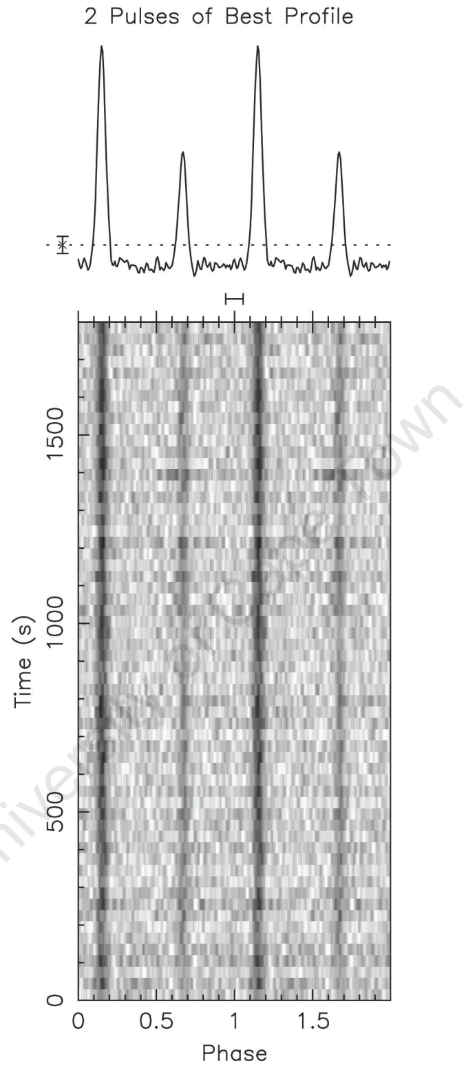
Figure 4.4: Pulse profile of PSR B1937+21 obtained using the Parkes Spectrometer with the NRAO Green Bank 140ft telescope. Image courtesy Glen Langston, Paul Demorest and Scott Ransom (NRAO).
