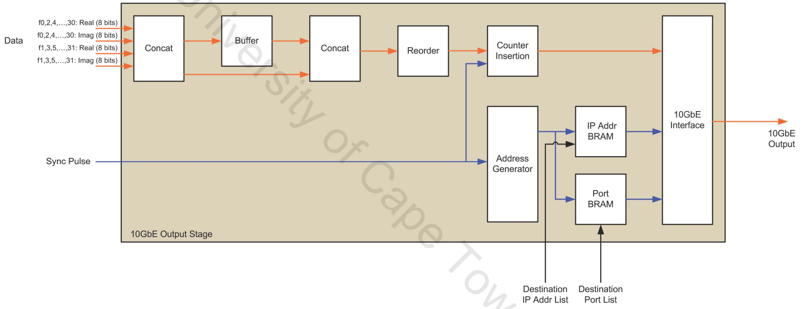
Figure 5.3: The 10GbE Output Stage.
