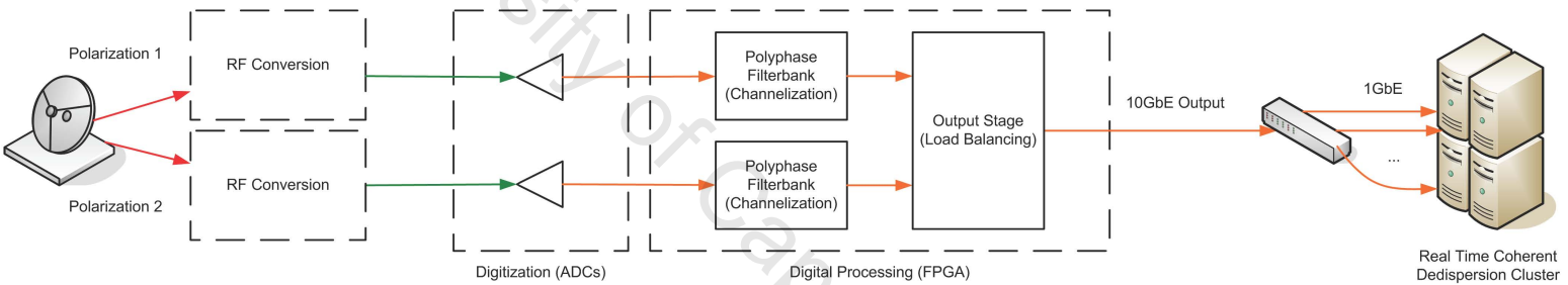
Figure 2.7: Data Flow in a Spectrometer for Coherent Dedispersion Applications.
