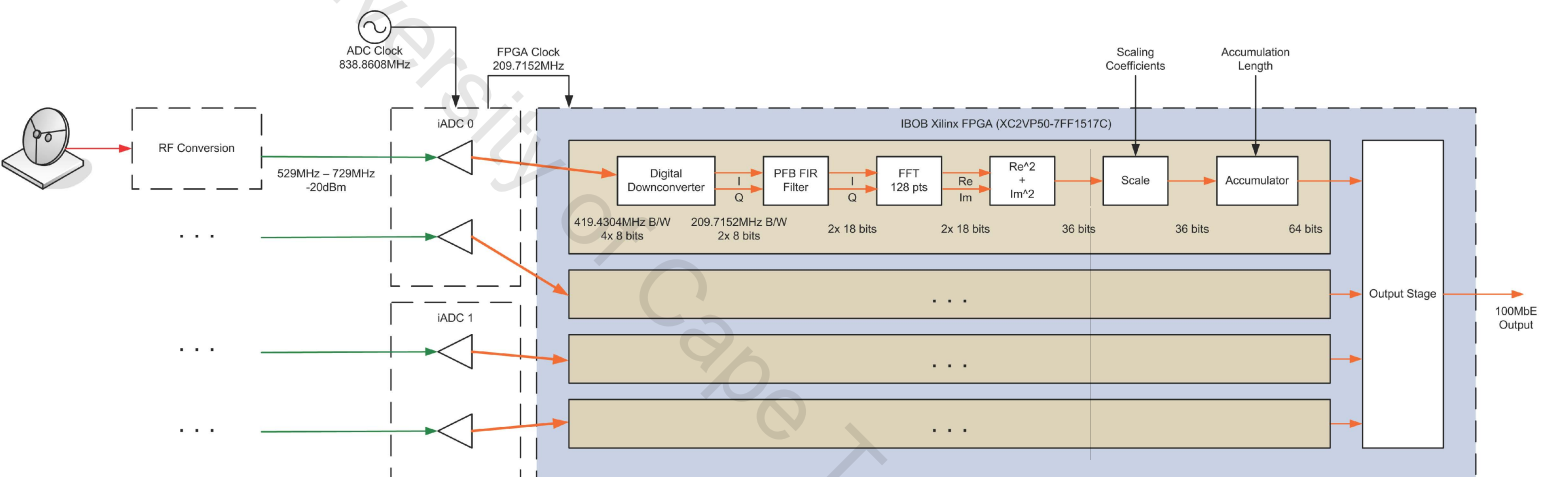
Figure 3.8: A Quad Spectrometer for the Fly's Eye. This single IBOB design implements four independent 210MHz spectrometers whose spectra are dumped over the IBOB's single 100MBE connection.
