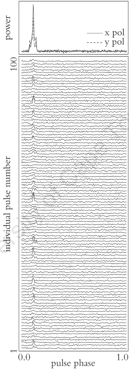
Figure 4.11: Detection of Individual Pulses from PSR B0329+54.
