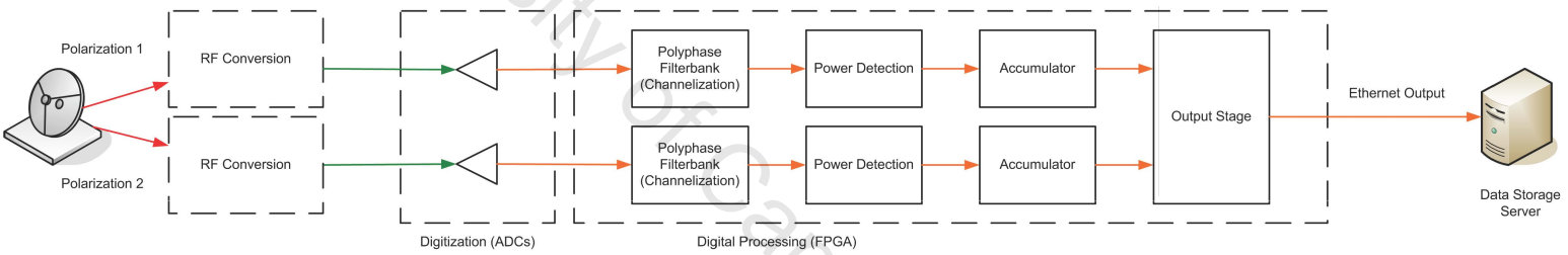
Figure 2.6: Data Flow in a Spectrometer for Incoherent Dedispersion Applications.
