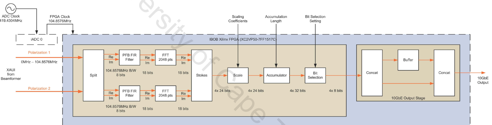
Figure 4.10: The Berkeley ATA Pulsar Processor Spectrometer: a 105MHz Fast-readout Dual Spectrometer with Digital Beamformer Interface
