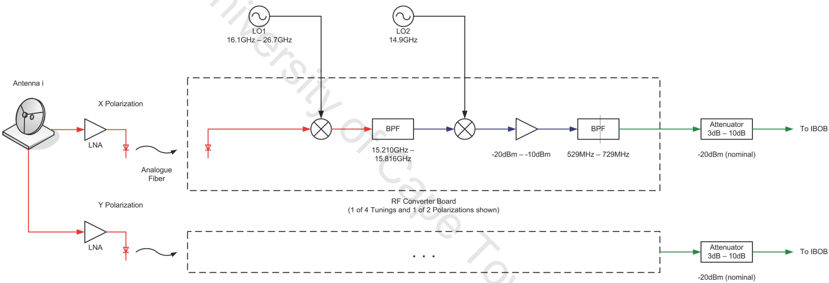
Figure 3.7: Signal path for the Fly's Eye Experiment at the ATA.
