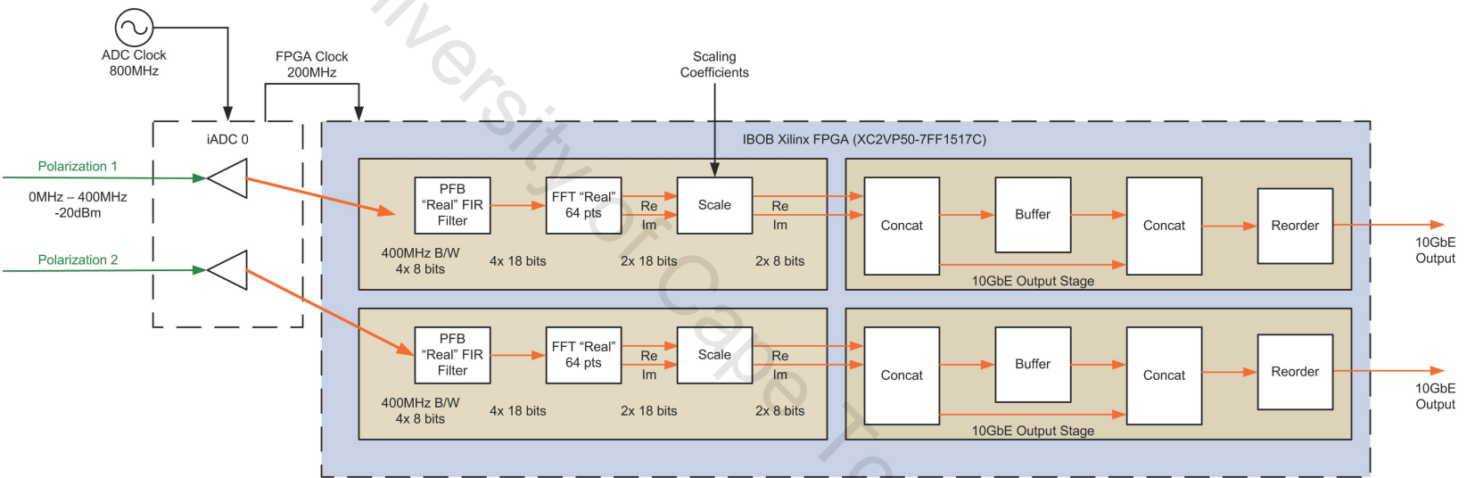
Figure 5.2: A Fast-readout Dual Spectrometer with “raw complex voltage” output.
