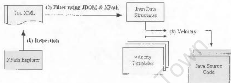
Figure 12: The Code Generation Process with Velocity
