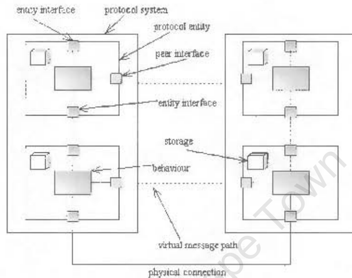
Figure 21: Protocol implementation elements
