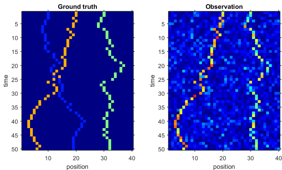
FIGURE 3.1: Sample instantiation of the synthetic one-dimensional adaptive tracking problem.
