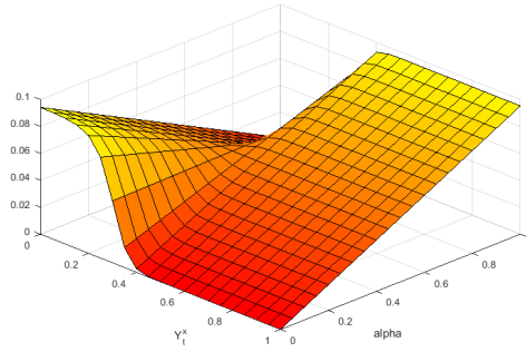
FIGURE 3.12: Update function for a uniform observation model with an alpha mask (normalised across \alpha ). For an observed pixel Y_t^x , the distribution on \alpha will be multiplied by the function defined by the plane for Y_t^x . The observation standard deviation \sigma_{obs} is set to 0.2 for this image.
