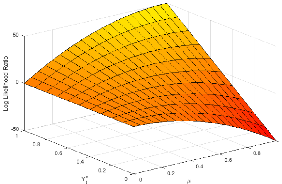
FIGURE 3.4: Model update function for synthetic problem. For a given observation Y_t^x , the distribution on \mu at x will be multiplied in a point-by-point fashion with the intersection of the plane defined by Y_t^x and the above surface.
