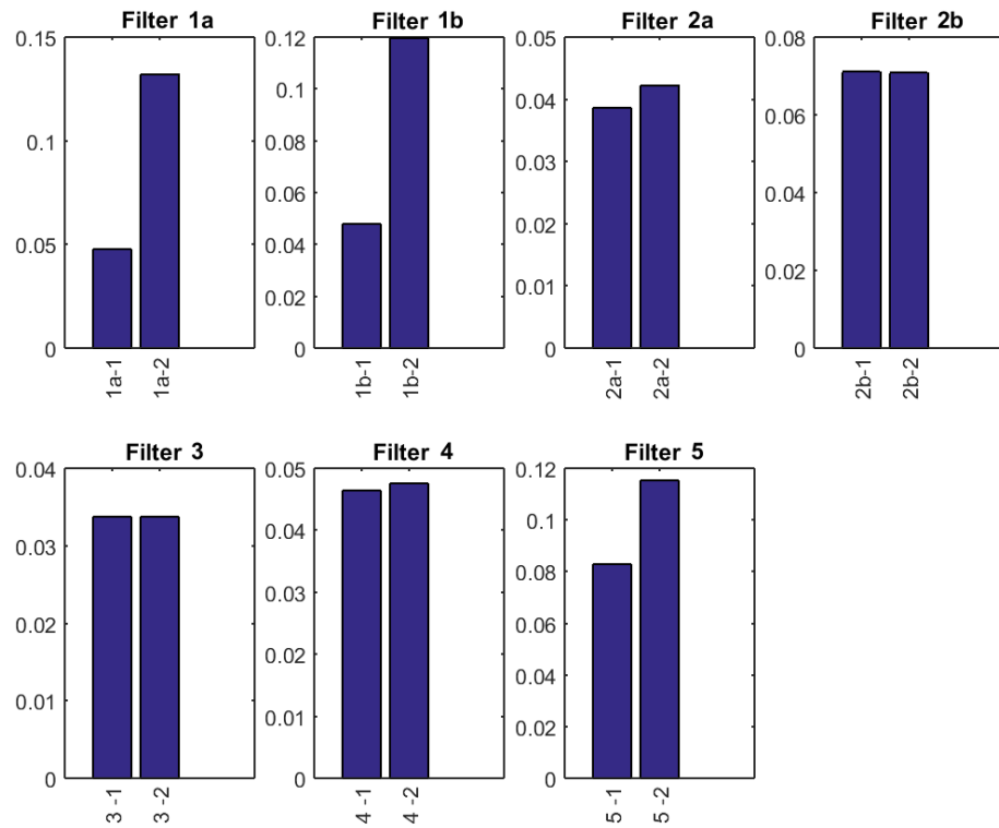
FIGURE 4.6: Naive and upper-bound performance for each saliency filter.
