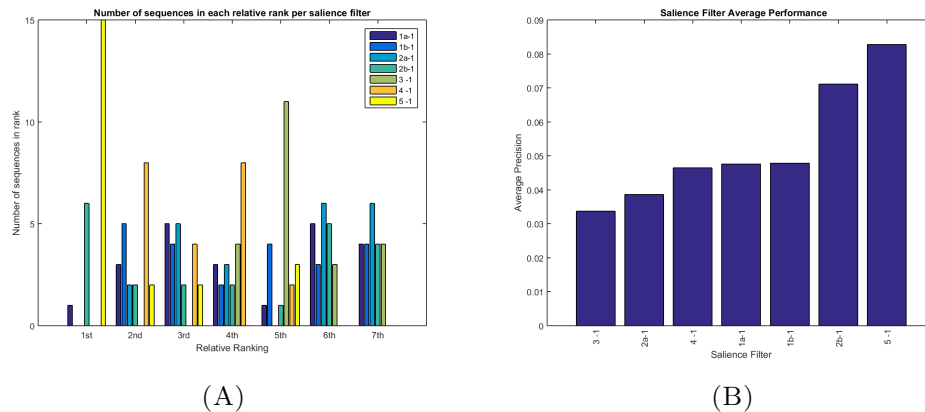
FIGURE 4.5: Saliency filter performance: (A) shows the distribution of relative ranks each filter achieved in number of sequences. (B) shows the average precision for each saliency filter across all sequences.
