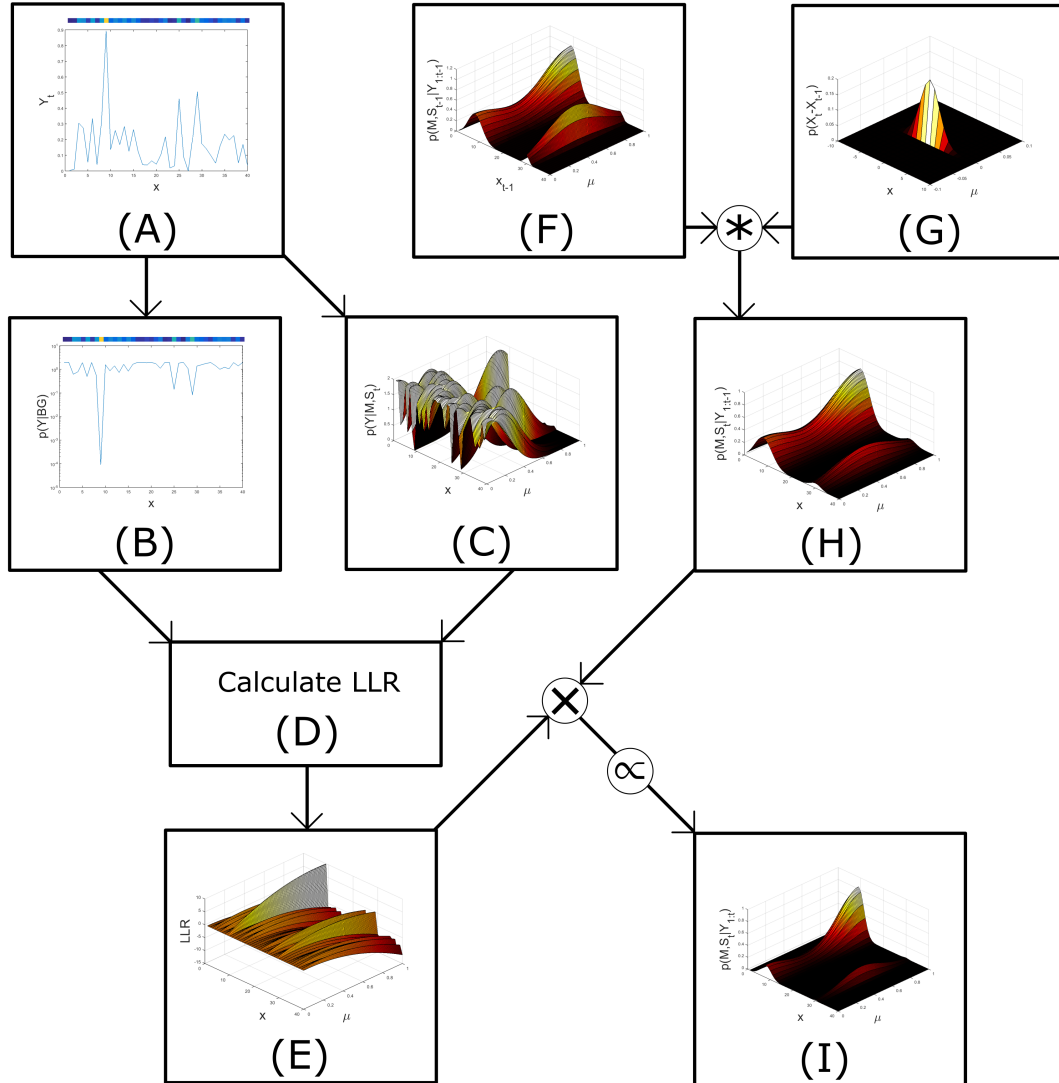
FIGURE 3.3: A single inference step for the synthetic problem. The observations ( Y_t ) for a particular time t are shown in (A). Each pixel ( Y_t^p ) in the observation is used to calculate background likelihoods ( p(Y_t^p|Bg_p) ) in (B) and foreground likelihoods ( p(Y_t^p|M, S_t) ) in (C). As an object affects only the pixel value at its location, the foreground likelihood is composed of slices for each pixel location, defining how well each model predicts the observed pixel. We look at this more in figures 3.4, 3.12 and 3.13, and define it as the update function. The calculation of the log likelihood ratio is done in (D). Each slice in (C) is divided by the appropriate value from (B), and the quotient's log is shown in (E). This forms the observation half of equation 3.2. The posterior for the previous time instance ( p(M, S_{t-1}|Y_{1:t-1}) ) is shown in (F). This is updated by convolution with the motion model (G) to produce the prediction ( p(M, S_t|Y_{1:t-1}) ) (H). The motion model never moves PDF mass from one M value to another, as all the time-varying properties are in S_t . Each M plane can define its own motion model. The prediction and the observation model are combined according to equation 3.2: using point-by-point multiplication, with the result normalised across the entire (M, S_t) plane, to create our posterior p(M, S_t|Y_{1:t}) (I). Our notation in this diagram assumes (E) is not in log-space; we do not include the converting of (E) and (H) to a common space for diagram complexity sake.
