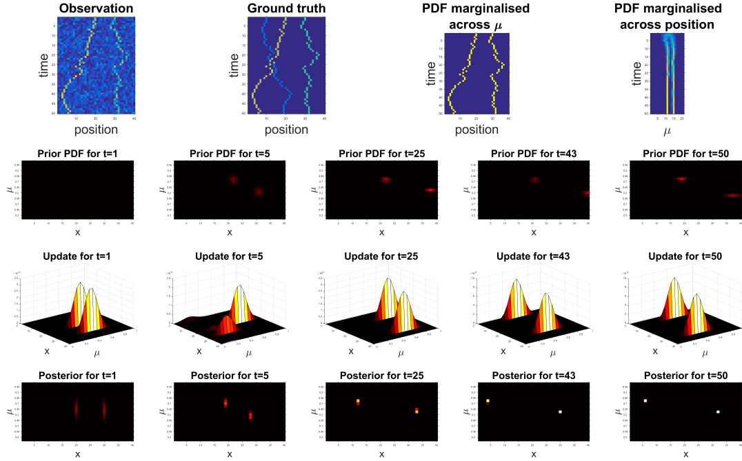
FIGURE 3.6: Results for the synthetic problem assuming that exactly two targets are visible. The top row shows observations given to the estimator, the ground truth locations for all targets in the data, and the p(M, S_t) as defined in the text, marginalised across \mu and x . Rows two to four show the prior (row 2), likelihood ratio (row 3), and posterior (row 4) for 5 different instances in time (the 4-dimensional PDF has been collapsed into a 2D representation as described in the text).
