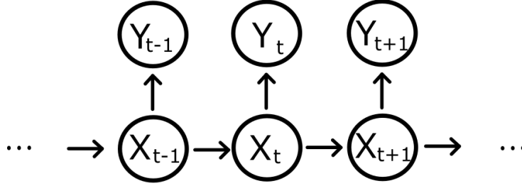
FIGURE 3.2: Bayesian network for a HMM. At each time instant, the current state X_t is dependent only on the previous time instant X_{t-1} . The state is not observable, so all reasoning about the system state needs to be done through the observable variables Y_t that are dependent on X_t .
