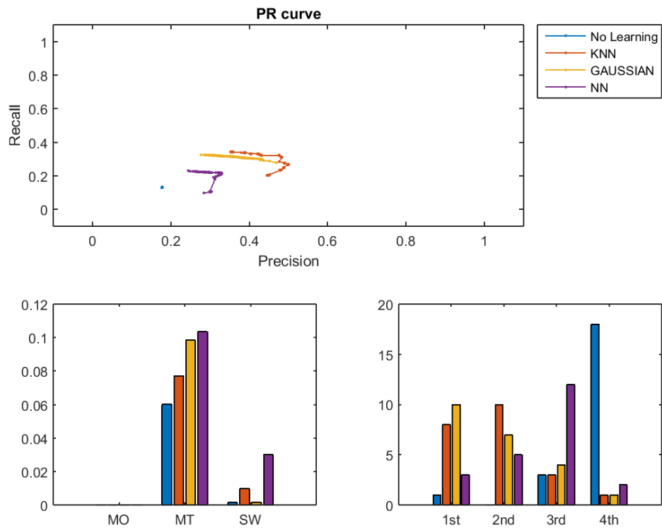
FIGURE 5.10: The top shows PR curves for the three persistent trackers relative to the baseline adaptive tracker. The lower left shows MT, MO, and SW scores for the different trackers. The lower right shows the number of sequences each tracker ranked in each position (as judged by F-score). The MT, MO, and SW errors use the arithmetic mean again, as the harmonic mean of any set with a zero element is zero.
