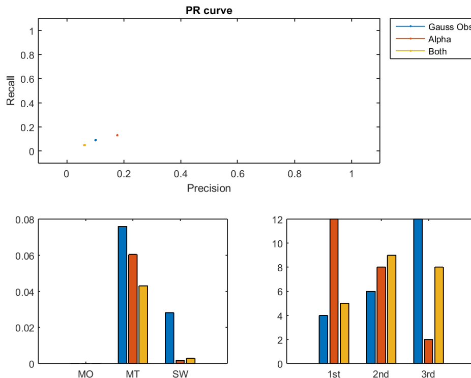
FIGURE 5.4: The top shows PR points for the three adaptive trackers. Learning to reject tracks, and hence move along a PR curve, comes with training that will be integral to our persistent trackers. The lower left shows MT, MO, and SW scores for the different trackers. The lower right shows the number of sequences each tracker ranked in each position (as judged by F-score). For the MT, MO, and SW errors we show the arithmetic mean instead of the harmonic, as the harmonic mean of any set with a zero element is zero, and hence would be meaningless for these metrics.
