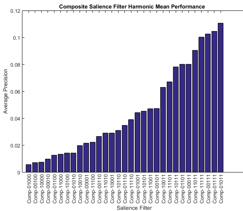
FIGURE 4.9: The harmonic mean precision for each composite filter.
