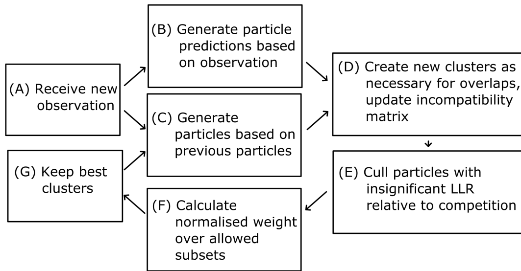
FIGURE 3.11: A single iteration of the particle-based SMAE tracking algorithm. For each frame that is received, (A) a set of hypothesised particles is created, using the pixels that are most salient (B) and the previous frame’s output (C). The algorithm then updates the clusters, calculates their LLR, and creates new clusters as necessary (D). The algorithm culls those particles whose LLR are insignificant compared to those they are competing against (E). This means that when particles overlap, and clusters are created to handle the various possibilities, insignificant ones are disregarded. Finally, the algorithm uses equation 3.12 to calculate the posterior for each particle (F), and keeps the best ones for the next frame (G).
