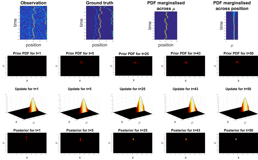
FIGURE 3.5: Results for the synthetic problem as STT. The top row shows observations given to the estimator, the ground truth locations for all targets in the data, and the posterior PDF marginalised across \mu and x . Rows two to four show the prior (row 2), likelihood ratio (row 3), and posterior (row 4) for 5 different instances in time.
