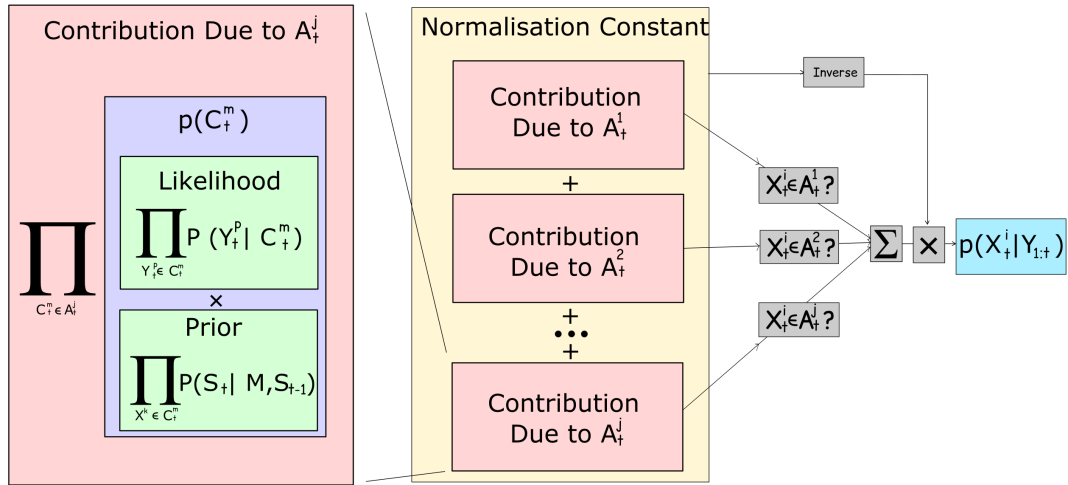
FIGURE 3.8: Multiple-target particle filter algorithm. Each cluster's contribution ( p(C_t^m) ) is calculated as the product of its prior (the product of all its constituent particles' priors) and its likelihood (the product of likelihoods for all the pixels it addresses). The viable subset of clusters A_t^j is iterated over, and each is assigned a contribution equal to the product of all the clusters it includes. The final posterior for particle X_t^i is the sum of contributions for the A_t^j that contain X_t^i , normalised by the sum of all A_t^j contributions.
