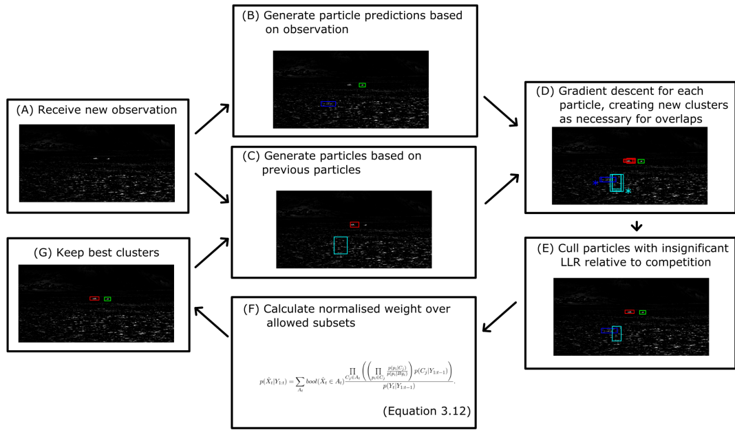
FIGURE 5.2: A single iteration of the tracking algorithm. For each frame that is received (A), a set of hypothesised particles is created using the large regions of salience (with perspective taken into account) (B) and the previous frame’s output (C). These particles are then fitted using a gradient descent optimising the LLR (D), creating new clusters as necessary. In this example, the blue and cyan particles overlap, and so the algorithm creates a cluster for the combination of particles in addition to the two original clusters (indicated with asterisks). The algorithm then culls those particles whose LLR is insignificant compared to those with which they compete (E). In this case, that is the clusters involved with the blue and cyan particles; the combination cluster has a much larger LLR, and the two individual clusters are rejected. Finally, the algorithm uses equation 3.12 to calculate the posterior for each particle (F), and keeps the best ones for the next frame (G). For all the frames, only the bounding-boxes are shown. Each particle has a distribution in M (not shown), as illustrated in figure 5.1.
