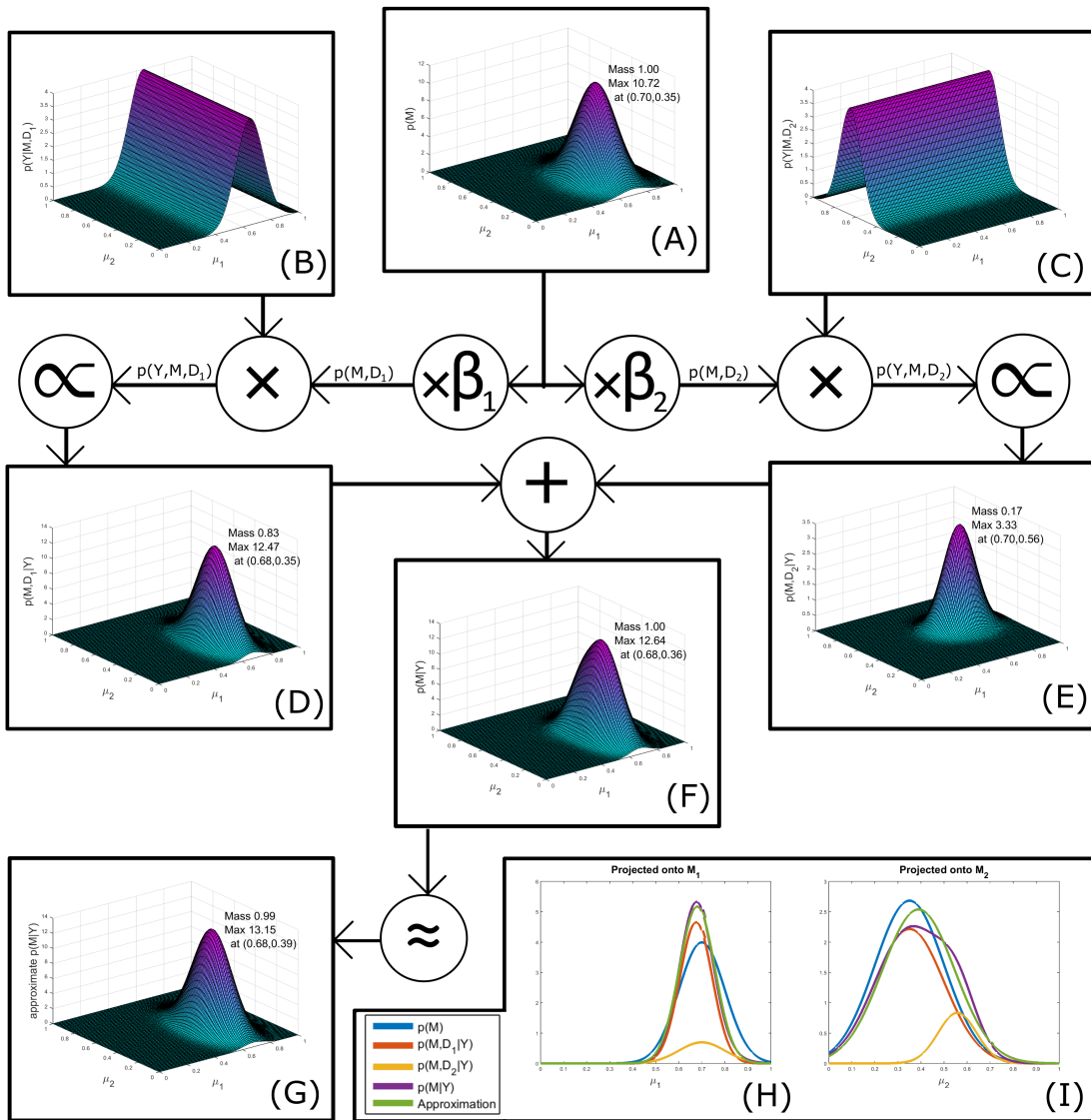
FIGURE 3.9: Model inference for overlapping particles. All surfaces shown are joint PDFs across the two particles' M -variables (their S -variables are the same, due to the overlap). We use the Cool color map (cyan to purple) to differentiate this from other joint surfaces previously shown, especially X the joint across a particle's (M, S_t) variables. The prior on the joint M space is shown in (A). This is constructed from independent Gaussian distributions for \mu_1 and \mu_2 . The likelihoods (i.e. observation models) given that the observation originated from \hat{X}_1 and \hat{X}_2 are shown in (B) and (C) respectively. By taking the point-by-point product of these (with the appropriate \beta values), we can get the two terms in the numerator of equation 3.23. To get the normalising factor, we take the sum of the masses of the distributions in these two terms. Once we have divided by this normalisation constant, we get (D) and (E), the posteriors attached to D_1 and D_2 respectively, and their sum (F). We then approximate this posterior, with \mu_1 and \mu_2 being independent Gaussian variables, to get (G). On account of this final approximation, we can do this entire process without constructing the joint PDF. This process projected onto M_1 and M_2 is shown in (H) and (I). Key features to note are as follows: (B) and (C) only affect their relevant variable. The peak of (D) has moved in \mu_1 and the Gaussian is narrower along \mu_1 's dimension, but the plot is unchanged in \mu_2 ; equivalently for (E). The relative scales of (D) and (E) are due to how far the observation was from the priors on \mu_1 and \mu_2 respectively. This leads to a posterior (F), that is a sum of Gaussians. We accept the inaccuracy of a single Gaussian approximation (G), as (F) will become dominated by a single Gaussian for disparate M_1 and M_2 variables.
