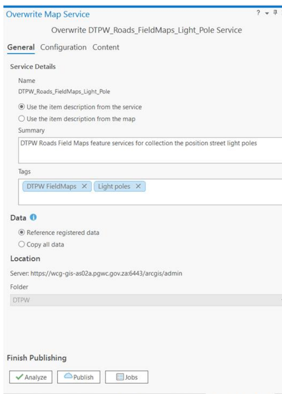
Figure 4: Publishing the field capture feature service in ArcPro.
