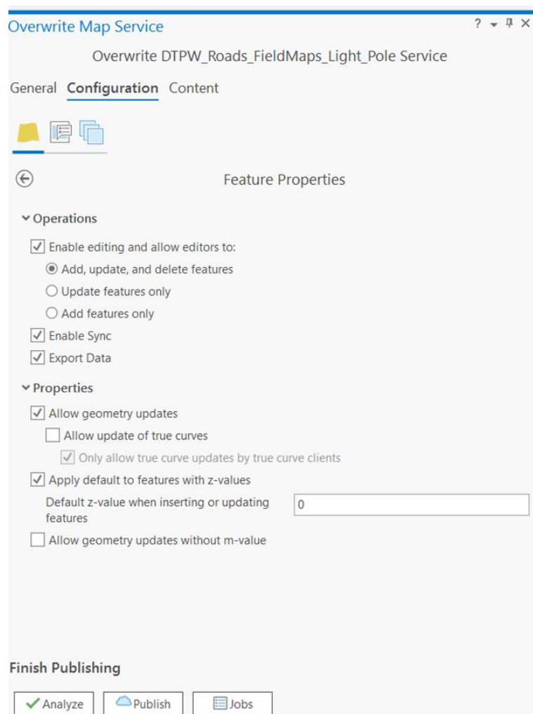
Figure 5: Allowing editability and synchronisation of the feature service
