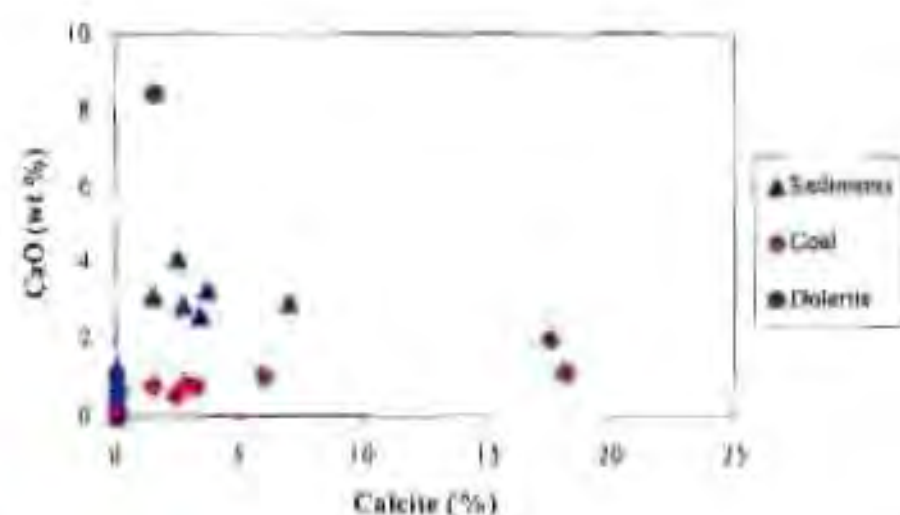
Figure 4.15: Relationship between calcium concentration and calcite composition of selected lithological units
