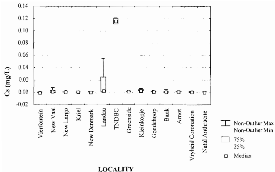
Figure 3.33a: Cesium concentration of water samples from Highveld collieries (n=162).
