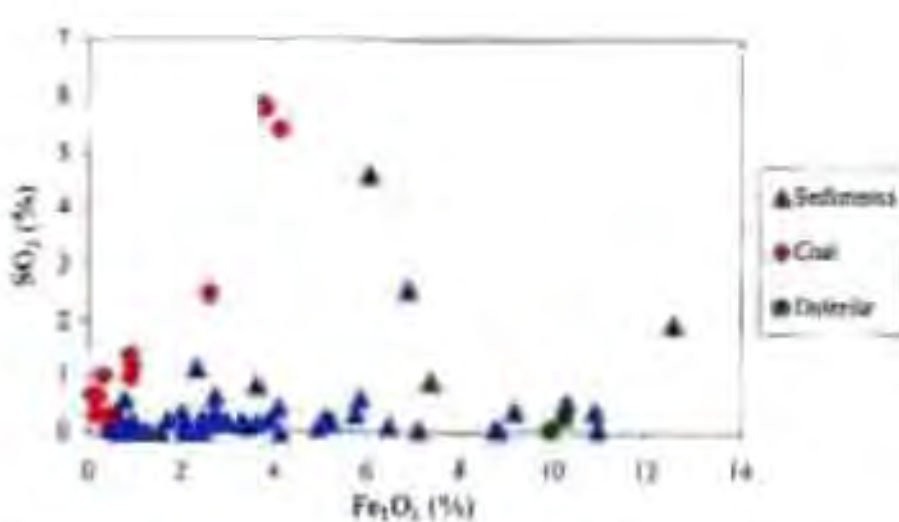
Figure 4.13: Relationship between total sulphur and iron concentration in selected lithological units.
