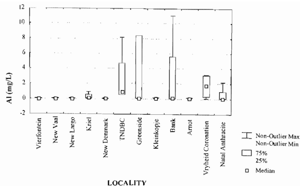
Figure 3.17b: Aluminium concentration of water samples from Highveld collieries, excluding Landau and Goedeheop.
