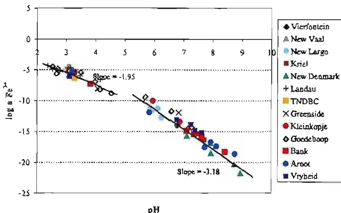
Figure 3.64: Plot of the \log Fe^{2+} activity against pH for the colliery waters. The solid lines show best fit of data between pH of 2 and 5, and pH between 5 and 9.
