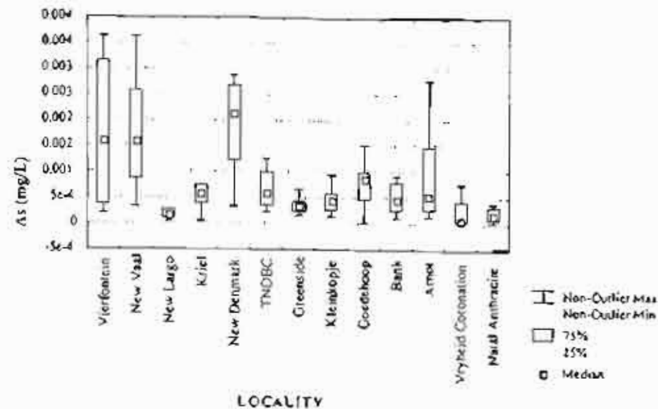
Figure 3.28b: Arsenic concentration of water samples from Highveld collieries, excluding Landau.
