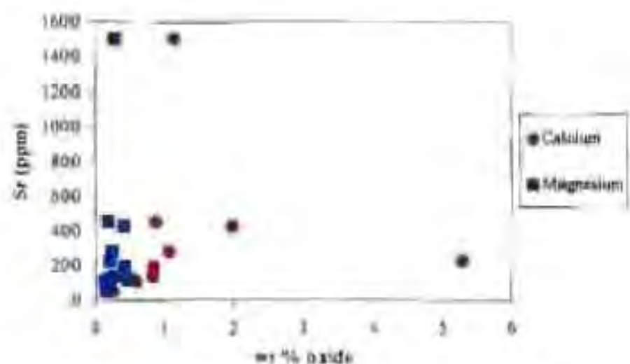
Figure 4.17: Relationship between calcium and magnesium, and strontium in selected lithological units
