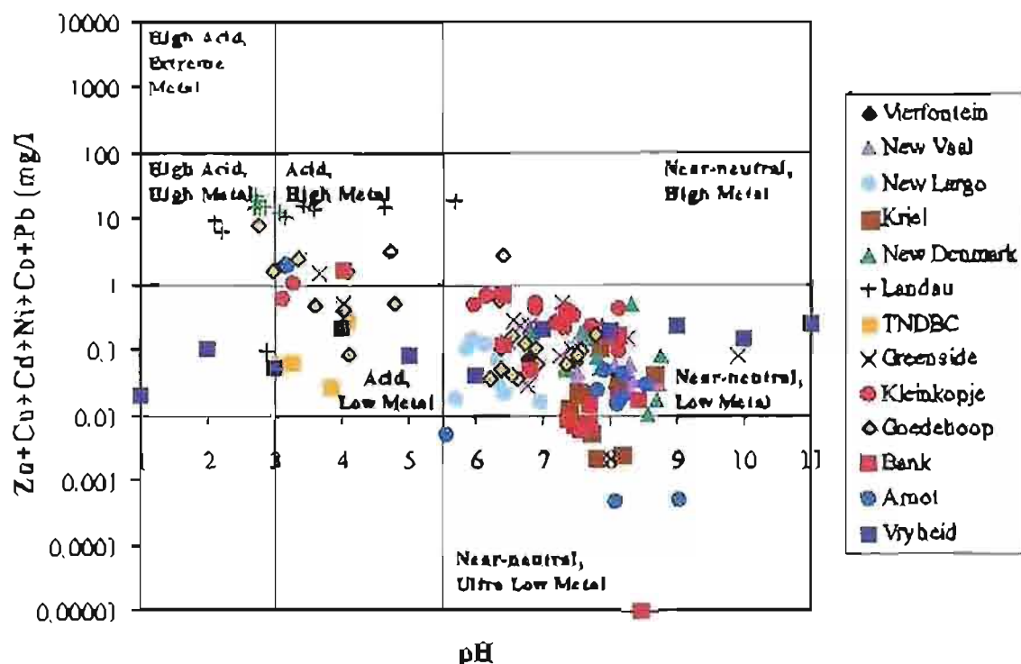
Figure 6.5: Ficklin plot classifying mine drainage based on trace metal concentrations.
