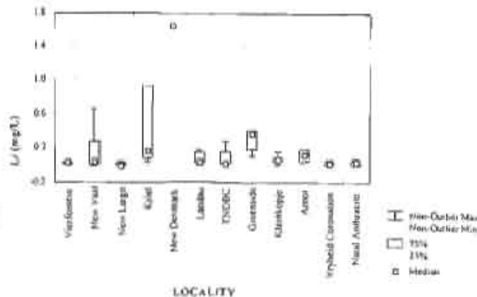
Figure 3.15b: Lithium concentration of water samples from Highveld collieries, excluding Goedehoop and Bank.
