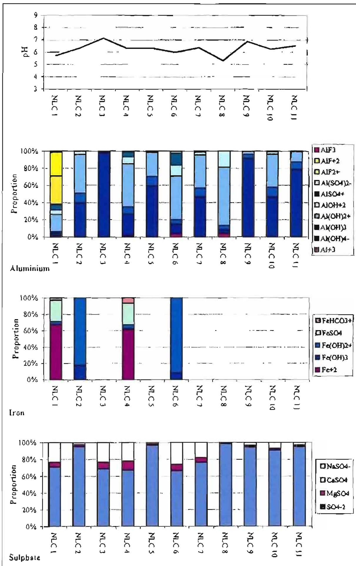
Figure A3.3: Speciation of selected ions in waters from New Lorgo colliery.
