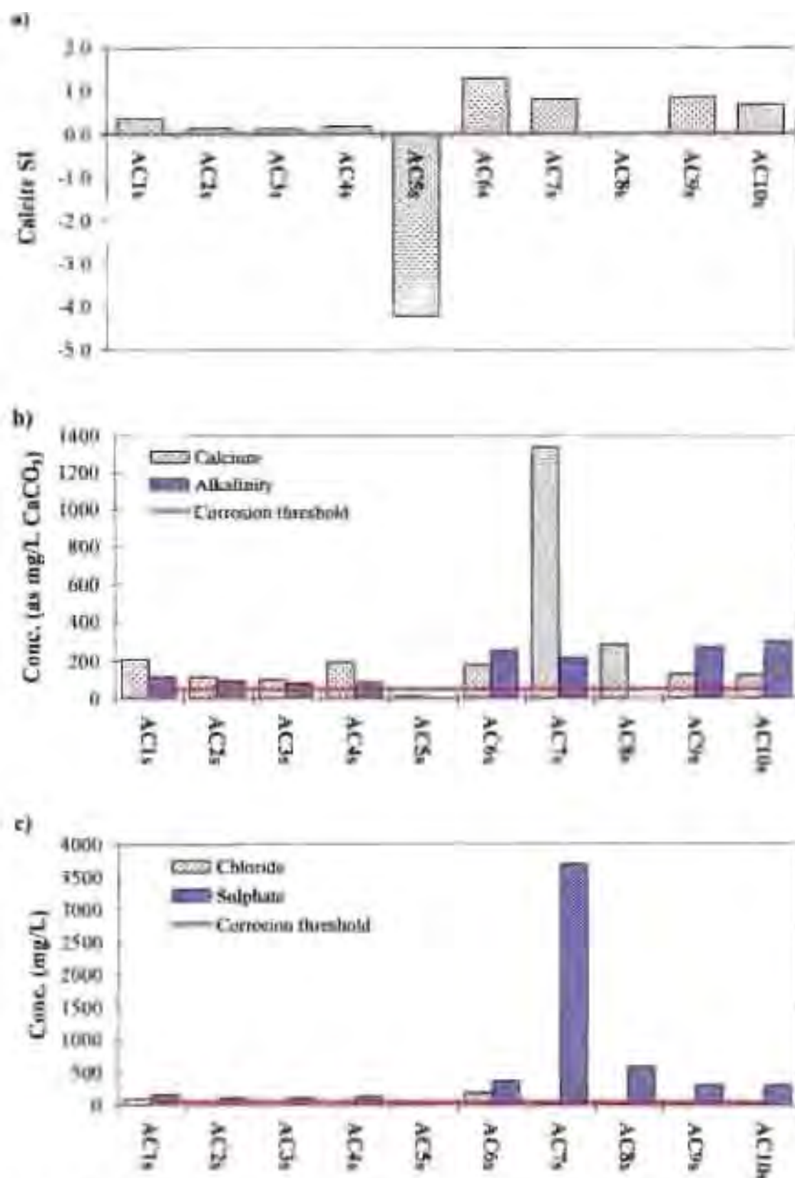
Figure A6.24: (a) Calcium saturation index of Arnot waters. For corrosion prevention SI = 0 (Loewenthal, 1986). (b) Calcium and alkalinity concentrations of Arnot waters. Both calcium and alkalinity concentrations should exceed 50mg/L ( CaCO_3 equivalent) for the prevention of corrosion (Loewenthal, 1986). (c) Chloride and sulphate concentration of Arnot waters. If chloride or sulphate concentration exceeds 50mg/L, the waters will corrode metal surfaces (Loewenthal, 1986).
