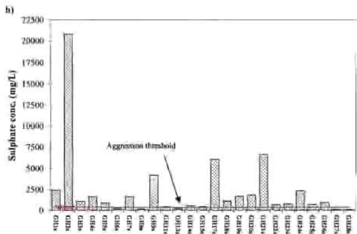
Figure A6.19(a) CCPP of Goedehoop waters in terms of the Laewenthal et al. (1986) guidelines for the prevention of aggression. A CCPP of 4mg/l. is recommended. (b) Sulphate concentration of Goedehoop waters in terms of the Laewenthal et al. (1986) guidelines for the prevention of aggression. The concentration should not exceed 350mg/l.
