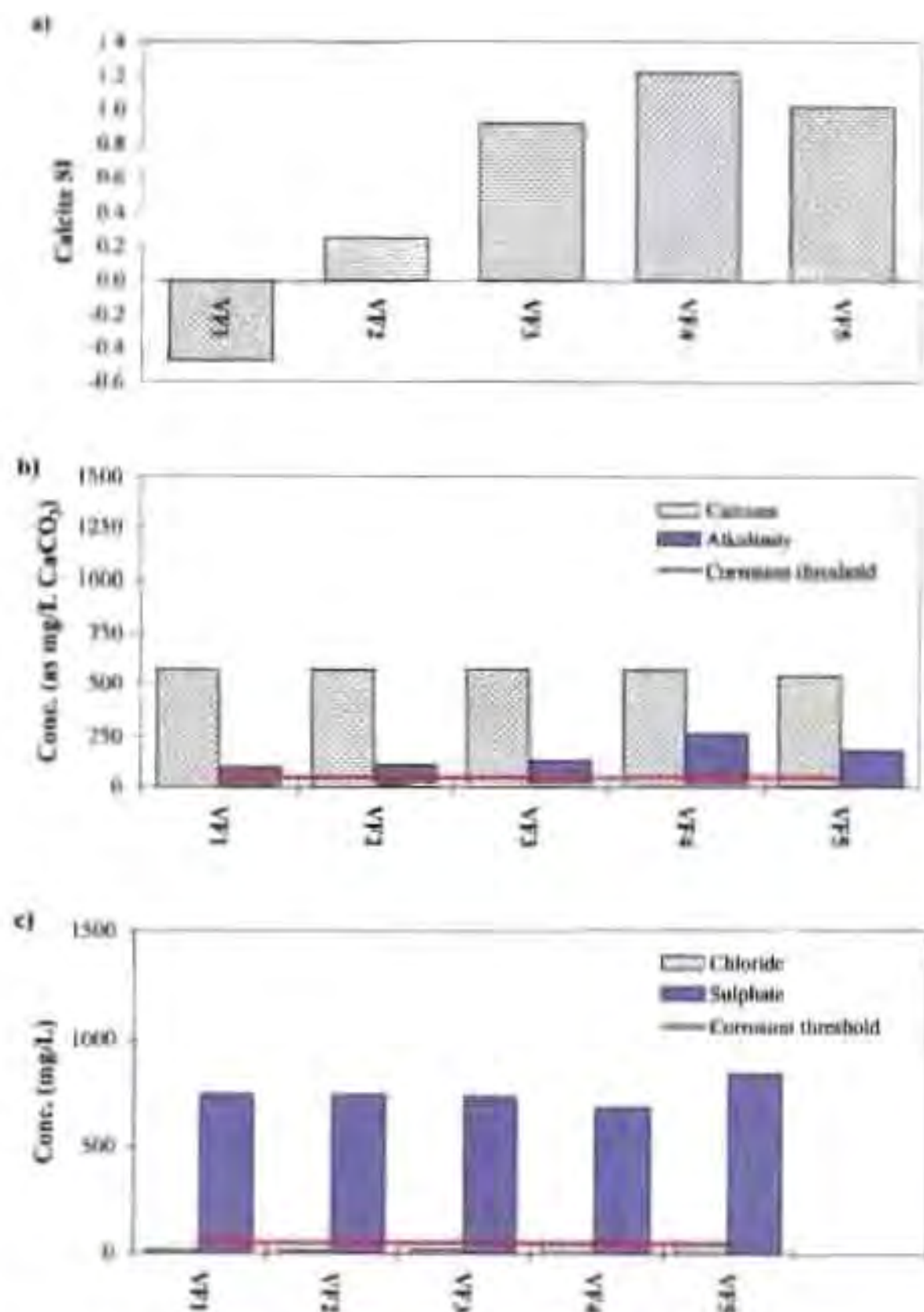
Figure A6.2: (a) Calcium saturation index of Virginian waters. For corrosion prevention, SI > 0 (Loewenthal, 1986). (b) Calcium and alkalinity concentrations of Virginian waters. Both calcium and alkalinity concentrations should exceed 50mg/L ( \text{CaCO}_3 equivalent) for the prevention of corrosion (Loewenthal, 1986). (c) Chloride and sulphate concentration of Virginian waters. If chloride or sulphate concentration exceeds 50mg/L the waters will corrode metal surfaces (Loewenthal, 1986).
