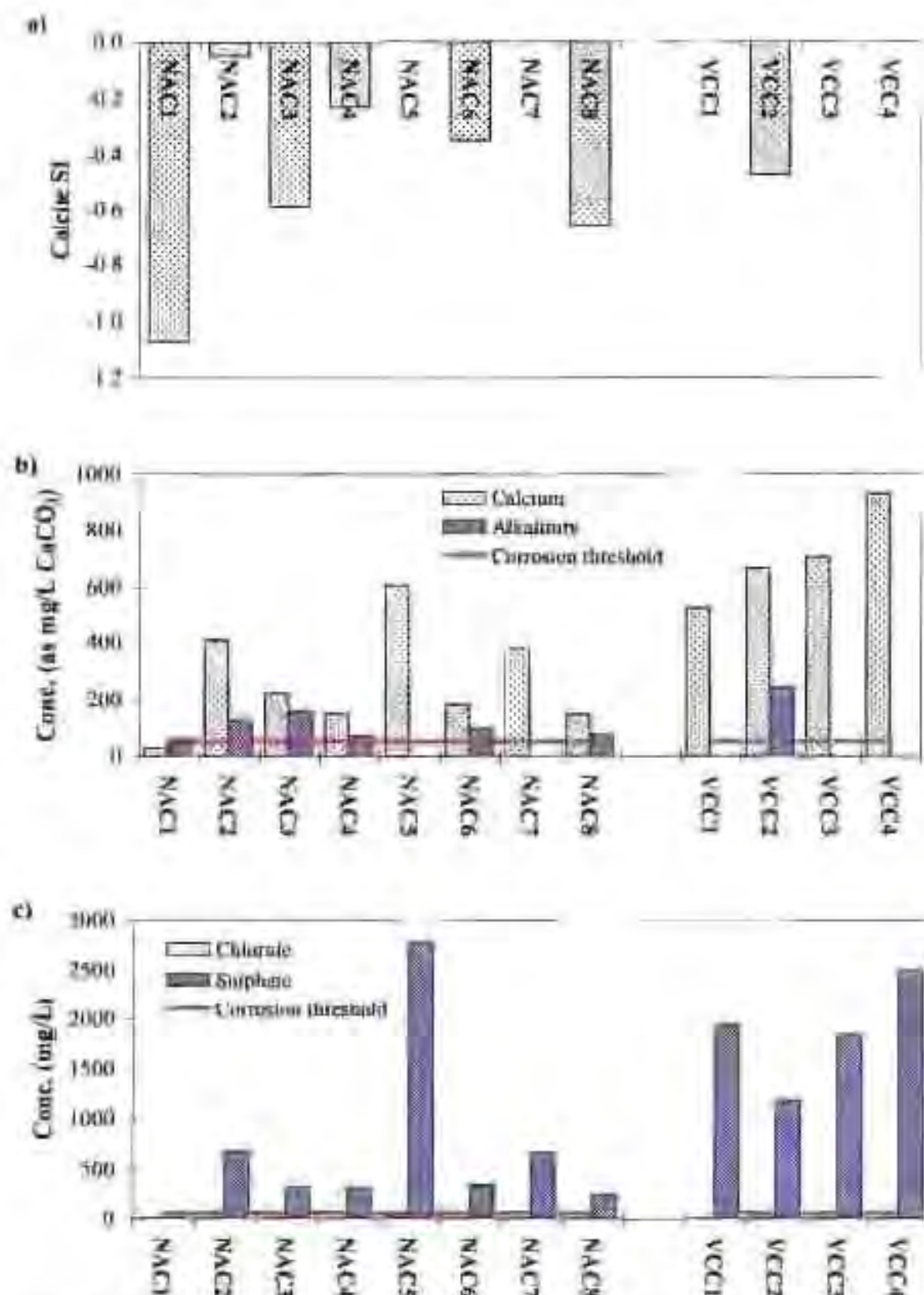
Figure A6.26: (a) Calcite saturation index of Vryheid waters. For corrosion prevention, SI \geq 0 (Loewenthal, 1986). (b) Calcium and alkalinity concentrations of Vryheid waters. Both calcium and alkalinity concentrations should exceed 50mg/L (as CaCO_3 equivalent) for the prevention of corrosion (Loewenthal, 1986). (c) Chloride and sulphate concentration of Vryheid waters. If chloride or sulphate concentration exceeds 50mg/L, the waters will corrode metal surfaces (Loewenthal, 1986).
