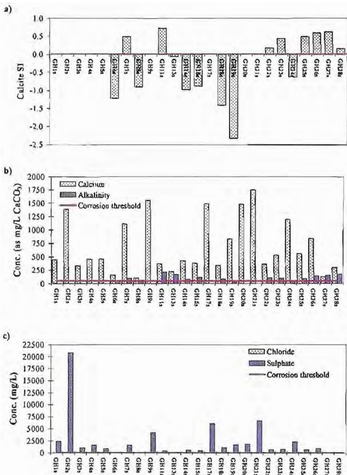
Figure A6.20: (a) Calcite saturation index of Goedeheop waters. For corrosion prevention, SI > 0 (Loewenthal, 1986). (b) Calcium and alkalinity concentrations of Goedeheop waters. Both calcium and alkalinity concentrations should exceed 50mg/L ( \text{CaCO}_3 equivalent) for the prevention of corrosion (Loewenthal, 1986). (c) Chloride and sulphate concentration of Goedeheop waters. If chloride or sulphate concentration exceeds 50mg/L the waters will corrode metal surfaces (Loewenthal, 1986).
