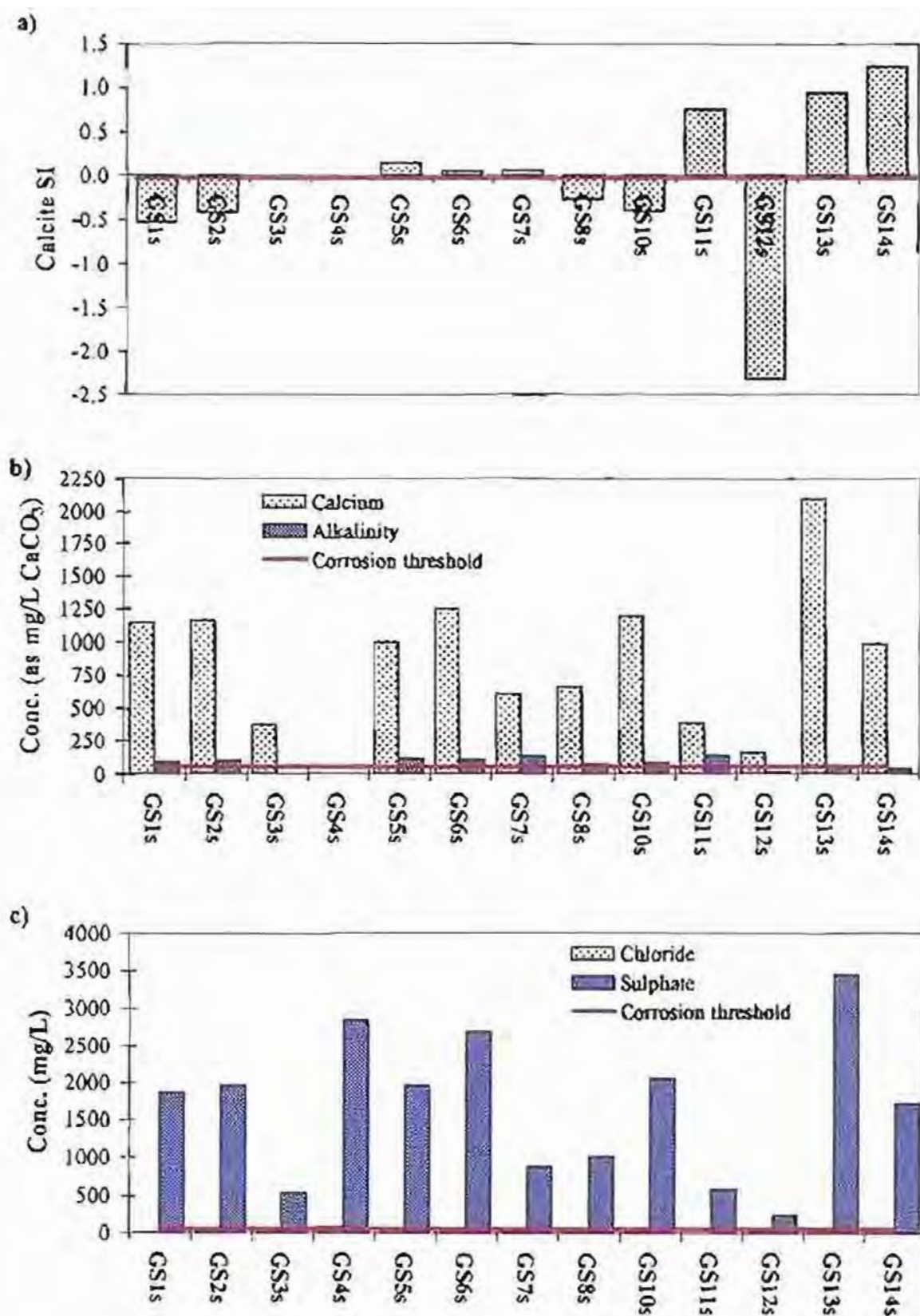
Figure A6.16: (a) Calcite saturation index of Greenside waters. For corrosion prevention, SI > 0 (Loewenthal, 1986). (b) Calcium and alkalinity concentrations of Greenside waters. Both calcium and alkalinity concentrations should exceed 50mg/L ( \text{CaCO}_3 equivalent) for the prevention of corrosion (Loewenthal, 1986). (c) Chloride and sulphate concentration of Greenside waters. If chloride or sulphate concentration exceeds 50mg/L the waters will corrode metal surfaces (Loewenthal, 1986).
