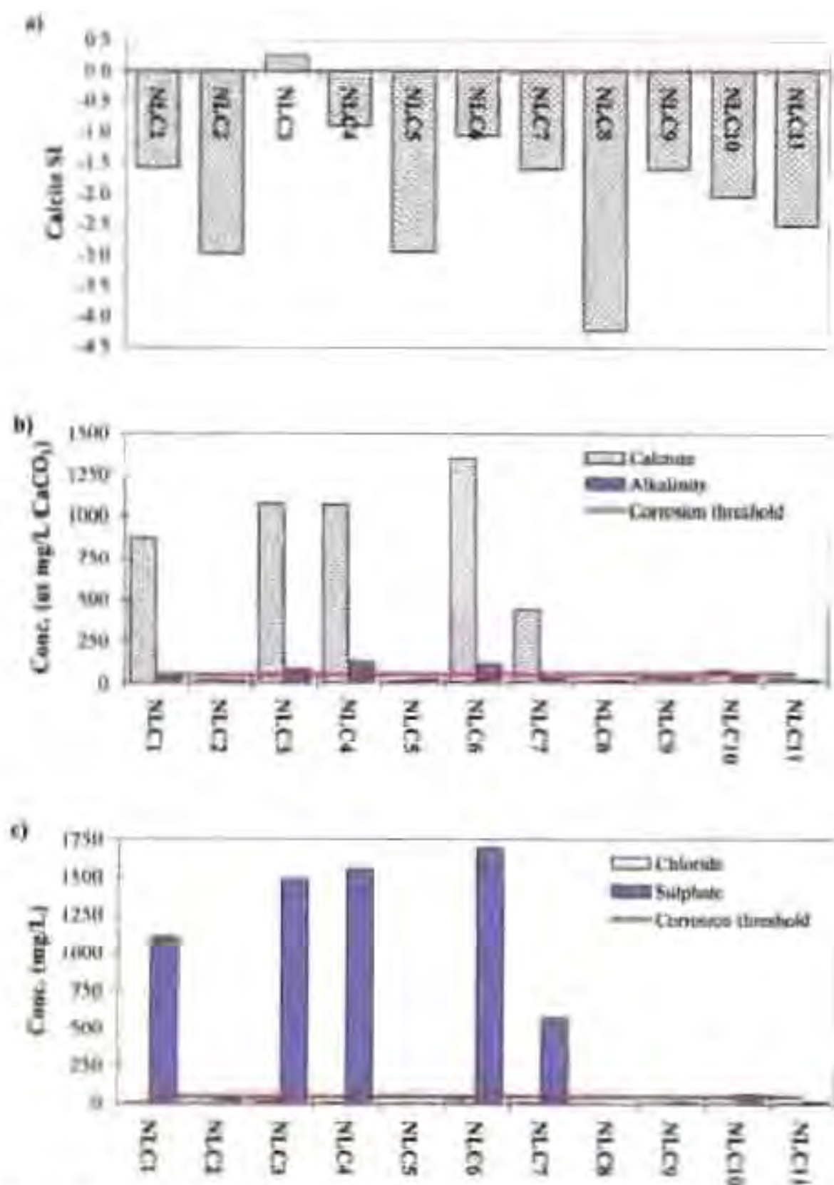
Figure A6.6: (a) Calcium saturation index of New Largs waters. For corrosion prevention, SI > 0 (Lewenzel, 1986). (b) Calcium and alkalinity concentrations of New Largs waters. Both calcium and alkalinity concentrations should exceed 50mg/L ( \text{CaCO}_3 equivalent) for the prevention of corrosion (Lewenzel, 1986). (c) Chloride and sulphate concentration of New Largs waters. If chloride or sulphate concentration exceeds 50mg/L, the waters will corrode metal surfaces (Lewenzel, 1986).
