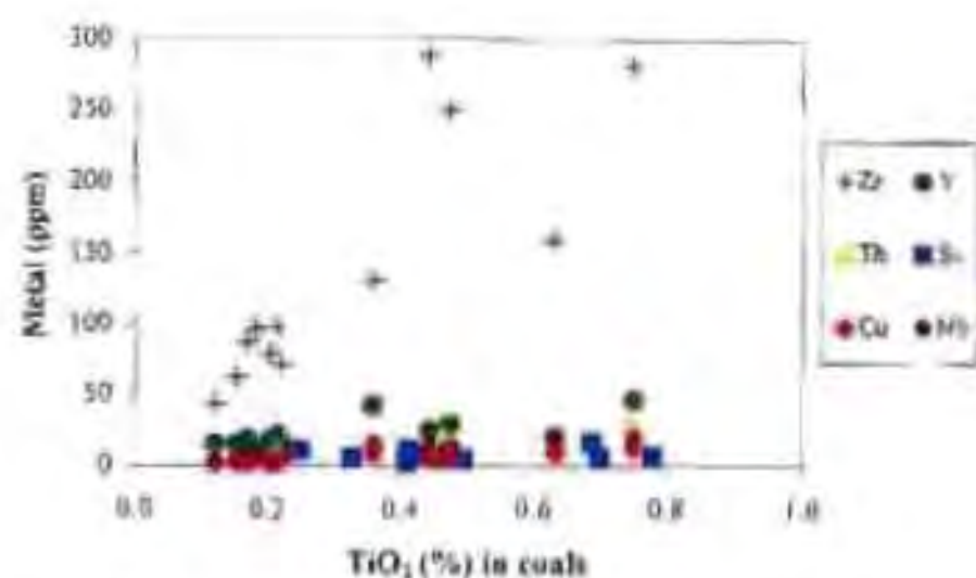
Figure 4.11: Relationship between various metals and titanium in selected lithological units.
