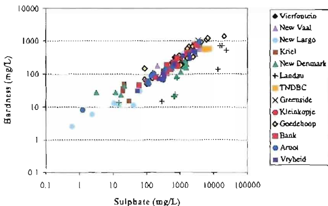
Figure 3.51: Correlation observed between hardness ( \text{Ca} + \text{Mg} ) and sulphate concentration ( r_s=0.907 ).
