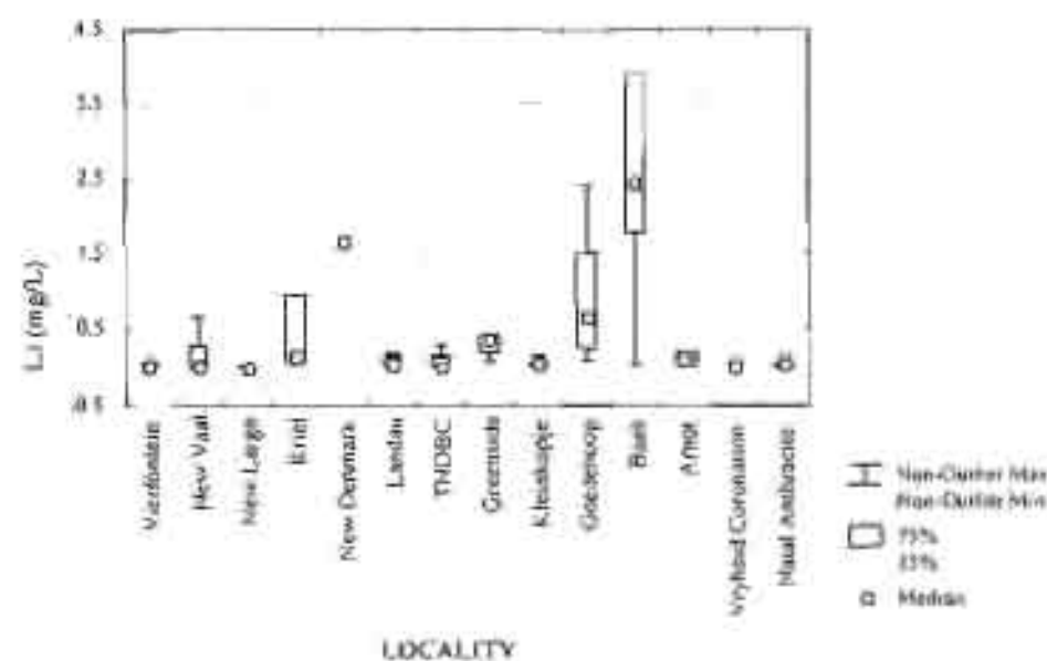
Figure 3.15a: Lithium concentration of water samples from Highveld collieries ( n=12 ).
