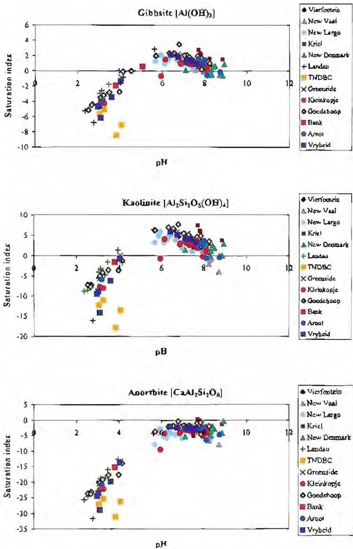
Figure 3.61: Saturation indices for selected aluminum-bearing minerals as a function of pH for the colliery waters.
