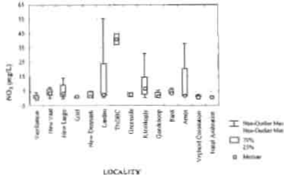
Figure 3.11a: Nitrate concentration of water samples from Highveld collieries (n=105).
