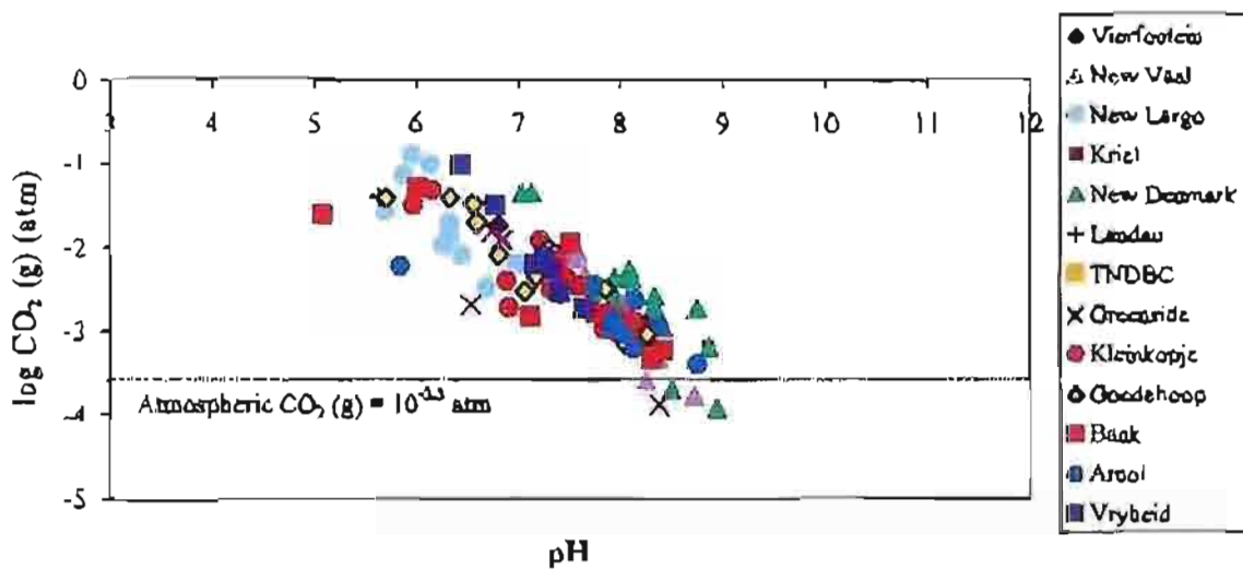
Figure 3.56: Equilibrium partial pressures of \text{CO}_2(\text{g}) as a function of pH for the colliery waters.
