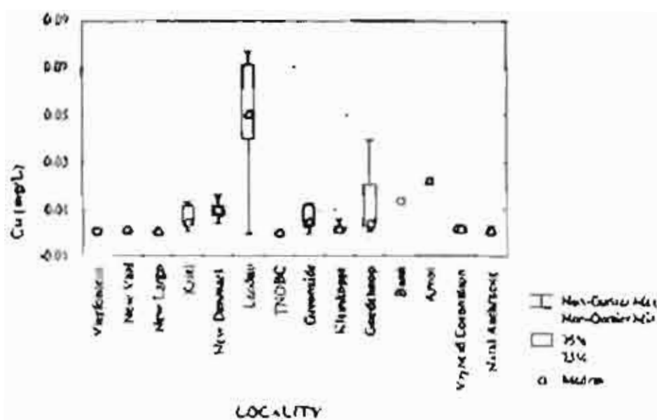
Figure 3.26a: Copper concentration of water samples from Highveld collieries (n=17).
