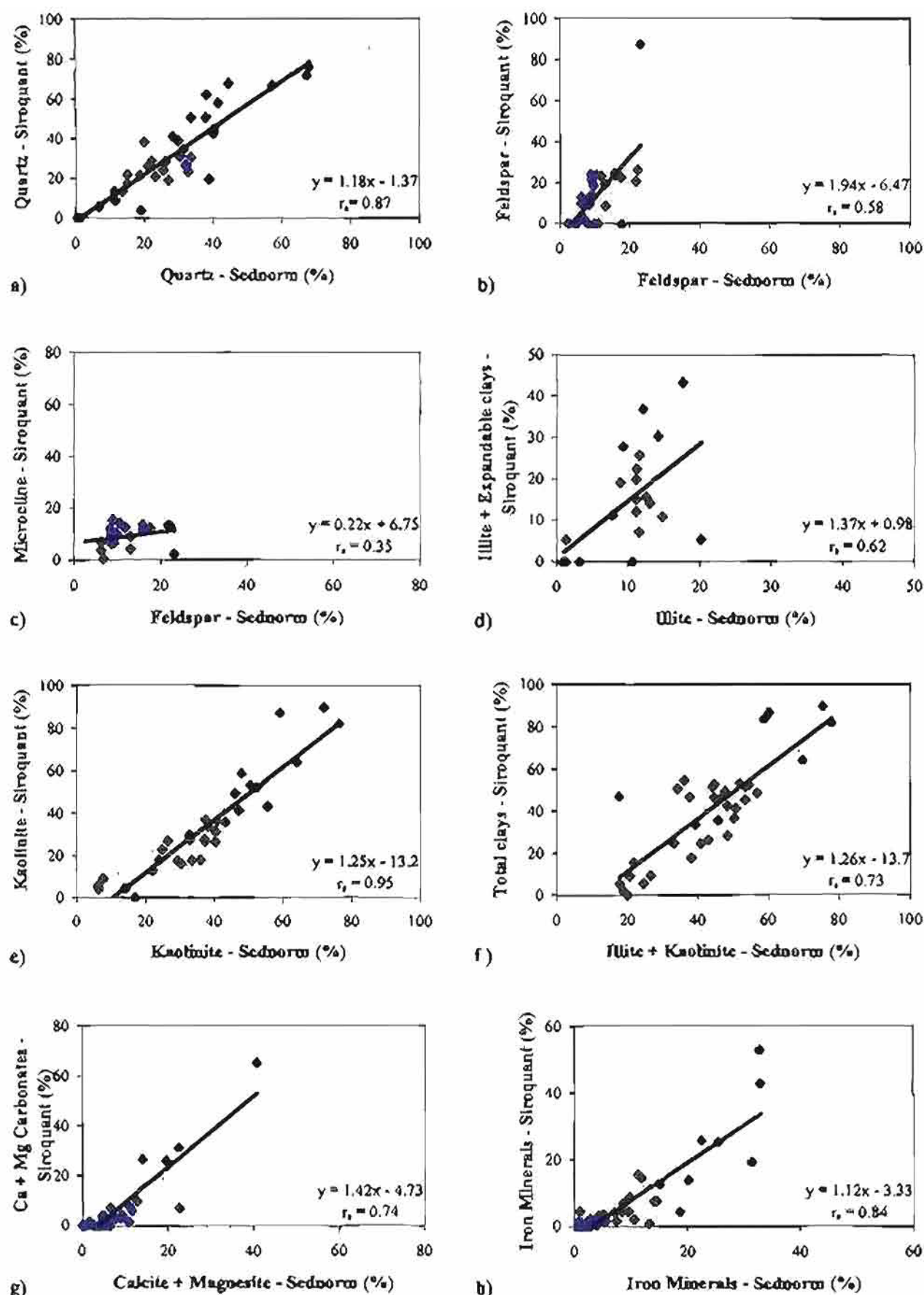
Figure 4.5: Comparison between percentages of different minerals indicated by SEDNORM and SIROQUANT. (a) Quartz, (b,c) Feldspar, (d) Illite and expandable clays, (e) Kaolinite, (f) Total clays, (g) Ca and Mg carbonates, and (h) Iron minerals. Thin dashed line is 1:1 correlation, while thick solid line is the actual correlation.
