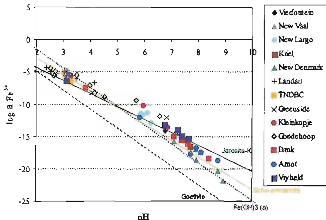
Figure 3.65: Plot of \text{Fe}^{3+} activity against pH for the colliery waters with solubility lines for goethite, jarosite-K, ferrihydrite and schwertmannite.
