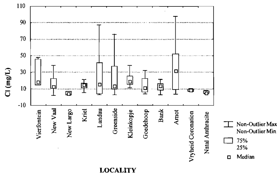
Figure 3.10b: Chloride concentration of water samples from Highveld collieries, excluding New Denmark and TNDBC.
