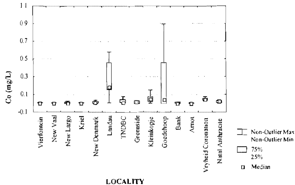
Figure 3.21a: Cobalt concentration of water samples from Highveld collieries (n=166).
