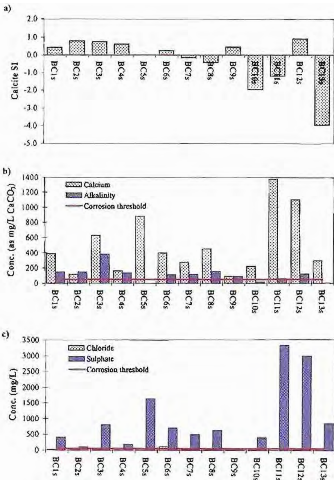
Figure A6.22: (a) Calcite saturation index of Bank waters. For corrosion prevention, SI > 0 (Loewenthal, 1986). (b) Calcium and alkalinity concentrations of Bank waters. Both calcium and alkalinity concentrations should exceed 50mg/L ( \text{CaCO}_3 equivalent) for the prevention of corrosion (Loewenthal, 1986). (c) Chloride and sulphate concentration of Bank waters. If chloride or sulphate concentration exceeds 50mg/L the waters will corrode metal surfaces (Loewenthal, 1986).
