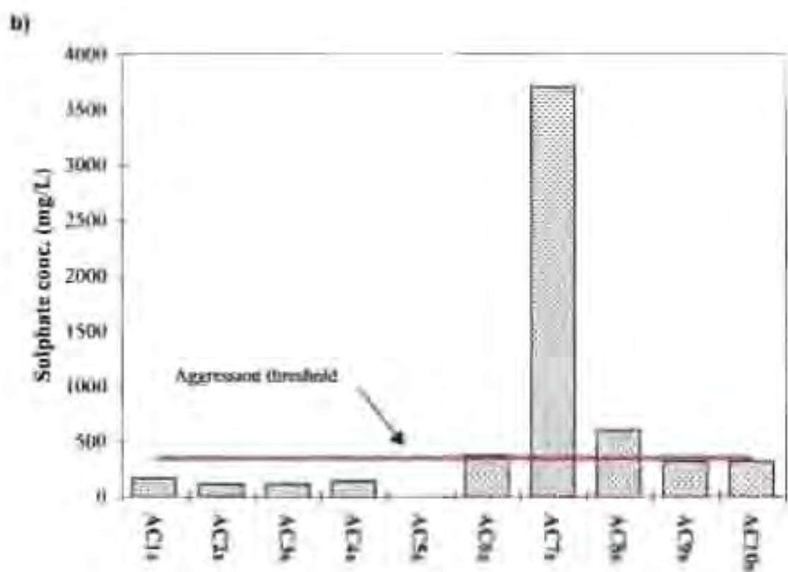
Figure A6.23: (a) Calcium carbonate precipitation potential (CCPP) of Arnot waters in terms of the Loevensthal et al. (1986) guidelines for the prevention of aggression. A CCPP of 4mg/L is recommended. (b) Sulphate concentration of Arnot waters in terms of the Loevensthal et al. (1986) guidelines for the prevention of aggression. The concentration should not exceed 300mg/L.
