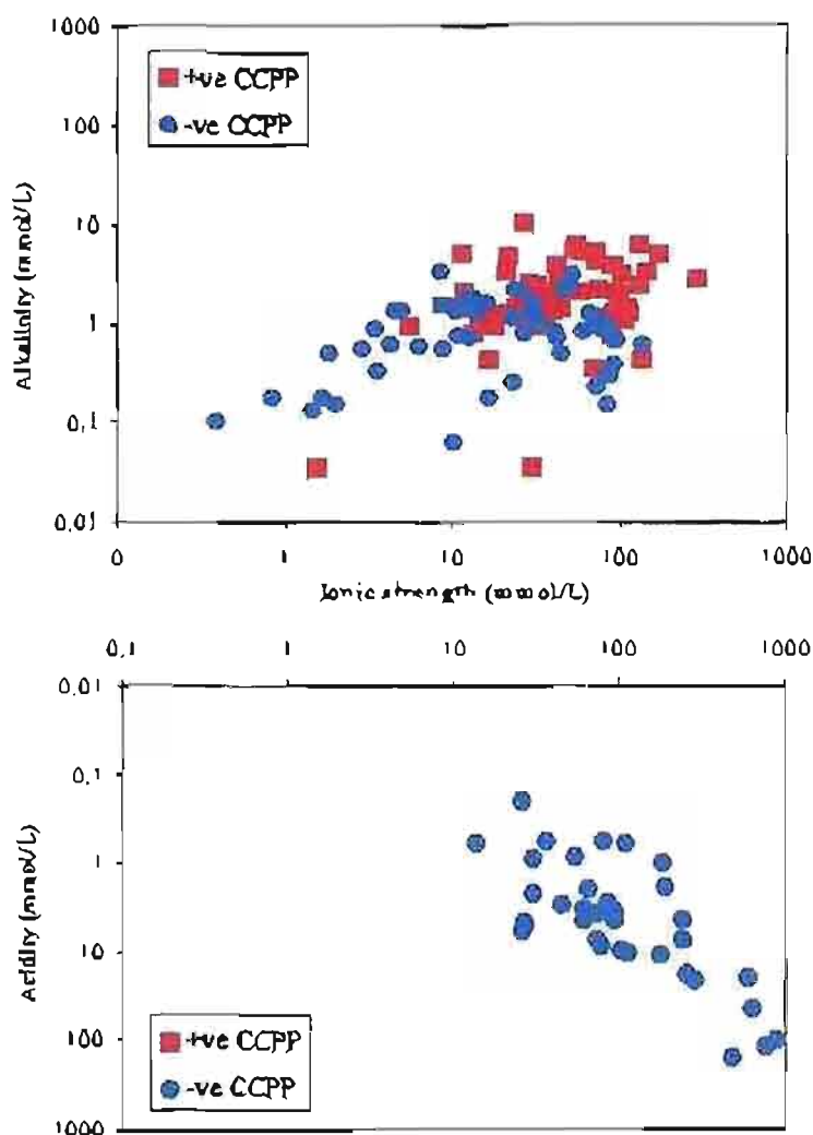
Figure 6.8: Corrosivity of waters in this study as a function of net alkalinity and solinity.
