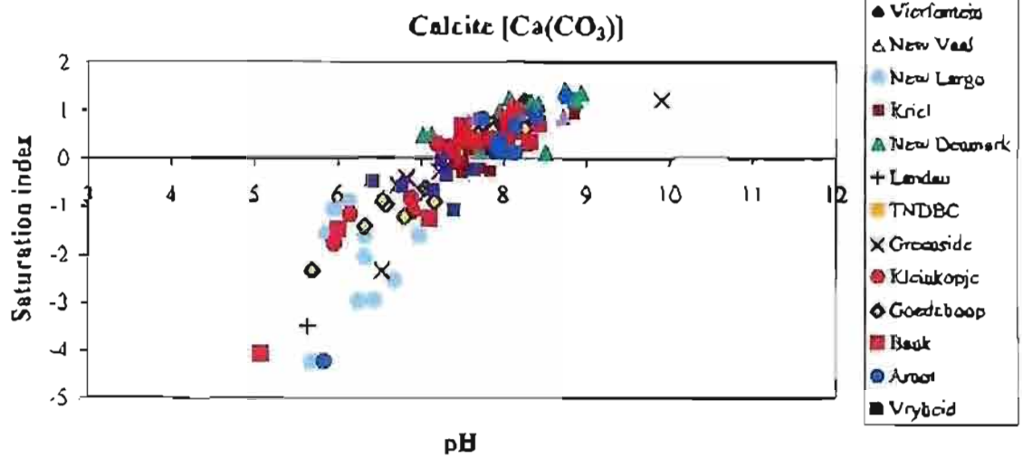
Figure 3.55: Saturation index of calcite as a function of pH for the colliery waters.
