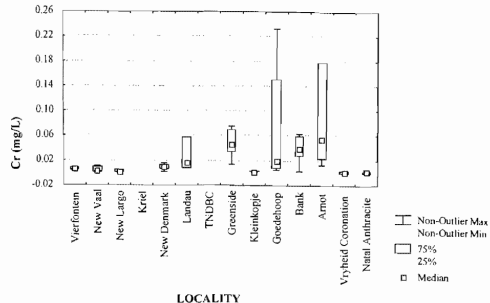
Figure 3.19: Chromium concentration of water samples from Highveld collieries ( n=117 ).
