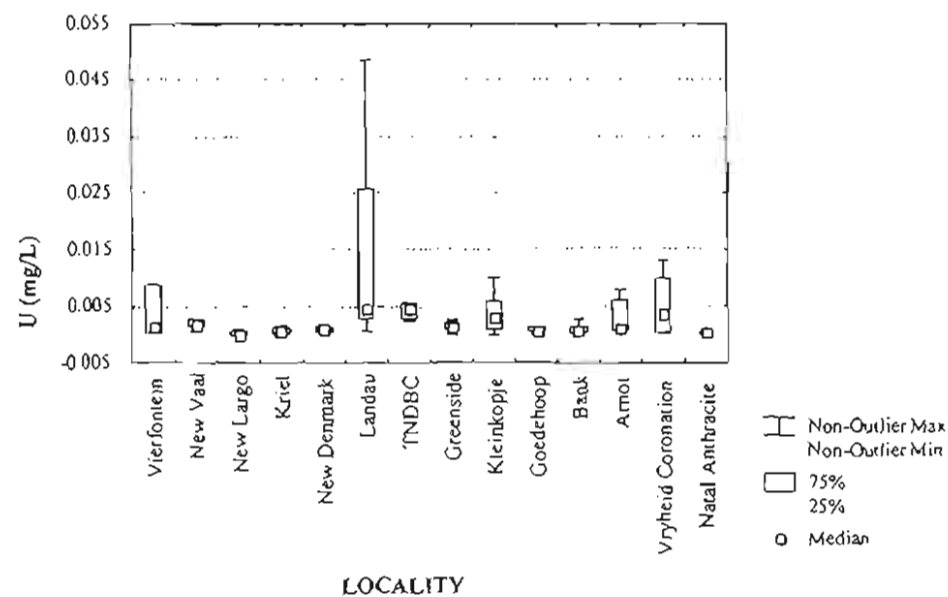
Figure 3.36a: Uranium concentration of water samples from Highveld collieries (n=16).
