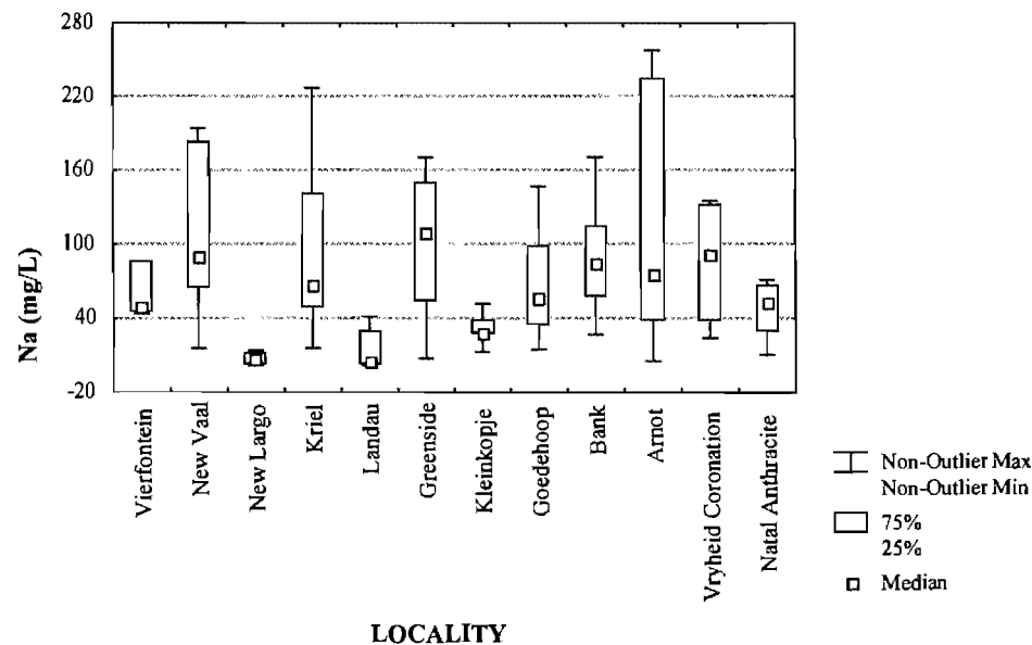
Figure 3.4b: Sodium concentration of water samples from Highveld collieries, excluding New Denmark and TNDBC.
