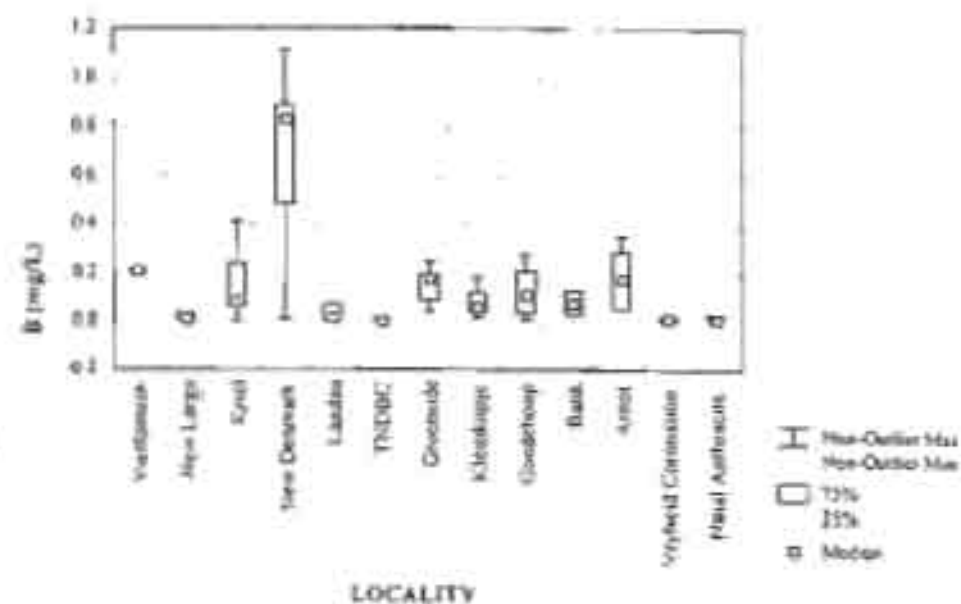
Figure 3.16b: Boron concentration of water samples from Highveld collieries, excluding New Vaal.
