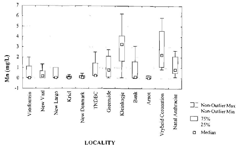
Figure 3.20b: Manganese concentration of water samples from Highveld collieries, excluding Landau & Goedeheop.
