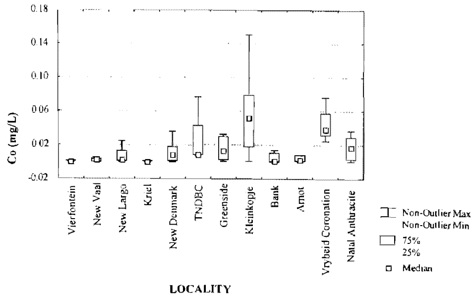
Figure 3.21b: Cobalt concentration of water samples from Highveld collieries, excluding Landau and Goedeheop.
