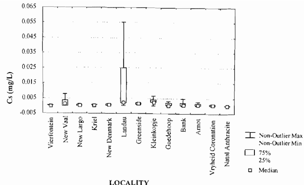
Figure 3.33b: Cesium concentration of water samples from Highveld collieries, excluding TNDBC.
