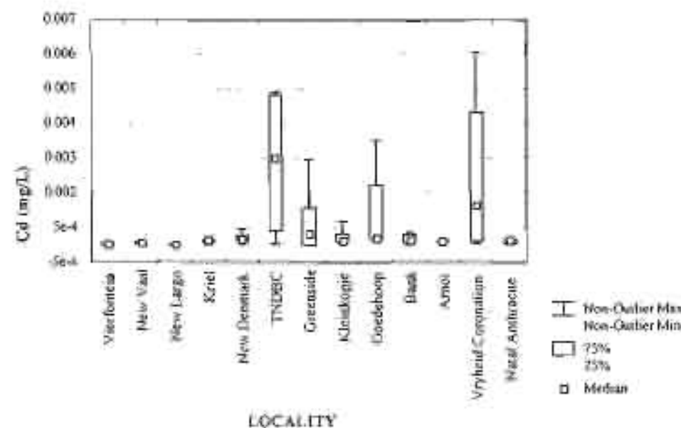
Figure 3.32b: Cadmium concentration of water samples from Highveld collieries, excluding Landau.
