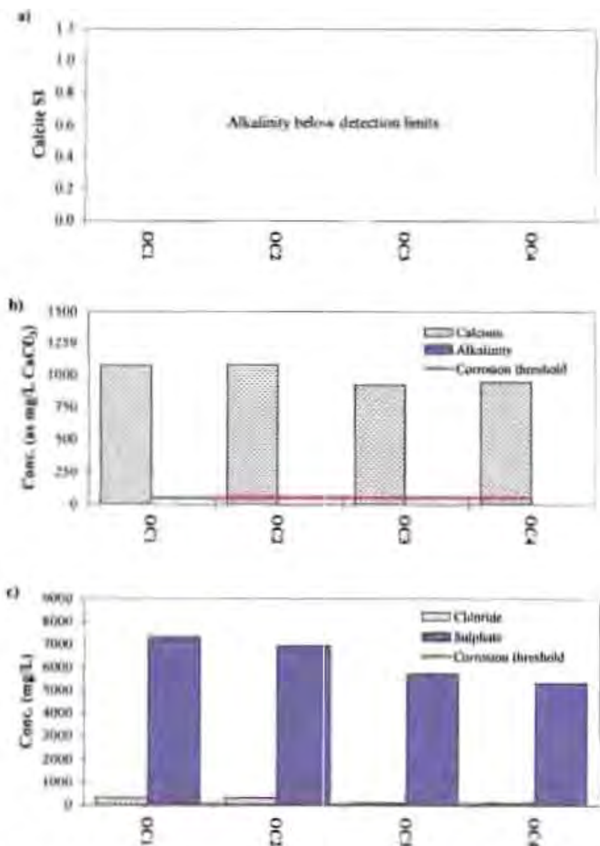
Figure A6.14: (a) Calcite saturation index of TNDBC waters. For corrosion prevention, SI \leq 0 (Lacwenhul, 1986). (b) Calcium and alkalinity concentrations of TNDBC waters. Both calcium and alkalinity concentrations should exceed 50mg/L ( \text{CaCO}_3 equivalent) for the prevention of corrosion (Lacwenhul, 1986). (c) Chloride and sulphate concentration of TNDBC waters. If chloride or sulphate concentration exceeds 30mg/L the waters will corrode metal surfaces (Lacwenhul, 1986).
