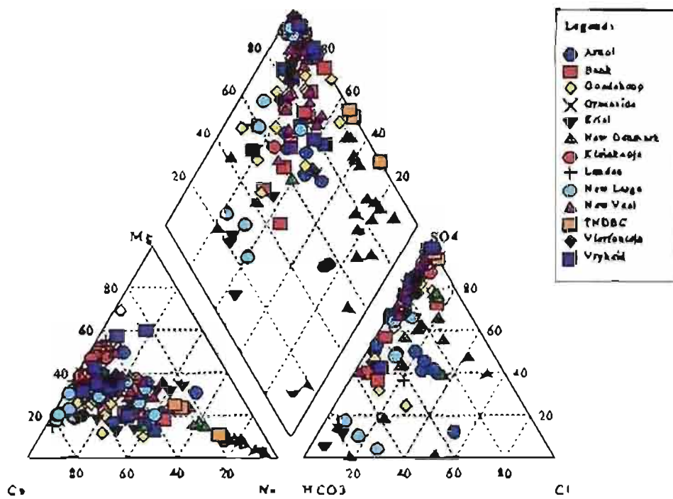
Figure 6.3: Piper (ternary) diagram of major ions in colliery waters.
