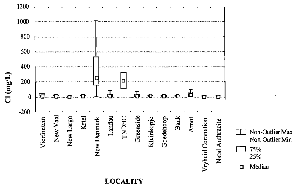
Figure 3.10a: Chloride concentration of water samples from Highveld collieries (n=167).
