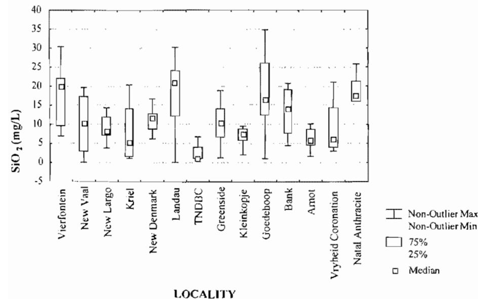
Figure 3.18: Silica concentration of water samples from Highveld collieries ( n=164 ).
