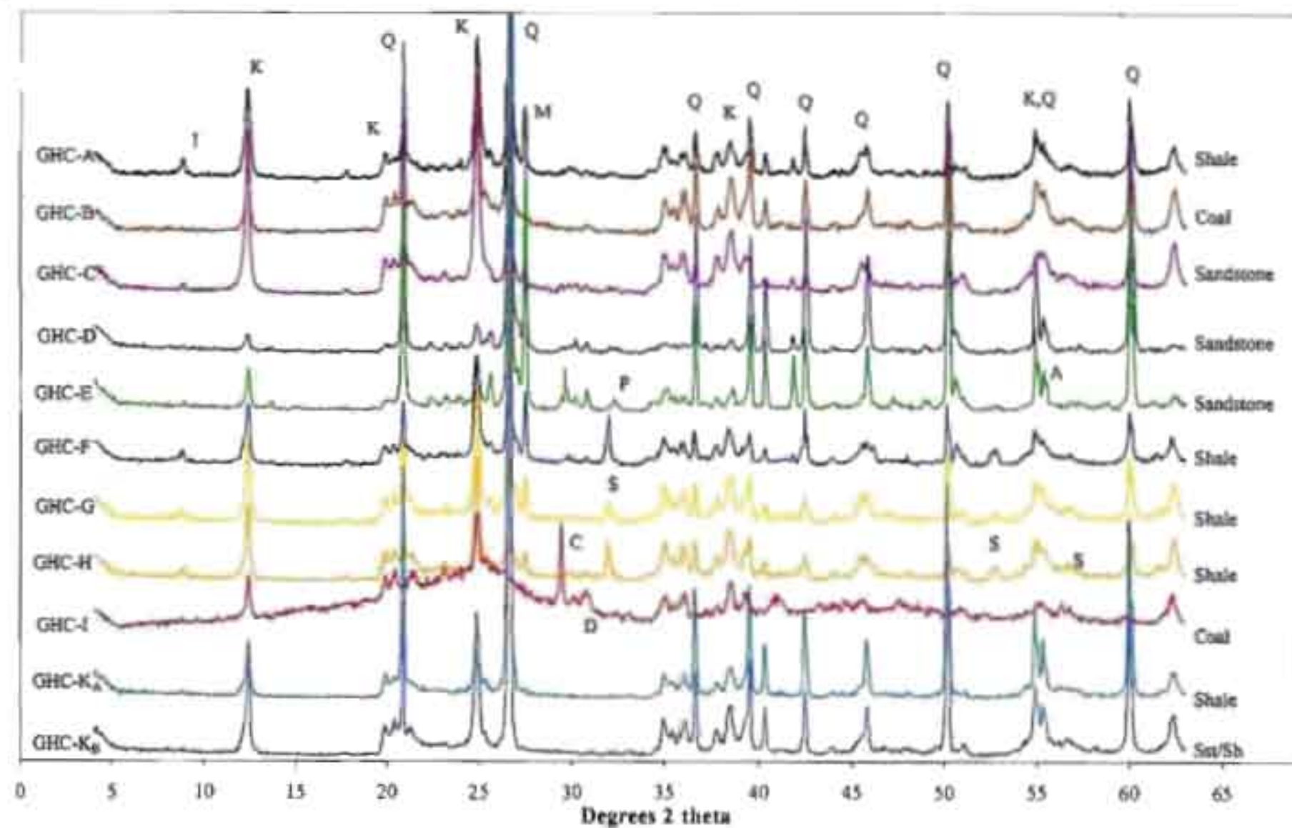
Figure A.5.4: Stacked XRD po P =pyrite and M =microcline.
