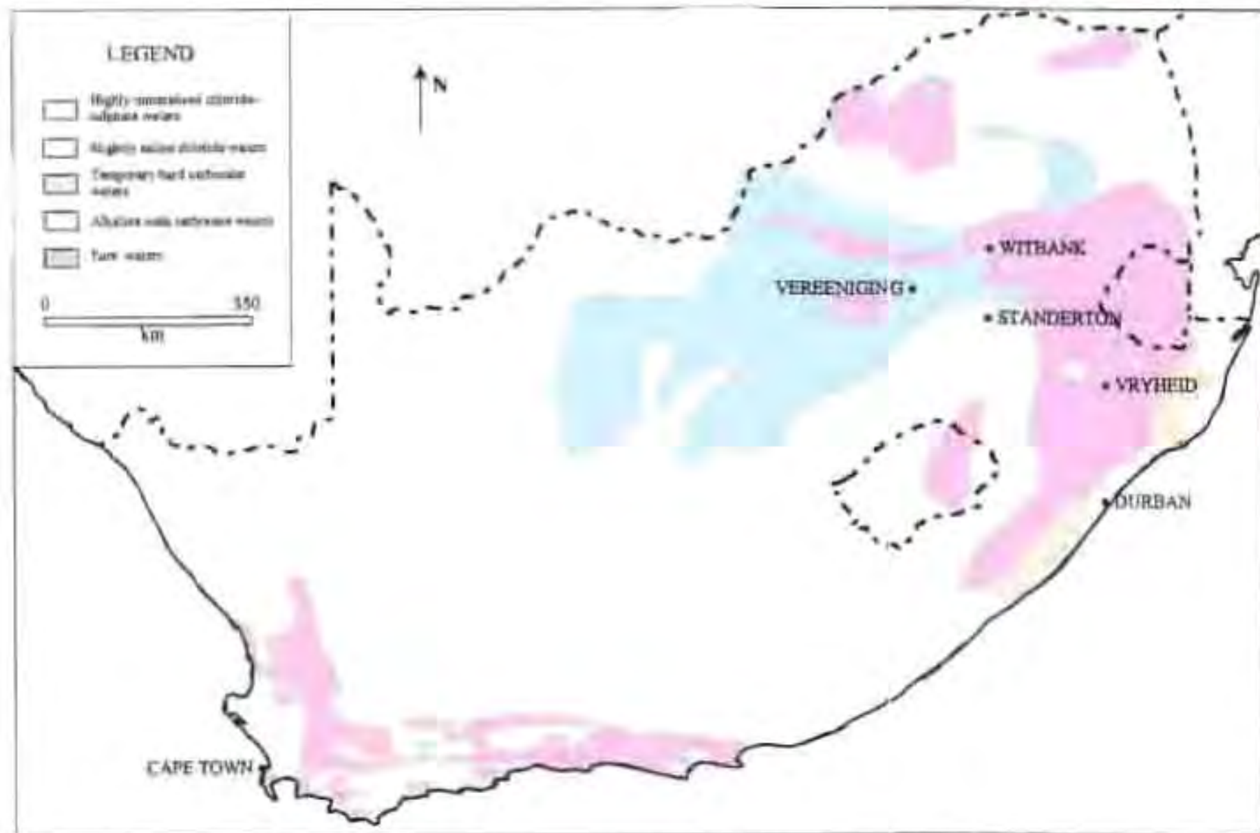
Figure 3.47: Water map of the Union of South Africa showing baseline water compositions. Compiled by Blom (1943).
