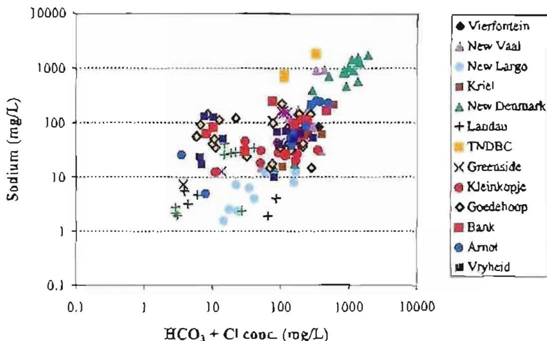
Figure 3.52: Correlation observed between sodium and \text{HCO}_3^- + \text{Cl}^- concentration ( r_s=0.693 ).
