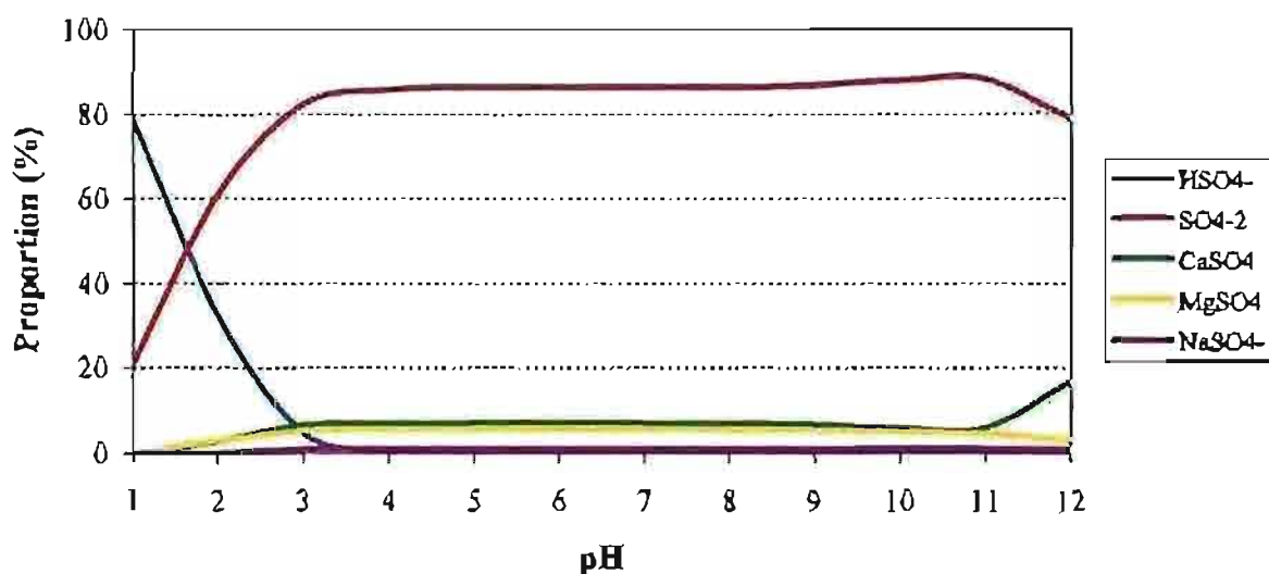
Figure 3.50: Ion speciation changes as a function of pH for a sample from Kriel colliery (KCBs).
