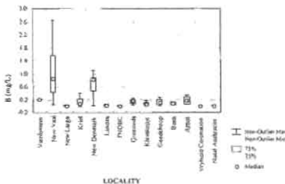
Figure 3.16a: Boron concentration of water samples from Highveld collieries ( n=13 ).
