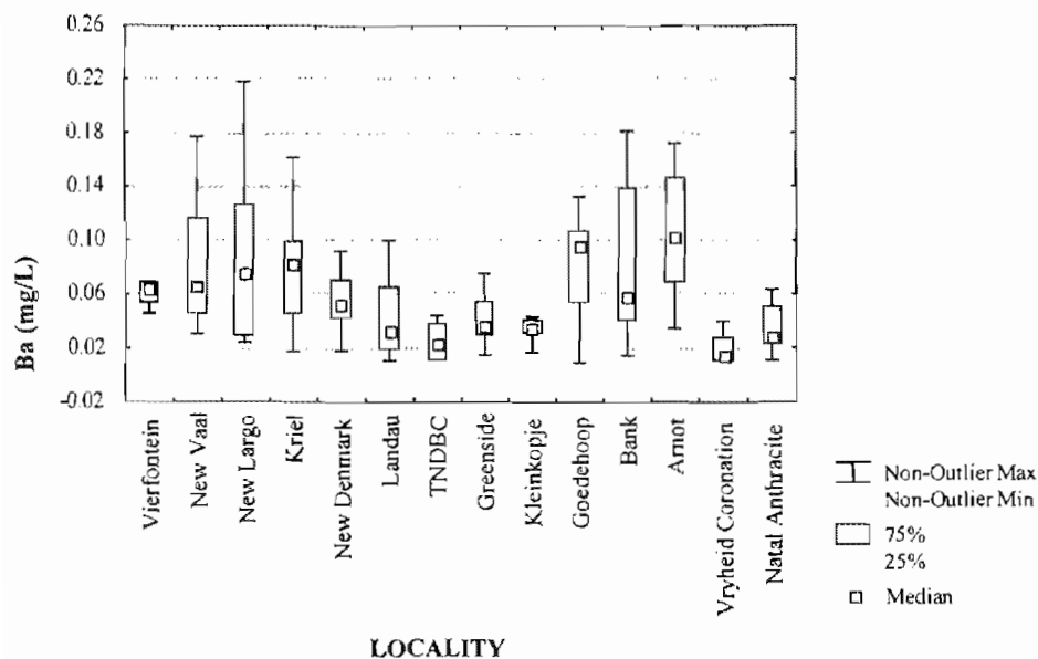
Figure 3.34: Barium concentration of water samples from Highveld collieries (n=166).
