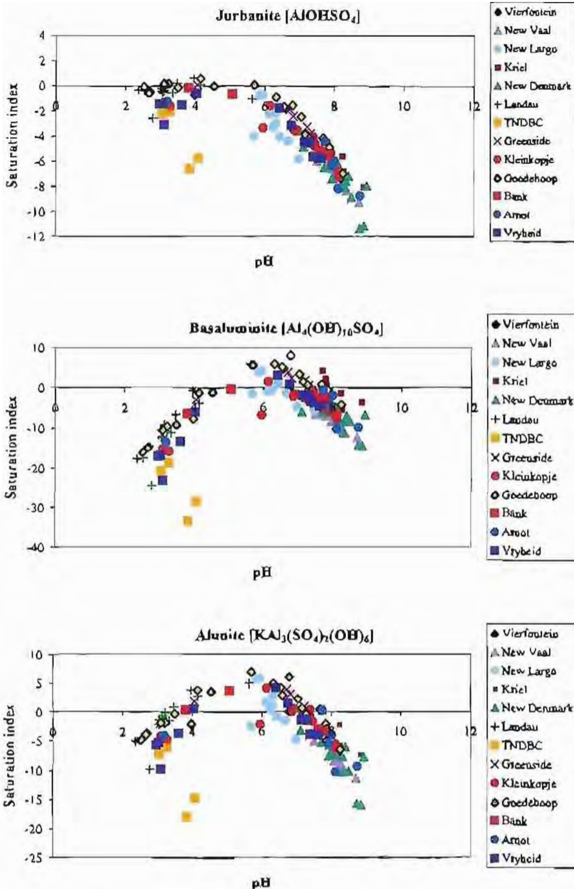
Figure 3.61 cont.: Saturation indices for selected aluminium-bearing minerals as a function of pH for the colliery waters.
