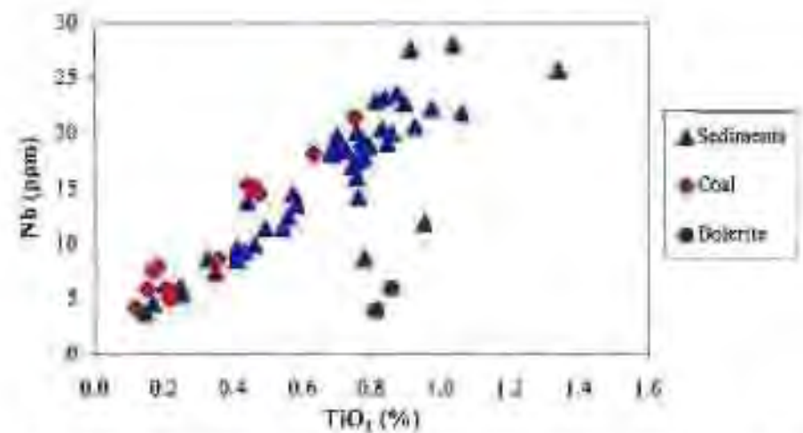
Figure 4.9: Relationship between niobium and titanium concentration in selected lithological units
