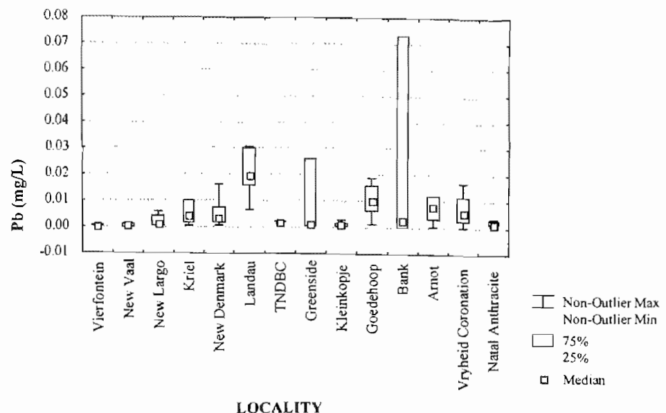
Figure 3.35: Lead concentration of water samples from Highveld collieries (n=134).
