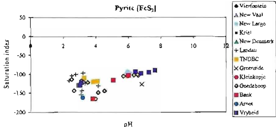
Figure 3.63: Saturation indices of selected iron-bearing minerals as a function of pH for the colliery waters.
