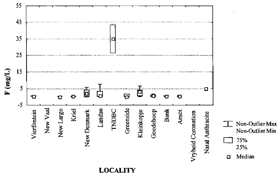
Figure 3.9a: Fluoride concentration of water samples from Highveld collieries (n=101).
