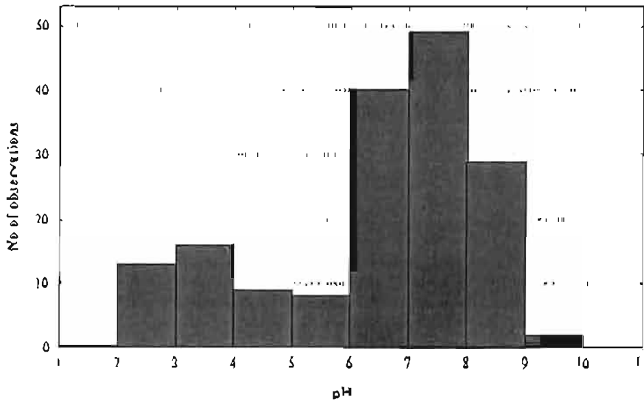
Figure 3.37: Bimodal pH distribution of water samples from 167 sites on 14 Highveld collieries.
