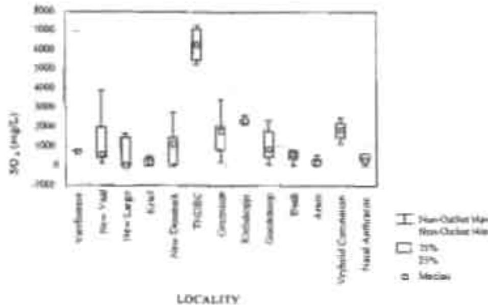
Figure 3.12a: Sulfate concentration of water samples from Highveld collieries (n=105).
