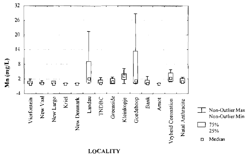
Figure 3.20a: Manganese concentration of water samples from Highveld collieries (n=167).
