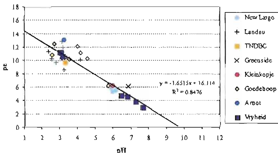
Figure 3.49: Relationship between pe and pH for waters containing the \text{Fe(II) / Fe(III)} pair.
