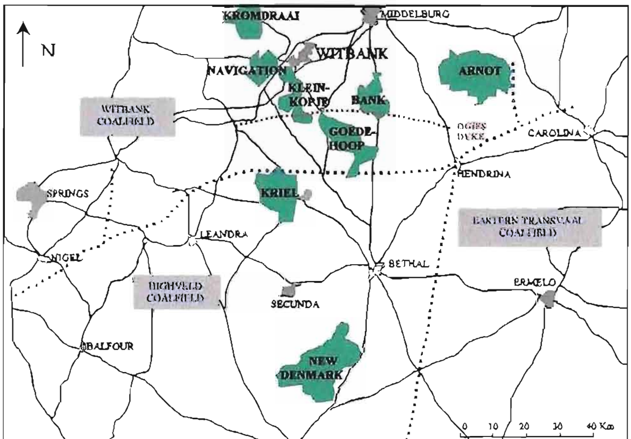
Figure 4.3: Highbveld and Witbank coalfields, showing location of the New Lorgo, Kriel, New Denmark, Landou (Navigation + Kromdraai), TNDBC, Greenside, Kleinkopje, Goedehoop, Bank and Arnot collieries (After Barker, 1999).
