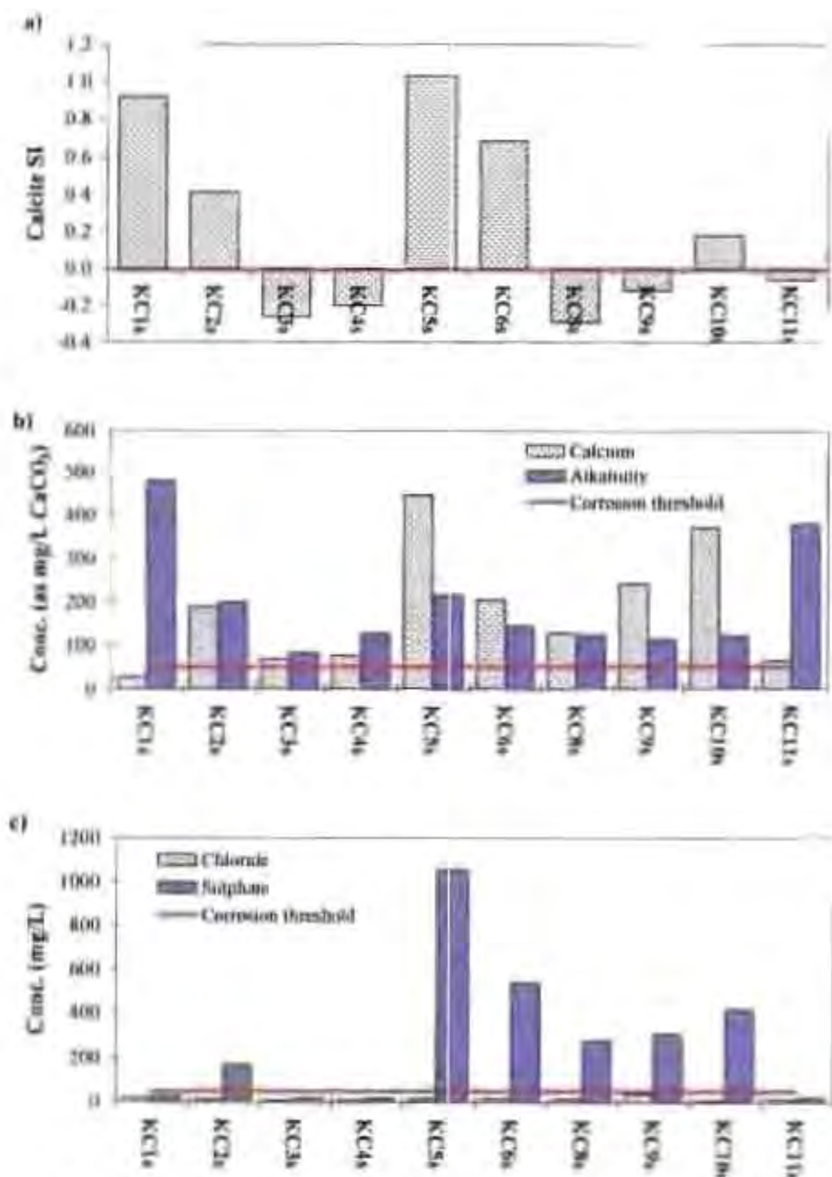
Figure 46.8: (a) Calcium saturation index of Kriel waters. For corrosion prevention, SI \geq 0 (Lewyenthal, 1986). (b) Calcium and alkalinity concentrations of Kriel waters. Both calcium and alkalinity concentration should exceed 50\text{mg/L} ( \text{Ca}^{2+}\text{O}_2 equivalent) for the prevention of corrosion (Lewyenthal, 1986). (c) Chloride and sulphate concentration of Kriel waters. If chloride or sulphate concentration exceeds 50\text{mg/L} , the waters will corrode metal surfaces (Lewyenthal, 1986).
