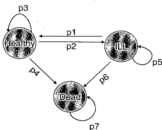
A Markov-state diagram adopted from Sonnenberg and Beck (1993)
