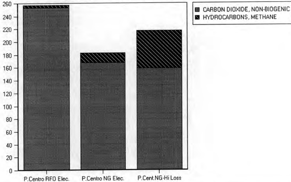
Figure 5.8: Greenhouse Gas Emissions by Gas, IPCC 100 Year Integration (Kg CO 2 Equivalent per GJ Final Energy)
