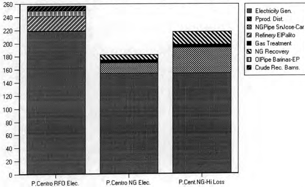
Figure 5.7: Greenhouse Gas Emissions by Stage, IPCC 100 Year Integration (kg CO 2 Equivalent per GJ Final Energy)
