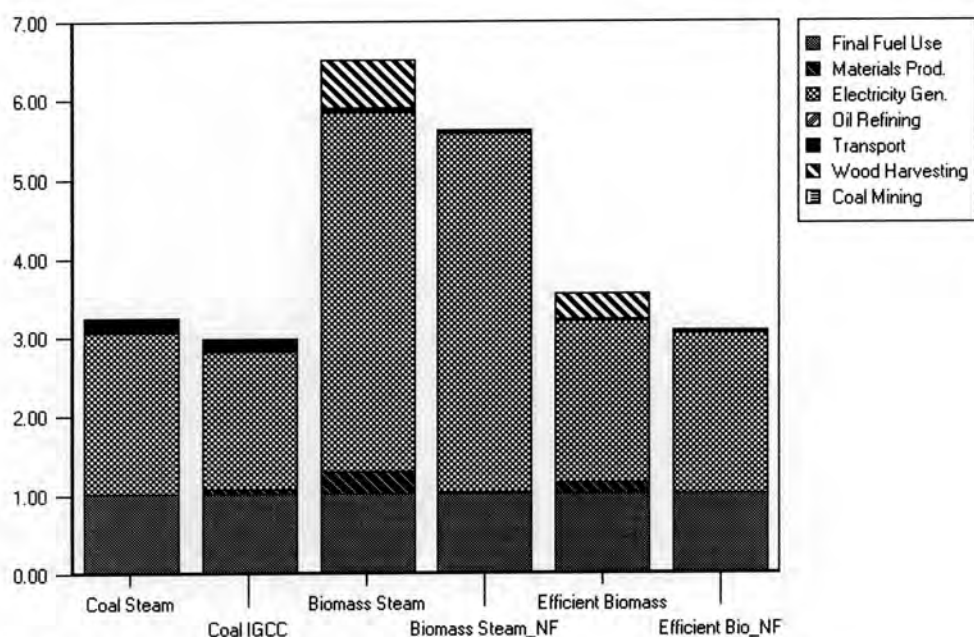
Figure 4.5: Net Energy Use: Stage By Fuel Chain (GJ per GJ Final Energy)
