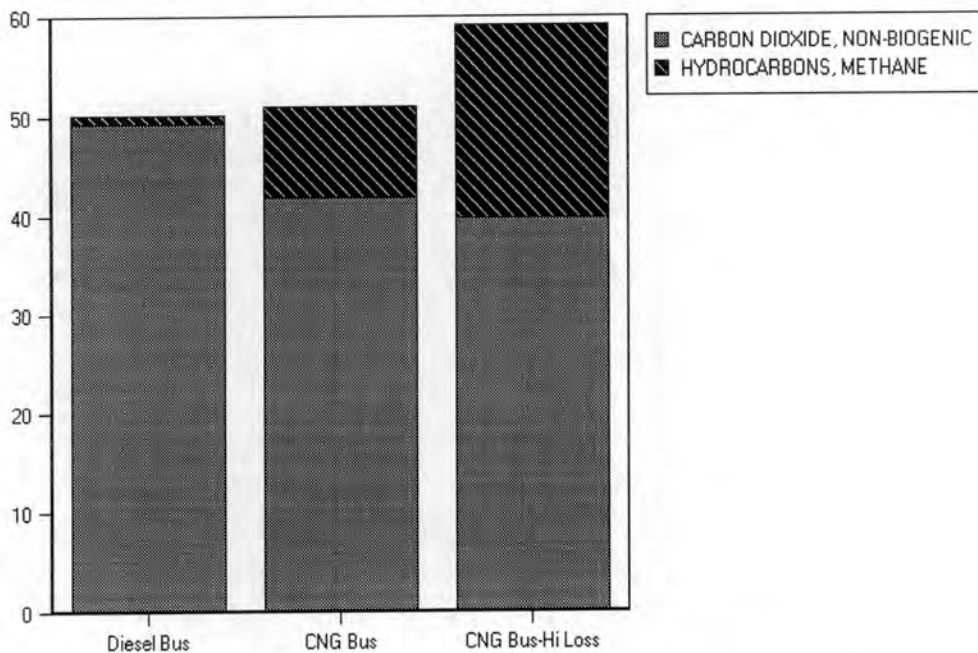
Figure 5.11: Greenhouse Gas Emissions by Gas, IPCC 100 Year Integration (Tonnes CO 2 Equivalent per Million Passenger-KM)
