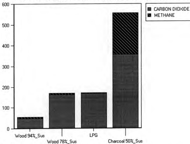
Figure 4.8: Net Global Warming Potential of Selected Household Fuel Chains in Sri Lanka (Tonnes CO 2 Equivalent per Thousand GJ Useful Energy)
