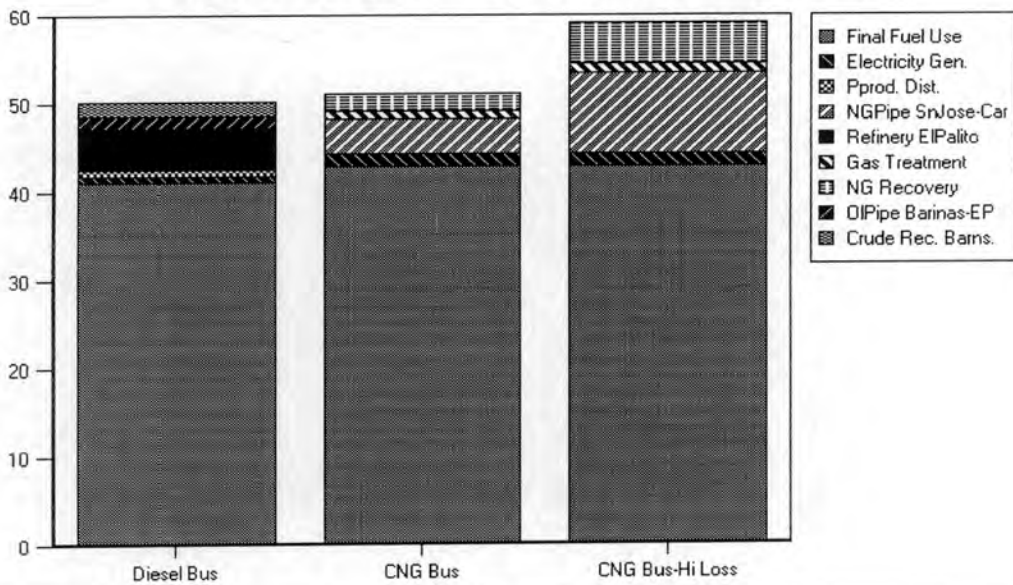
Figure 5.10: Greenhouse Gas Emissions by Stage, IPCC 100 Year Integration (Tonnes CO 2 Equivalent per Million Passenger-KM)
