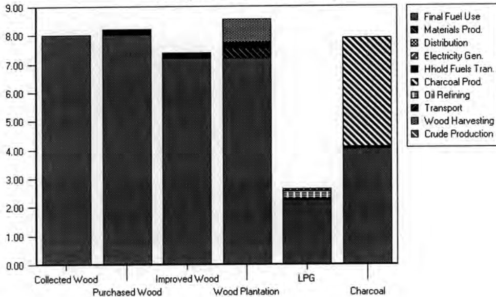
Figure 4.6: Final and Upstream Fuel Use for Selected Household Fuel Chains (GJ per GJ Useful Energy)
