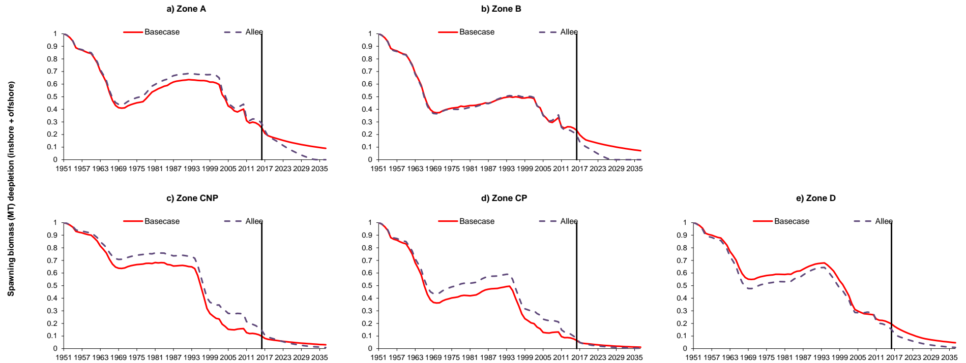
Figure 3. Total (inshore + offshore) depletion trajectories shown for Zones A to D for the Updated Basecase model compared to sensitivity test that takes an Allee effect into account. Note that the 20-yr projections shown (after the vertical bar) represent scenarios under which future poaching levels are assumed to remain at the current estimated level (average of 2015 and 2016) and future commercial catches are set to 25 tons in each of Zones A and B only.
