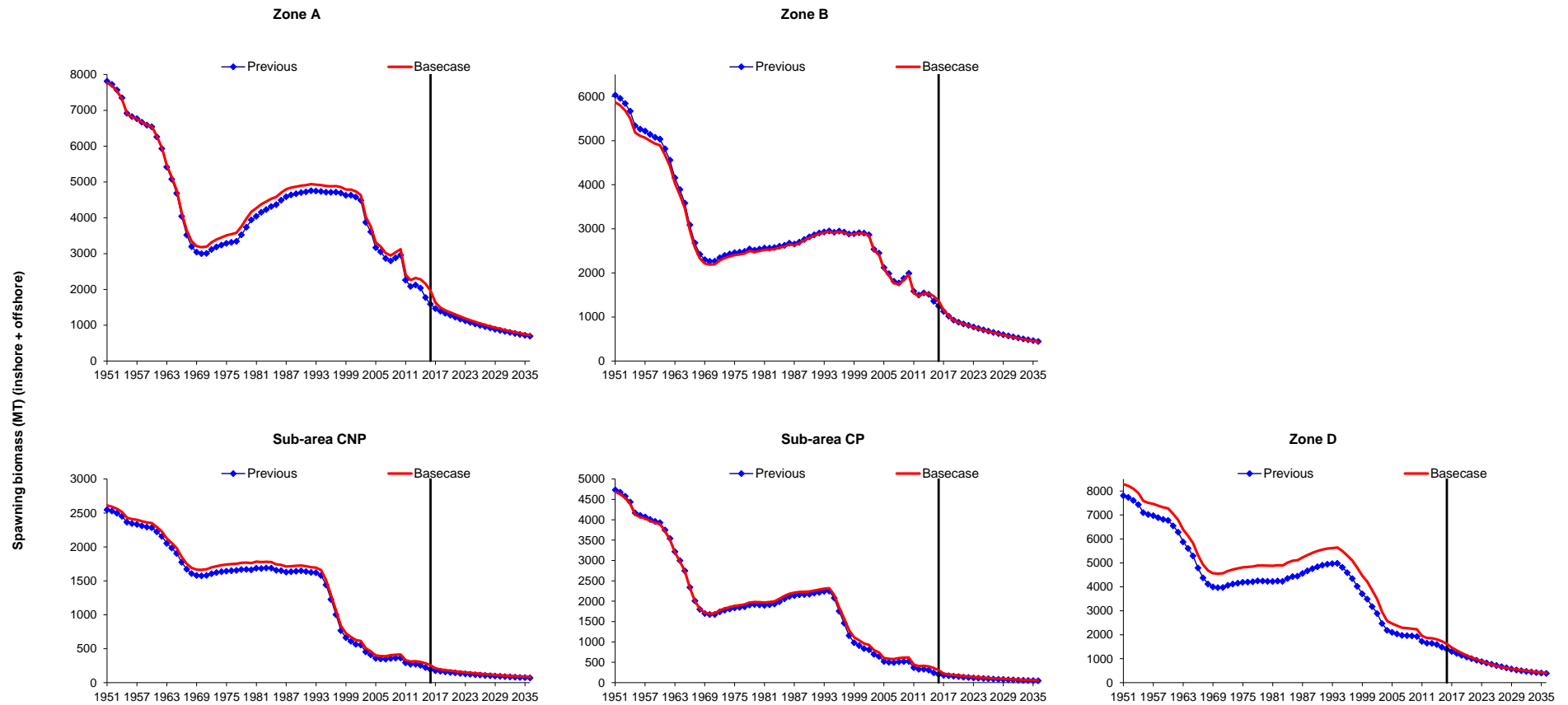
Figure 1. Total (inshore + offshore) spawning biomass trajectories shown for Zones A to D for the Updated Basecase model compared to the “Previous” results obtained in the 2015 assessment. Note that the 20-yr projections shown (after the vertical bar) represent scenarios under which future poaching levels are assumed to remain at the “current” estimated values (average of 2014 and 2015 for the “Previous” model and the average of 2015 and 2016 for the “Basecase”) and future CNP commercial catches are set to 25 tons in each of Zones A and B only.
