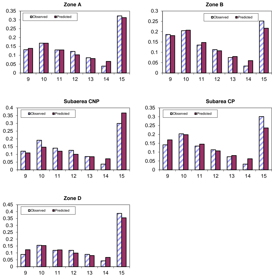
Figure A6. Comparison for the average over all the years between observed and model predicted catch-at-age proportions for the commercial sector for Zones A to D for the Updated Basecase model.
