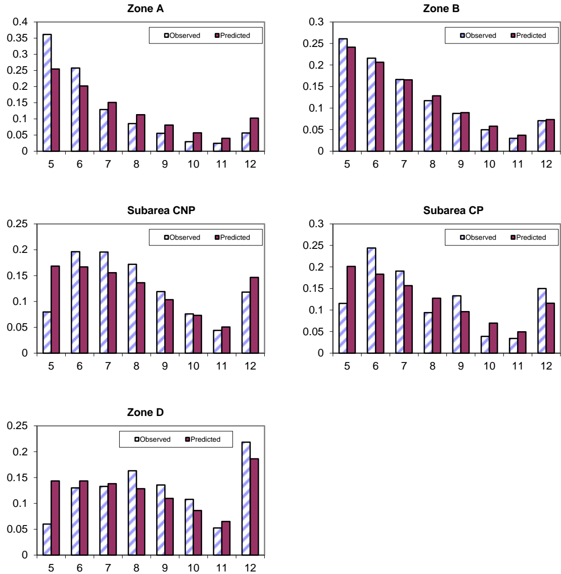
Figure A9. Comparison for the average over all the years between observed and model predicted catch-at-age proportions for the FIAS inshore survey data for Zones A to D for the Updated Basecase model.
