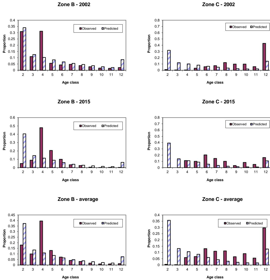
Figure A10. Comparison between observed and model predicted catch-at-age proportions for the full population survey data for Zones B and C for the Updated Basecase model.
