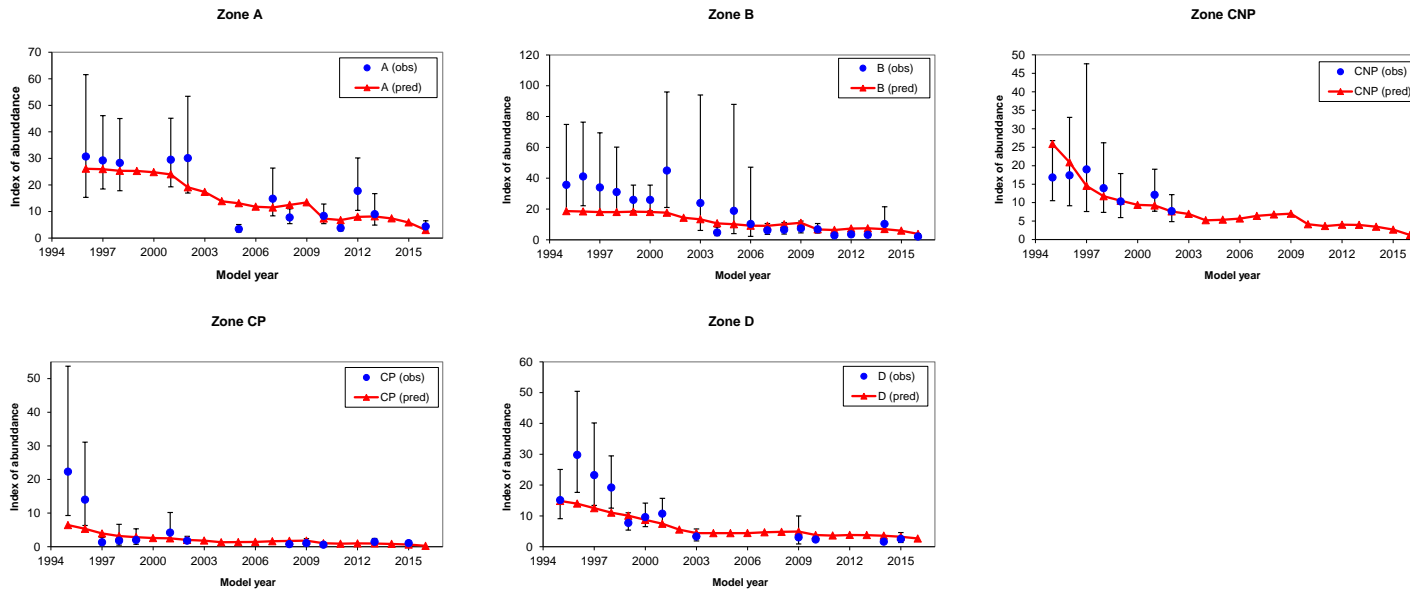
Figure A4. Comparison of observed FIAS and model-predicted trends for the Updated Basecase model for Zones A to D. Note that the 95% confidence intervals shown have been computed as: \text{estimate} \cdot \exp(\pm 1.96 \cdot \text{CV}) .
