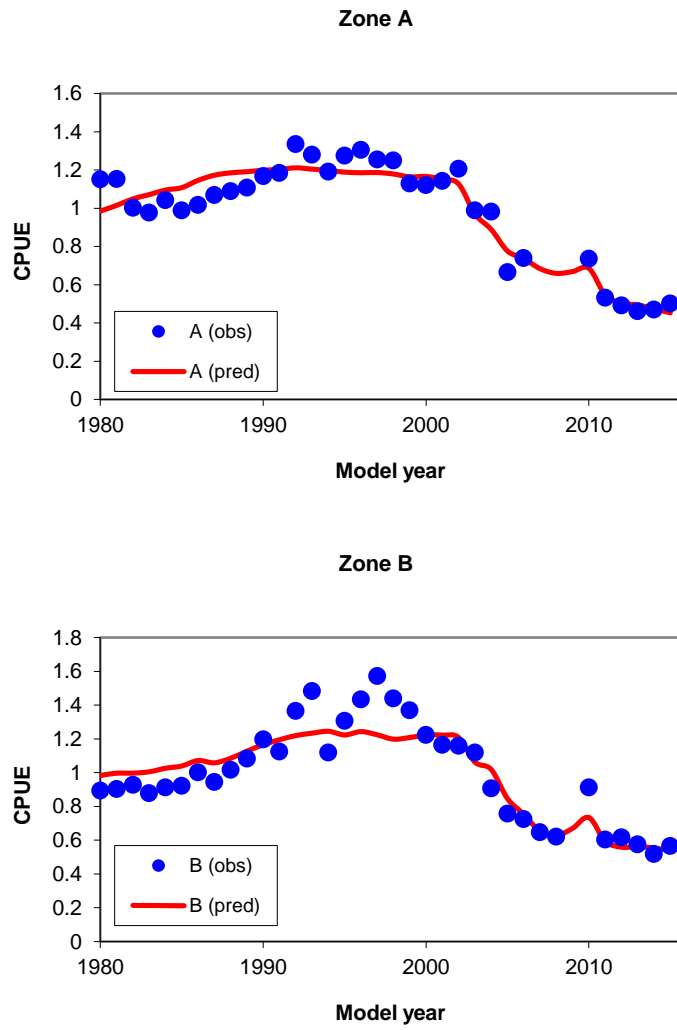
Figure A3. Comparisons between the standardised CPUE (obs) and model-predicted CPUE values for the Updated Basecase for Zones A and B.
