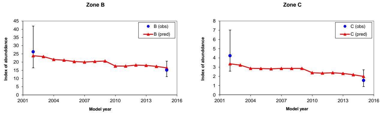
Figure A5. Comparison of observed extractive survey and model-predicted values and trends for the Updated Basecase model for Zones B and C. Note that the 95% confidence intervals shown have been computed as: estimate*exp( \pm 1.96 *CV).
