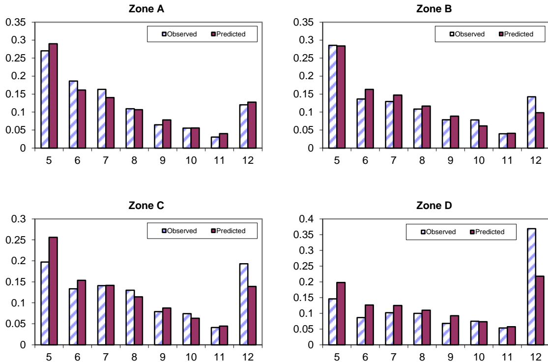
Figure A8. Comparison for the average over all the years between observed and model predicted catch-at-age proportions for the poaching sector for Zones A to D for the Updated Basecase model.
