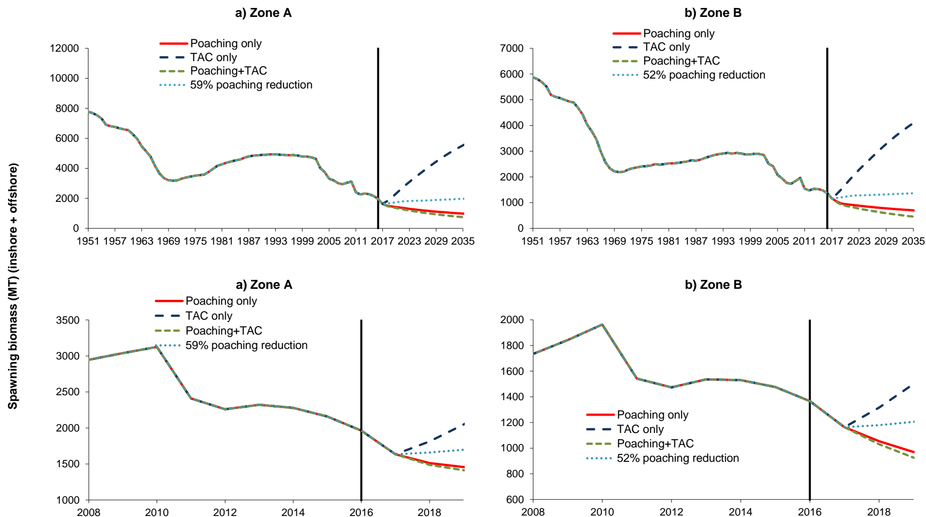
Figure 4. Total (inshore + offshore) spawning biomass trajectories shown for Zones A and B for the Updated Basecase model. The 20-yr projections shown (after the vertical bar) represent four different scenarios for future commercial and poaching catches. Unless a zero amount is assigned, future poaching levels are assumed to remain at the current estimated level (average of 2015 and 2016) and future commercial catches in each of these two Zones are set to the current TAC of 25 tons. The bottom plots zoom in on a shorter period to be able to distinguish the curves more clearly. In each plot, the required reduction in poaching necessary to keep the resource stable at its present level under the current TAC is also shown, with the required reduction indicated in the legend.
