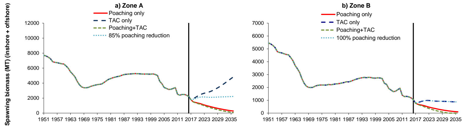
Figure 5. Total (inshore + offshore) spawning biomass trajectories shown for Zones A and B for the Updated Basecase model taking an Allee effect into account. The 20-yr projections shown (after the vertical bar) represent four different scenarios for future commercial and poaching catches. Unless a zero amount is assigned, future poaching levels are assumed to remain at the current estimated level (average of 2015 and 2016) and future commercial catches are set to the current TAC of 25 tons. In each plot, the required reduction in poaching necessary to keep the resource stable at its present level under the current TAC is also shown, with the required reduction indicated in the legend.
