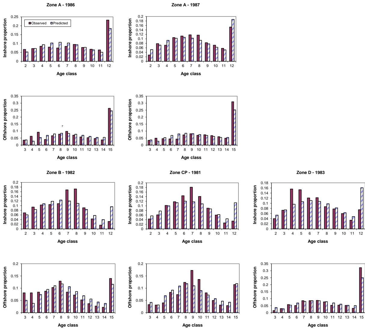
Figure A11. Comparison between observed and model predicted catch-at-age proportions for the “old” inshore and offshore survey data for Zones A to D for the Updated Basecase model.
