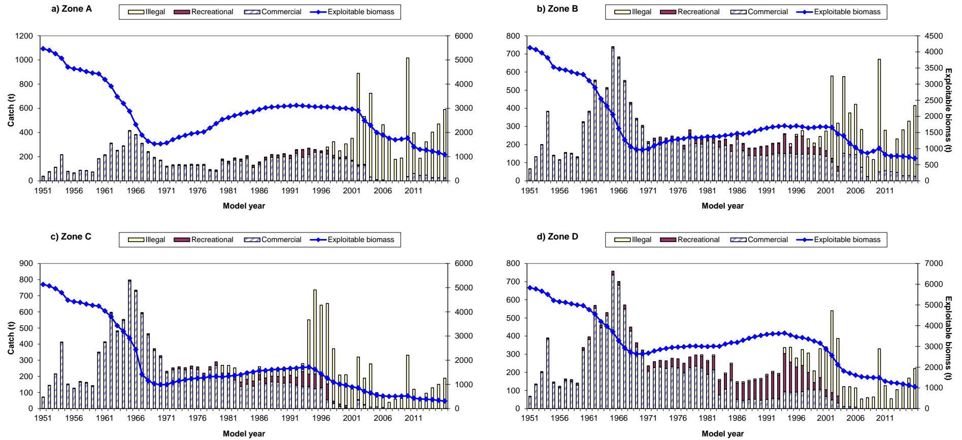
Figure A1. Estimated commercial exploitable biomass for the Updated Basecase model for Zones A to D (right hand axis) in tons and total catches (commercial + recreational + estimated illegal) for the Zones (left hand axis).
