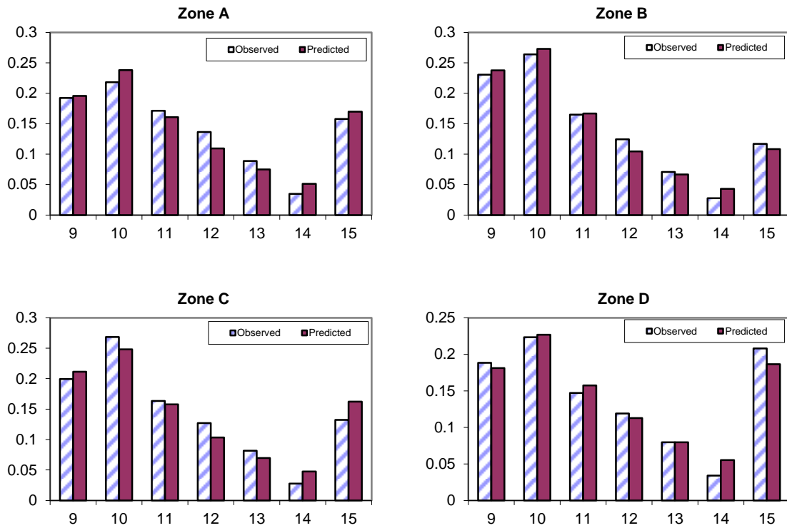
Figure A7. Comparison for the average over all the years between observed and model predicted catch-at-age proportions for the recreational sector for Zones A to D for the Updated Basecase model.
