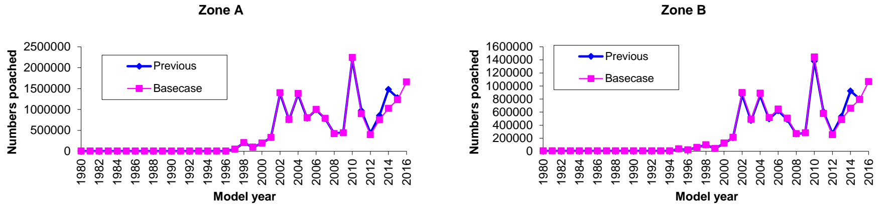
Figure 2. Comparison of model-predicted numbers of abalone poached for Zones A and B for the Updated Basecase model and those obtained in the 2015 assessment (“Previous”).
