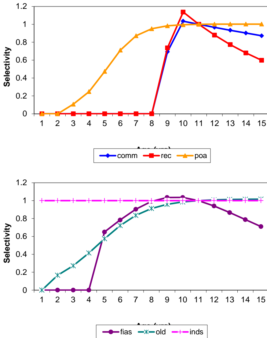
Figure A2. Plots of the Updated Basecase model selectivity functions estimated for the commercial (comm), recreational (rec) and poaching (poa) fishery sectors, and for FIAS (fias) and the old 1980's surveys (old). A uniform value is assumed for the full population surveys (inds) because of the extractive nature of the sampling methodology used.
