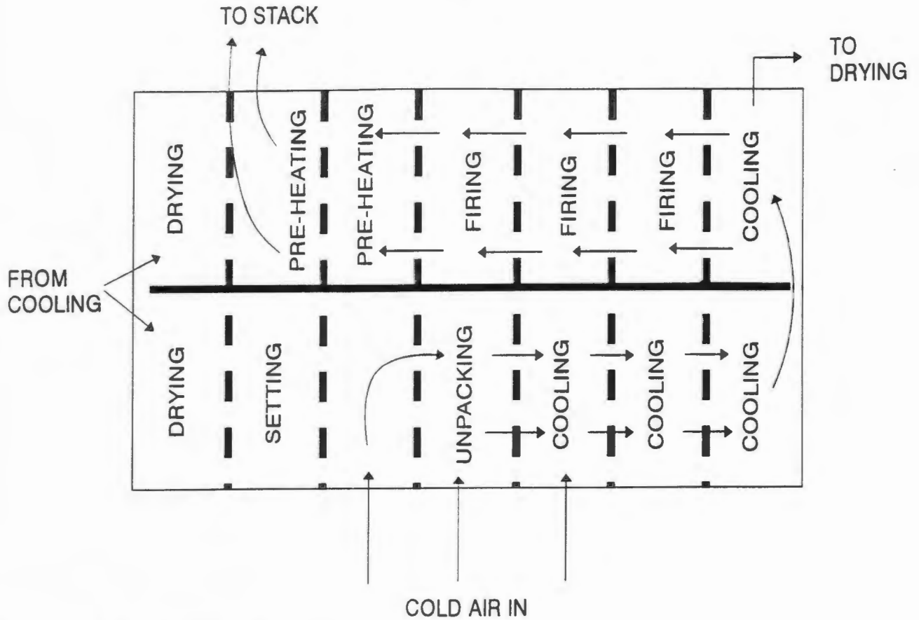
Figure 10. The Tunnel Kiln
