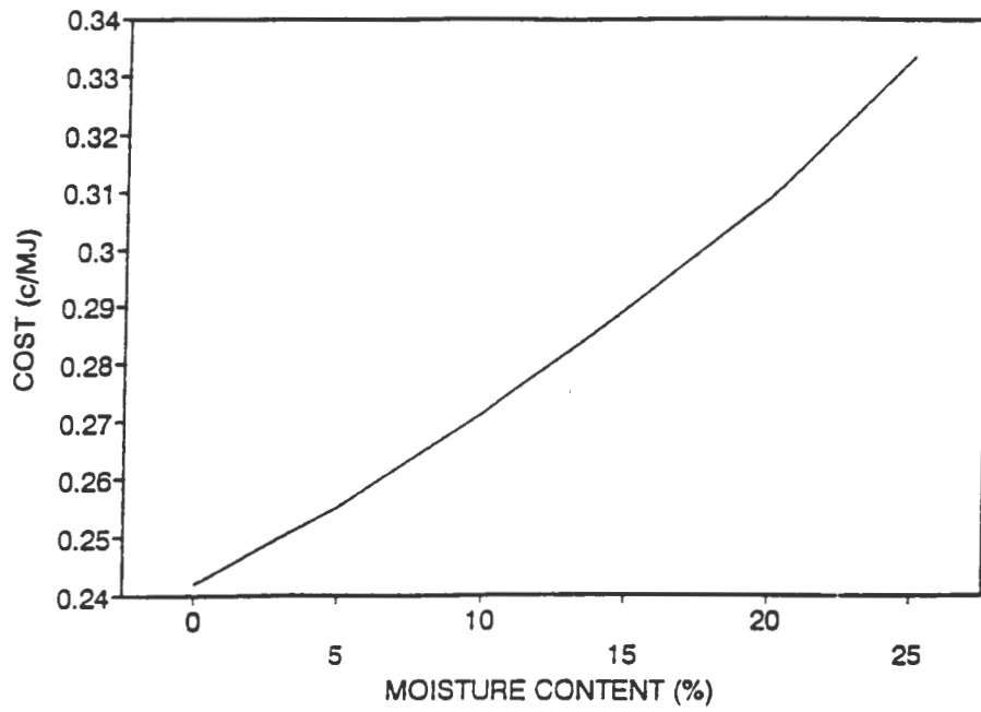
Figure D2.2 Cost per unit energy vs moisture content
