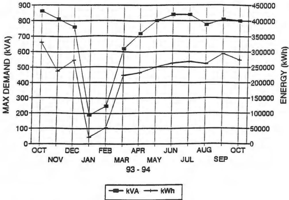
Figure 3. Electricity consumption
