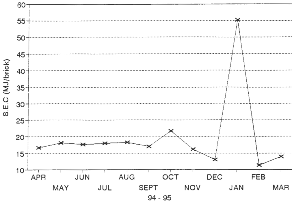
Figure 3. Specific Energy Consumption
