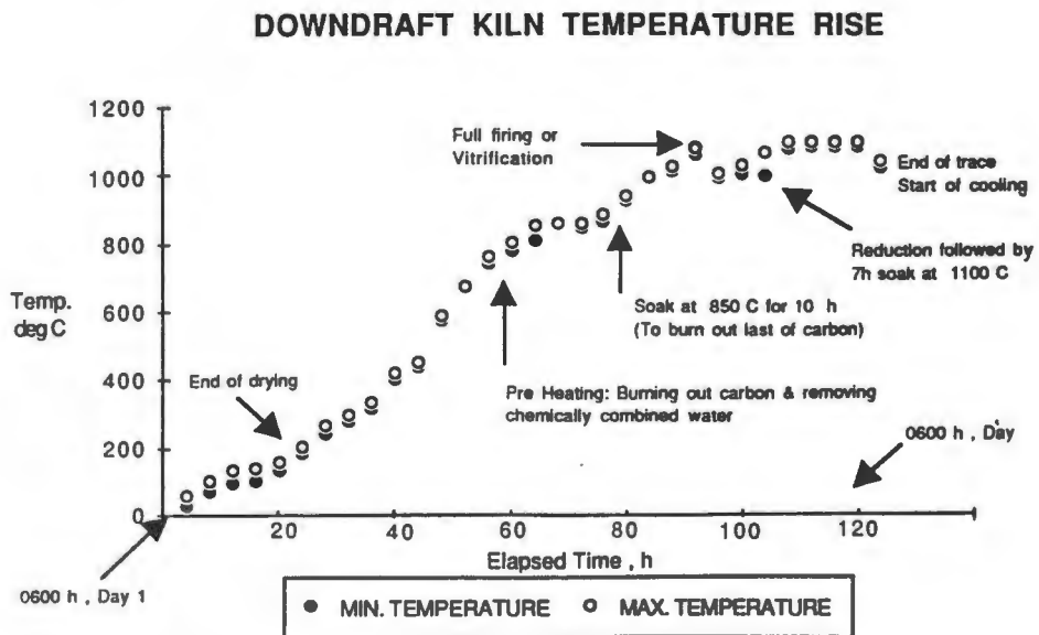
Figure 12. Typical firing cycle for Downdraught Kiln (12)
