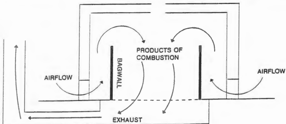
Figure 7. Downdraught Kiln
