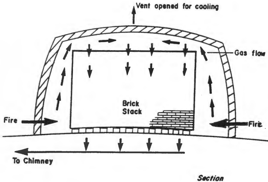
Figure 11. The Downdraught Kiln (12)
