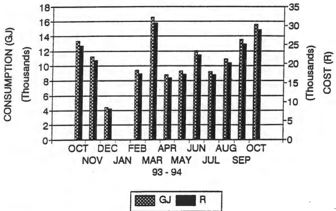
Figure 5. Duff coal consumption
