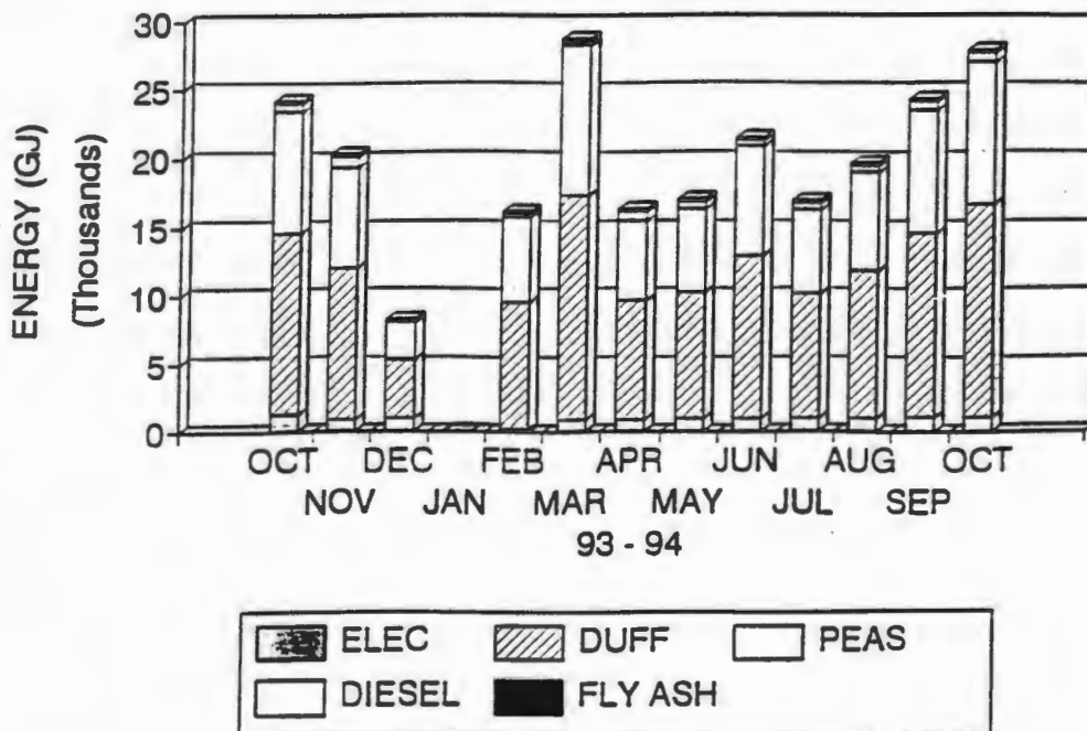
Figure 8. Total energy use per month
