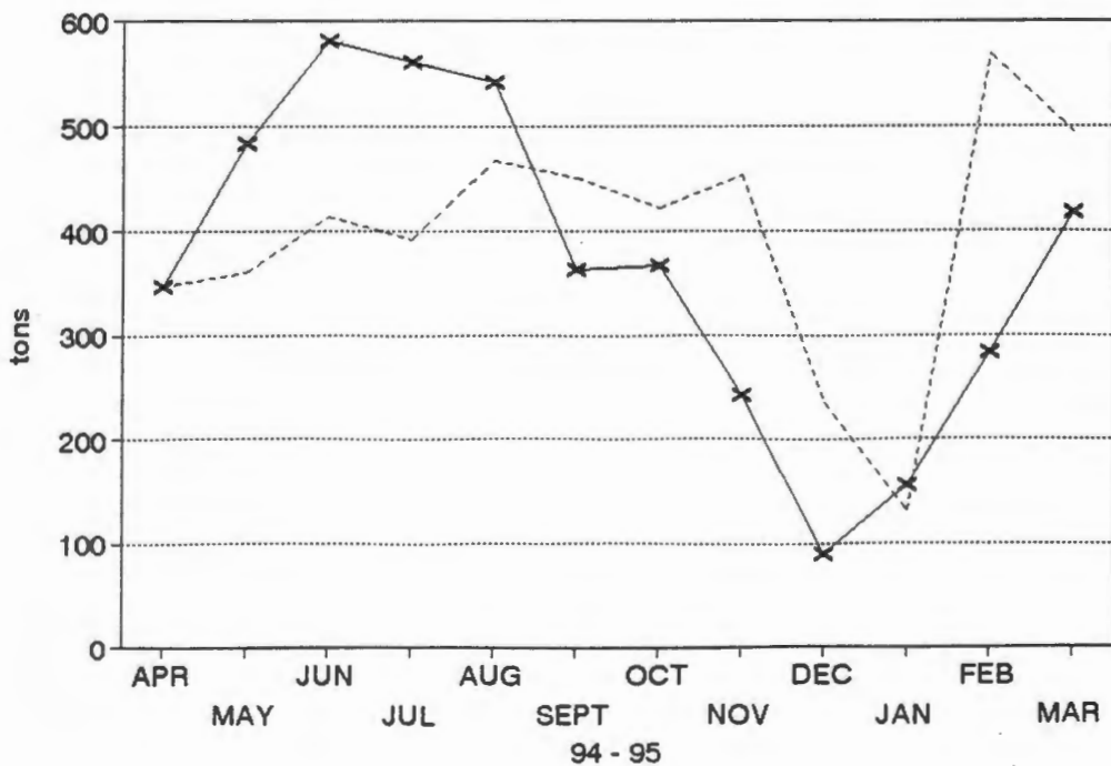
Figure 2. Coal cobbles consumption
