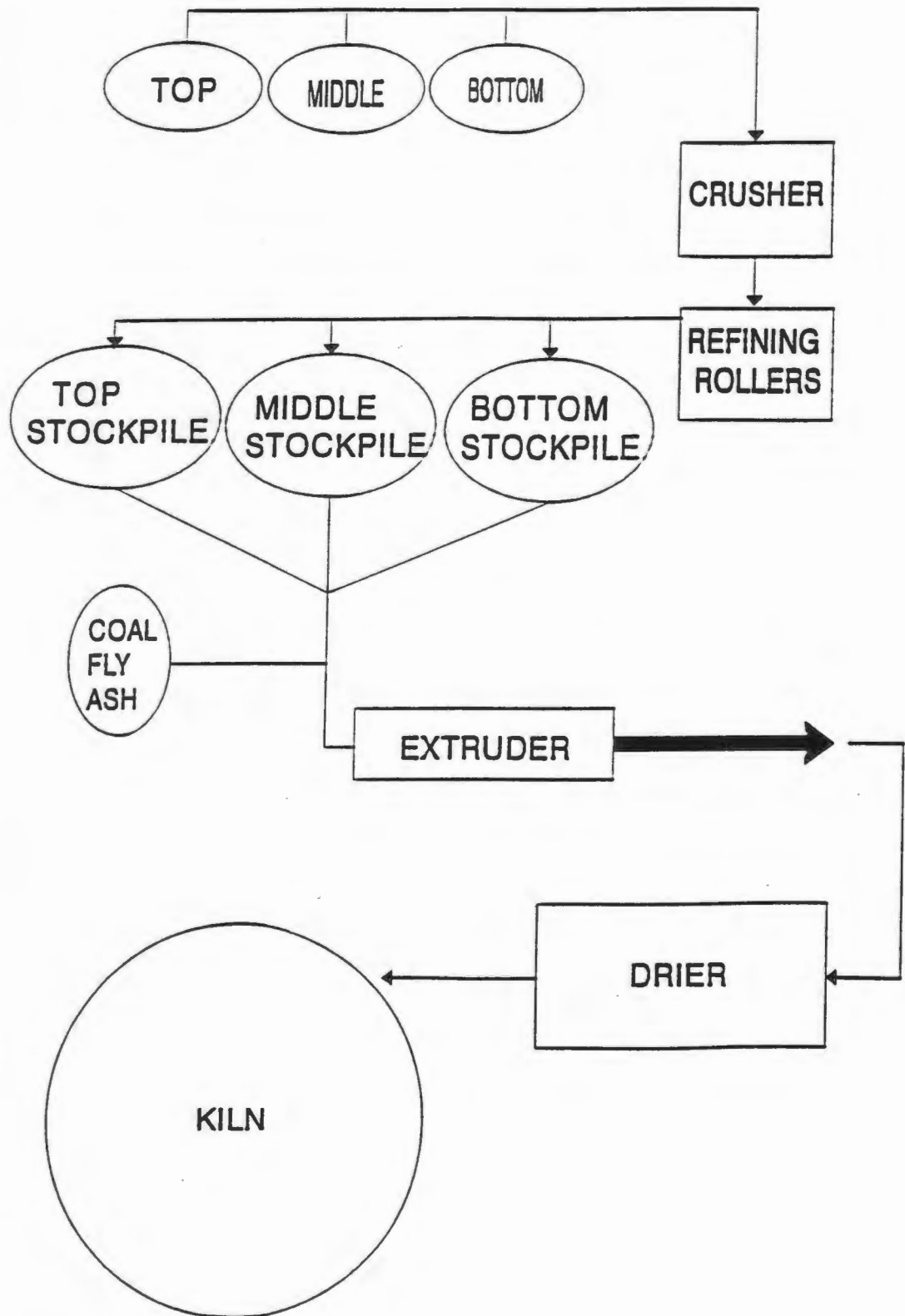
Figure 1. Schematic diagram of the process
