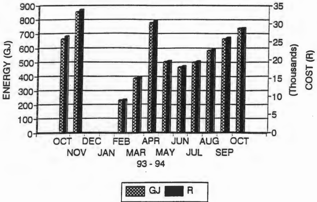
Figure 7. Diesel consumption
