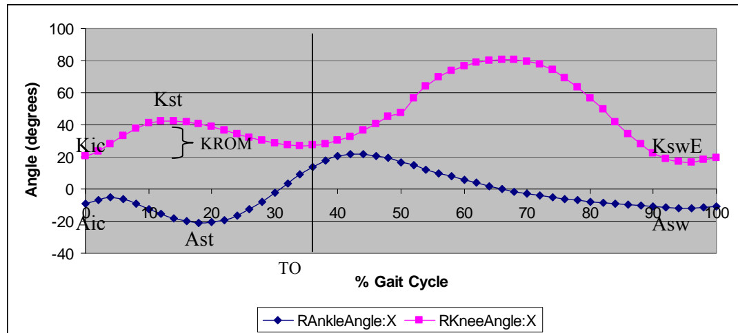
Figure 3.6. Typical knee and ankle kinematics during running - sagittal plane. Abbreviations: TO = toe-off, Kic = knee angle at initial contact, Kst = knee angle at stance phase, KROM = knee range of motion, Aic = ankle angle at initial contact, Ast = angle at stance phase.
