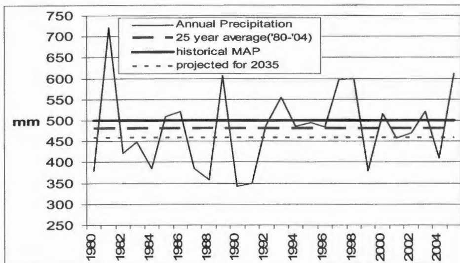
Figure 3: Annual precipitation for Bredasdorp
