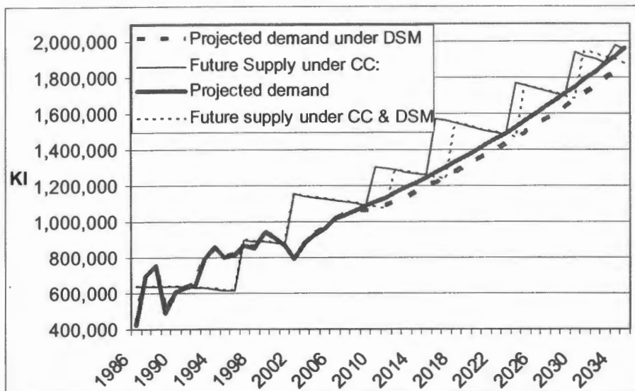
Figure 8: Projected water supply till 2035 under climate change and DSM conditions
