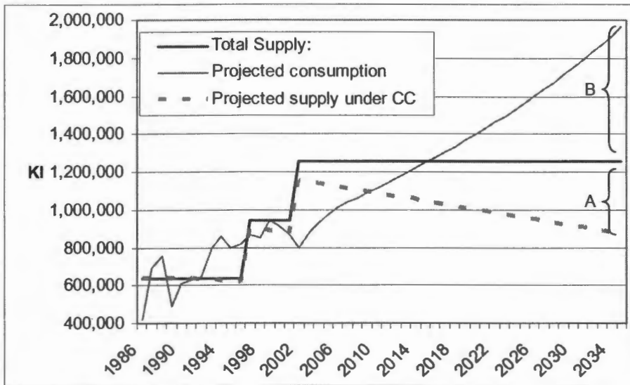
Figure 4: Water supply and demand graph under historical and climate change conditions for Bredasdorp
