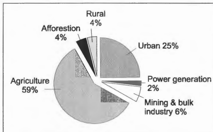
Figure 1: Water demand for 2000 per sector
