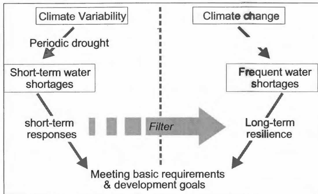
Figure 2: Diagrammatic view of the linkage between climate variability and climate change
